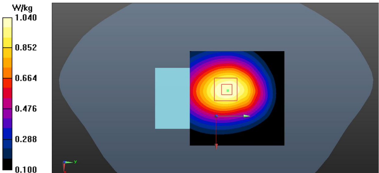
Fig.2 GSM 850 Body-worn
