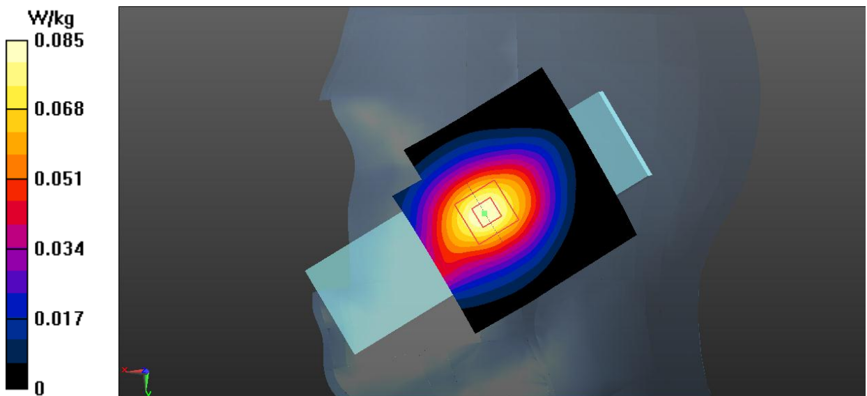
Fig.3 GSM 1900 Head
