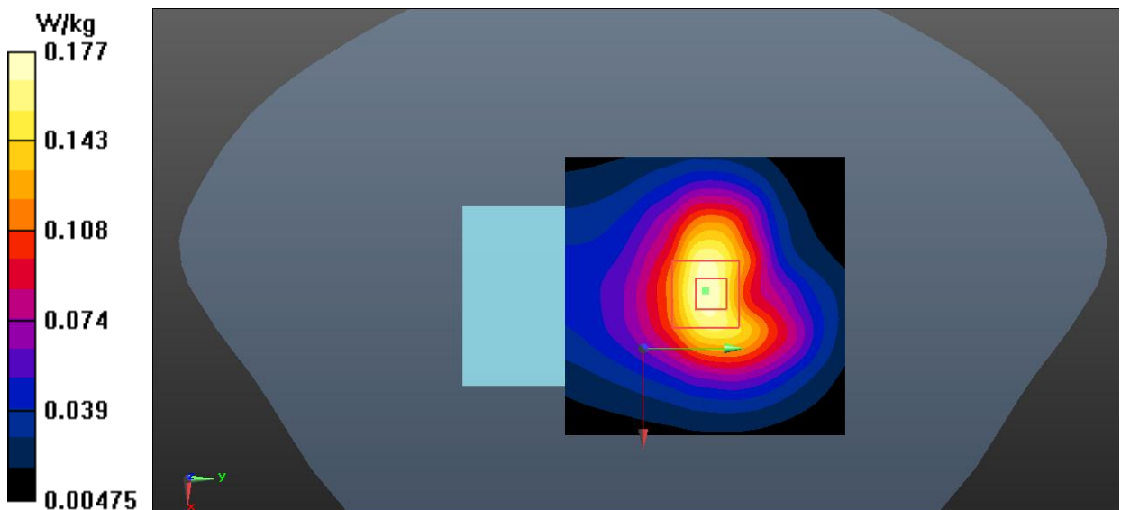
Fig.4 GSM 1900 Body-worn
