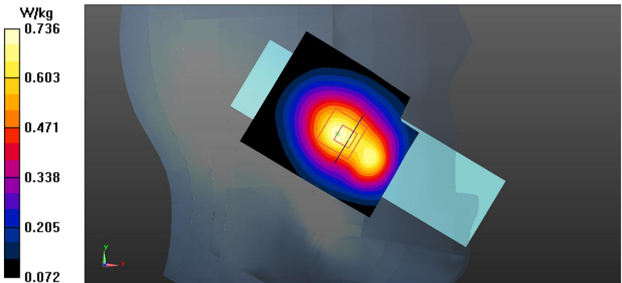
Fig.1 GSM 850 Head
