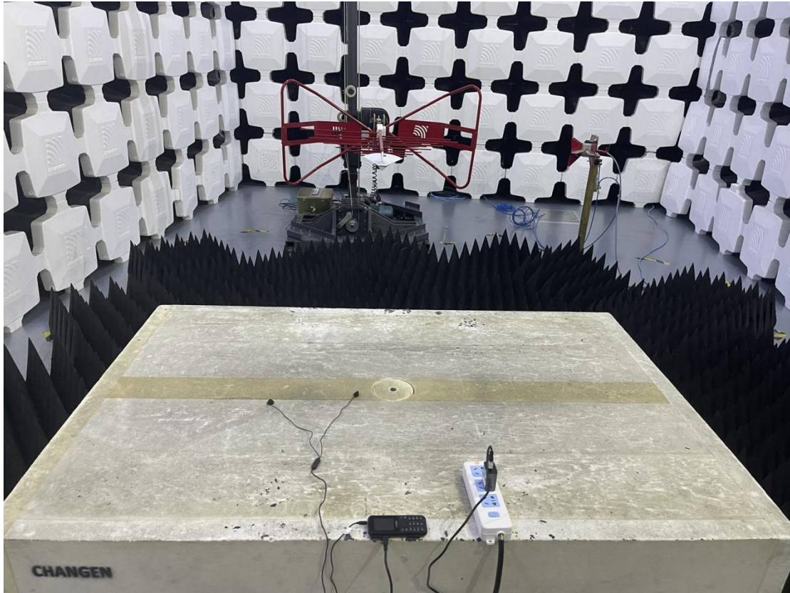
4. Radiated Emissions (Part 15B, Camera/GSM receiver, 1GHz-18GHz)
