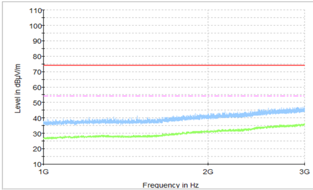
Fig.2. Radiated Emission (Charging Mode, 1GHz to 3GHz)
