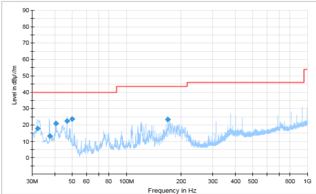
Fig.1. Radiated Emission (Charging Mode, 30MHz to 1GHz)
