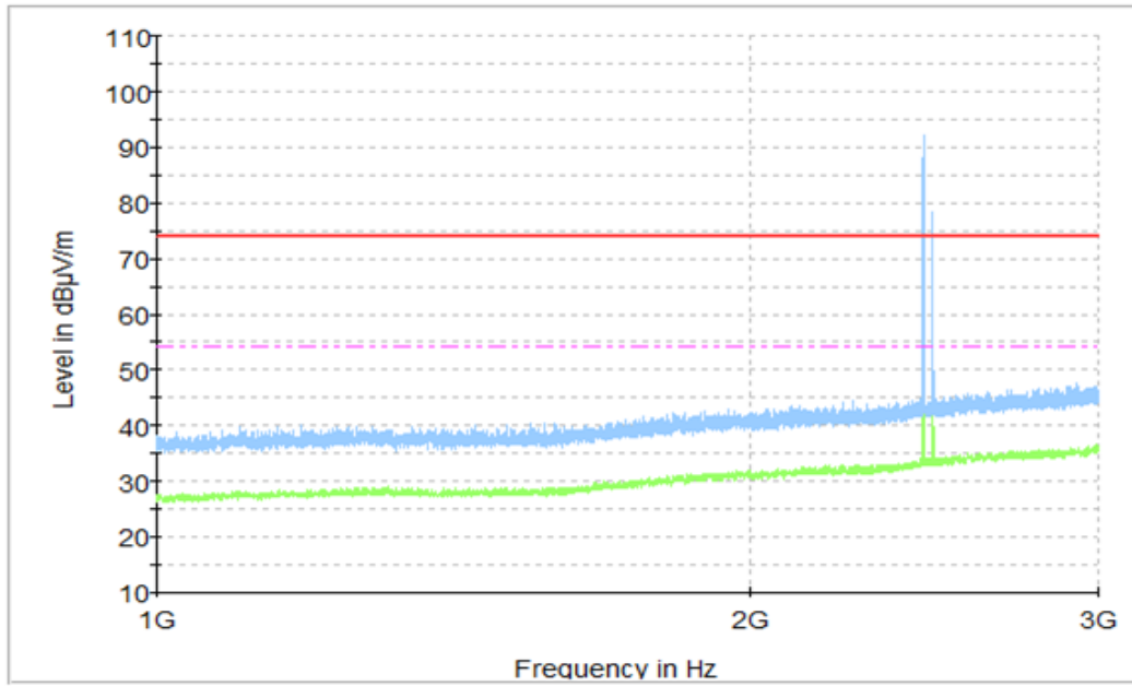
Fig.5. Radiated Emission (Normal Workingz, 1GHz to 3GHz)
