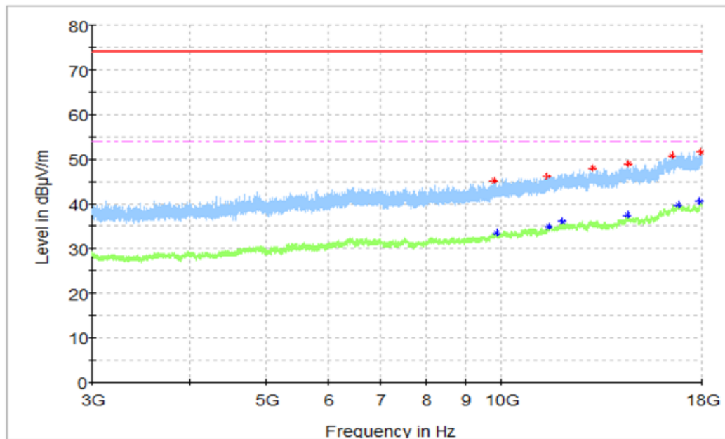
Fig.3. Radiated Emission (Charging Mode, 3GHz to 18GHz)
