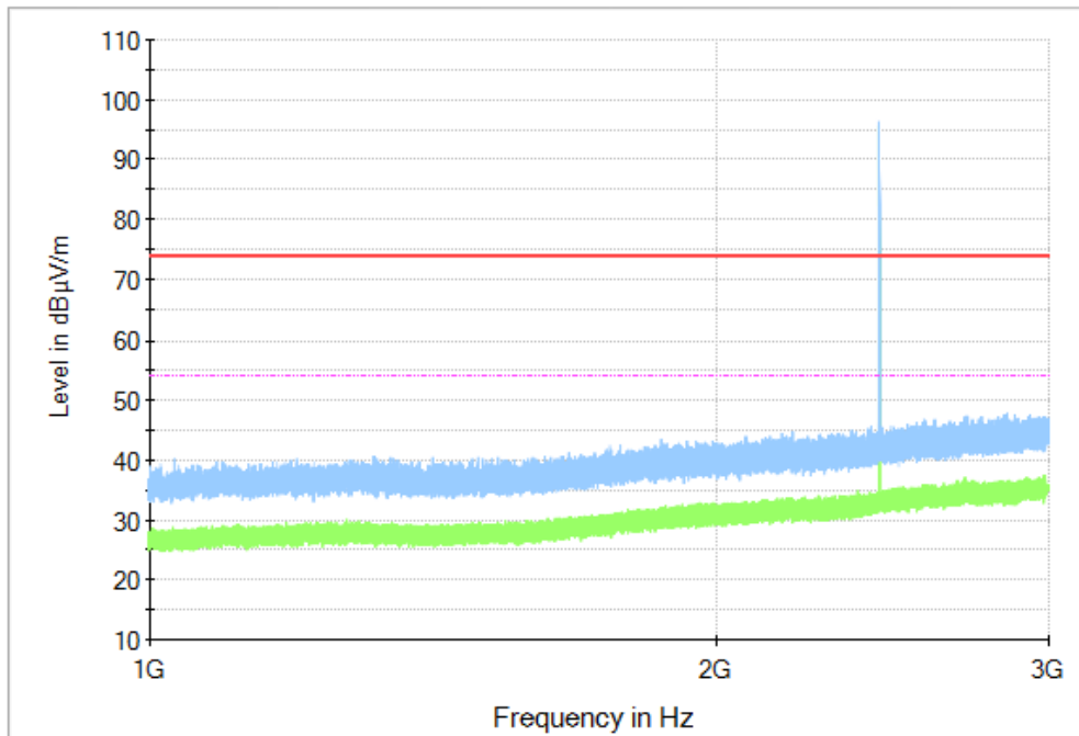
Fig. 35 Radiated Spurious Emission (GFSK, Ch39, 1 GHz ~3 GHz)
