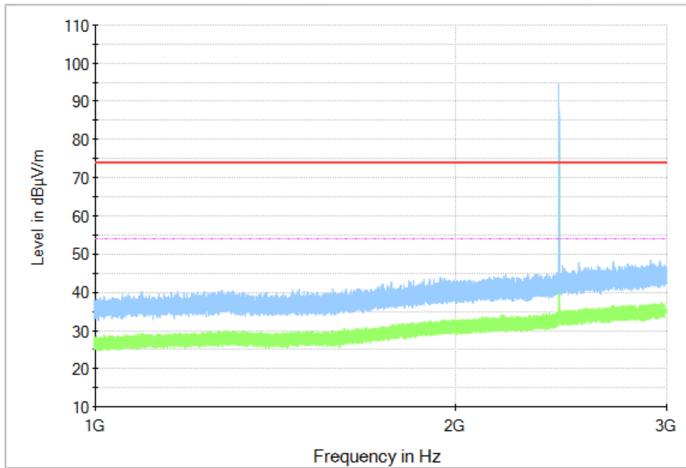
Fig. 51 Radiated Spurious Emission (8DPSK, Ch39, 1 GHz ~3 GHz)
