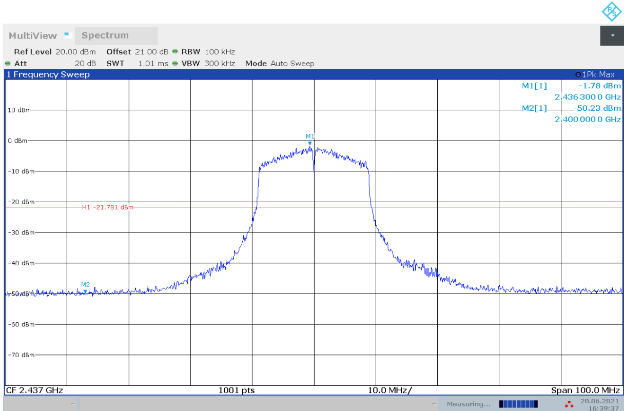
Fig.A.6.1.51 Transmitter Spurious Emission - Conducted (802.11n-HT20, Ch6, Center Frequency)
