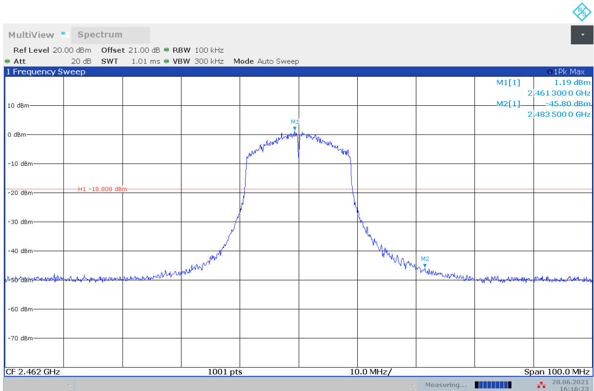
Fig.A.6.1.29 Transmitter Spurious Emission - Conducted (802.11n-HT20, Ch11, Center Frequency)
