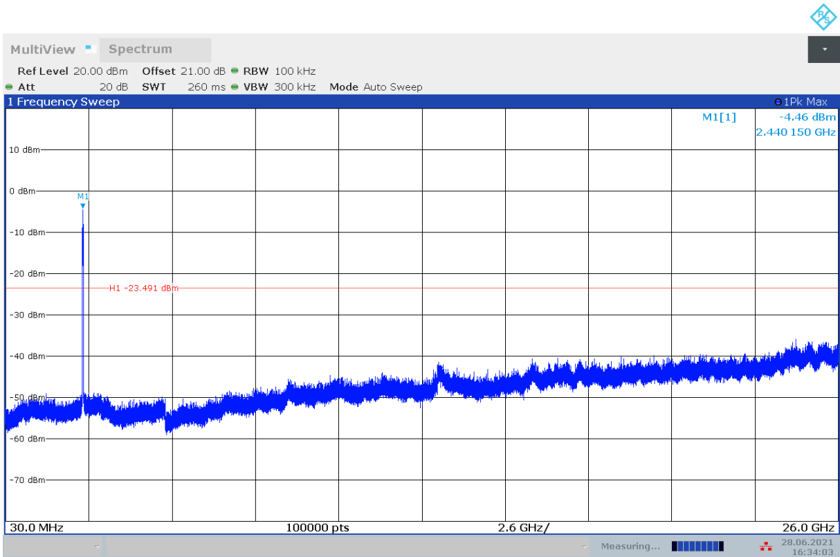
Fig.A.6.1.46 Transmitter Spurious Emission - Conducted (802.11n-HT40, Ch6, 30 MHz-26 GHz)
