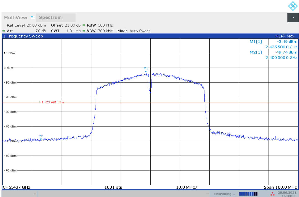
Fig.A.6.1.45 Transmitter Spurious Emission - Conducted (802.11n-HT40, Ch6, Center Frequency)
