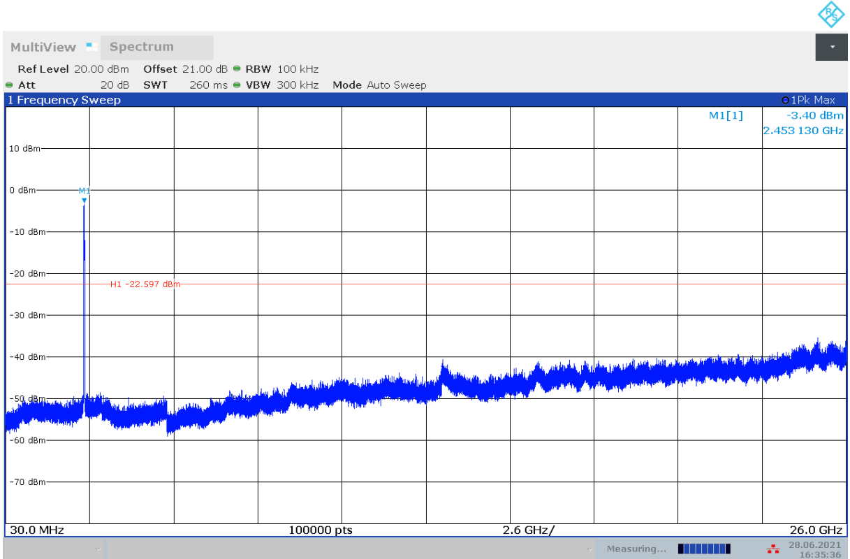
Fig.A.6.1.48 Transmitter Spurious Emission - Conducted (802.11n-HT40, Ch9, 30 MHz-26 GHz)
