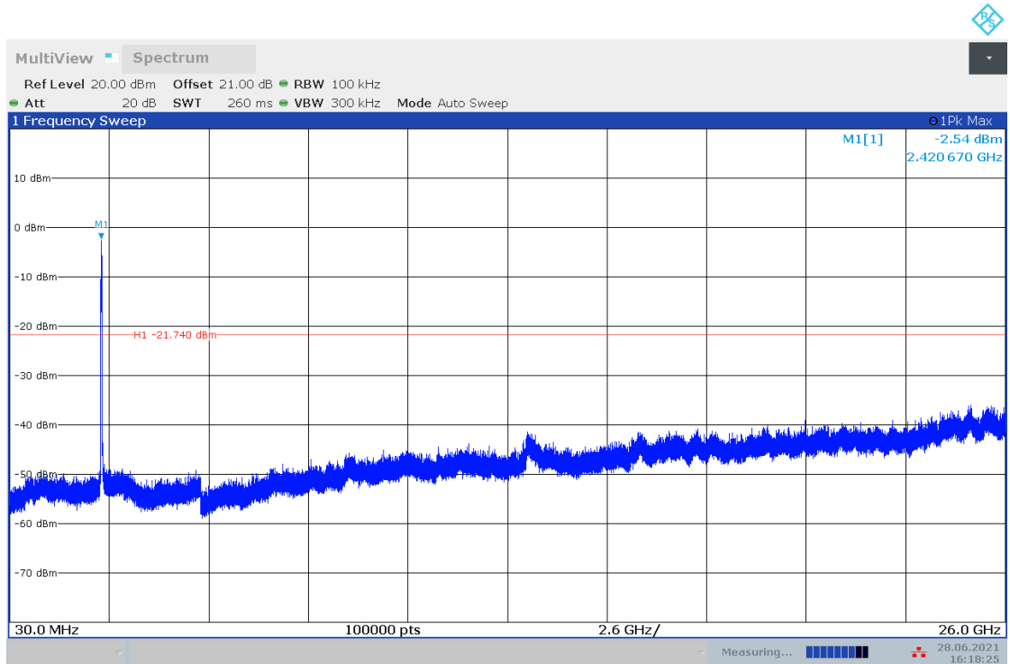
Fig.A.6.1.32 Transmitter Spurious Emission - Conducted (802.11n-HT40, Ch3, 30 MHz-26 GHz)
