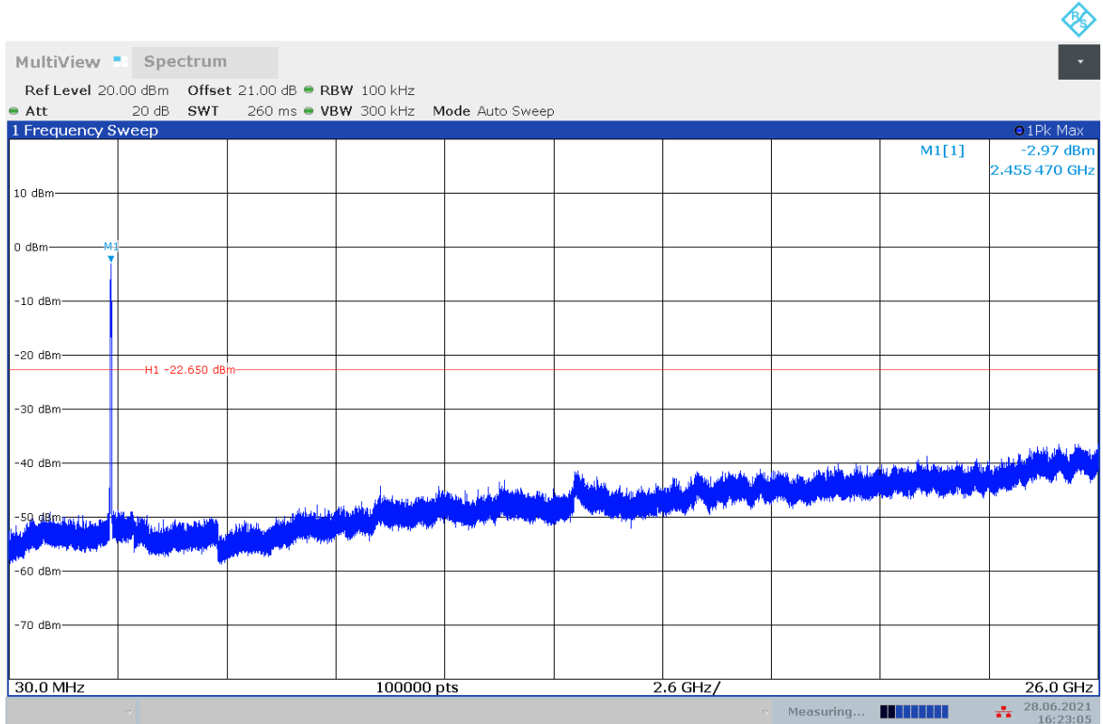
Fig.A.6.1.36 Transmitter Spurious Emission - Conducted (802.11n-HT40, Ch9, 30 MHz-26 GHz)
