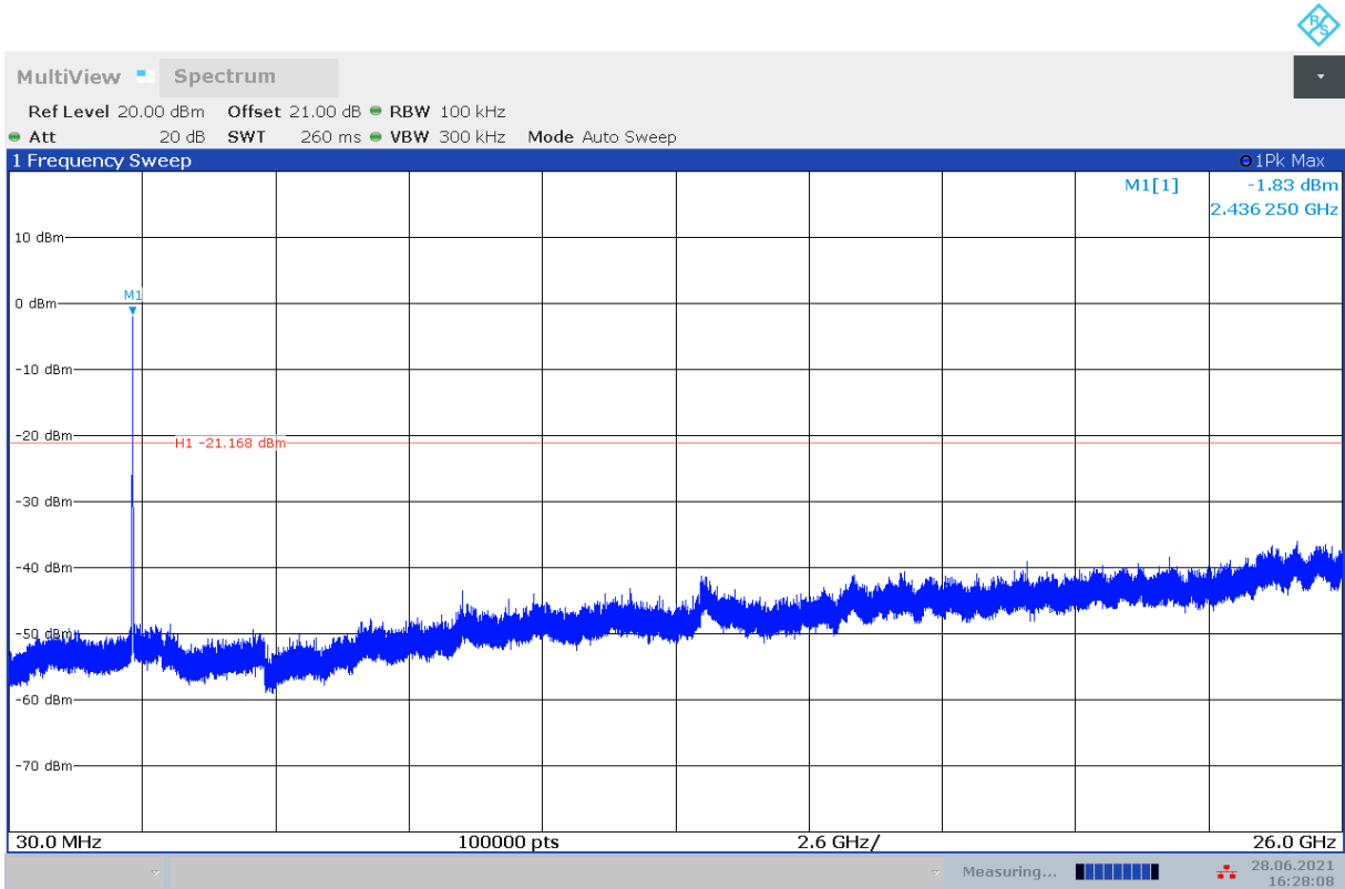
Fig.A.6.1.40 Transmitter Spurious Emission - Conducted (802.11n-HT20, Ch6, 30 MHz-26 GHz)
