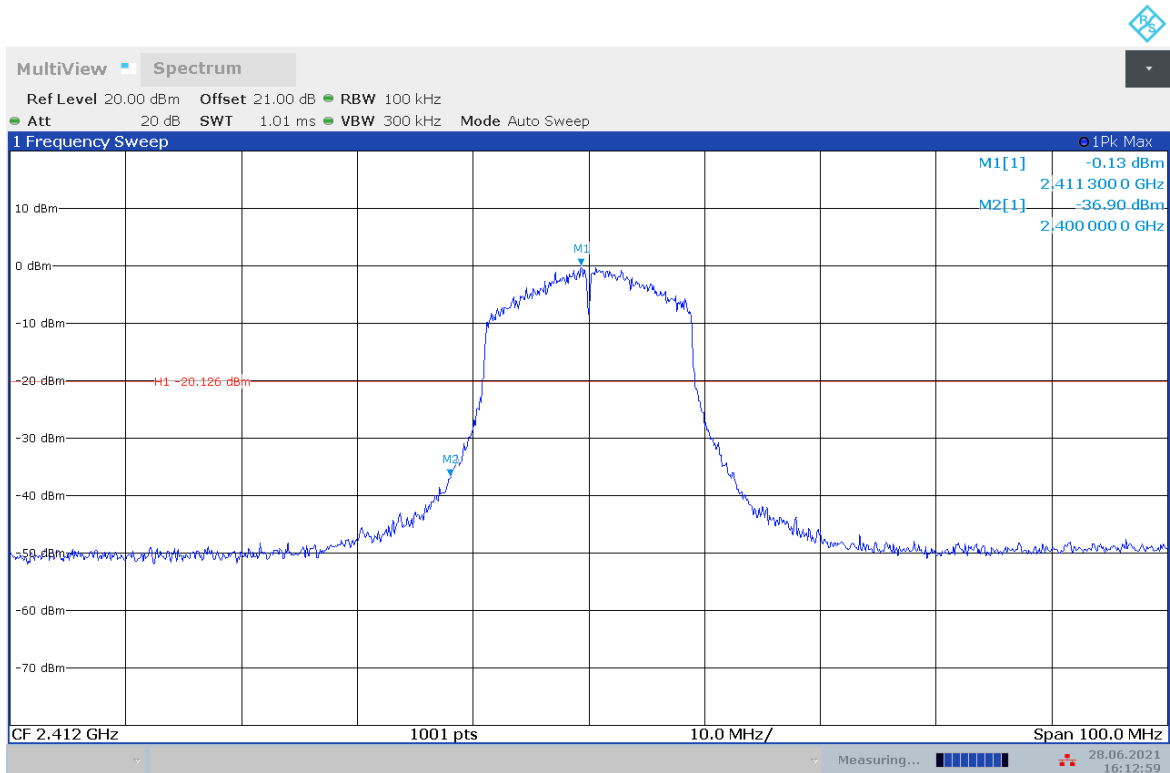
Fig.A.6.1.25 Transmitter Spurious Emission - Conducted (802.11n-HT20, Ch1, Center Frequency)
