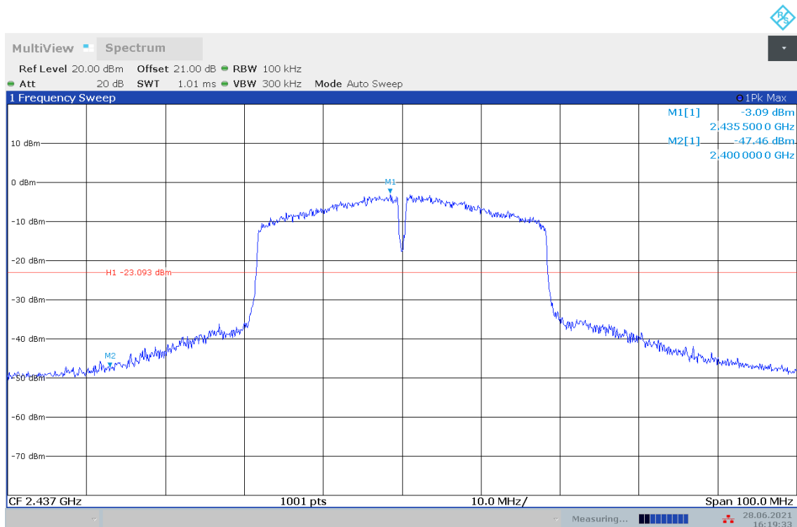
Fig.A.6.1.33 Transmitter Spurious Emission - Conducted (802.11n-HT40, Ch6, Center Frequency)
