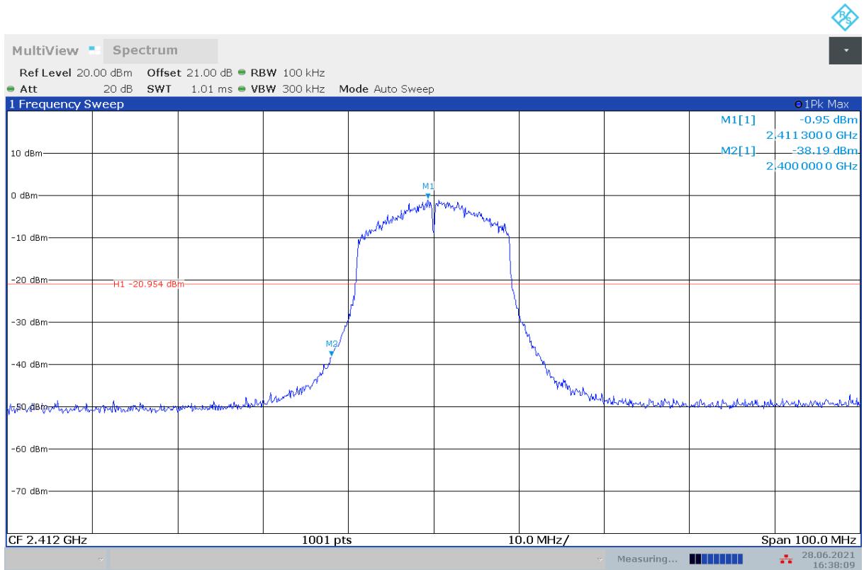
Fig.A.6.1.49 Transmitter Spurious Emission - Conducted (802.11n-HT20, Ch1, Center Frequency)
