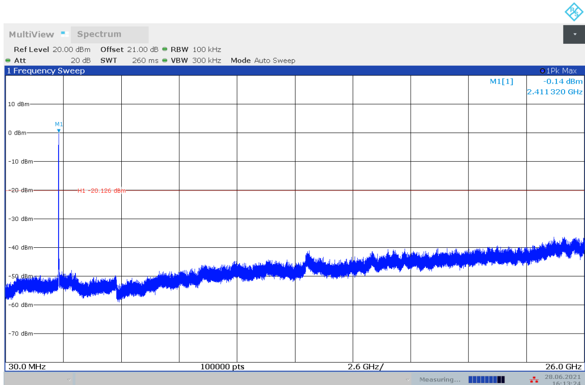
Fig.A.6.1.26 Transmitter Spurious Emission - Conducted (802.11n-HT20, Ch1, 30 MHz-26 GHz)
