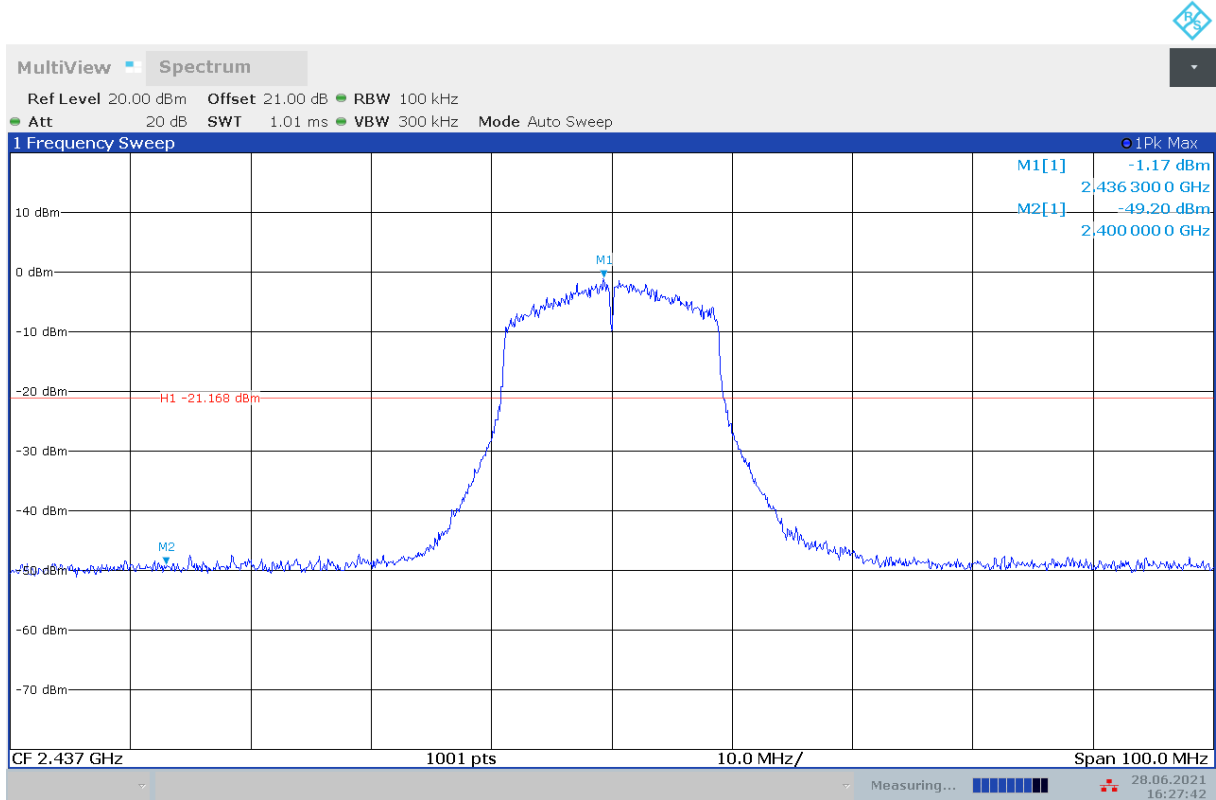
Fig.A.6.1.39 Transmitter Spurious Emission - Conducted (802.11n-HT20, Ch6, Center Frequency)
