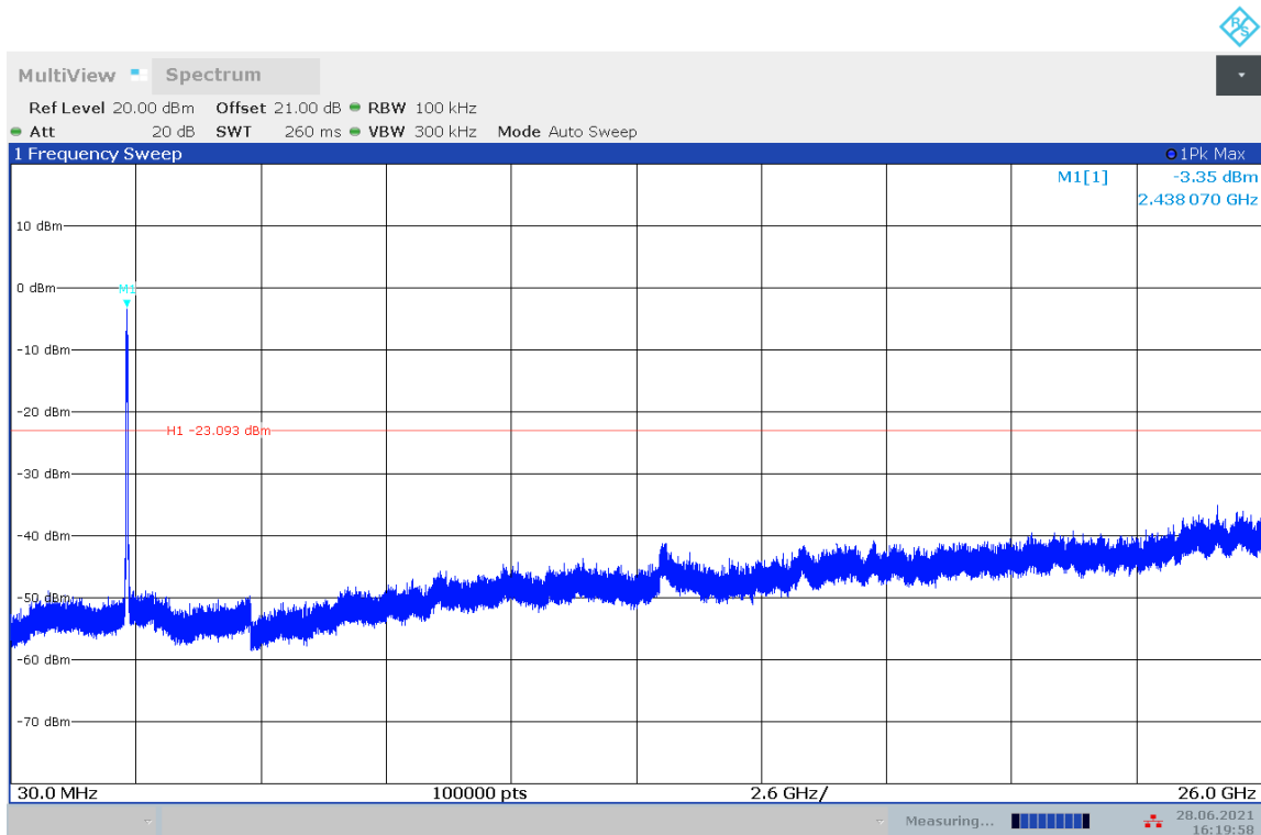
Fig.A.6.1.34 Transmitter Spurious Emission - Conducted (802.11n-HT40, Ch6, 30 MHz-26 GHz)
