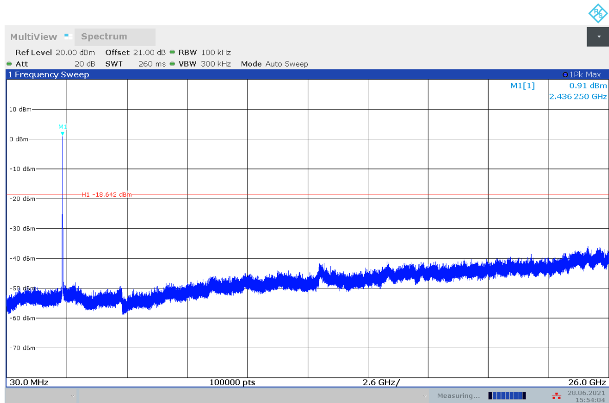
Fig.A.6.1.10 Transmitter Spurious Emission - Conducted (802.11g, Ch6, 30 MHz-26
