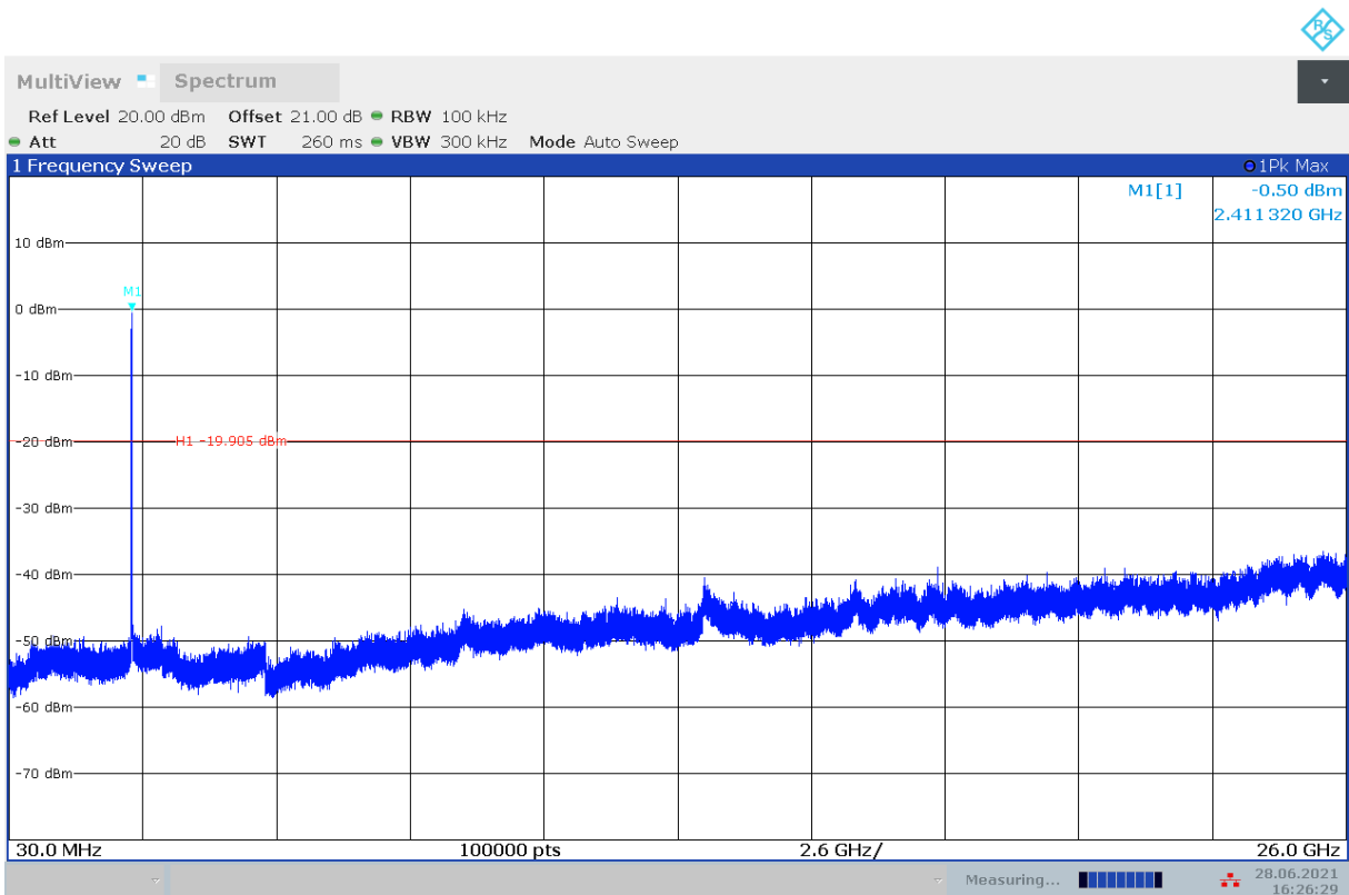
Fig.A.6.1.37 Transmitter Spurious Emission - Conducted (802.11n-HT20, Ch1, Center Frequency)
