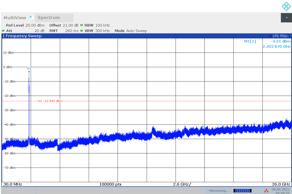
Fig.A.6.1.59 Transmitter Spurious Emission - Conducted (802.11n-HT40, Ch9, Center Frequency)
