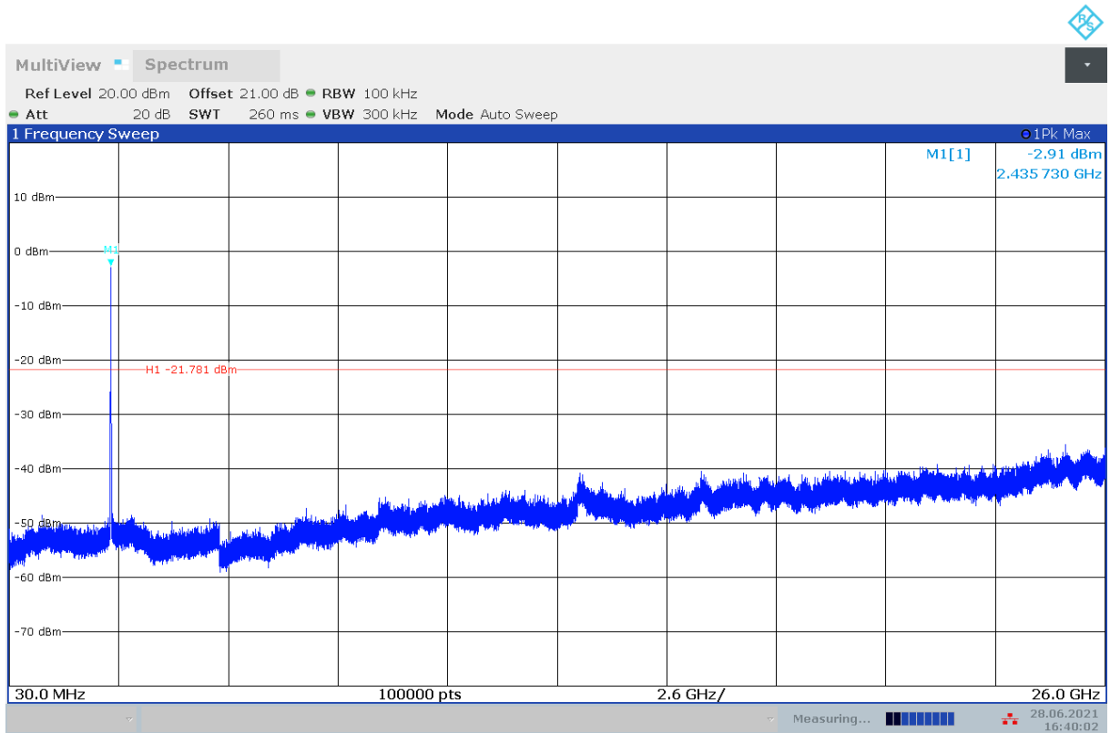
Fig.A.6.1.52 Transmitter Spurious Emission - Conducted (802.11n-HT20, Ch6, 30 MHz-26 GHz)
