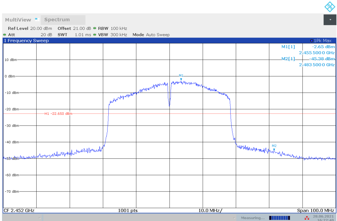
Fig.A.6.1.35 Transmitter Spurious Emission - Conducted (802.11n-HT40, Ch9, Center Frequency)
