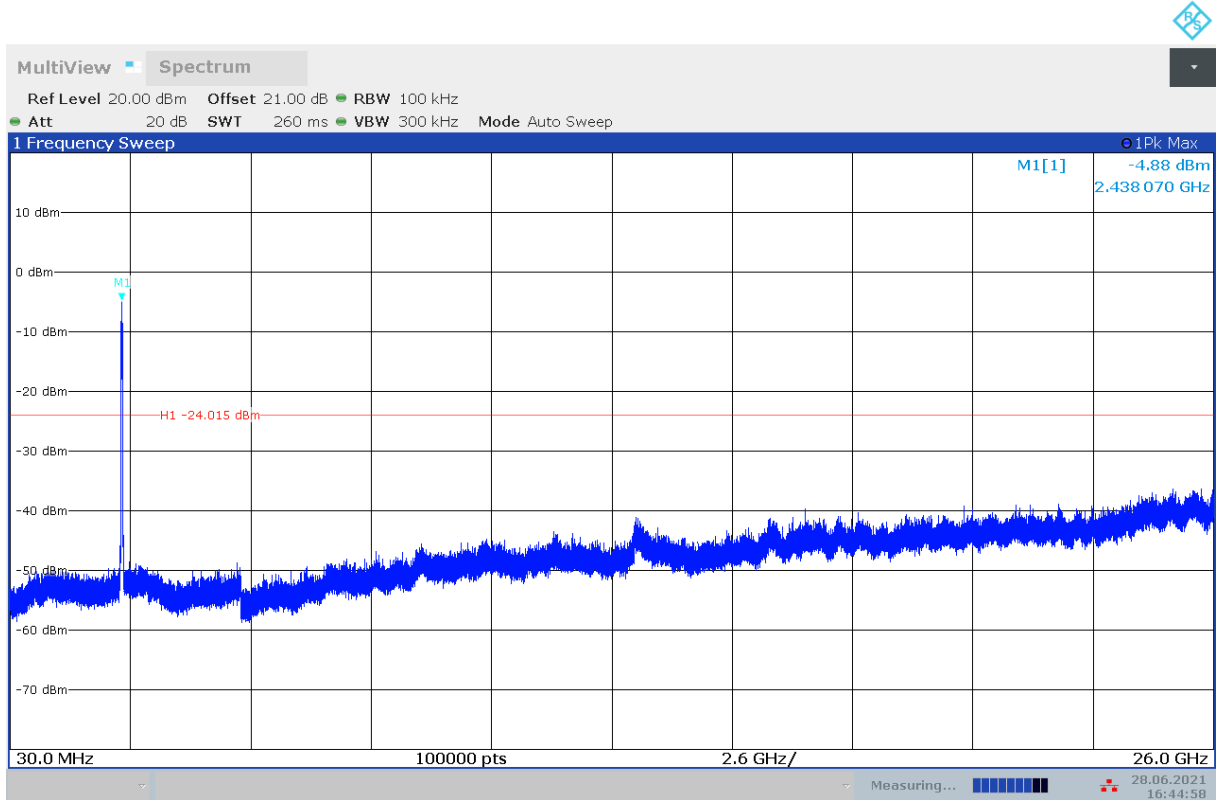
Fig.A.6.1.58 Transmitter Spurious Emission - Conducted (802.11n-HT40, Ch6, 30 MHz-26 GHz)
