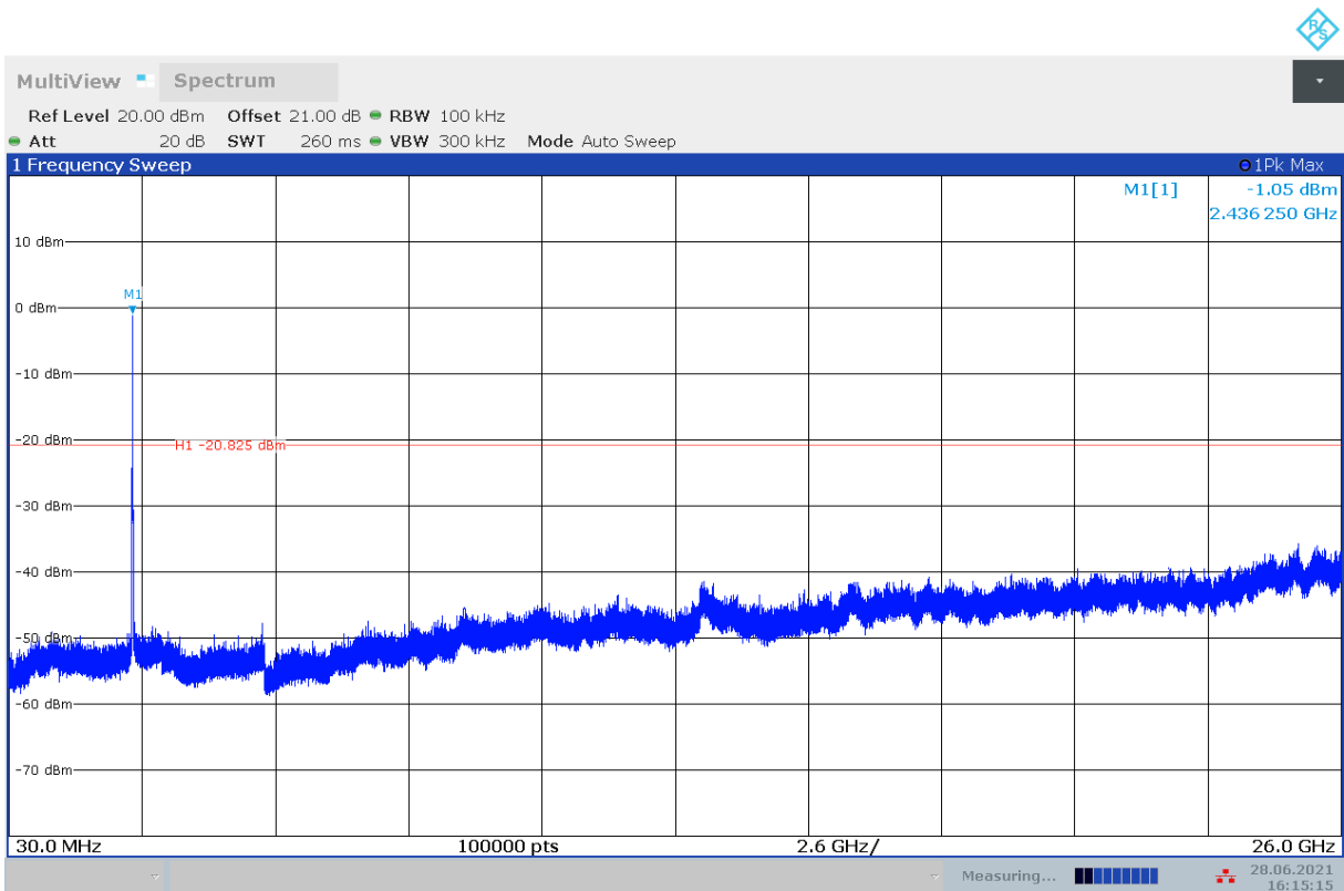
Fig.A.6.1.27 Transmitter Spurious Emission - Conducted (802.11n-HT20, Ch6, Center Frequency)
