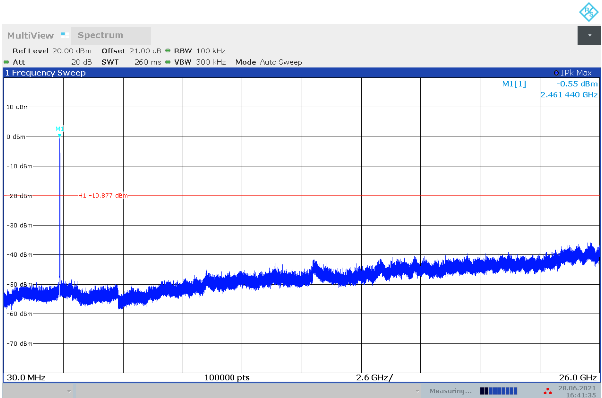
Fig.A.6.1.54 Transmitter Spurious Emission - Conducted (802.11n-HT20, Ch11, 30 MHz-26 GHz)
