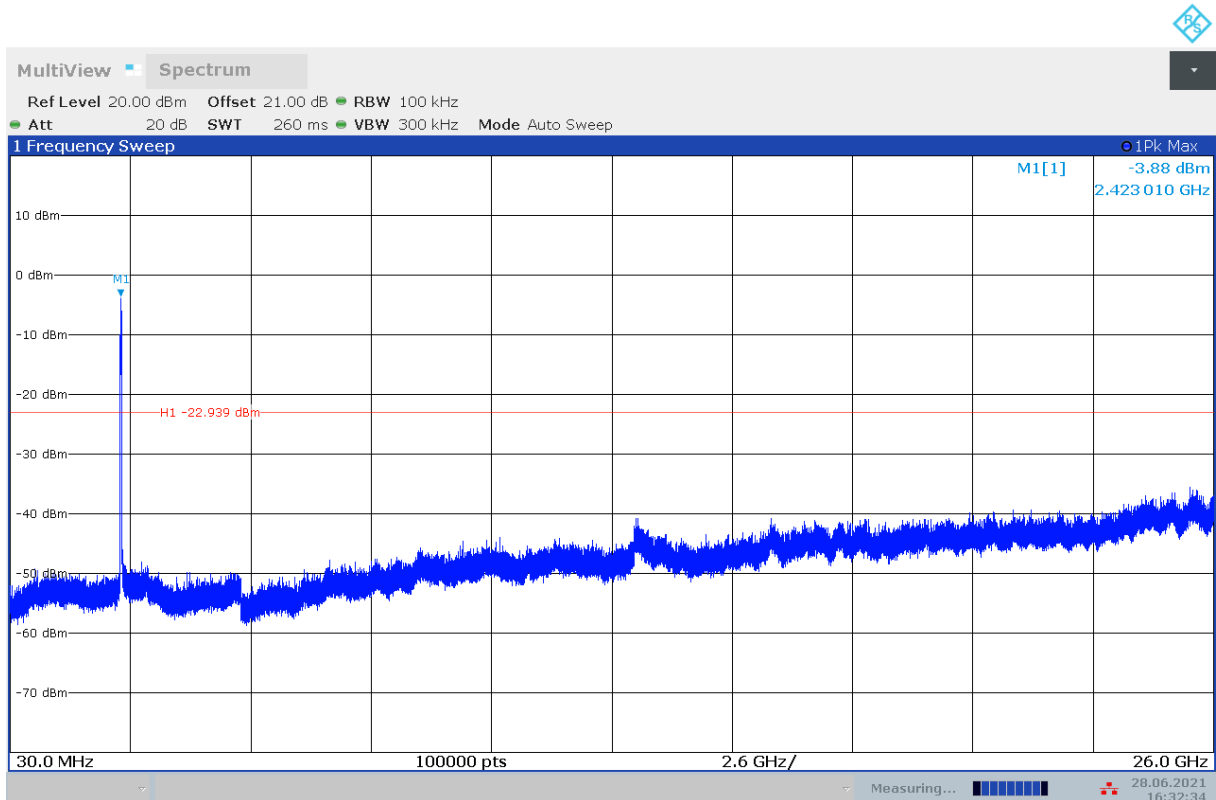
Fig.A.6.1.43 Transmitter Spurious Emission - Conducted (802.11n-HT40, Ch3, Center Frequency)
