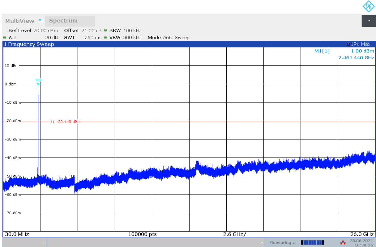
Fig.A.6.1.42 Transmitter Spurious Emission - Conducted (802.11n-HT20, Ch11, 30 MHz-26 GHz)
