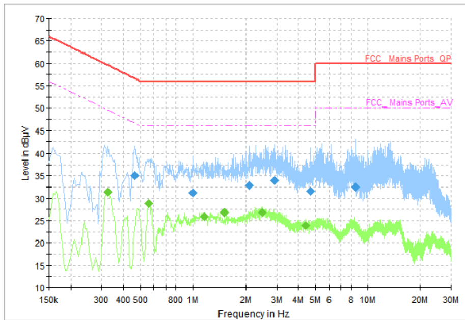
Fig.70 AC Power line Conducted Emission (Idle, AE3, 120V)
