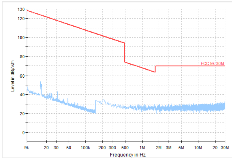
Fig.21 Radiated Spurious Emission (Ch19, 9kHz - 30MHz), 1M
