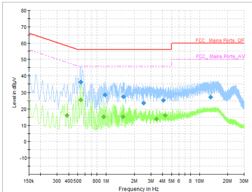
Fig.29 AC Power line Conducted Emission (Traffic, AE3, 120V), 1M
