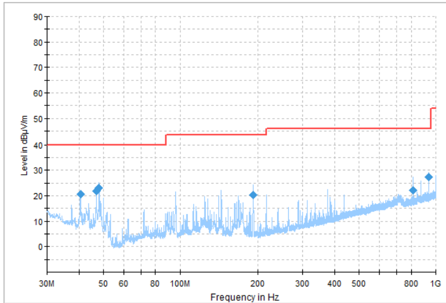
Fig.22 Radiated Spurious Emission (Ch19, 30MHz - 1GHz), 1M
