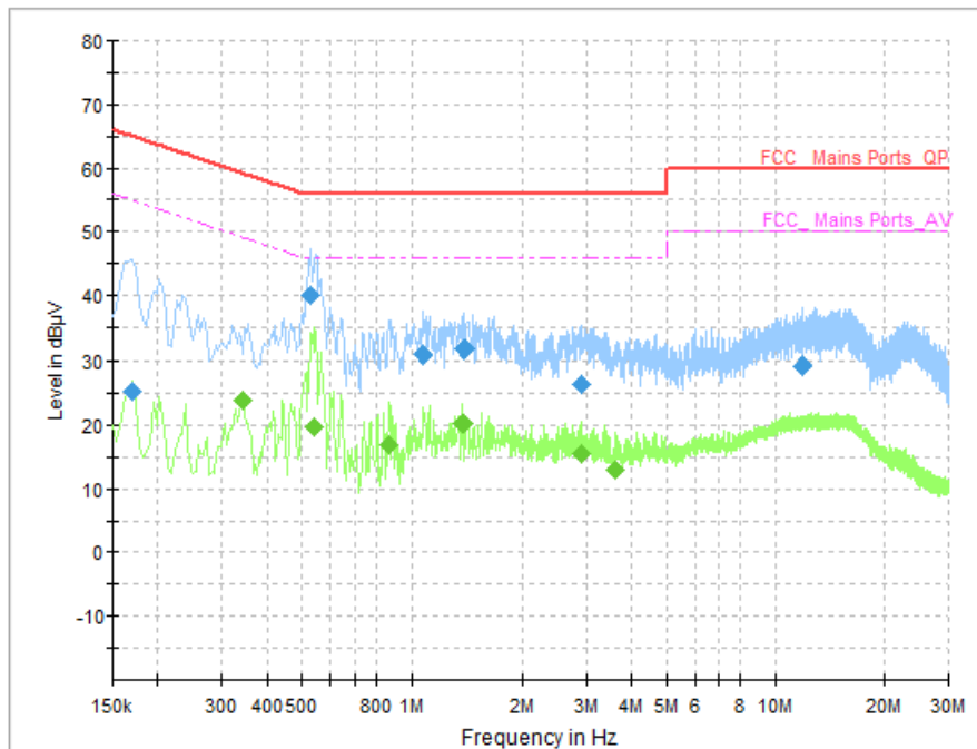
Fig.30 AC Power line Conducted Emission (Idle, AE3, 120V), 1M
