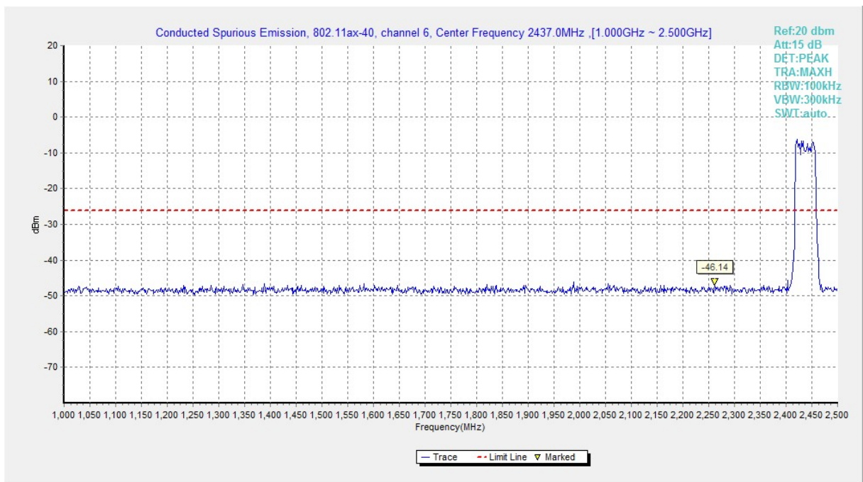
Fig.A.6.1.275 Transmitter Spurious Emission - Conducted (802.11ax-HE40, Ch6, 1 GHz-2.5 GHz)
