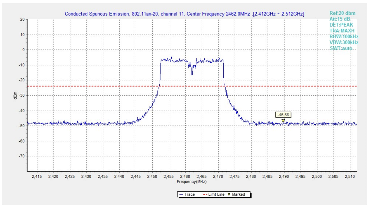
Fig.A.6.1.257 Transmitter Spurious Emission - Conducted (802.11ax-HE20, Ch11, Center Frequency)
