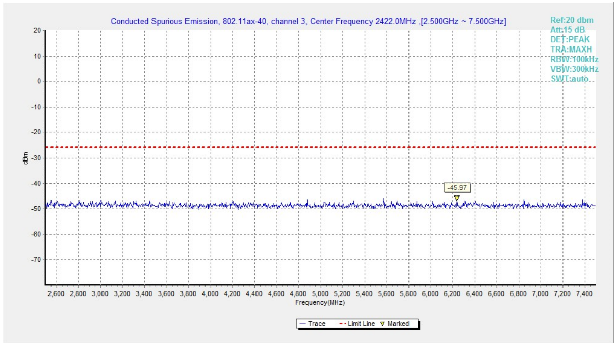
Fig.A.6.1.268 Transmitter Spurious Emission - Conducted (802.11ax-HE40, Ch3, 2.5 GHz-7.5 GHz)
