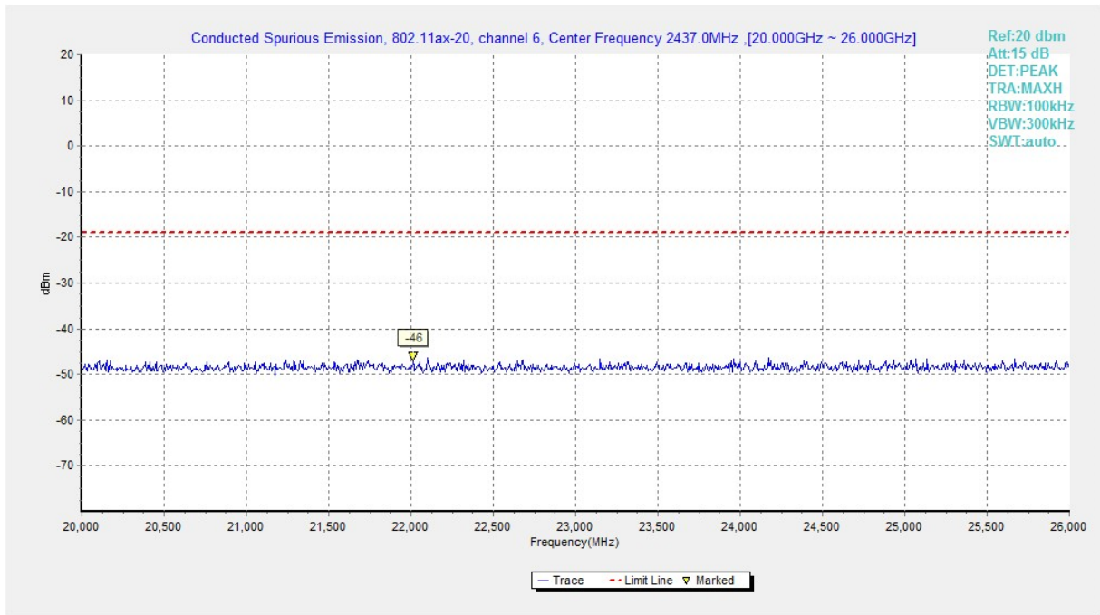
Fig.A.6.1.256 Transmitter Spurious Emission - Conducted (802.11ax-HE20, Ch6, 20 GHz-26 GHz)
