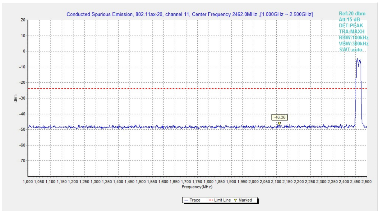
Fig.A.6.1.259 Transmitter Spurious Emission - Conducted (802.11ax-HE20, Ch11, 1 GHz-2.5 GHz)
