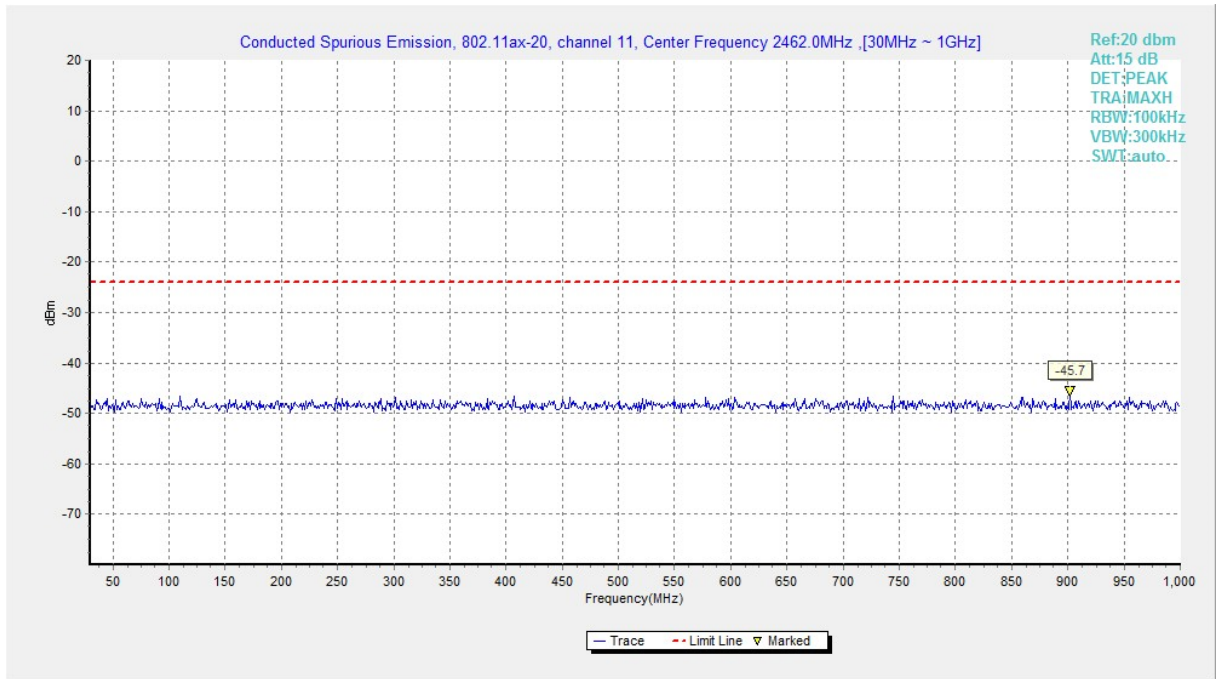
Fig.A.6.1.258 Transmitter Spurious Emission - Conducted (802.11ax-HE20, Ch11, 30 MHz-1 GHz)
