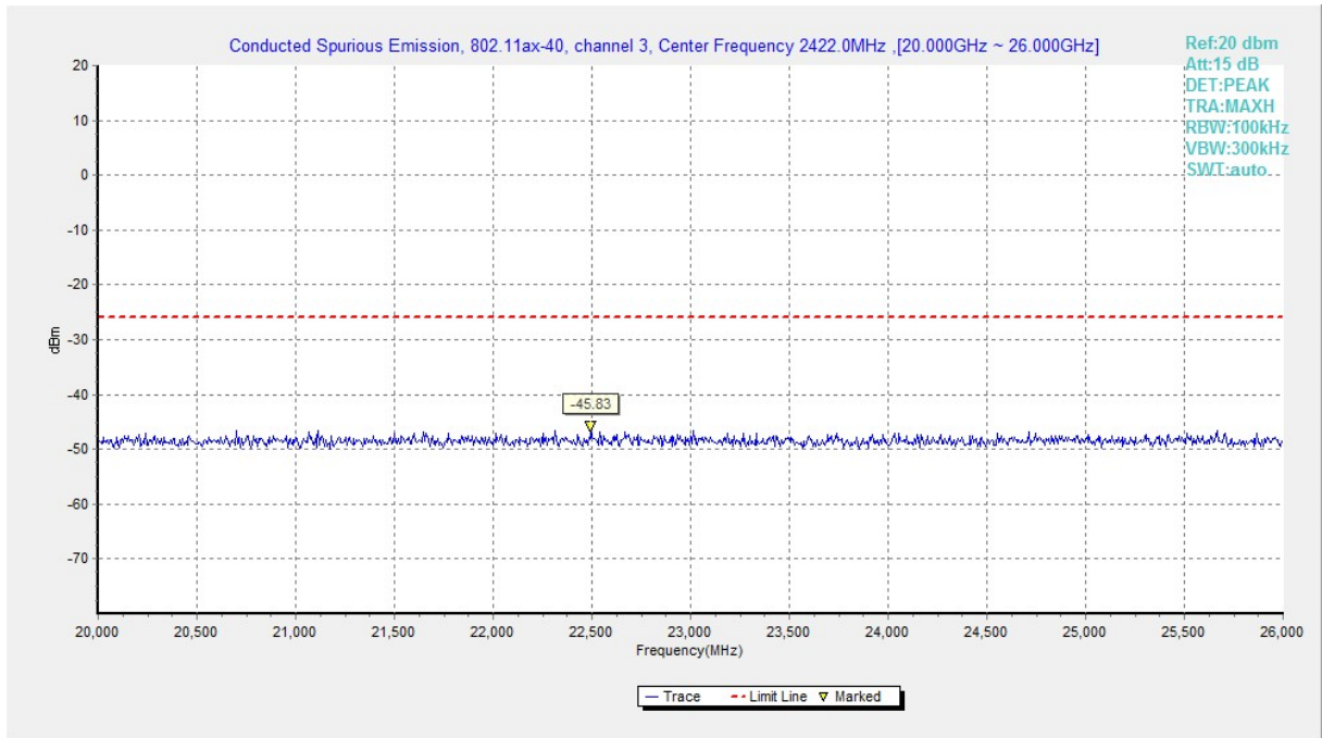
Fig.A.6.1.272 Transmitter Spurious Emission - Conducted (802.11ax-HE40, Ch3, 20 GHz-26 GHz)
