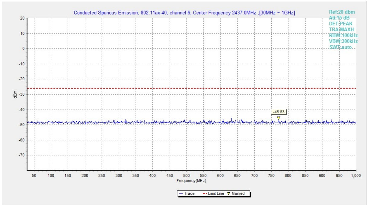
Fig.A.6.1.274 Transmitter Spurious Emission - Conducted (802.11ax-HE40, Ch6, 30 MHz-1 GHz)
