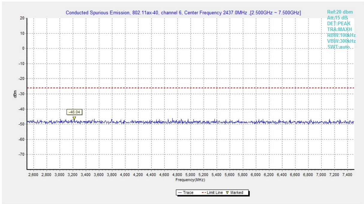
Fig.A.6.1.276 Transmitter Spurious Emission - Conducted (802.11ax-HE40, Ch6, 2.5 GHz-7.5 GHz)
