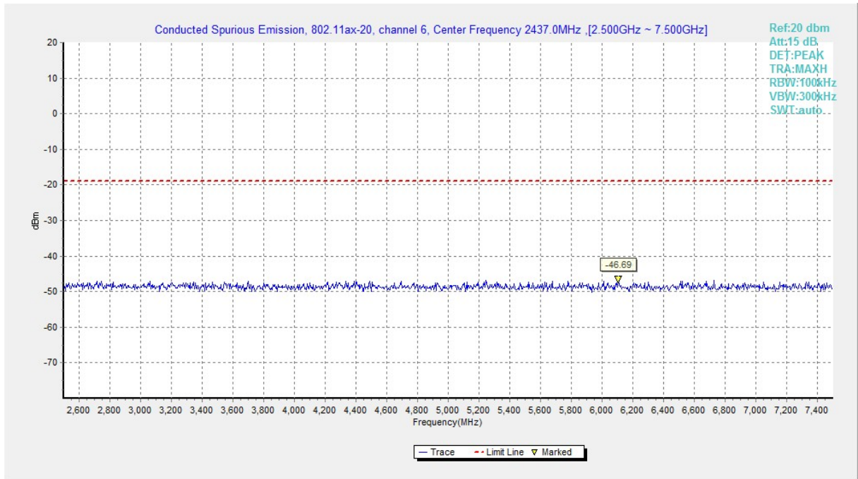
Fig.A.6.1.252 Transmitter Spurious Emission - Conducted (802.11ax-HE20, Ch6, 2.5 GHz-7.5 GHz)
