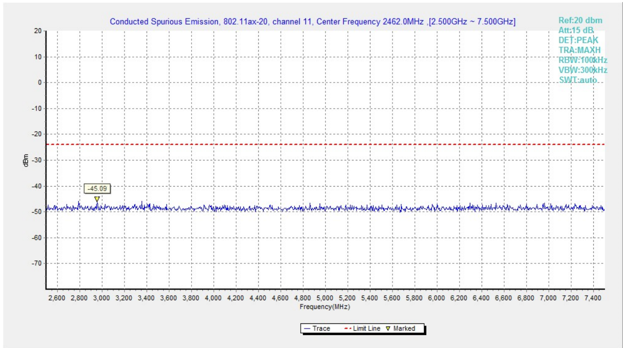
Fig.A.6.1.260 Transmitter Spurious Emission - Conducted (802.11ax-HE20, Ch11, 2.5 GHz-7.5 GHz)
