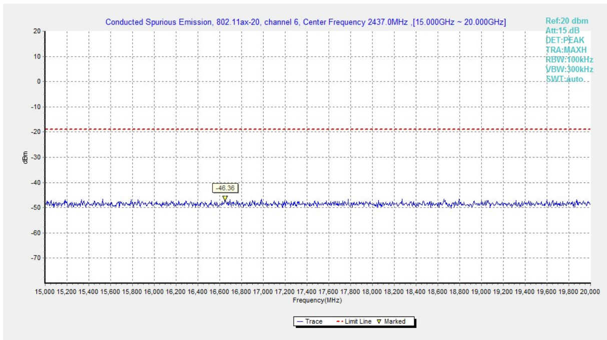
Fig.A.6.1.255 Transmitter Spurious Emission - Conducted (802.11ax-HE20, Ch6, 15 GHz-20 GHz)
