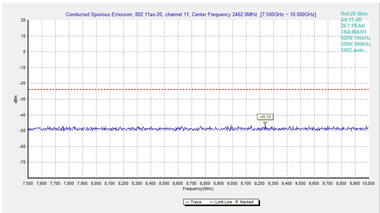
Fig.A.6.1.261 Transmitter Spurious Emission - Conducted (802.11ax-HE20, Ch11, 7.5 GHz-10 GHz)
