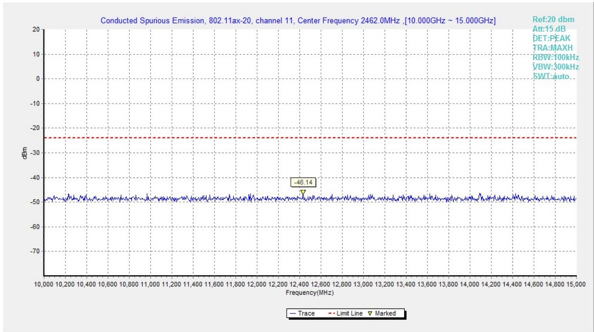
Fig.A.6.1.262 Transmitter Spurious Emission - Conducted (802.11ax-HE20, Ch11, 10 GHz-15 GHz)
