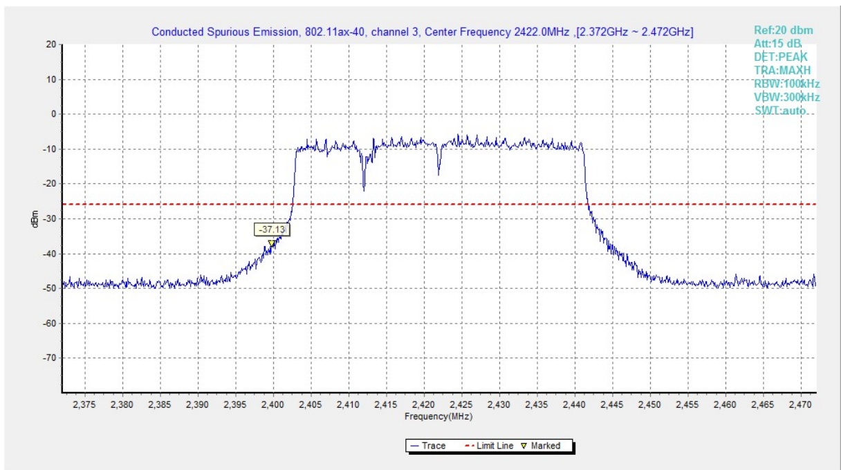
Fig.A.6.1.265 Transmitter Spurious Emission - Conducted (802.11ax-HE40, Ch3, Center Frequency)
