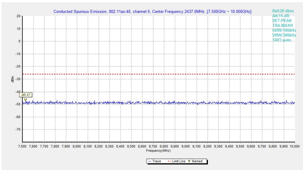
Fig.A.6.1.277 Transmitter Spurious Emission - Conducted (802.11ax-HE40, Ch6, 7.5 GHz-10 GHz)
