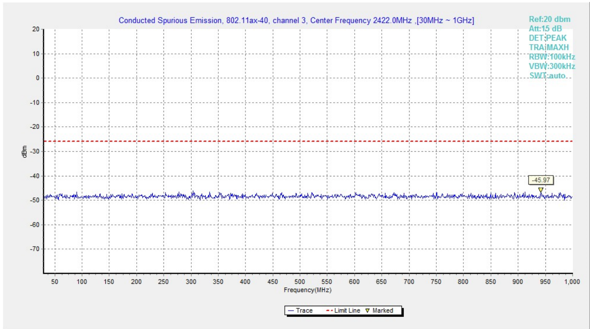
Fig.A.6.1.266 Transmitter Spurious Emission - Conducted (802.11ax-HE40, Ch3, 30 MHz-1 GHz)
