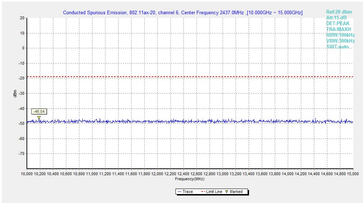
Fig.A.6.1.254 Transmitter Spurious Emission - Conducted (802.11ax-HE20, Ch6, 10 GHz-15 GHz)
