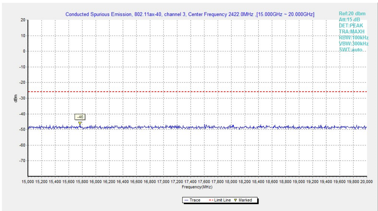
Fig.A.6.1.271 Transmitter Spurious Emission - Conducted (802.11ax-HE40, Ch3, 15 GHz-20 GHz)
