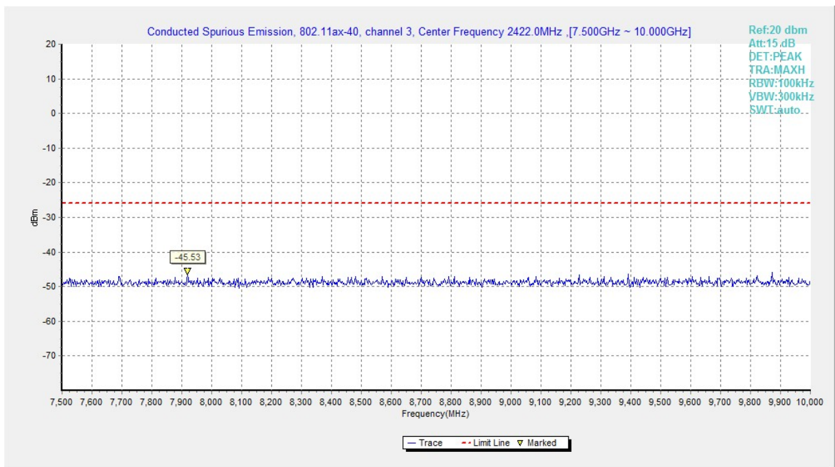
Fig.A.6.1.269 Transmitter Spurious Emission - Conducted (802.11ax-HE40, Ch3, 7.5 GHz-10 GHz)
