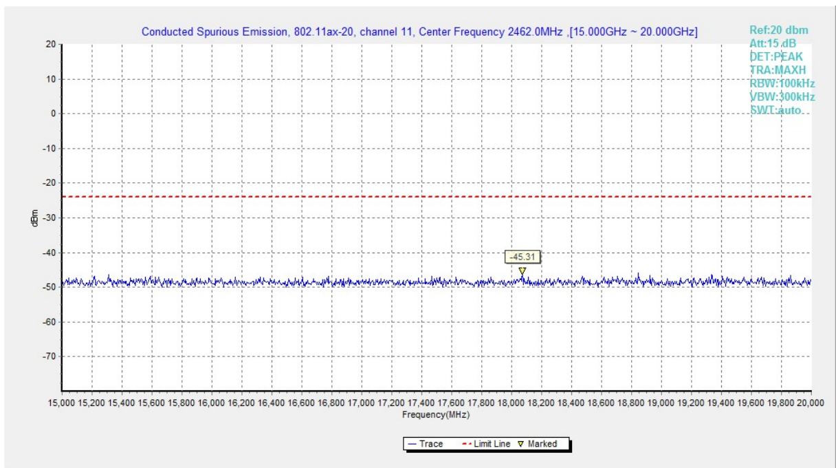
Fig.A.6.1.263 Transmitter Spurious Emission - Conducted (802.11ax-HE20, Ch11, 15 GHz-20 GHz)
