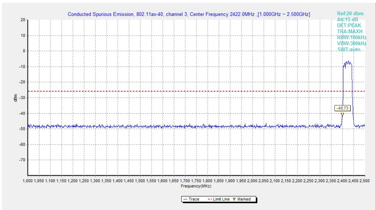
Fig.A.6.1.267 Transmitter Spurious Emission - Conducted (802.11ax-HE40, Ch3, 1 GHz-2.5 GHz)
