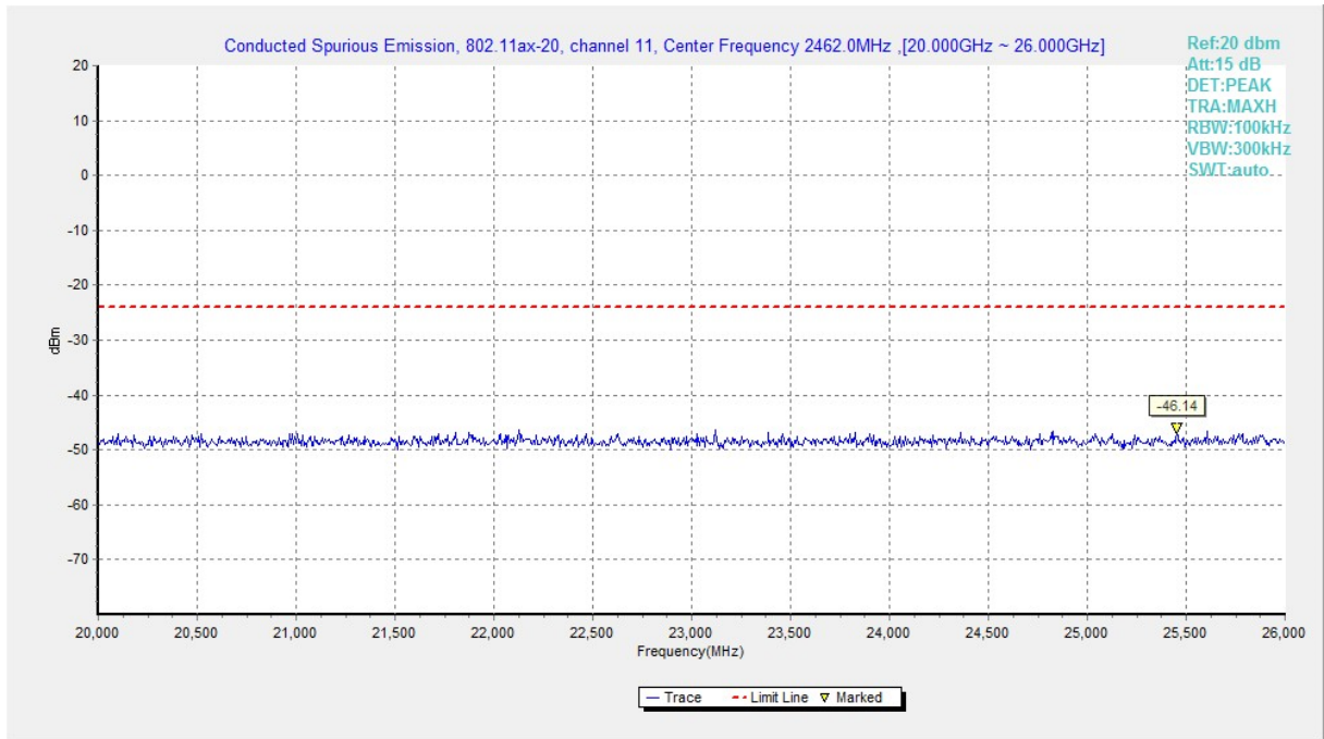
Fig.A.6.1.264 Transmitter Spurious Emission - Conducted (802.11ax-HE20, Ch11, 20 GHz-26 GHz)
