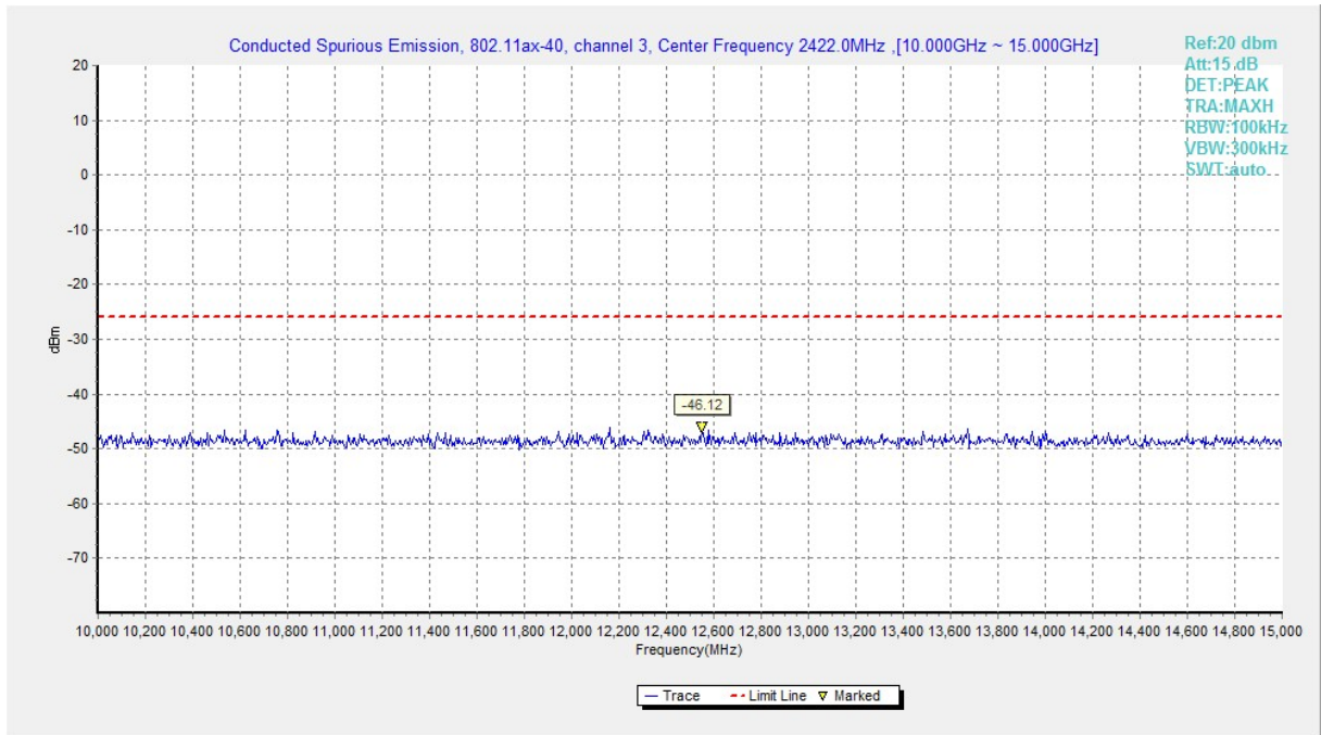
Fig.A.6.1.270 Transmitter Spurious Emission - Conducted (802.11ax-HE40, Ch3, 10 GHz-15 GHz)
