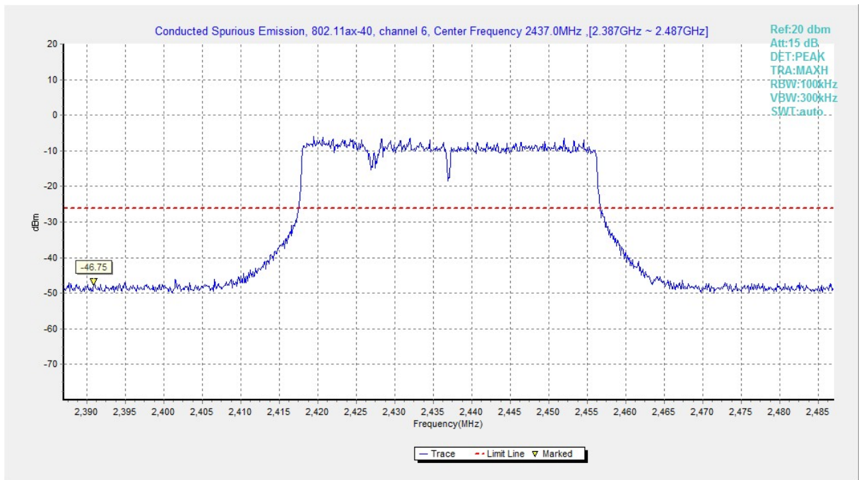
Fig.A.6.1.273 Transmitter Spurious Emission - Conducted (802.11ax-HE40, Ch6, Center Frequency)
