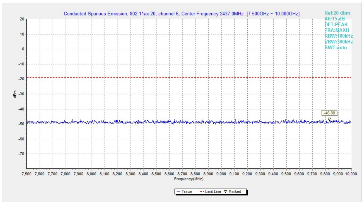
Fig.A.6.1.253 Transmitter Spurious Emission - Conducted (802.11ax-HE20, Ch6, 7.5 GHz-10 GHz)
