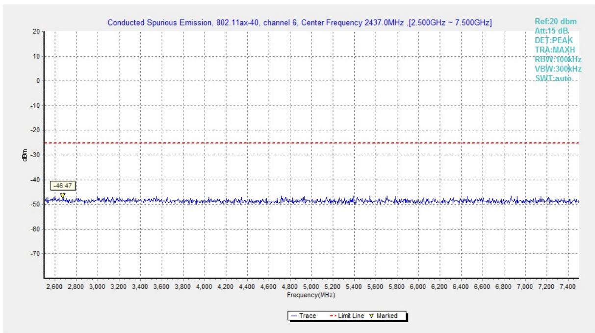
Fig.A.6.1.204 Transmitter Spurious Emission - Conducted (802.11ax-HE40, Ch6, 2.5 GHz-7.5 GHz)
