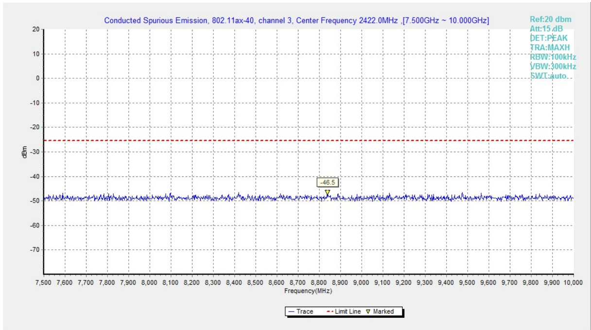
Fig.A.6.1.197 Transmitter Spurious Emission - Conducted (802.11ax-HE40, Ch3, 7.5 GHz-10 GHz)
