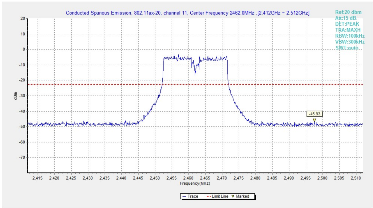
Fig.A.6.1.185 Transmitter Spurious Emission - Conducted (802.11ax-HE20, Ch11, Center Frequency)
