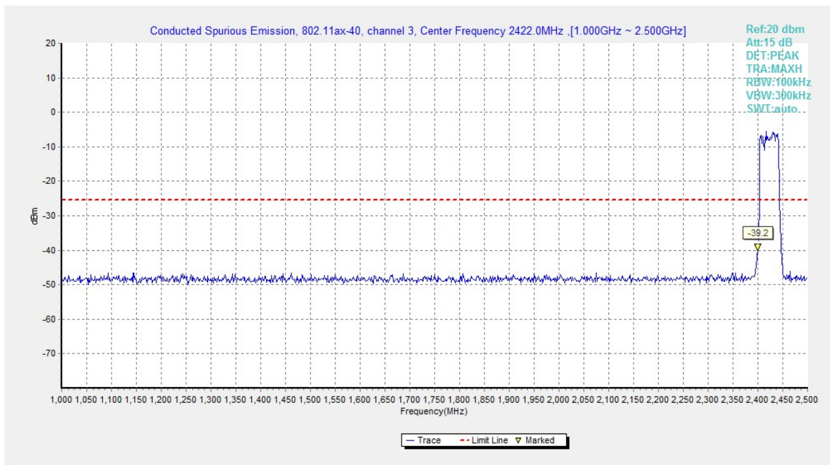
Fig.A.6.1.195 Transmitter Spurious Emission - Conducted (802.11ax-HE40, Ch3, 1 GHz-2.5 GHz)
