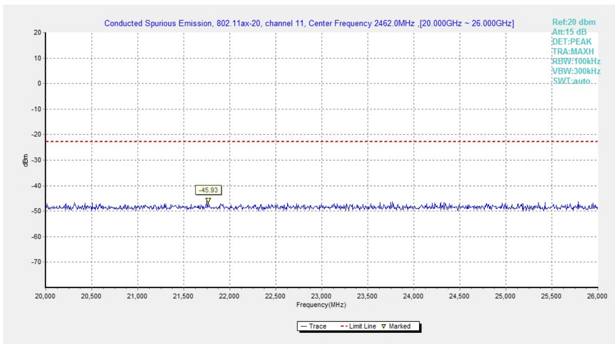
Fig.A.6.1.192 Transmitter Spurious Emission - Conducted (802.11ax-HE20, Ch11, 20 GHz-26 GHz)
