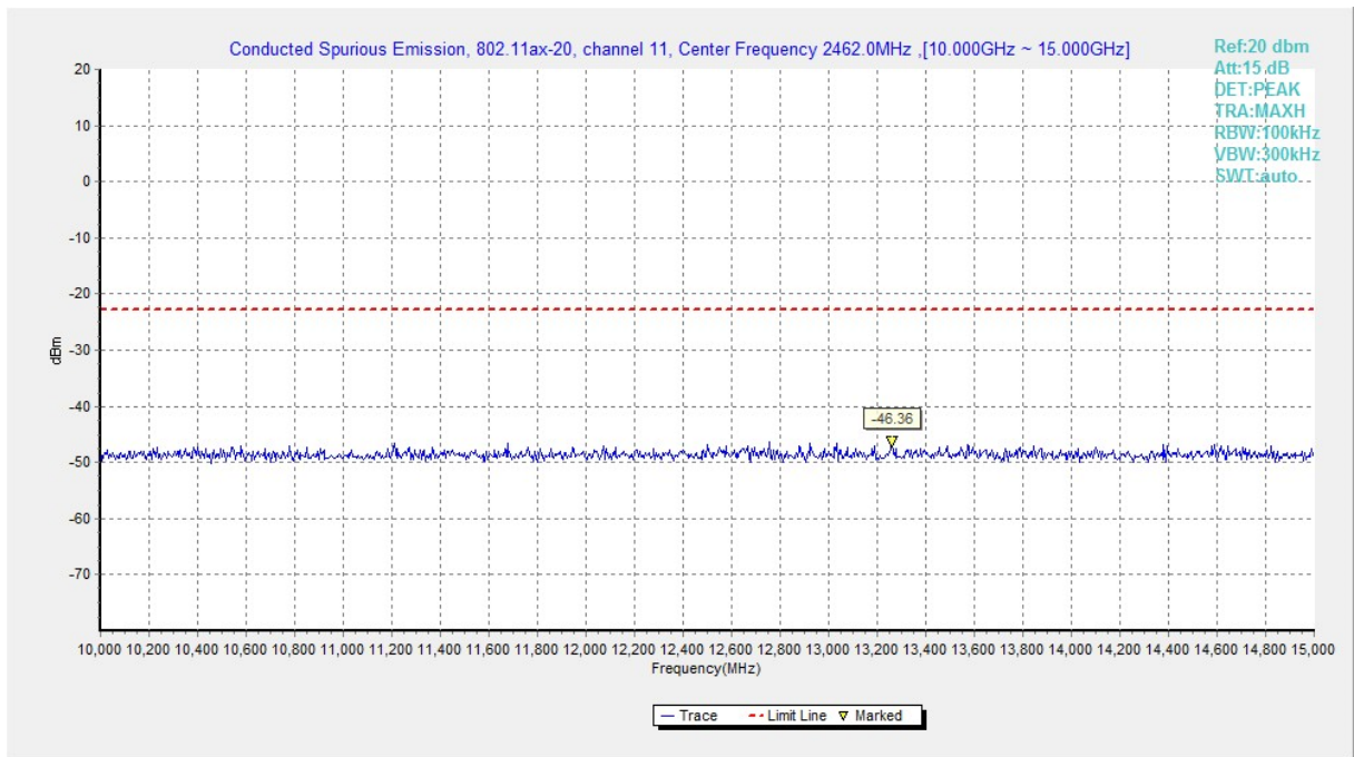
Fig.A.6.1.190 Transmitter Spurious Emission - Conducted (802.11ax-HE20, Ch11, 10 GHz-15 GHz)
