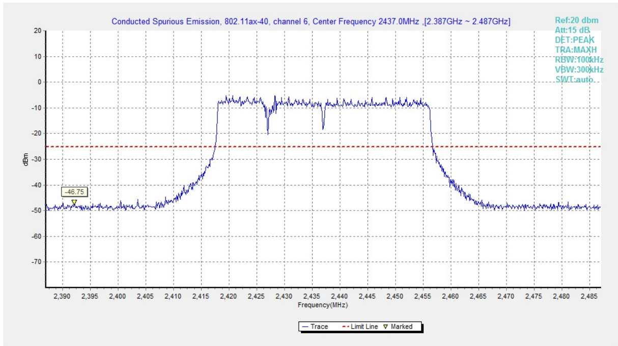
Fig.A.6.1.201 Transmitter Spurious Emission - Conducted (802.11ax-HE40, Ch6, Center Frequency)
