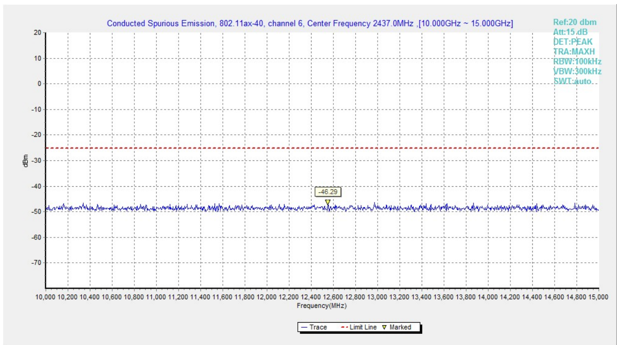
Fig.A.6.1.206 Transmitter Spurious Emission - Conducted (802.11ax-HE40, Ch6, 10 GHz-15 GHz)
