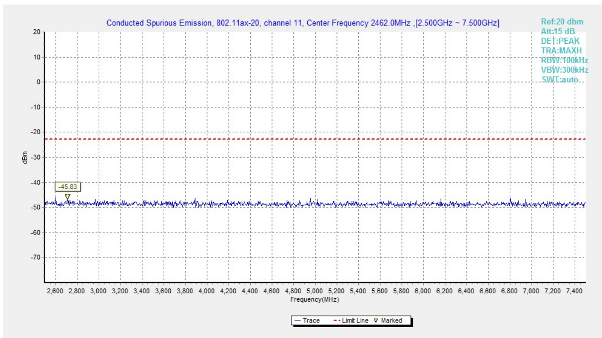
Fig.A.6.1.188 Transmitter Spurious Emission - Conducted (802.11ax-HE20, Ch11, 2.5 GHz-7.5 GHz)
