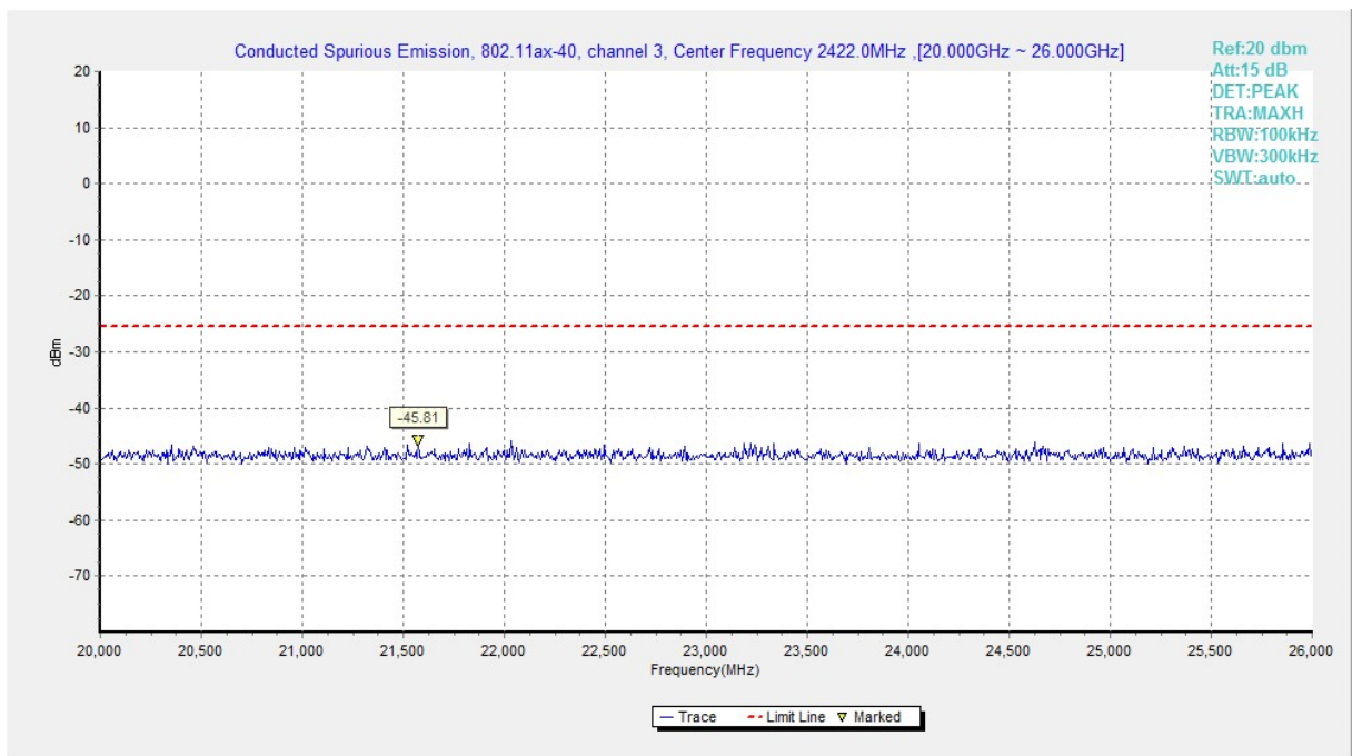
Fig.A.6.1.200 Transmitter Spurious Emission - Conducted (802.11ax-HE40, Ch3, 20 GHz-26 GHz)
