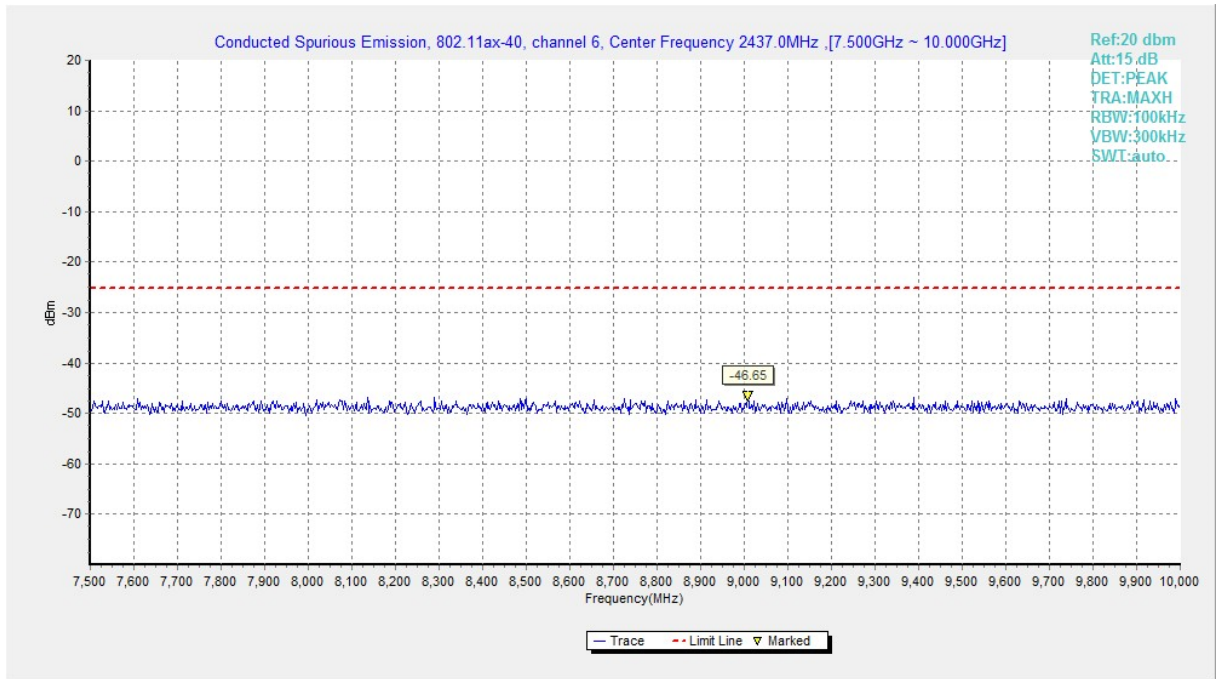
Fig.A.6.1.205 Transmitter Spurious Emission - Conducted (802.11ax-HE40, Ch6, 7.5 GHz-10 GHz)
