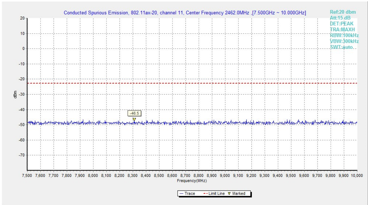
Fig.A.6.1.189 Transmitter Spurious Emission - Conducted (802.11ax-HE20, Ch11, 7.5 GHz-10 GHz)
