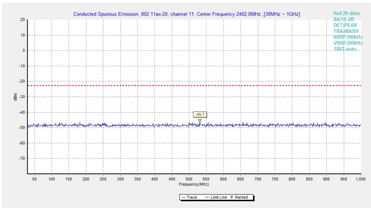
Fig.A.6.1.186 Transmitter Spurious Emission - Conducted (802.11ax-HE20, Ch11, 30 MHz-1 GHz)
