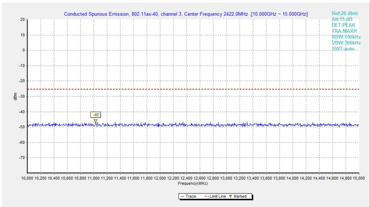
Fig.A.6.1.198 Transmitter Spurious Emission - Conducted (802.11ax-HE40, Ch3, 10 GHz-15 GHz)
