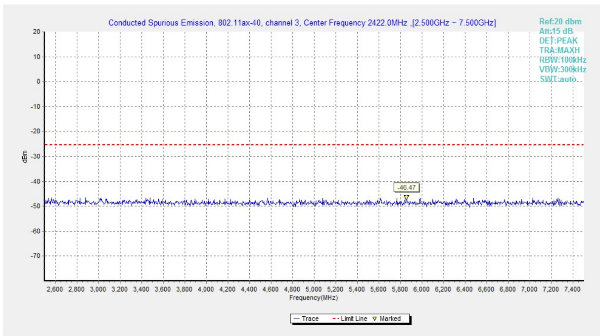
Fig.A.6.1.196 Transmitter Spurious Emission - Conducted (802.11ax-HE40, Ch3, 2.5 GHz-7.5 GHz)
