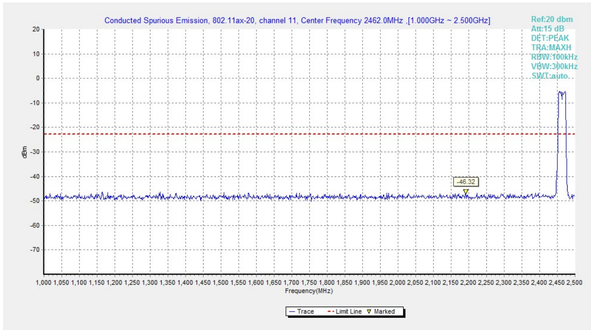
Fig.A.6.1.187 Transmitter Spurious Emission - Conducted (802.11ax-HE20, Ch11, 1 GHz-2.5 GHz)
