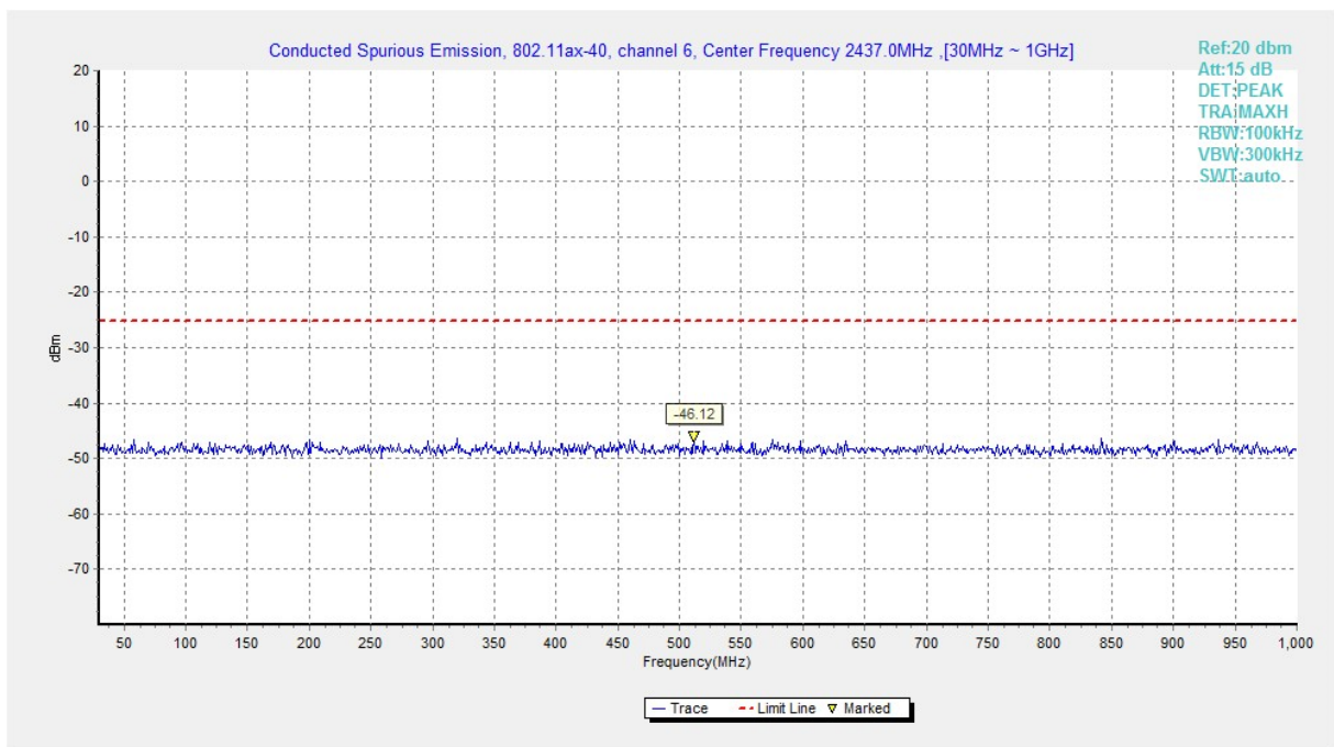
Fig.A.6.1.202 Transmitter Spurious Emission - Conducted (802.11ax-HE40, Ch6, 30 MHz-1 GHz)
