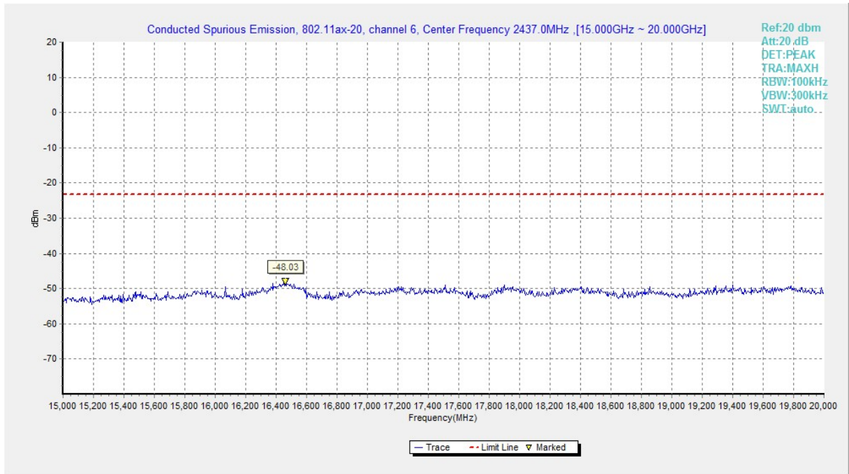
Fig.A.6.1.183 Transmitter Spurious Emission - Conducted (802.11ax-HE20, Ch6, 15 GHz-20 GHz)
