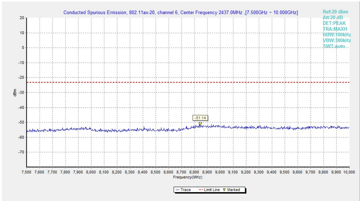
Fig.A.6.1.181 Transmitter Spurious Emission - Conducted (802.11ax-HE20, Ch6, 7.5 GHz-10 GHz)
