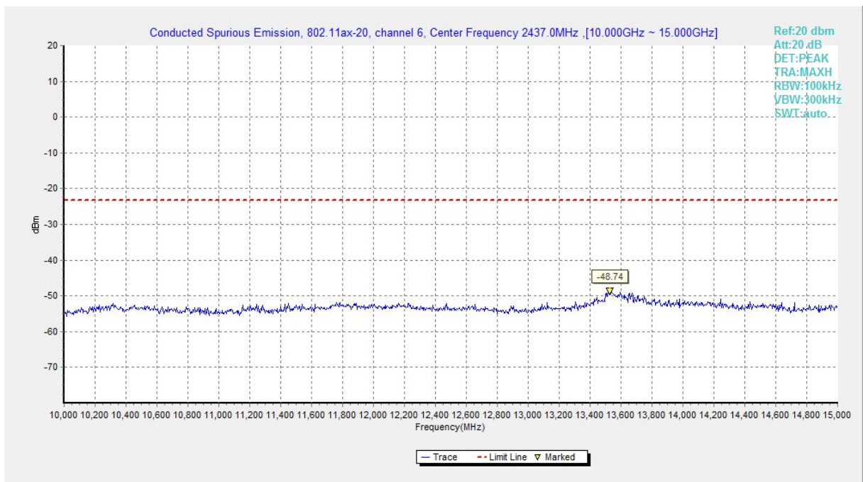
Fig.A.6.1.182 Transmitter Spurious Emission - Conducted (802.11ax-HE20, Ch6, 10 GHz-15 GHz)
