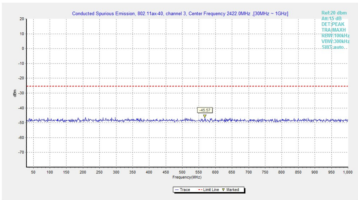
Fig.A.6.1.194 Transmitter Spurious Emission - Conducted (802.11ax-HE40, Ch3, 30 MHz-1 GHz)
