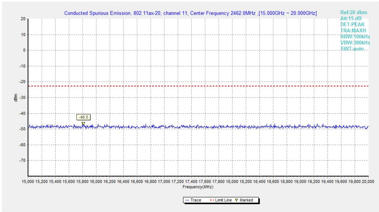
Fig.A.6.1.191 Transmitter Spurious Emission - Conducted (802.11ax-HE20, Ch11, 15 GHz-20 GHz)
