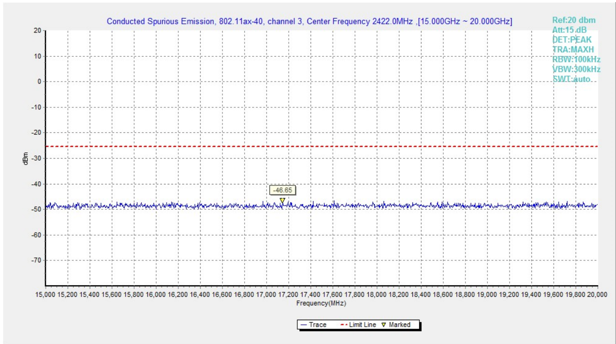
Fig.A.6.1.199 Transmitter Spurious Emission - Conducted (802.11ax-HE40, Ch3, 15 GHz-20 GHz)
