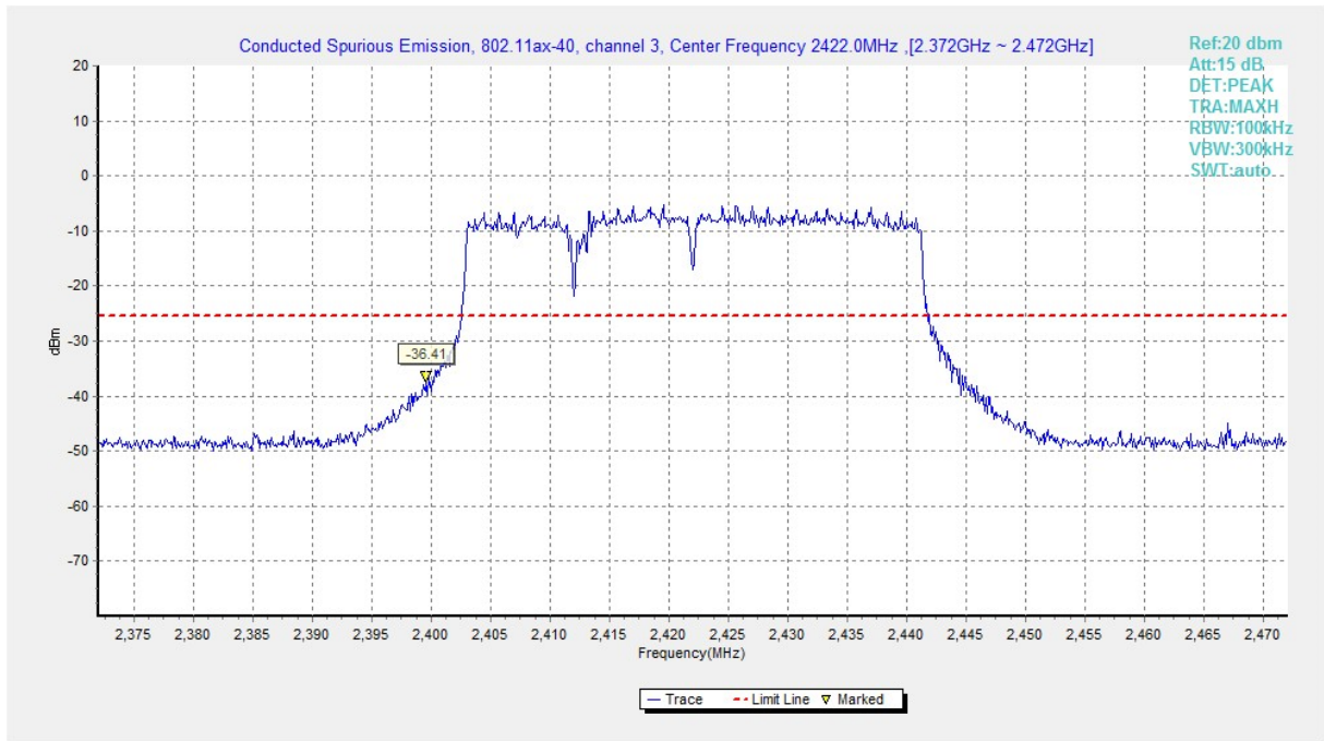
Fig.A.6.1.193 Transmitter Spurious Emission - Conducted (802.11ax-HE40, Ch3, Center Frequency)
