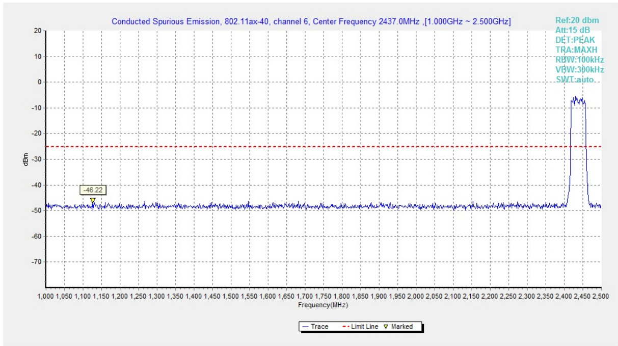
Fig.A.6.1.203 Transmitter Spurious Emission - Conducted (802.11ax-HE40, Ch6, 1 GHz-2.5 GHz)
