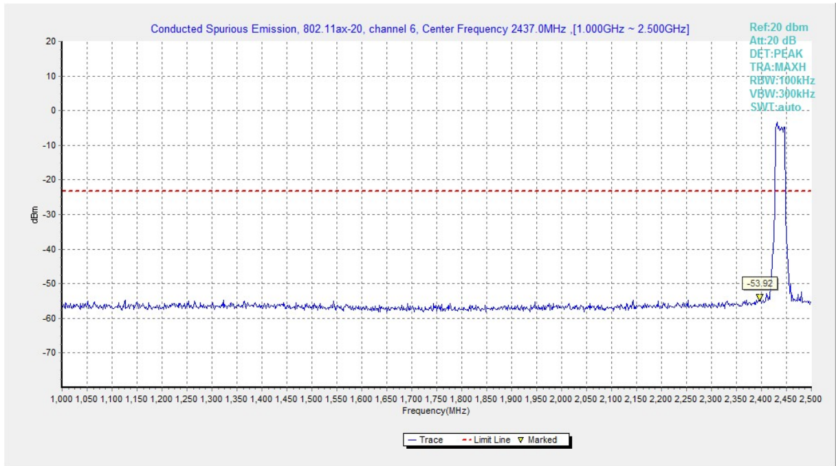
Fig.A.6.1.179 Transmitter Spurious Emission - Conducted (802.11ax-HE20, Ch6, 1 GHz-2.5 GHz)
