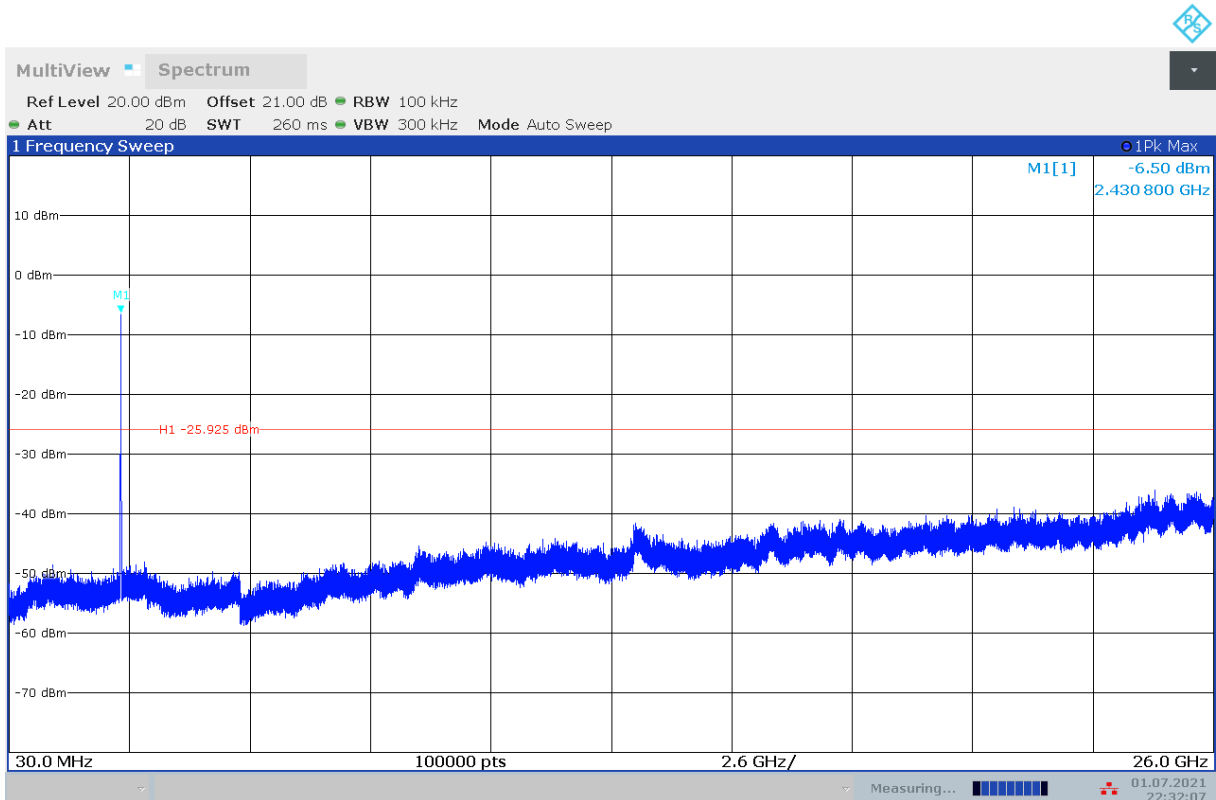
Fig.A.6.1.153 Transmitter Spurious Emission - Conducted (802.11g, Ch6, Center Frequency)
