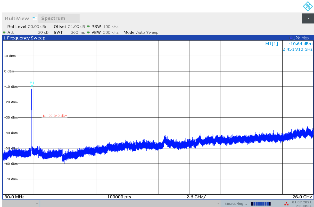
Fig.A.6.1.166 Transmitter Spurious Emission - Conducted (802.11n-HT40, Ch6, 30 MHz-26 GHz)
