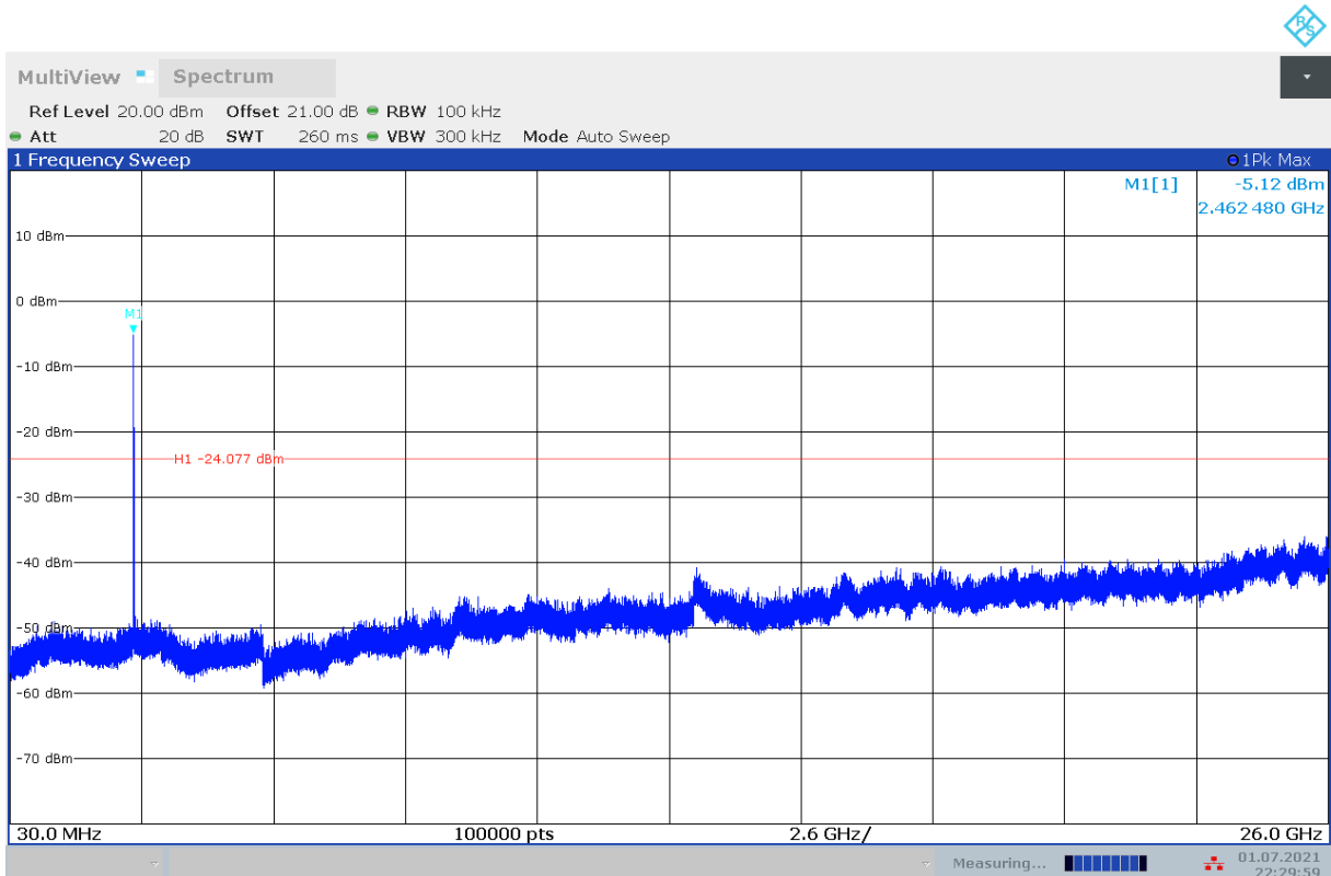
Fig.A.6.1.149 Transmitter Spurious Emission - Conducted (802.11b, Ch11, Center Frequency)
