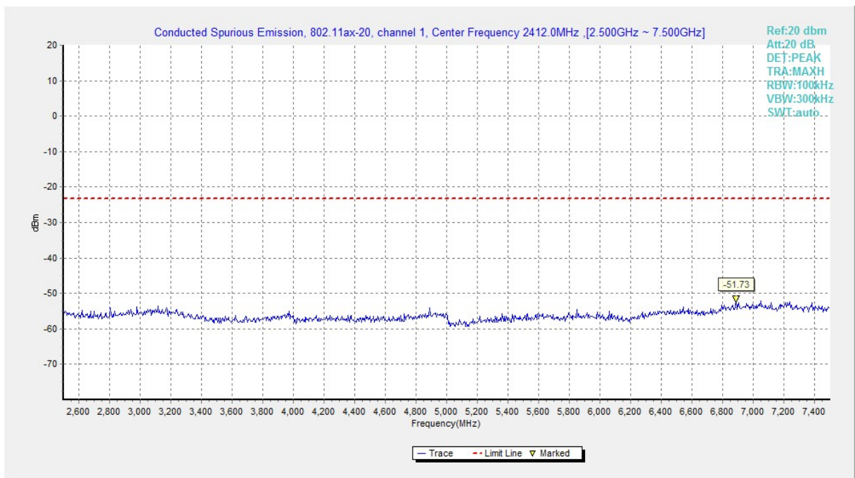
Fig.A.6.1.172 Transmitter Spurious Emission - Conducted (802.11ax-HE20, Ch1, 2.5 GHz-7.5 GHz)
