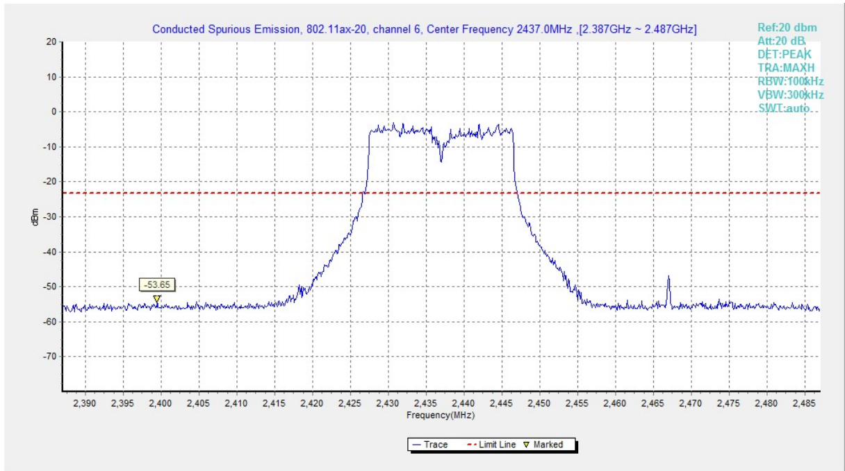
Fig.A.6.1.177 Transmitter Spurious Emission - Conducted (802.11ax-HE20, Ch6, Center Frequency)
