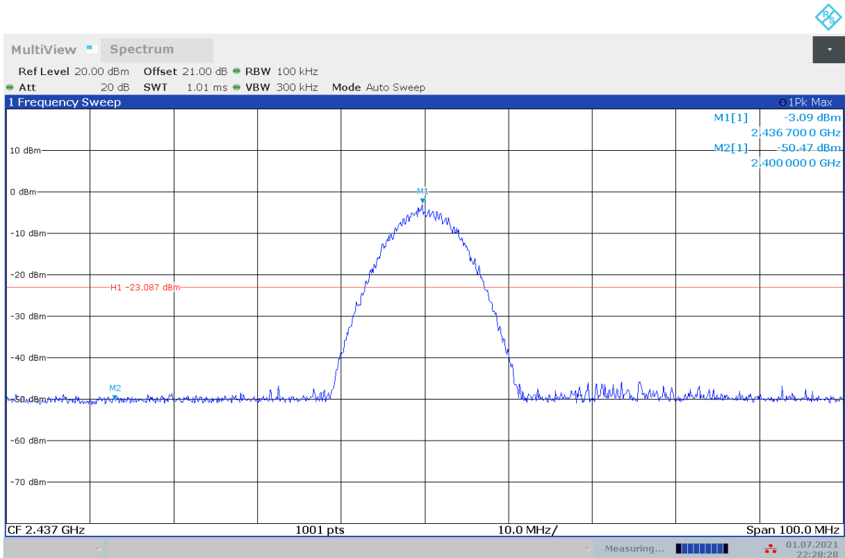
Fig.A.6.1.147 Transmitter Spurious Emission - Conducted (802.11b, Ch6, Center Frequency)
