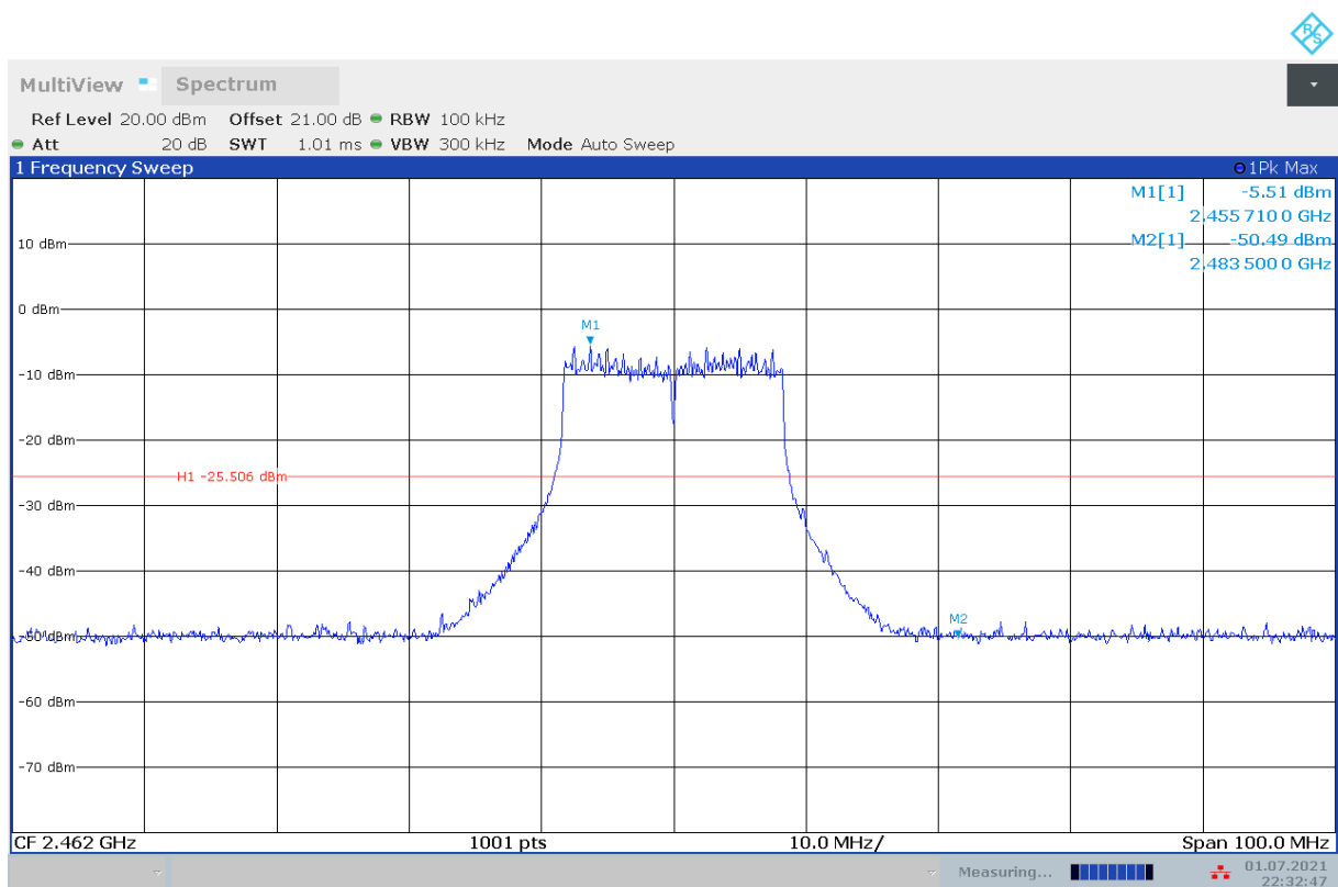
Fig.A.6.1.155 Transmitter Spurious Emission - Conducted (802.11g, Ch11, Center Frequency)
