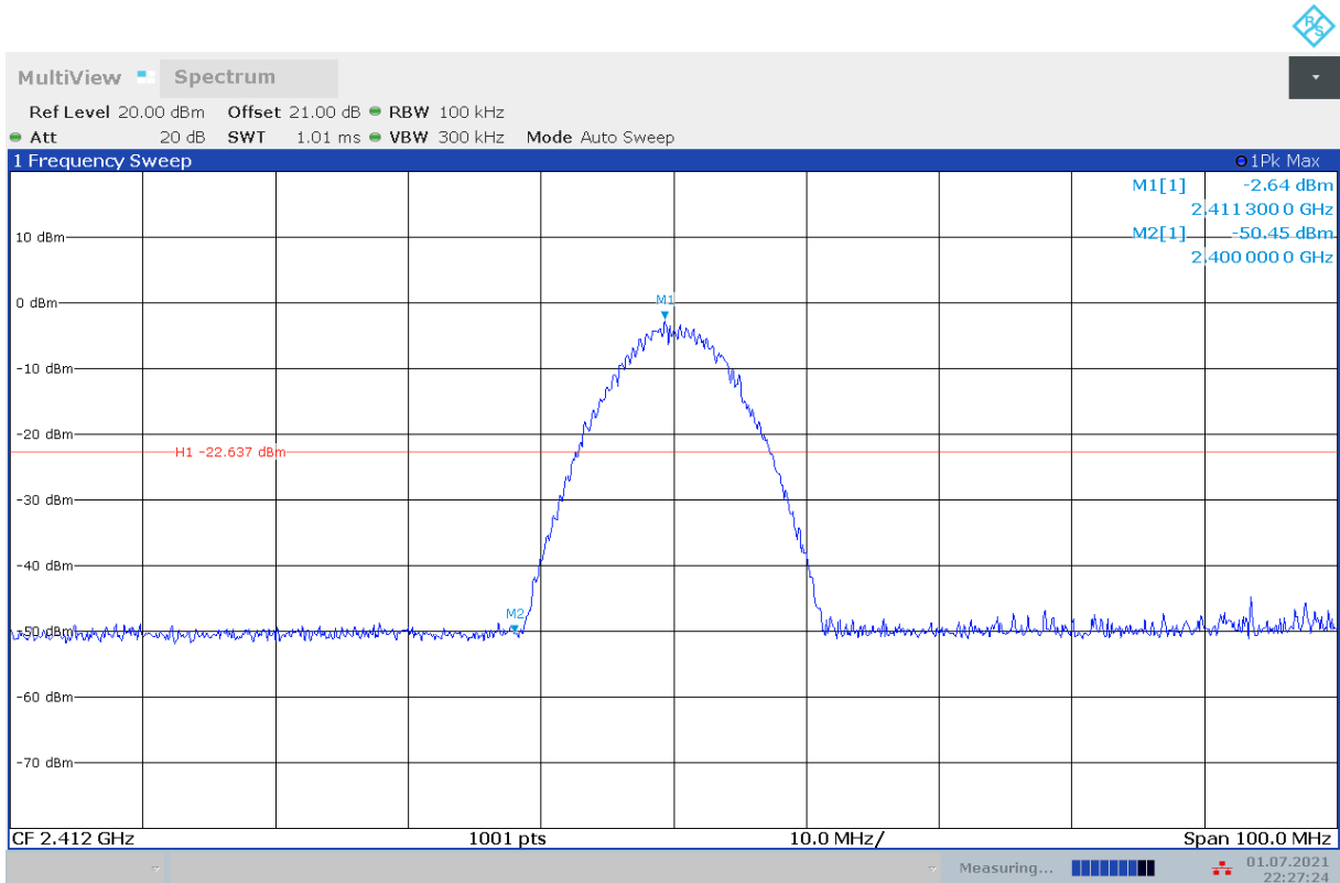
Fig.A.6.1.145 Transmitter Spurious Emission - Conducted (802.11b, Ch1, Center Frequency)
