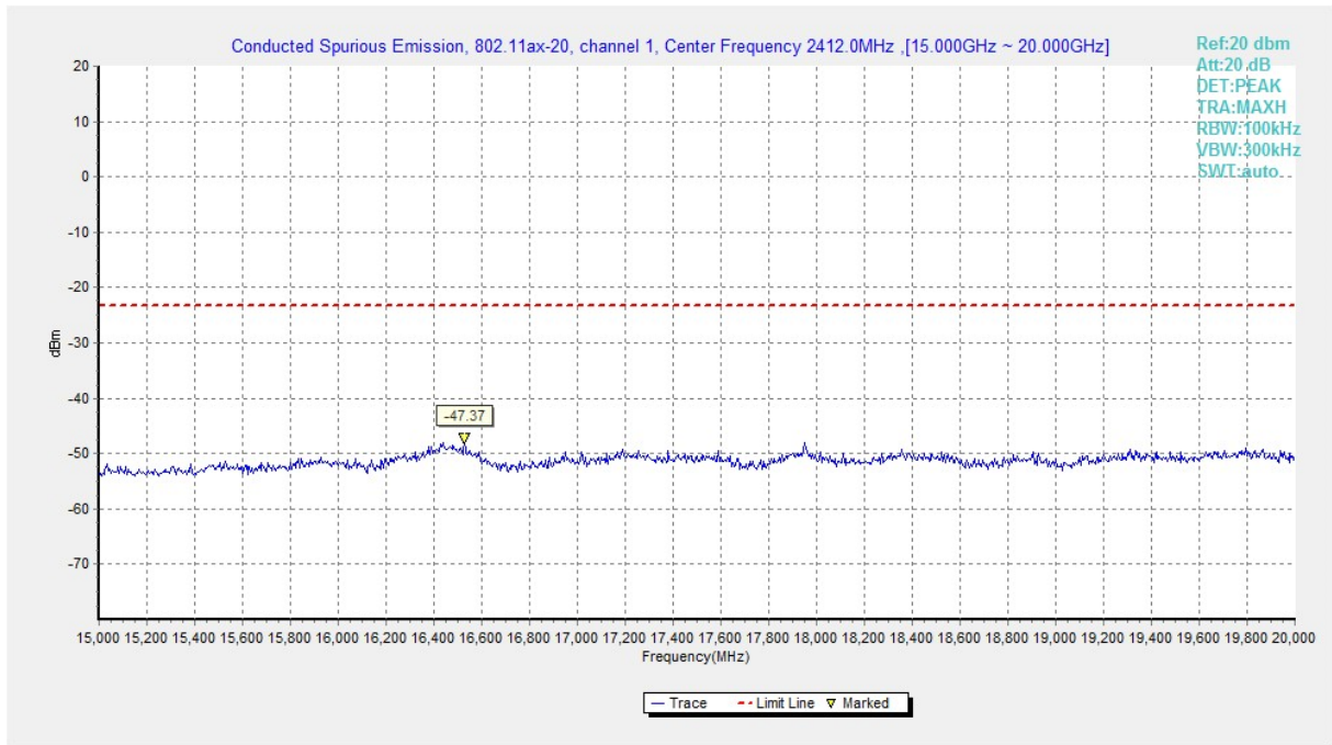
Fig.A.6.1.175 Transmitter Spurious Emission - Conducted (802.11ax-HE20, Ch1, 15 GHz-20 GHz)
