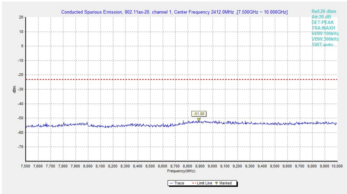
Fig.A.6.1.173 Transmitter Spurious Emission - Conducted (802.11ax-HE20, Ch1, 7.5 GHz-10 GHz)
