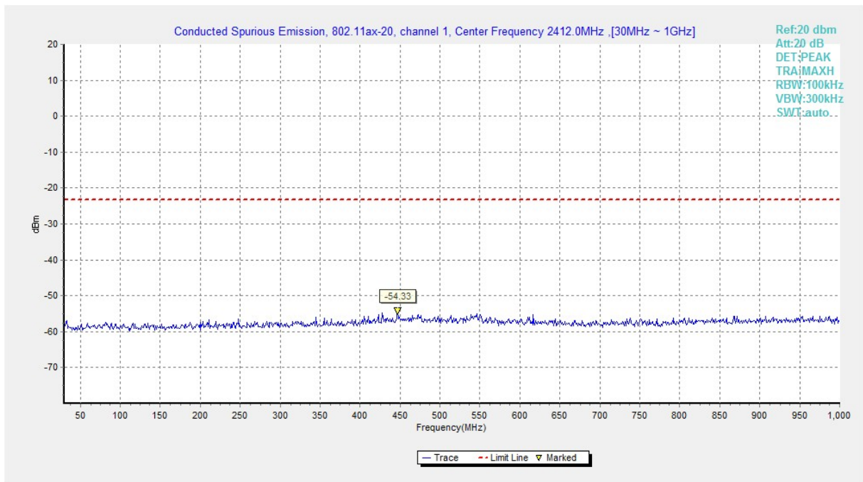
Fig.A.6.1.170 Transmitter Spurious Emission - Conducted (802.11ax-HE20, Ch1, 30 MHz-1 GHz)
