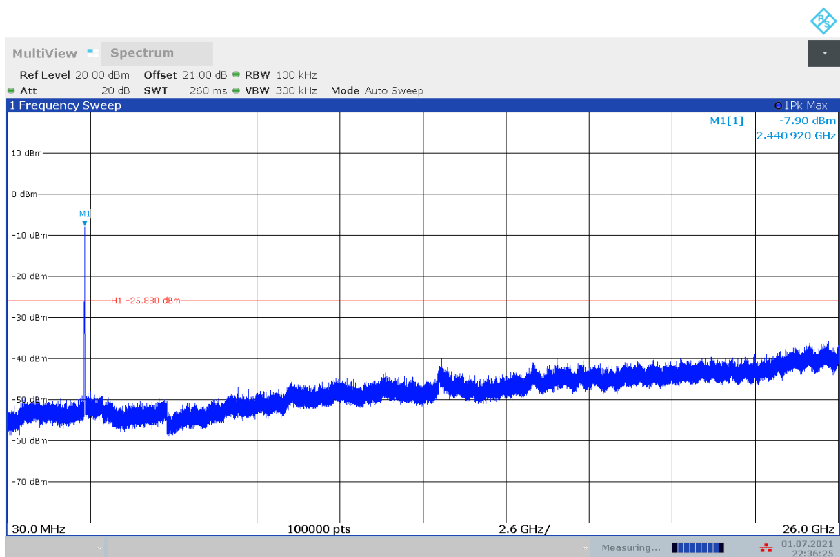
Fig.A.6.1.160 Transmitter Spurious Emission - Conducted (802.11n-HT20, Ch6, 30 MHz-26 GHz)
