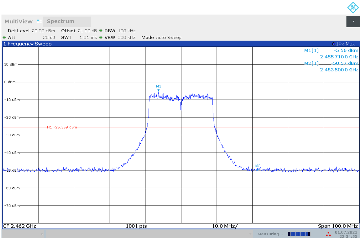
Fig.A.6.1.161 Transmitter Spurious Emission - Conducted (802.11n-HT20, Ch11, Center Frequency)
