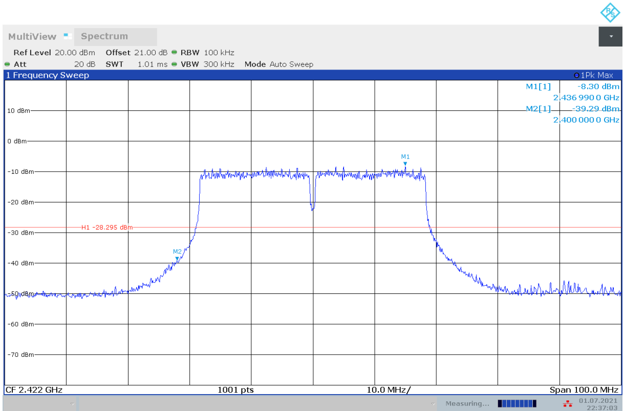
Fig.A.6.1.163 Transmitter Spurious Emission - Conducted (802.11n-HT40, Ch3, Center Frequency)
