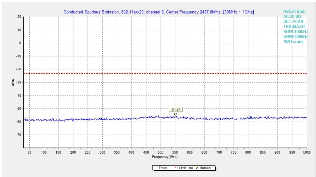
Fig.A.6.1.178 Transmitter Spurious Emission - Conducted (802.11ax-HE20, Ch6, 30 MHz-1 GHz)
