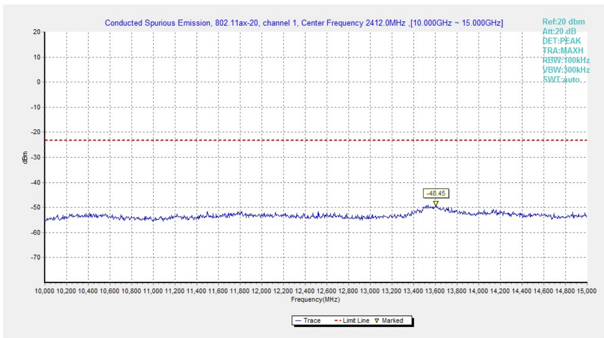
Fig.A.6.1.174 Transmitter Spurious Emission - Conducted (802.11ax-HE20, Ch1, 10 GHz-15 GHz)
