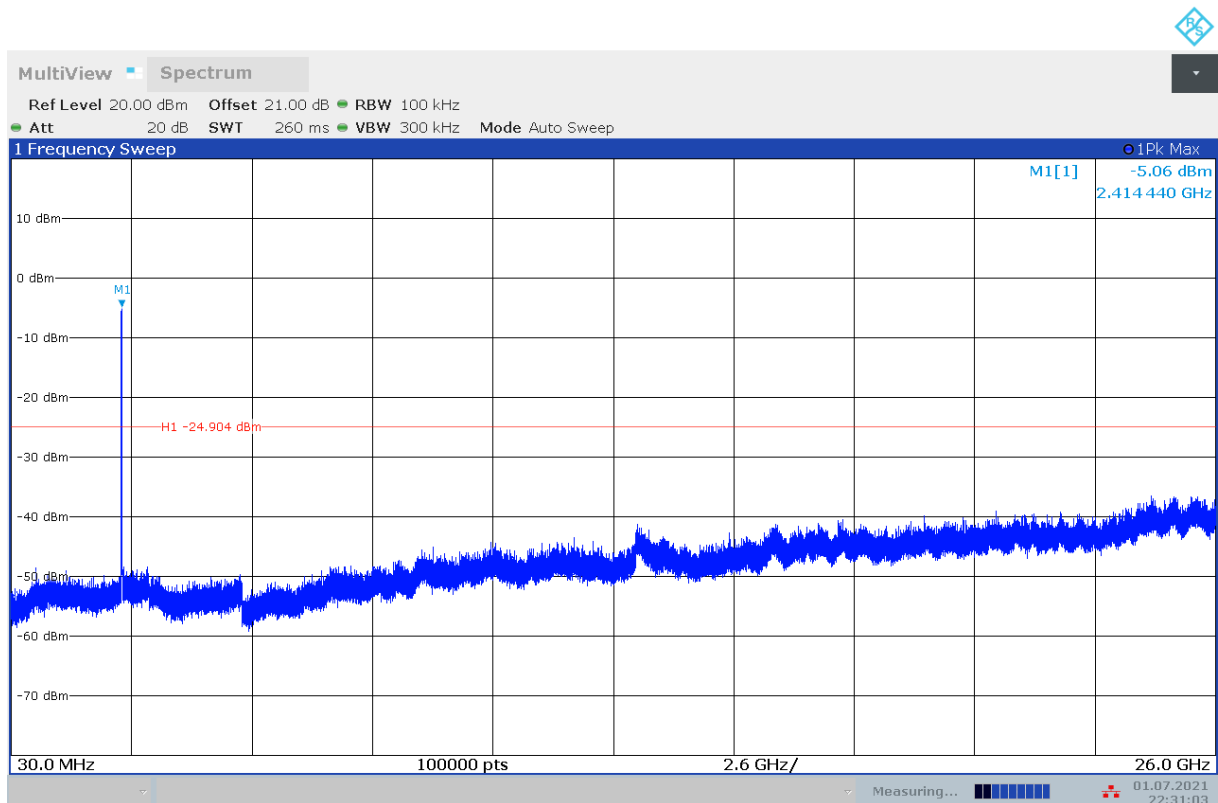
Fig.A.6.1.151 Transmitter Spurious Emission - Conducted (802.11g, Ch1, Center Frequency)
