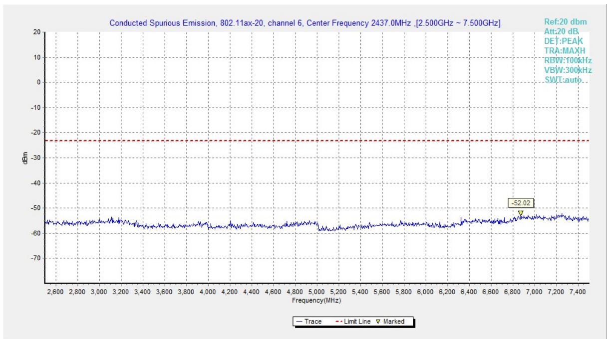
Fig.A.6.1.180 Transmitter Spurious Emission - Conducted (802.11ax-HE20, Ch6, 2.5 GHz-7.5 GHz)
