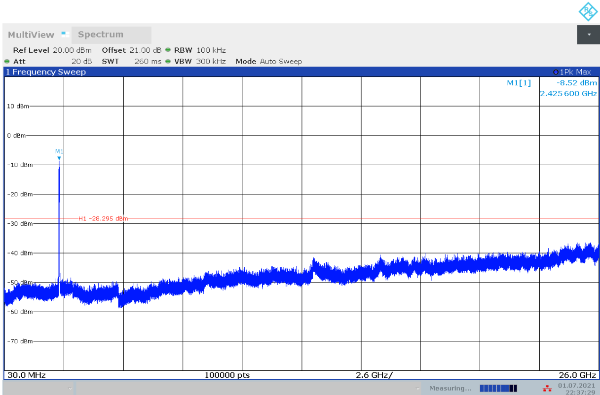
Fig.A.6.1.164 Transmitter Spurious Emission - Conducted (802.11n-HT40, Ch3, 30 MHz-26 GHz)
