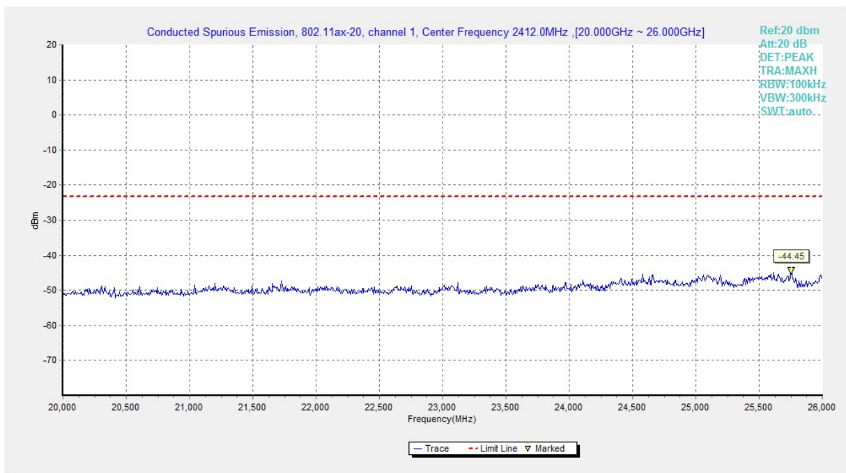
Fig.A.6.1.176 Transmitter Spurious Emission - Conducted (802.11ax-HE20, Ch1, 20 GHz-26 GHz)
