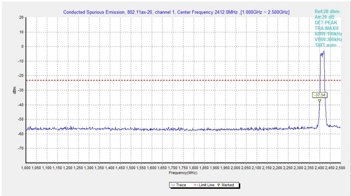
Fig.A.6.1.171 Transmitter Spurious Emission - Conducted (802.11ax-HE20, Ch1, 1 GHz-2.5 GHz)
