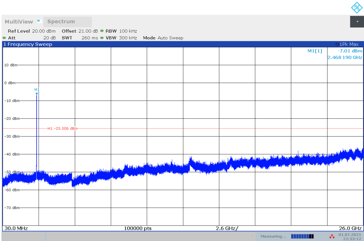
Fig.A.6.1.156 Transmitter Spurious Emission - Conducted (802.11g, Ch11, 30 MHz-26 GHz)
