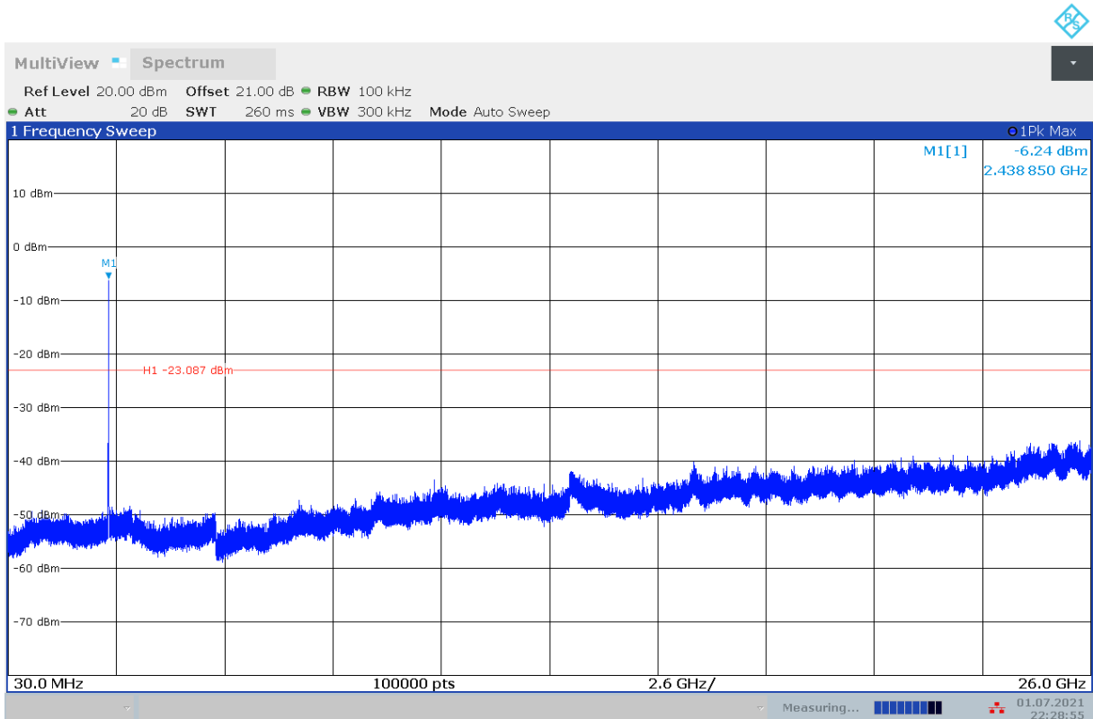
Fig.A.6.1.148 Transmitter Spurious Emission - Conducted (802.11b, Ch6, 30 MHz-26 GHz)
