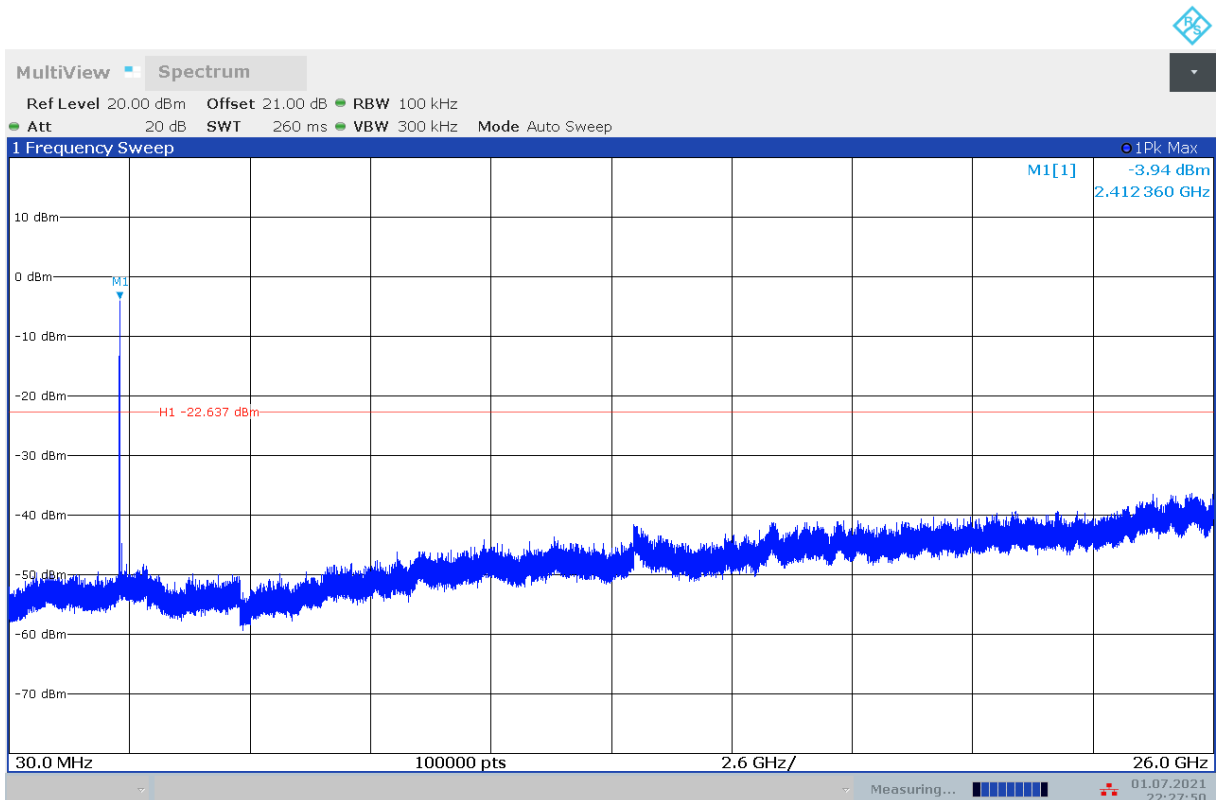
Fig.A.6.1.146 Transmitter Spurious Emission - Conducted (802.11b, Ch1, 30 MHz-26 GHz)
