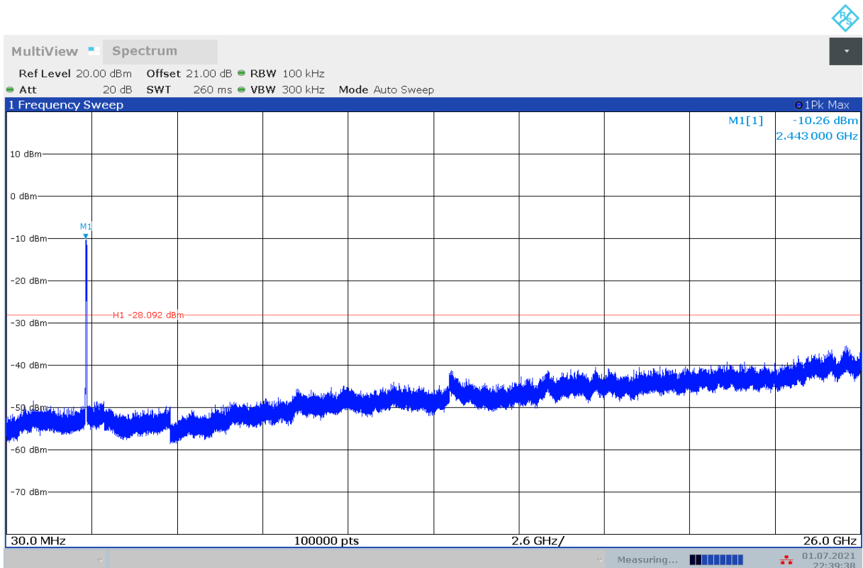
Fig.A.6.1.167 Transmitter Spurious Emission - Conducted (802.11n-HT40, Ch9, Center Frequency)
