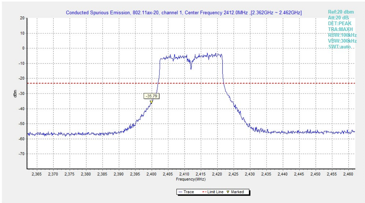
Fig.A.6.1.169 Transmitter Spurious Emission - Conducted (802.11ax-HE20, Ch1, Center Frequency)
