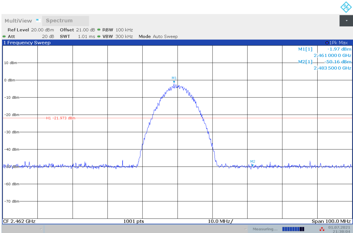
Fig.A.6.1.77 Transmitter Spurious Emission - Conducted (802.11b, Ch11, Center Frequency)
