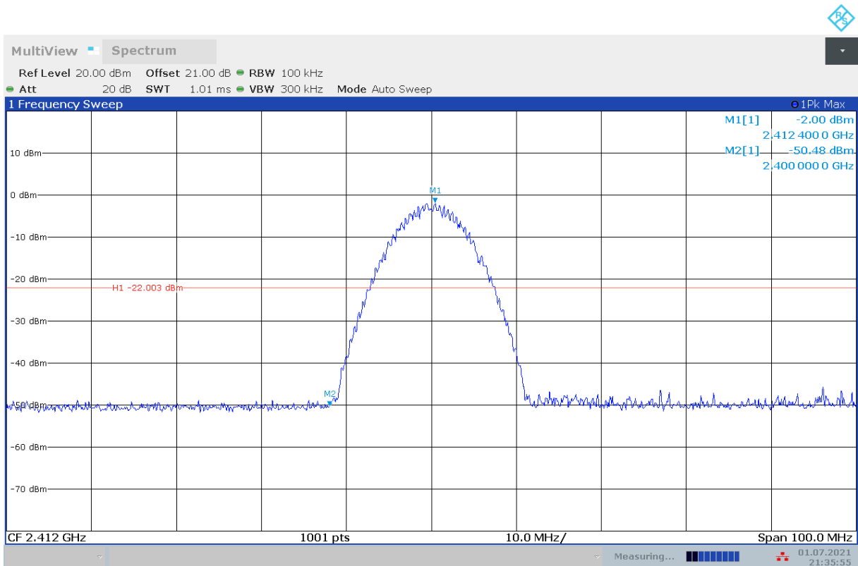
Fig.A.6.1.73 Transmitter Spurious Emission - Conducted (802.11b, Ch1, Center Frequency)
