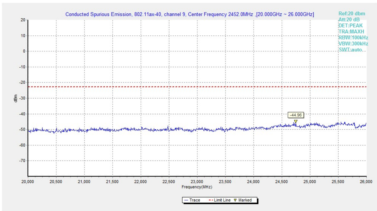
Fig.A.6.1.72 Transmitter Spurious Emission - Conducted (802.11ax-HE40, Ch9, 20 GHz-26 GHz)
