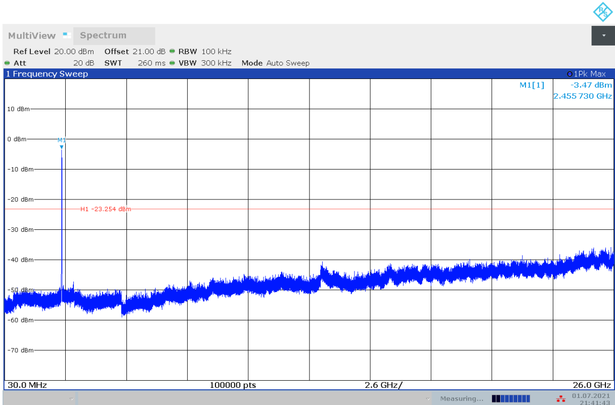
Fig.A.6.1.84 Transmitter Spurious Emission - Conducted (802.11g, Ch11, 30 MHz-26 GHz)
