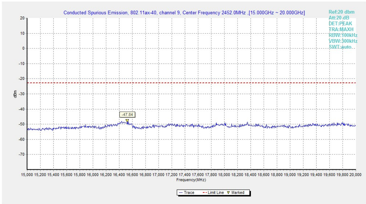
Fig.A.6.1.71 Transmitter Spurious Emission - Conducted (802.11ax-HE40, Ch9, 15 GHz-20 GHz)
