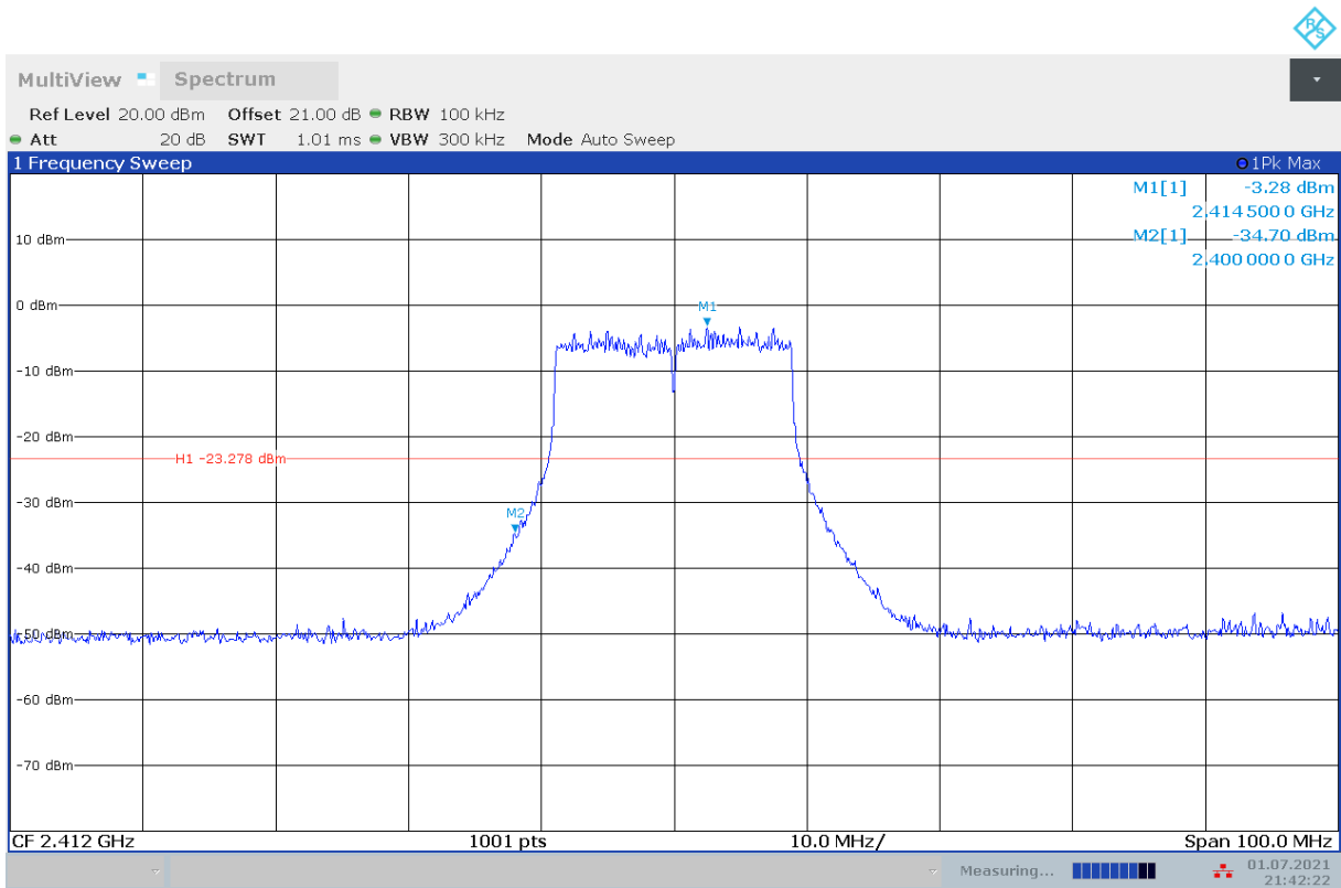
Fig.A.6.1.85 Transmitter Spurious Emission - Conducted (802.11n-HT20, Ch1, Center Frequency)
