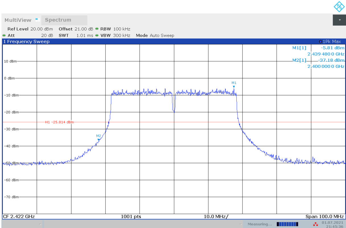
Fig.A.6.1.91 Transmitter Spurious Emission - Conducted (802.11n-HT40, Ch3, Center Frequency)
