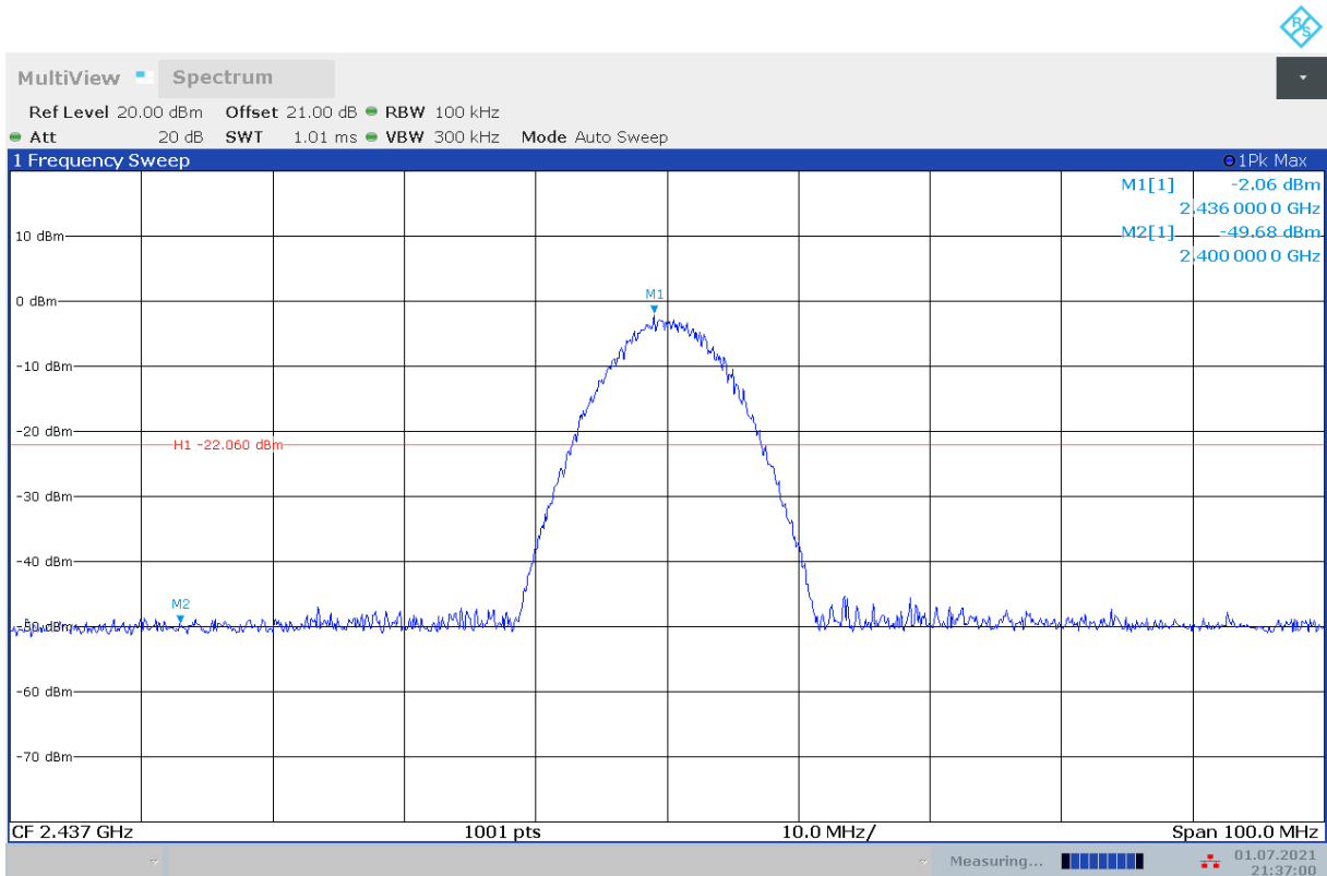
Fig.A.6.1.75 Transmitter Spurious Emission - Conducted (802.11b, Ch6, Center Frequency)
