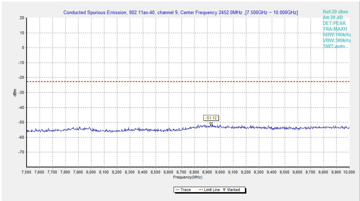
Fig.A.6.1.69 Transmitter Spurious Emission - Conducted (802.11ax-HE40, Ch9, 7.5 GHz-10 GHz)
