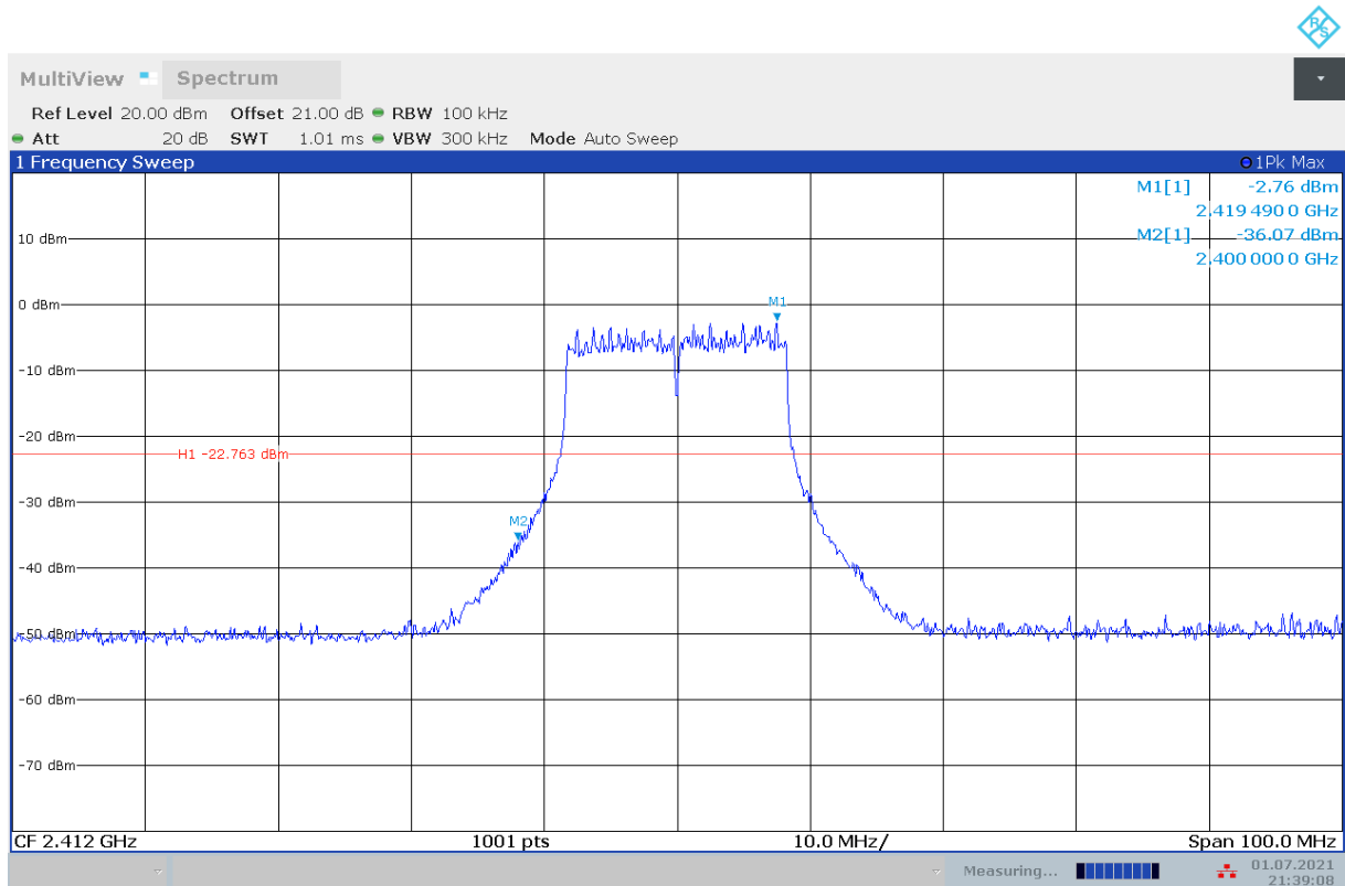
Fig.A.6.1.79 Transmitter Spurious Emission - Conducted (802.11g, Ch1, Center Frequency)
