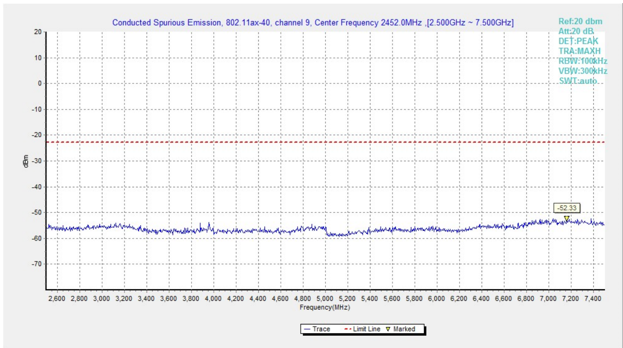
Fig.A.6.1.68 Transmitter Spurious Emission - Conducted (802.11ax-HE40, Ch9, 2.5 GHz-7.5 GHz)
