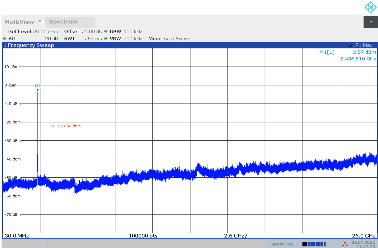
Fig.A.6.1.76 Transmitter Spurious Emission - Conducted (802.11b, Ch6, 30 MHz-26 GHz)
