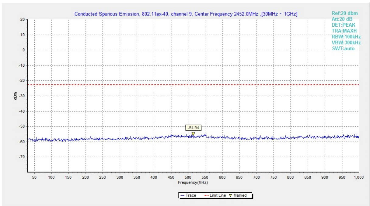
Fig.A.6.1.66 Transmitter Spurious Emission - Conducted (802.11ax-HE40, Ch9, 30 MHz-1 GHz)
