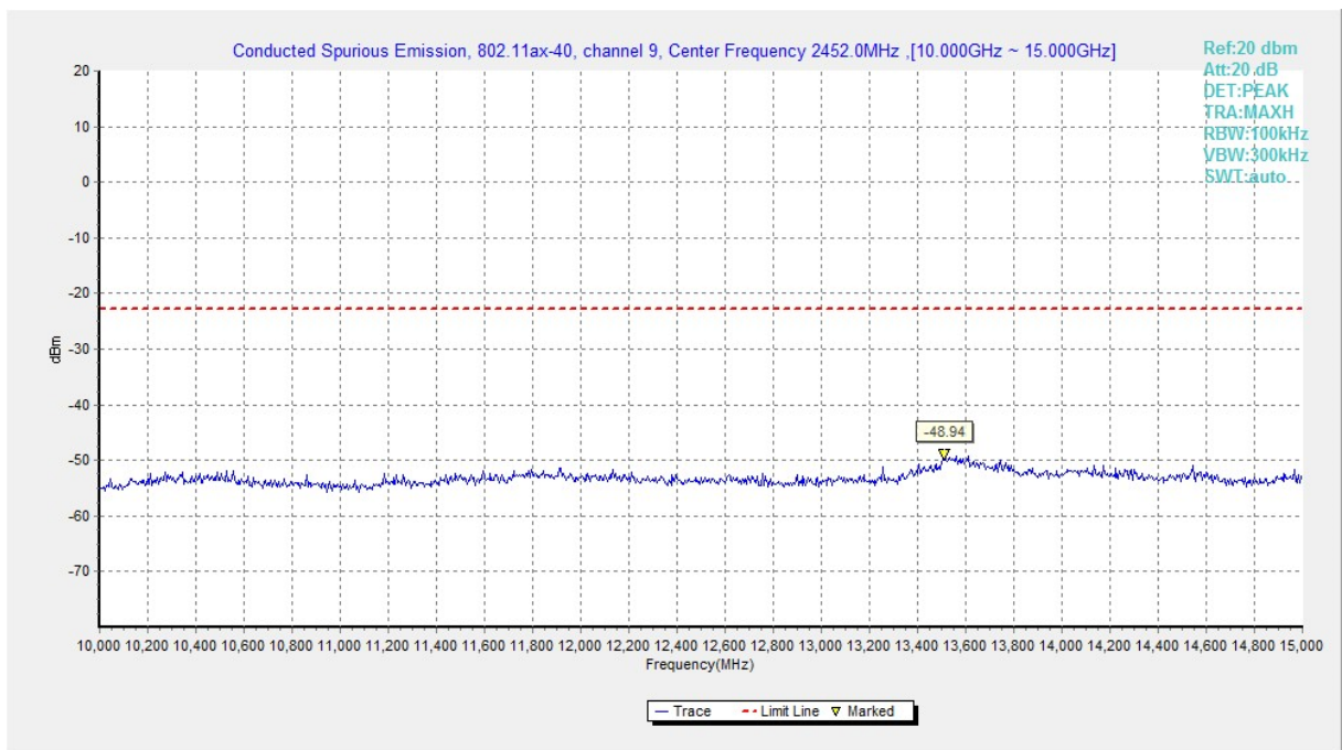
Fig.A.6.1.70 Transmitter Spurious Emission - Conducted (802.11ax-HE40, Ch9, 10 GHz-15 GHz)
