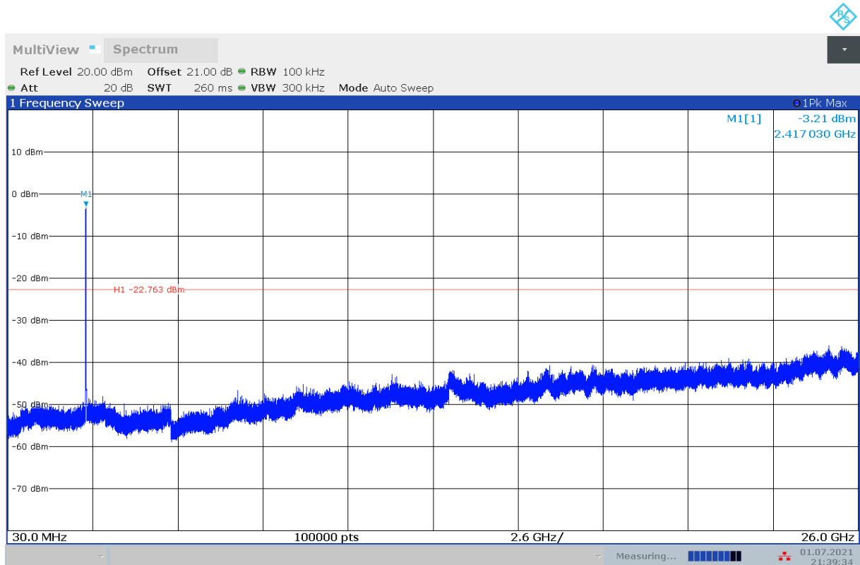
Fig.A.6.1.80 Transmitter Spurious Emission - Conducted (802.11g, Ch1, 30 MHz-26 GHz)
