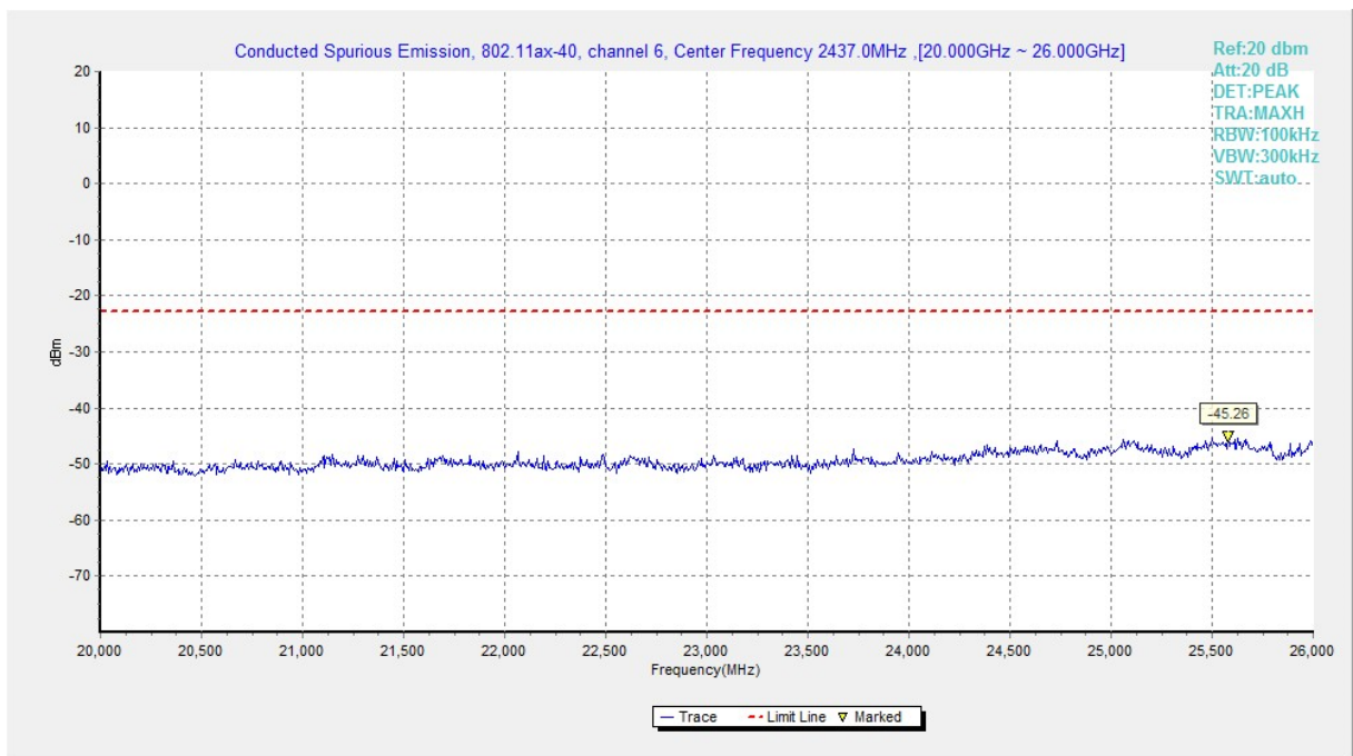
Fig.A.6.1.64 Transmitter Spurious Emission - Conducted (802.11ax-HE40, Ch6, 20 GHz-26 GHz)
