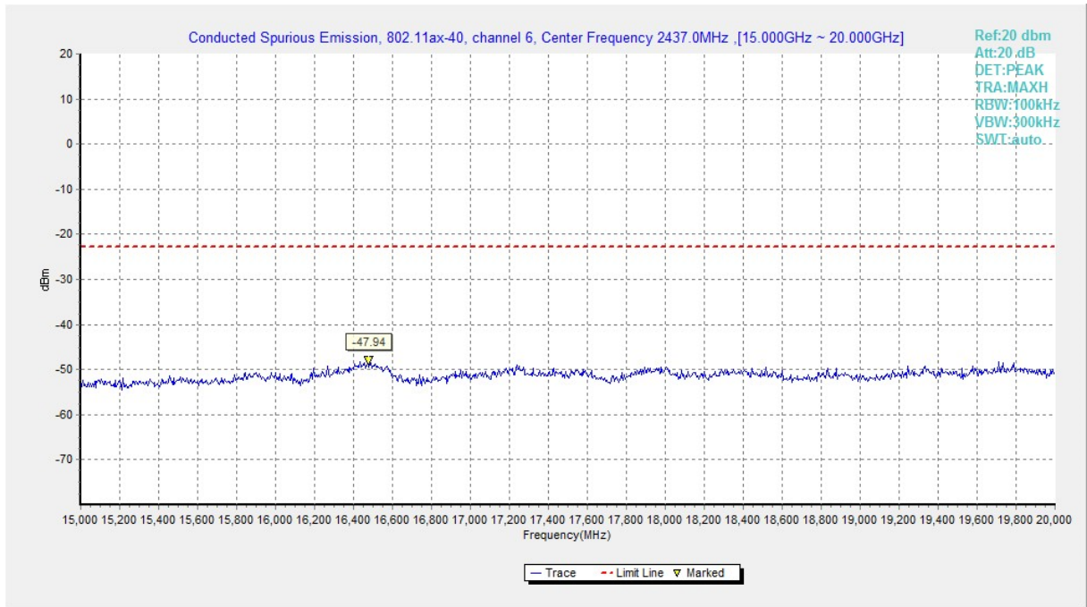
Fig.A.6.1.63 Transmitter Spurious Emission - Conducted (802.11ax-HE40, Ch6, 15 GHz-20 GHz)
