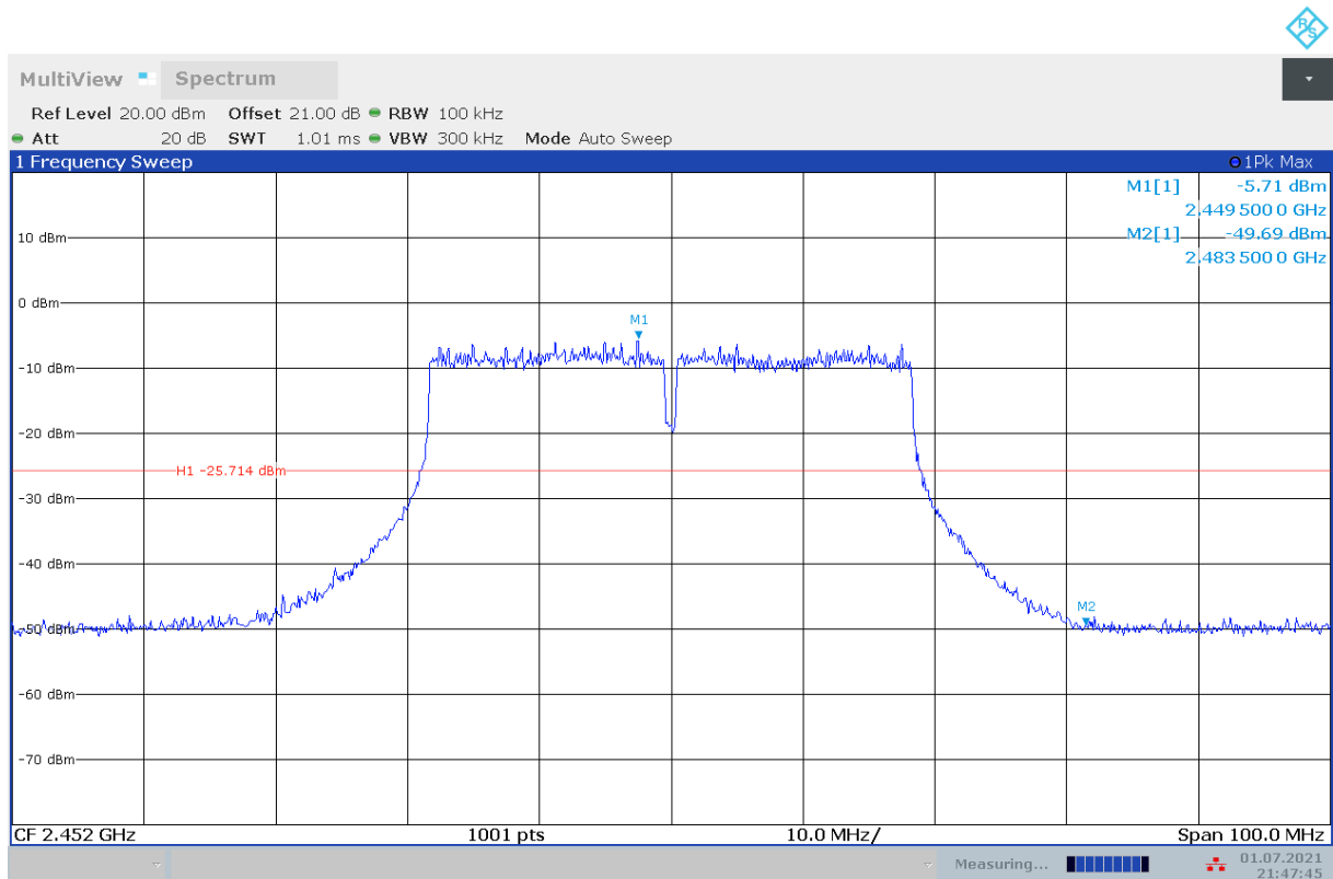
Fig.A.6.1.95 Transmitter Spurious Emission - Conducted (802.11n-HT40, Ch9, Center Frequency)
