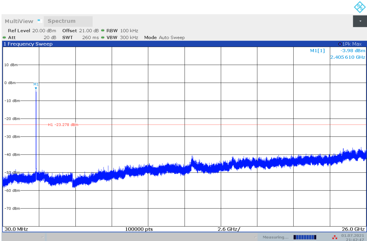
Fig.A.6.1.86 Transmitter Spurious Emission - Conducted (802.11n-HT20, Ch1, 30 MHz-26 GHz)
