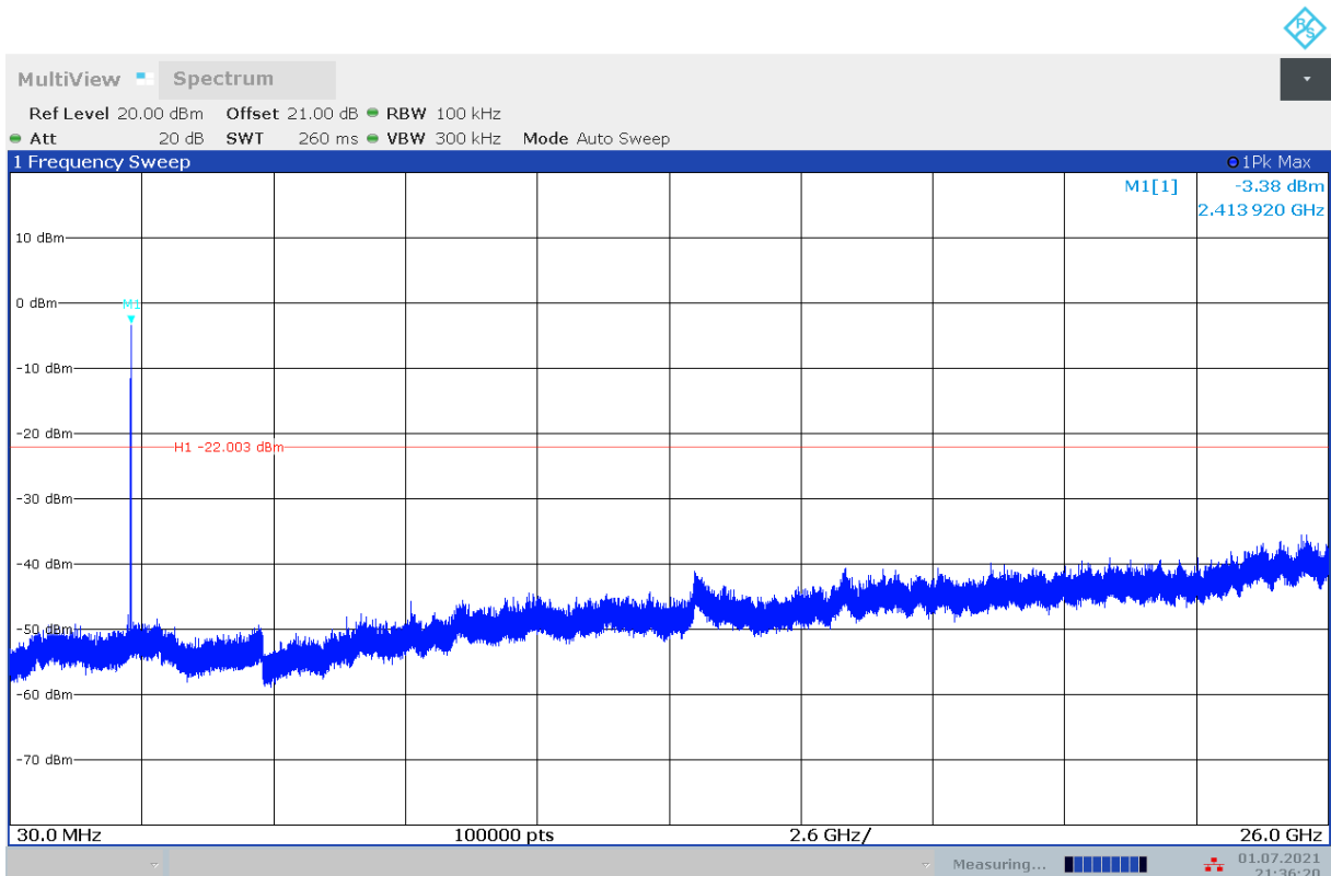
Fig.A.6.1.74 Transmitter Spurious Emission - Conducted (802.11b, Ch1, 30 MHz-26 GHz)
