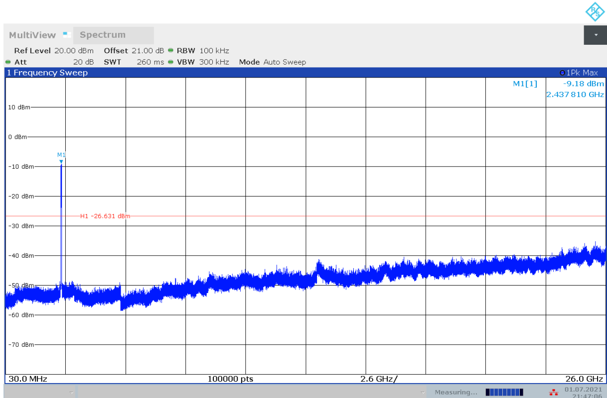
Fig.A.6.1.93 Transmitter Spurious Emission - Conducted (802.11n-HT40, Ch6, Center Frequency)
