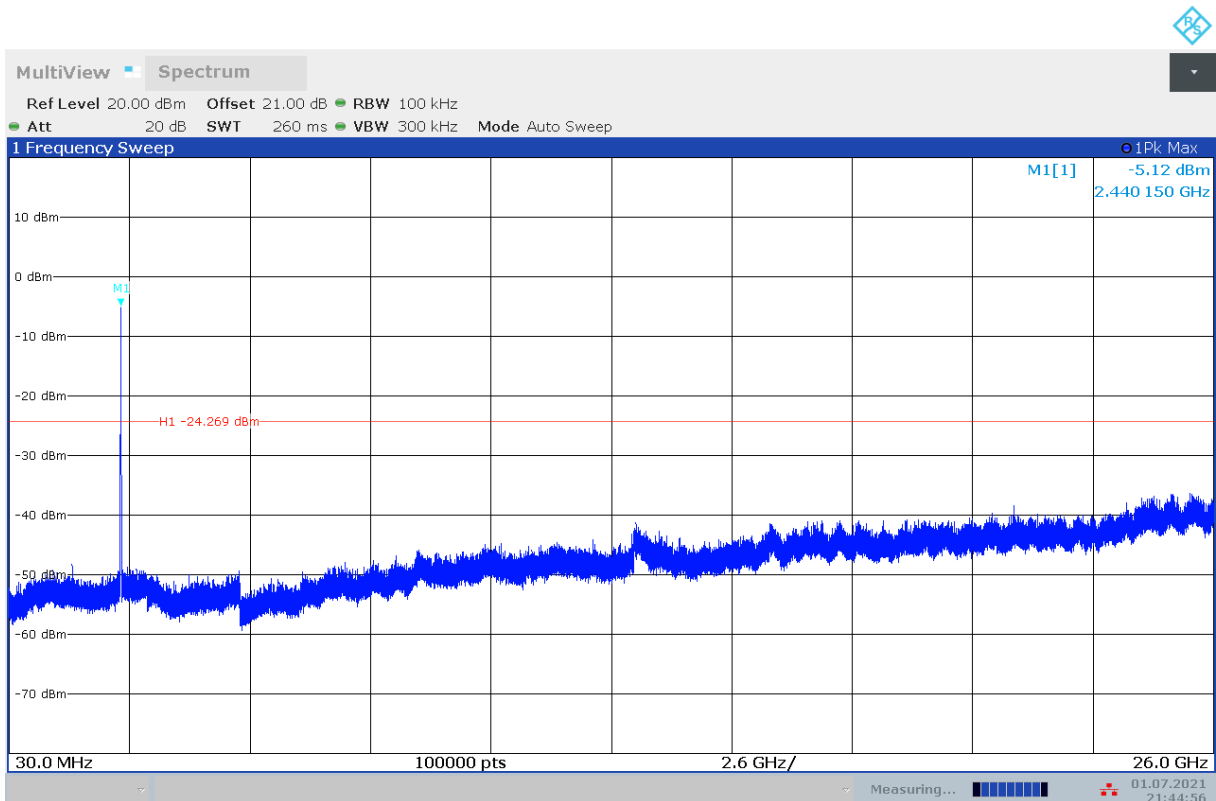
Fig.A.6.1.87 Transmitter Spurious Emission - Conducted (802.11n-HT20, Ch6, Center Frequency)
