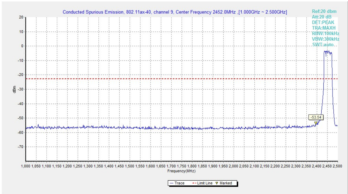
Fig.A.6.1.67 Transmitter Spurious Emission - Conducted (802.11ax-HE40, Ch9, 1 GHz-2.5 GHz)
