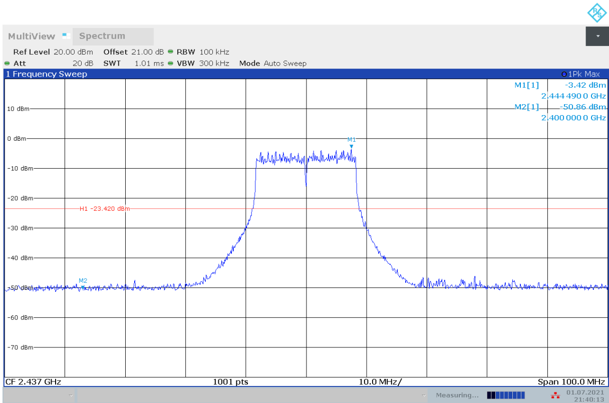
Fig.A.6.1.81 Transmitter Spurious Emission - Conducted (802.11g, Ch6, Center Frequency)
