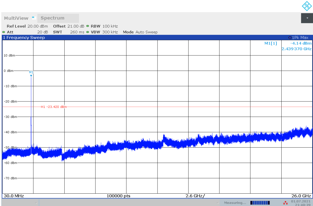
Fig.A.6.1.82 Transmitter Spurious Emission - Conducted (802.11g, Ch6, 30 MHz-26 GHz)
