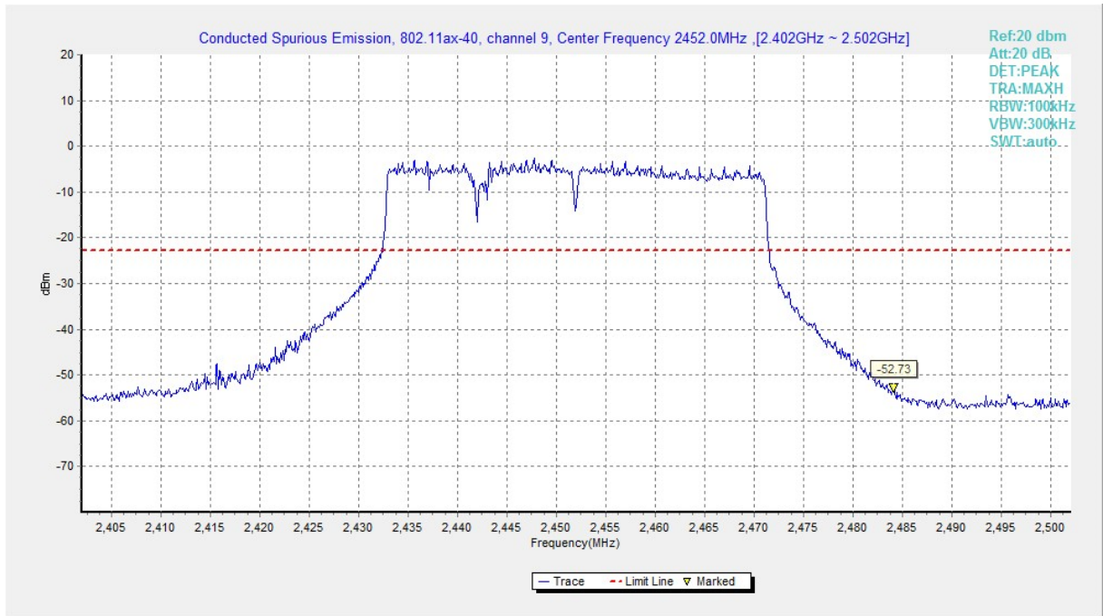
Fig.A.6.1.65 Transmitter Spurious Emission - Conducted 802.11ax-HE40, Ch9, Center Frequency)
