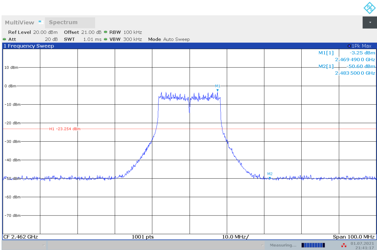
Fig.A.6.1.83 Transmitter Spurious Emission - Conducted (802.11g, Ch11, Center Frequency)
