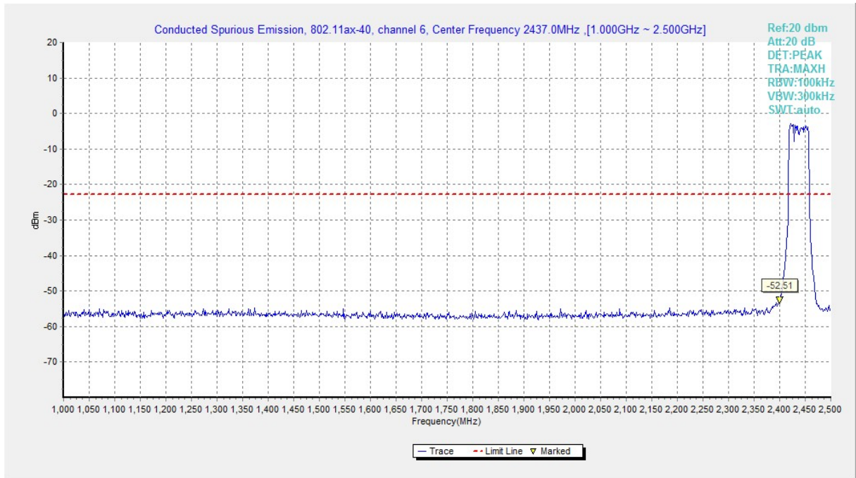
Fig.A.6.1.59 Transmitter Spurious Emission - Conducted (802.11ax-HE40, Ch6, 1 GHz-2.5 GHz)
