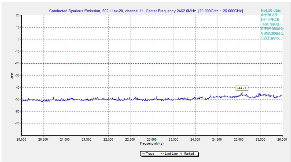
Fig.A.6.1.48 Transmitter Spurious Emission - Conducted (802.11ax-HE20, Ch11, 20 GHz-26 GHz)
