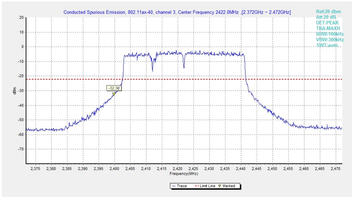
Fig.A.6.1.49 Transmitter Spurious Emission - Conducted (802.11ax-HE40, Ch3, Center Frequency)
