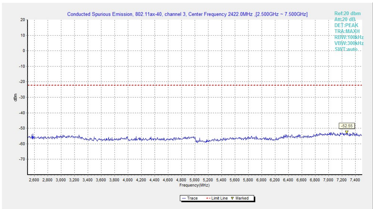
Fig.A.6.1.52 Transmitter Spurious Emission - Conducted (802.11ax-HE40, Ch3, 2.5 GHz-7.5 GHz)
