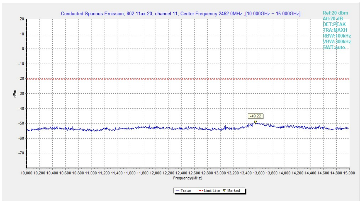
Fig.A.6.1.46 Transmitter Spurious Emission - Conducted (802.11ax-HE20, Ch11, 10 GHz-15 GHz)
