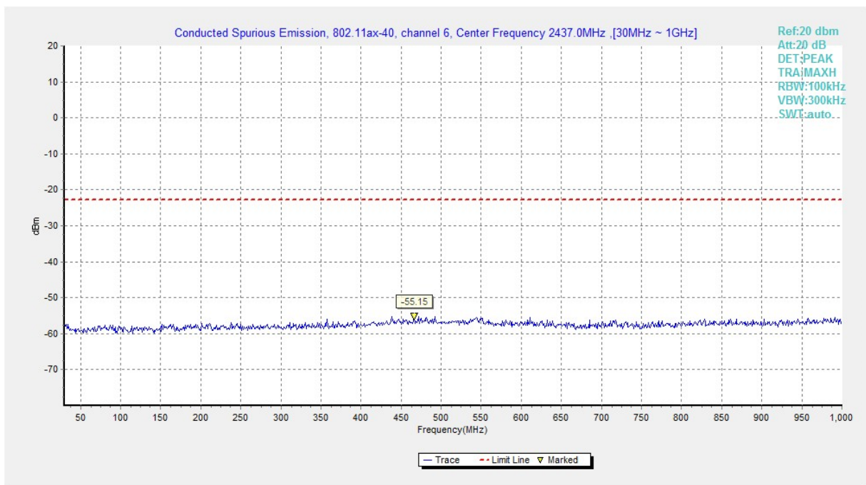
Fig.A.6.1.58 Transmitter Spurious Emission - Conducted (802.11ax-HE40, Ch6, 30 MHz-1 GHz)
