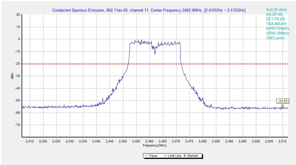
Fig.A.6.1.41 Transmitter Spurious Emission - Conducted (802.11ax-HE20, Ch11, Center Frequency)
