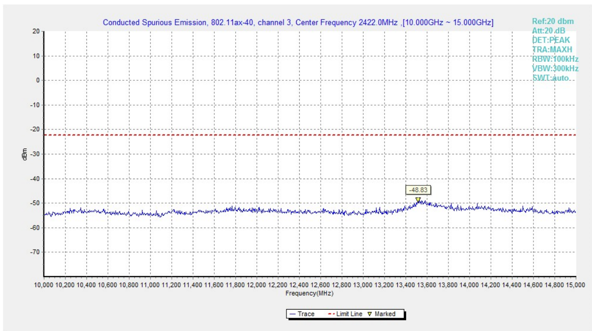
Fig.A.6.1.54 Transmitter Spurious Emission - Conducted (802.11ax-HE40, Ch3, 10 GHz-15 GHz)
