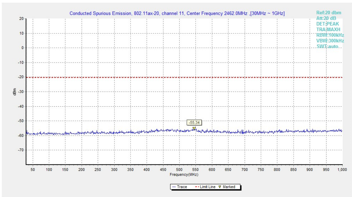
Fig.A.6.1.42 Transmitter Spurious Emission - Conducted (802.11ax-HE20, Ch11, 30 MHz-1 GHz)
