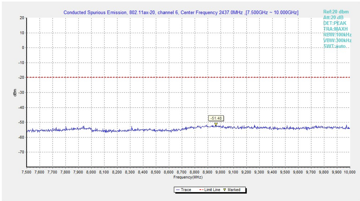
Fig.A.6.1.37 Transmitter Spurious Emission - Conducted (802.11ax-HE20, Ch6, 7.5 GHz-10 GHz)
