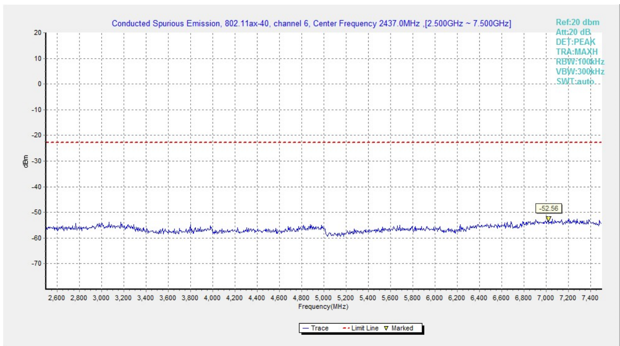
Fig.A.6.1.60 Transmitter Spurious Emission - Conducted (802.11ax-HE40, Ch6, 2.5 GHz-7.5 GHz)
