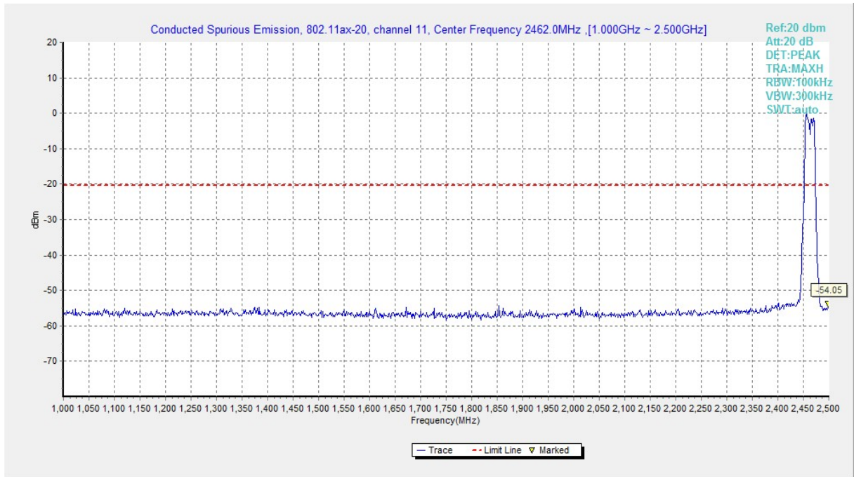
Fig.A.6.1.43 Transmitter Spurious Emission - Conducted (802.11ax-HE20, Ch11, 1 GHz-2.5 GHz)
