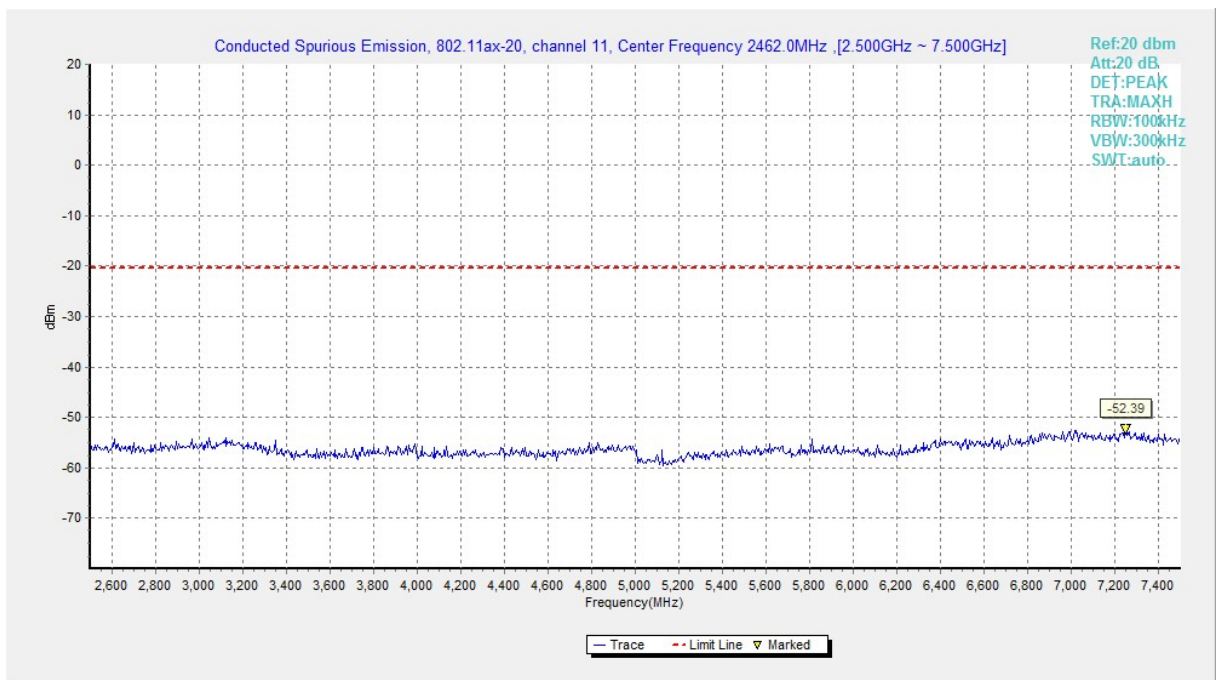
Fig.A.6.1.44 Transmitter Spurious Emission - Conducted (802.11ax-HE20, Ch11, 2.5 GHz-7.5 GHz)
