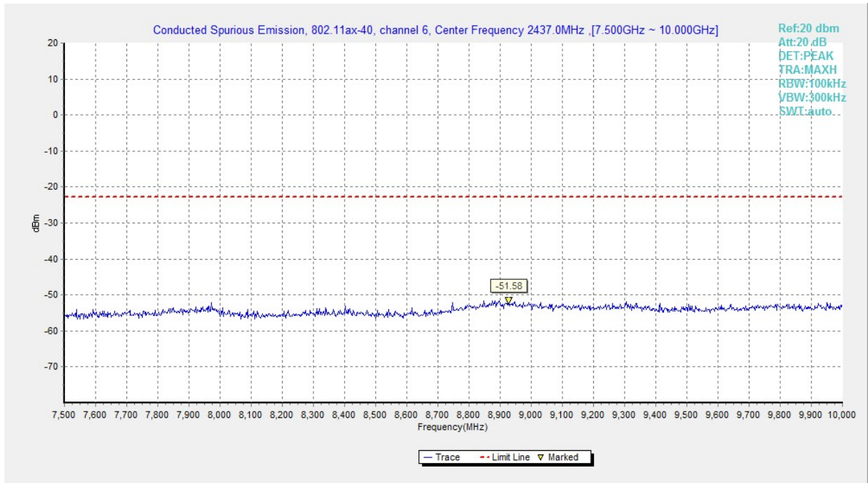
Fig.A.6.1.61 Transmitter Spurious Emission - Conducted (802.11ax-HE40, Ch6, 7.5 GHz-10 GHz)
