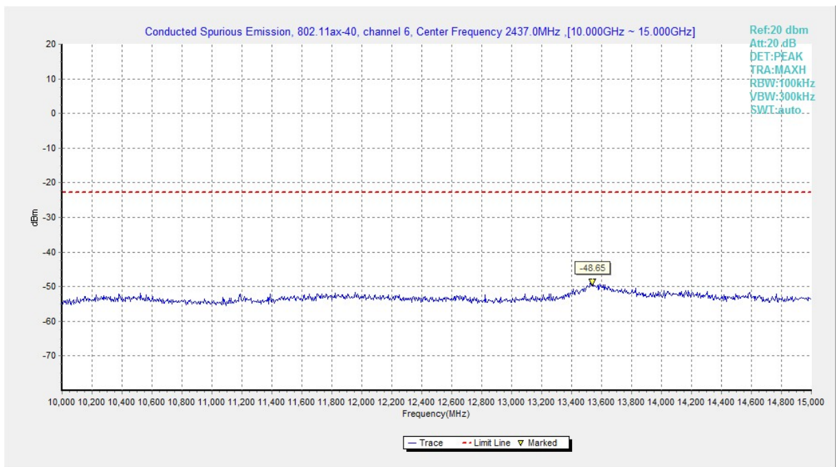
Fig.A.6.1.62 Transmitter Spurious Emission - Conducted (802.11ax-HE40, Ch6, 10 GHz-15 GHz)
