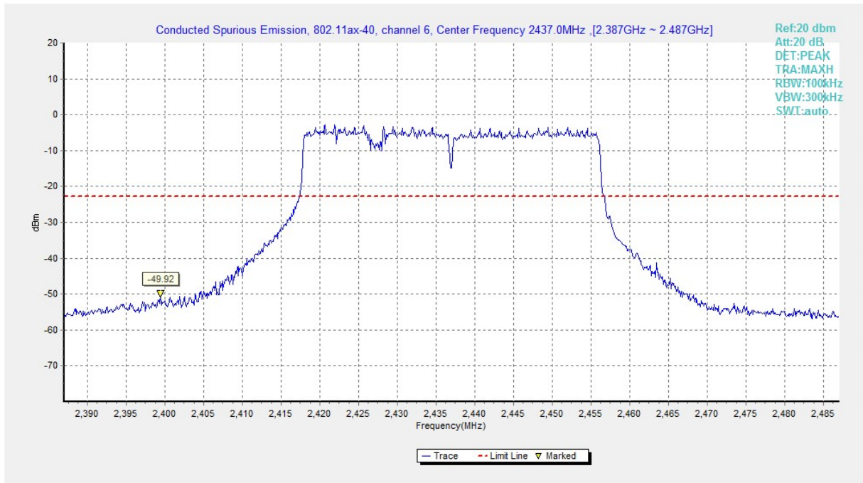
Fig.A.6.1.57 Transmitter Spurious Emission - Conducted (802.11ax-HE40, Ch6, Center Frequency)
