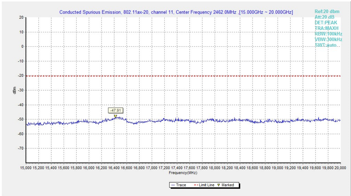
Fig.A.6.1.47 Transmitter Spurious Emission - Conducted (802.11ax-HE20, Ch11, 15 GHz-20 GHz)
