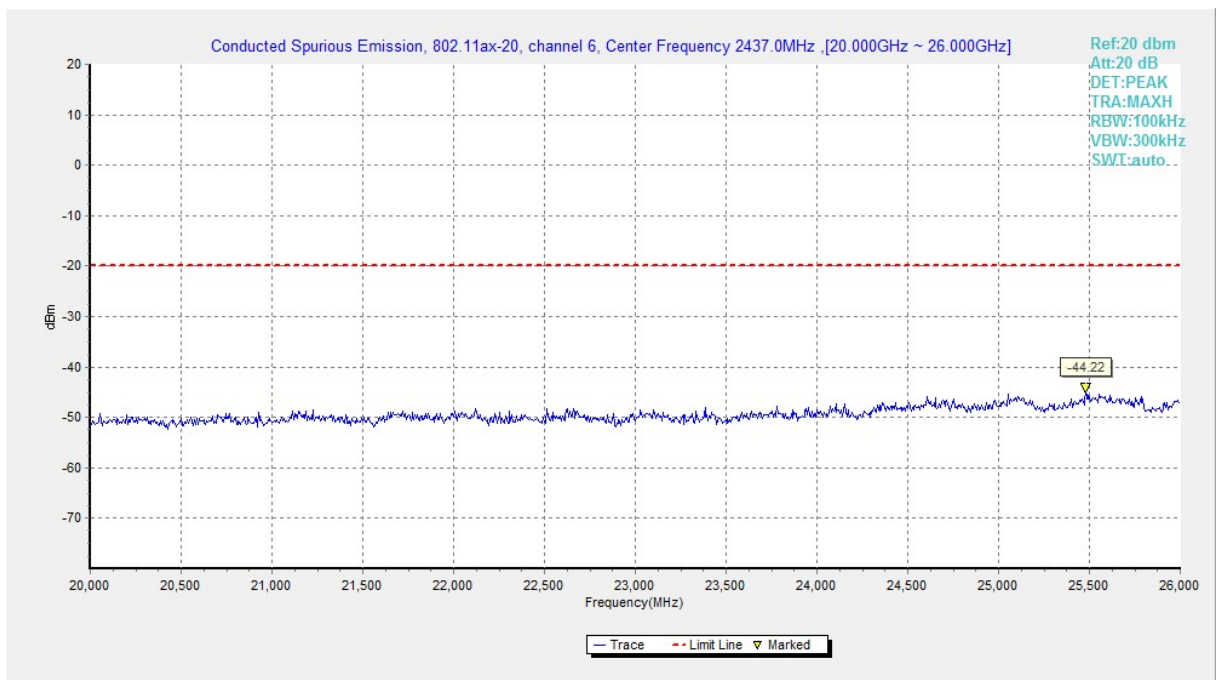
Fig.A.6.1.40 Transmitter Spurious Emission - Conducted (802.11ax-HE20, Ch6, 20 GHz-26 GHz)
