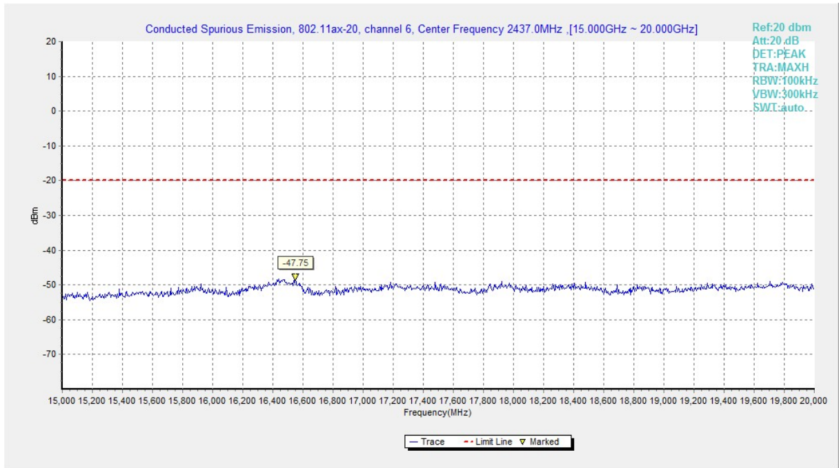
Fig.A.6.1.39 Transmitter Spurious Emission - Conducted (802.11ax-HE20, Ch6, 15 GHz-20 GHz)
