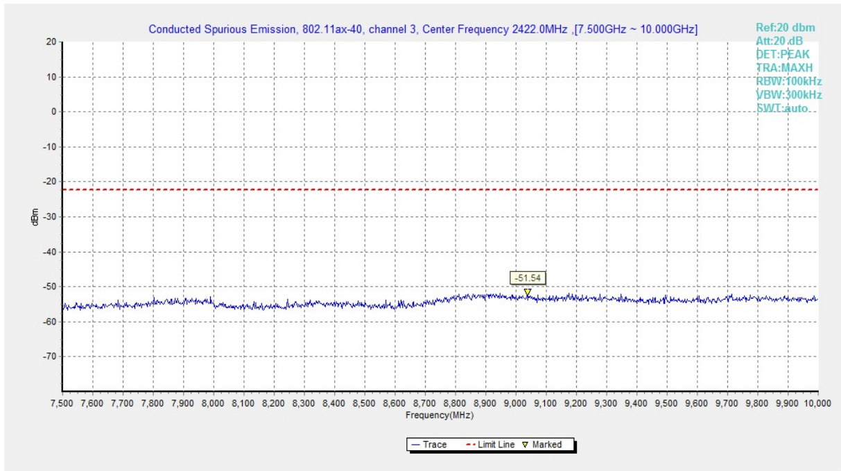
Fig.A.6.1.53 Transmitter Spurious Emission - Conducted (802.11ax-HE40, Ch3, 7.5 GHz-10 GHz)
