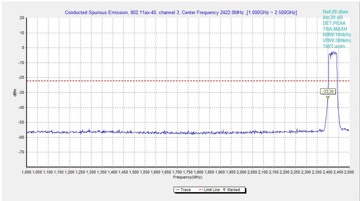
Fig.A.6.1.51 Transmitter Spurious Emission - Conducted (802.11ax-HE40, Ch3, 1 GHz-2.5 GHz)
