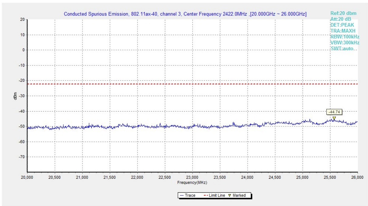
Fig.A.6.1.56 Transmitter Spurious Emission - Conducted (802.11ax-HE40, Ch3, 20 GHz-26 GHz)
