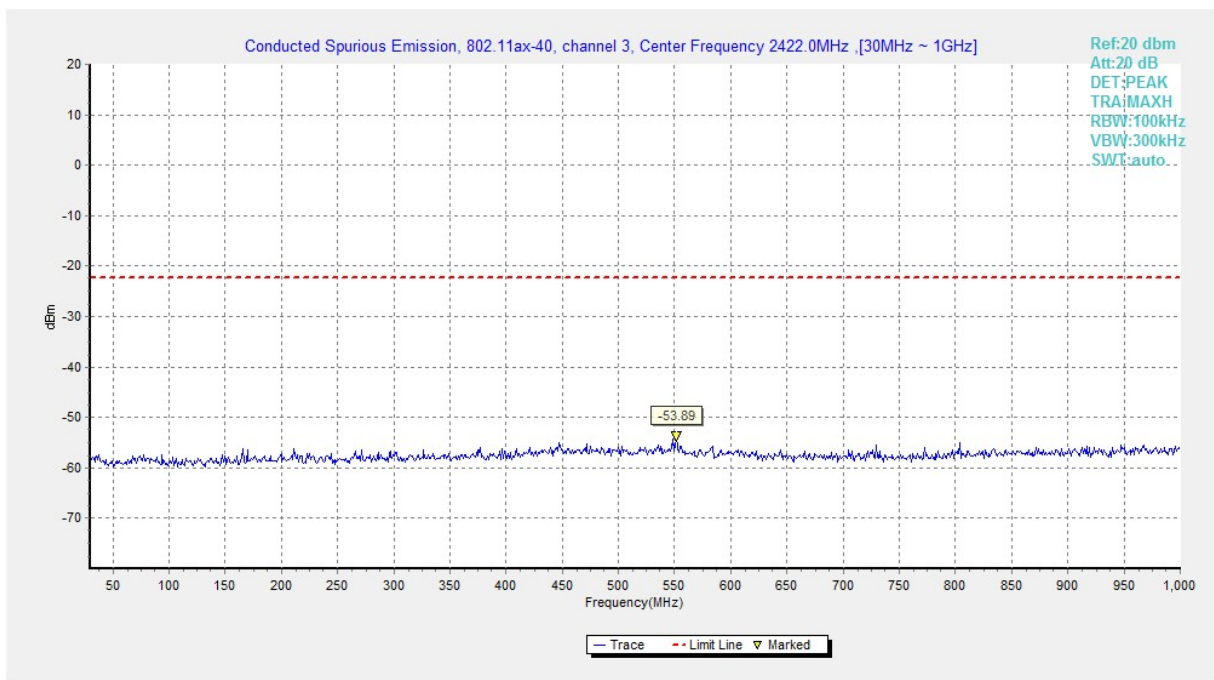
Fig.A.6.1.50 Transmitter Spurious Emission - Conducted (802.11ax-HE40, Ch3, 30 MHz-1 GHz)
