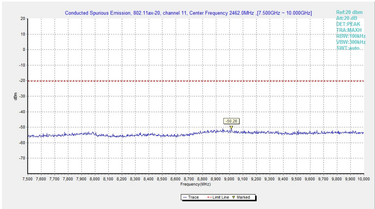
Fig.A.6.1.45 Transmitter Spurious Emission - Conducted (802.11ax-HE20, Ch11, 7.5 GHz-10 GHz)
