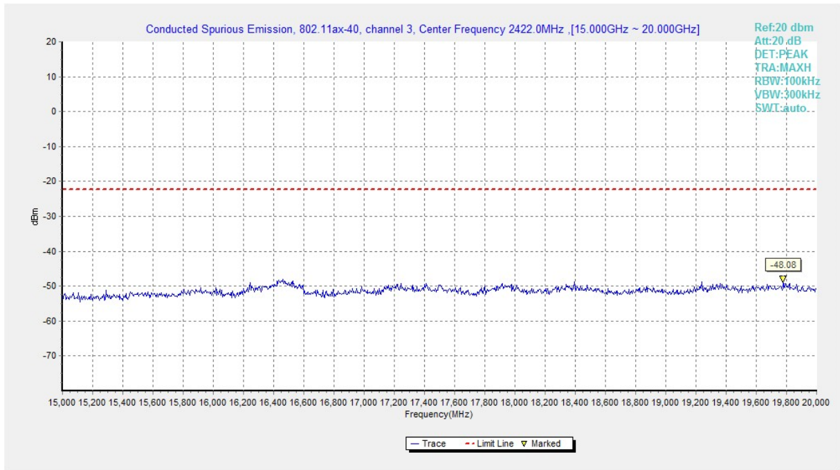
Fig.A.6.1.55 Transmitter Spurious Emission - Conducted (802.11ax-HE40, Ch3, 15 GHz-20 GHz)
