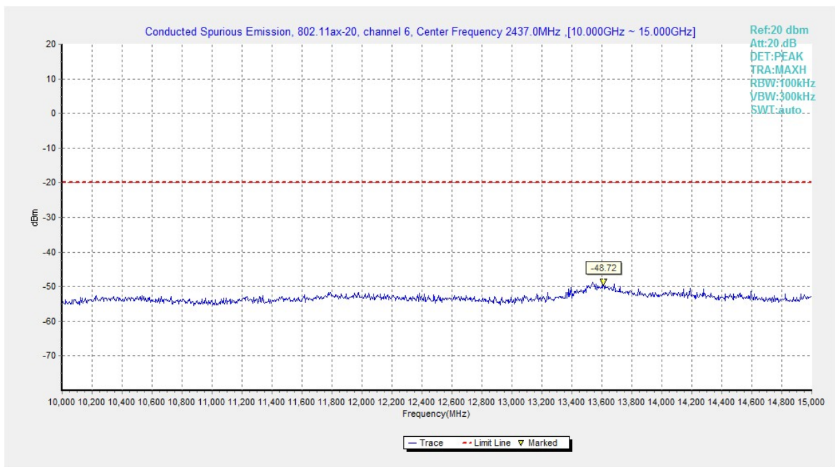
Fig.A.6.1.38 Transmitter Spurious Emission - Conducted (802.11ax-HE20, Ch6, 10 GHz-15 GHz)
