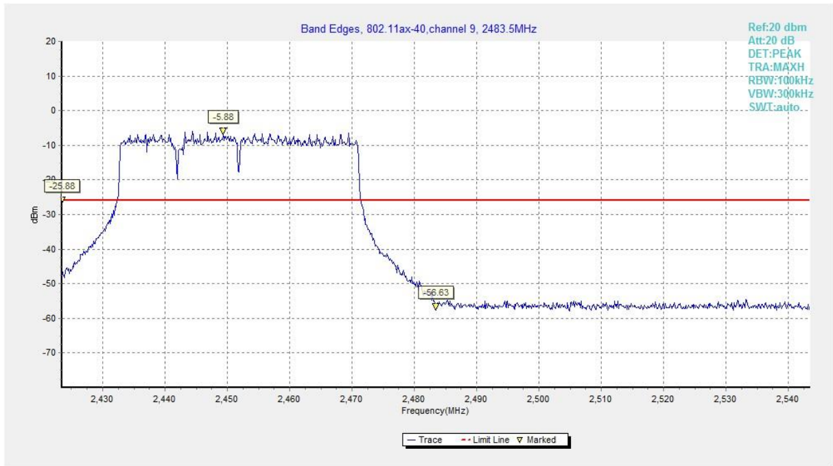
Fig.A.5.24 Band Edges (802.11ax-HE40, Ch 9)
