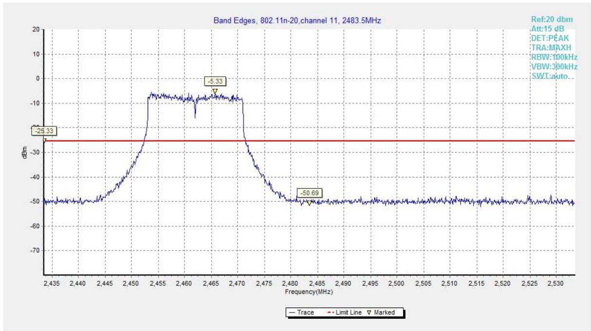
Fig.A.5.42 Band Edges (802.11n-HT20, Ch 11)
