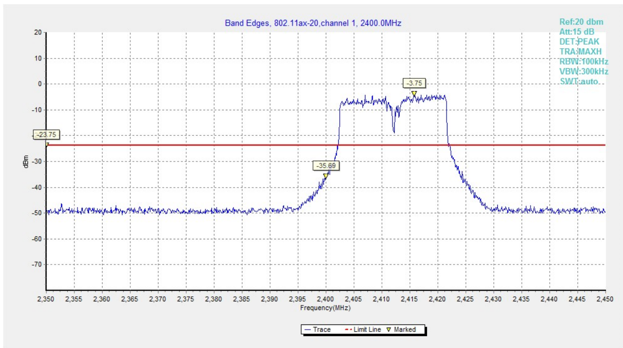
Fig.A.5.45 Band Edges (802.11ax-HE20, Ch 1)
