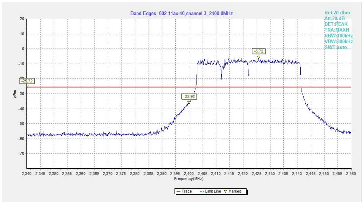
Fig.A.5.35 Band Edges (802.11ax-HE40, Ch 3)
