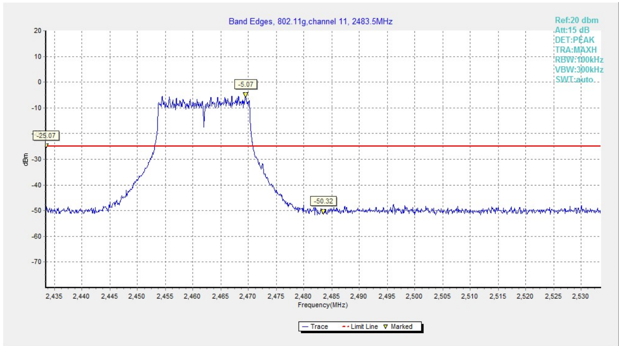
Fig.A.5.40 Band Edges (802.11g, Ch 11)
