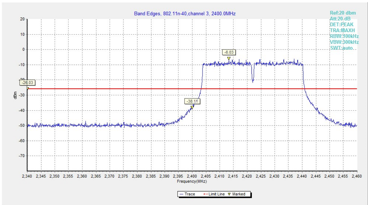
Fig.A.5.31 Band Edges (802.11n-HT40, Ch 3)
