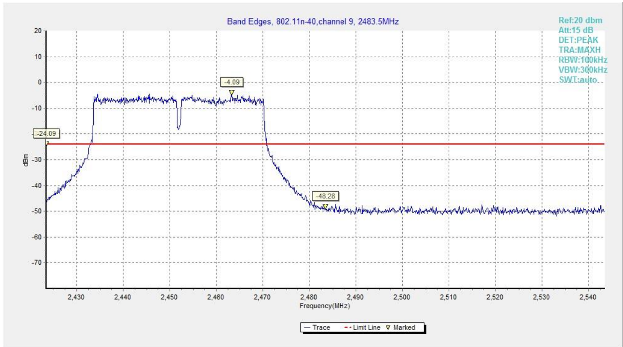
Fig.A.5.20 Band Edges (802.11n-HT40, Ch 9)
