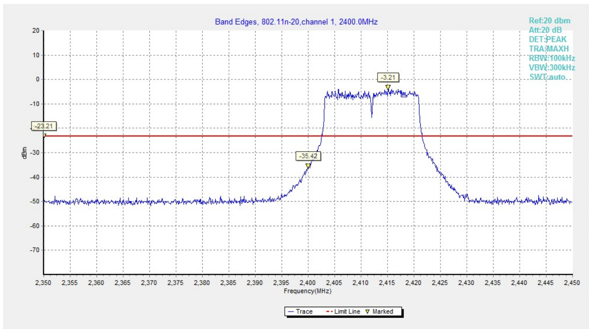
Fig.A.5.29 Band Edges (802.11n-HT20, Ch 1)
