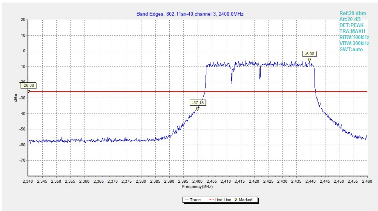
Fig.A.5.23 Band Edges (802.11ax-HE40, Ch 3)
