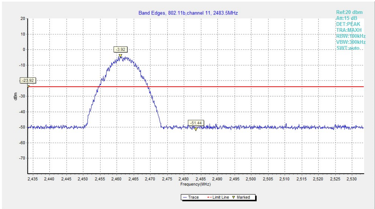
Fig.A.5.38 Band Edges (802.11b, Ch 11)
