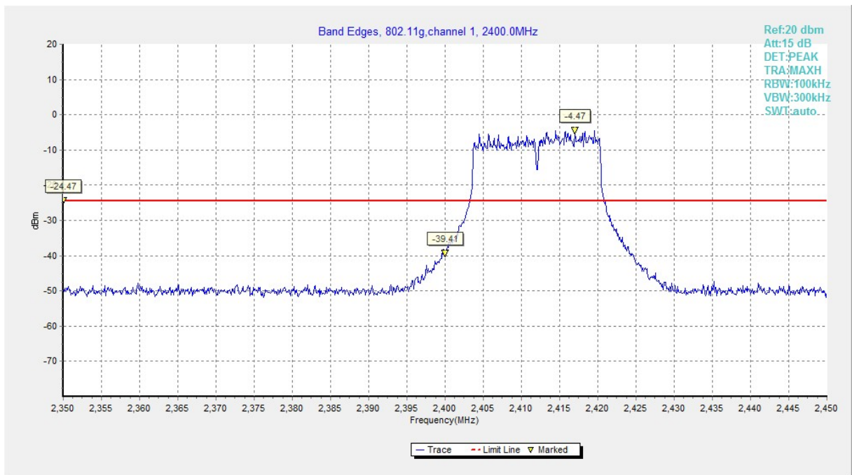
Fig.A.5.39 Band Edges (802.11g, Ch 1)
