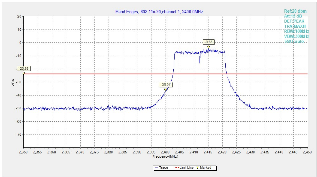
Fig.A.5.41 Band Edges (802.11n-HT20, Ch 1)
