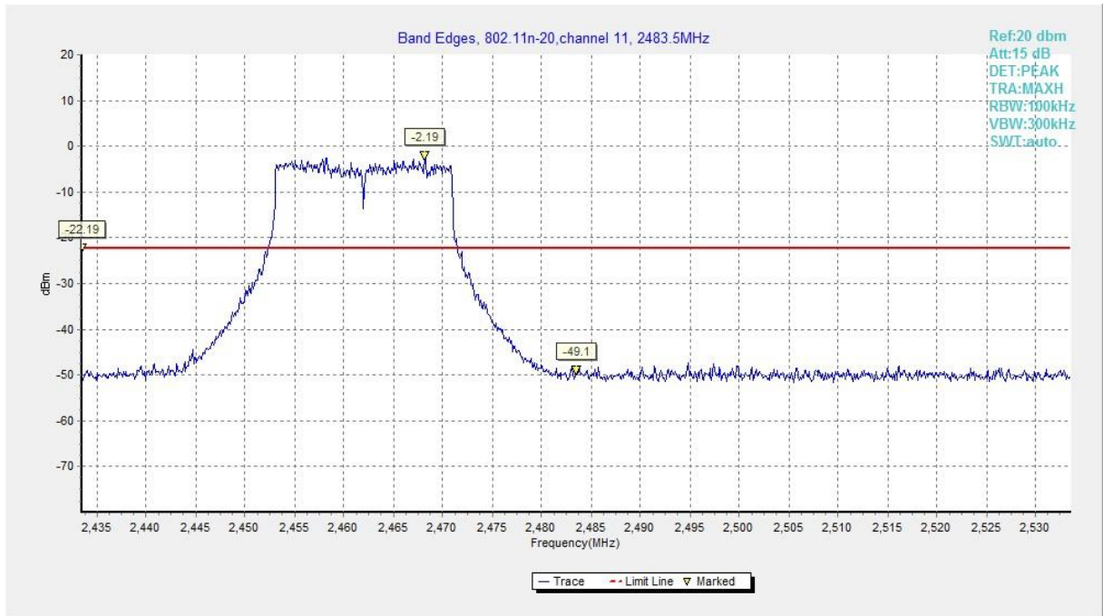
Fig.A.5.18 Band Edges (802.11n-HT20, Ch 11)
