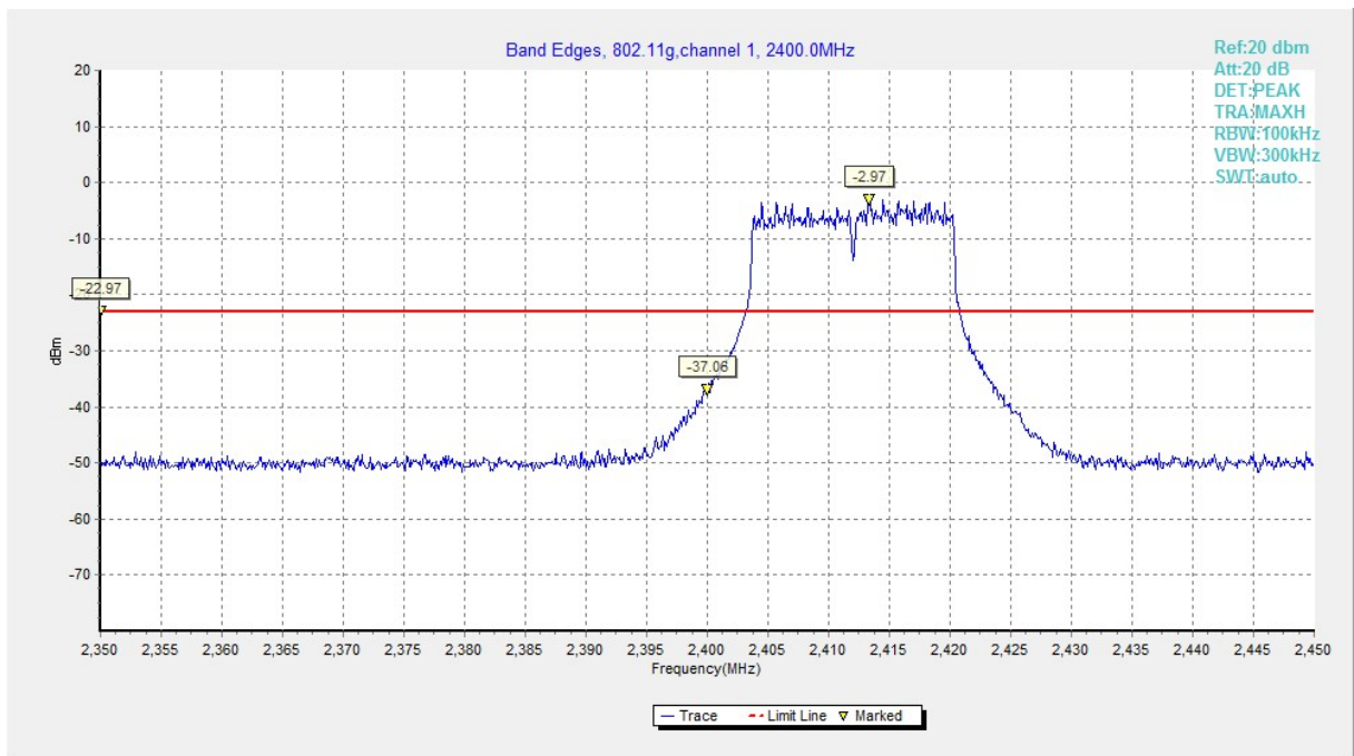
Fig.A.5.27 Band Edges (802.11g, Ch 1)
