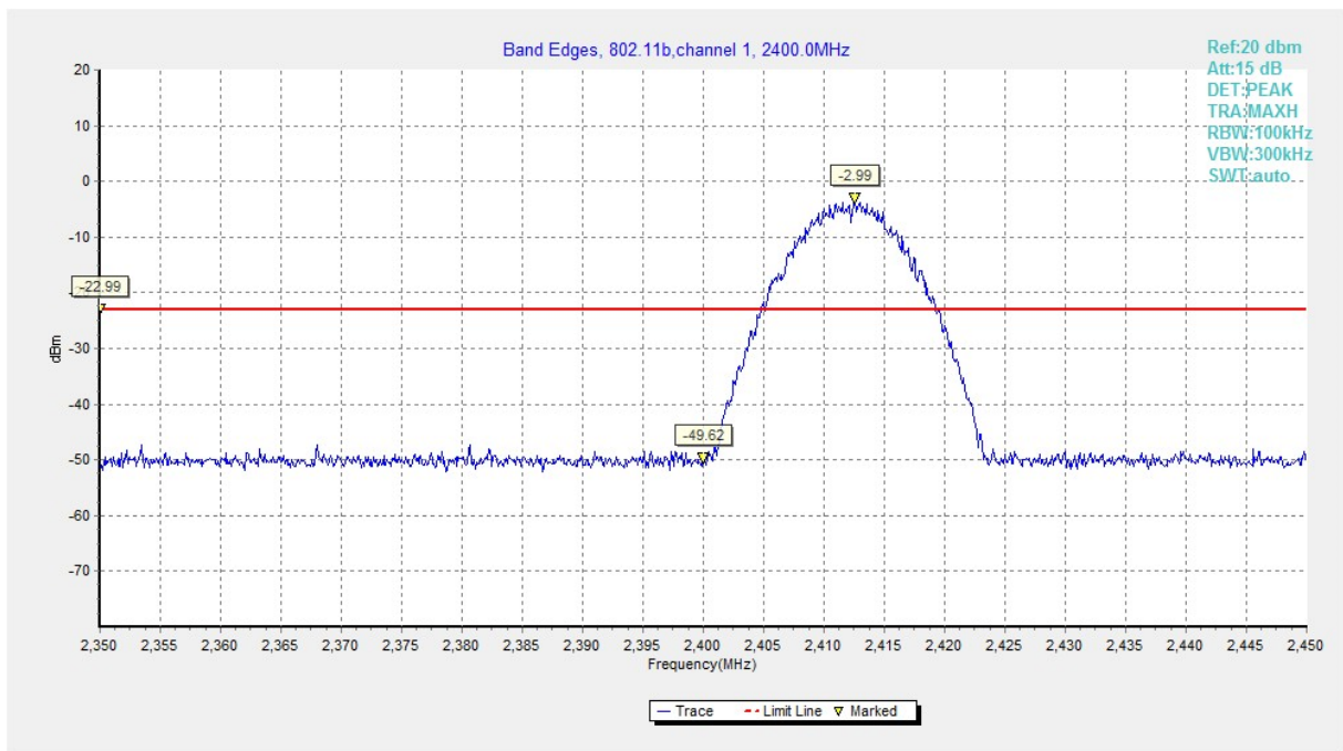
Fig.A.5.37 Band Edges (802.11b, Ch 1)
