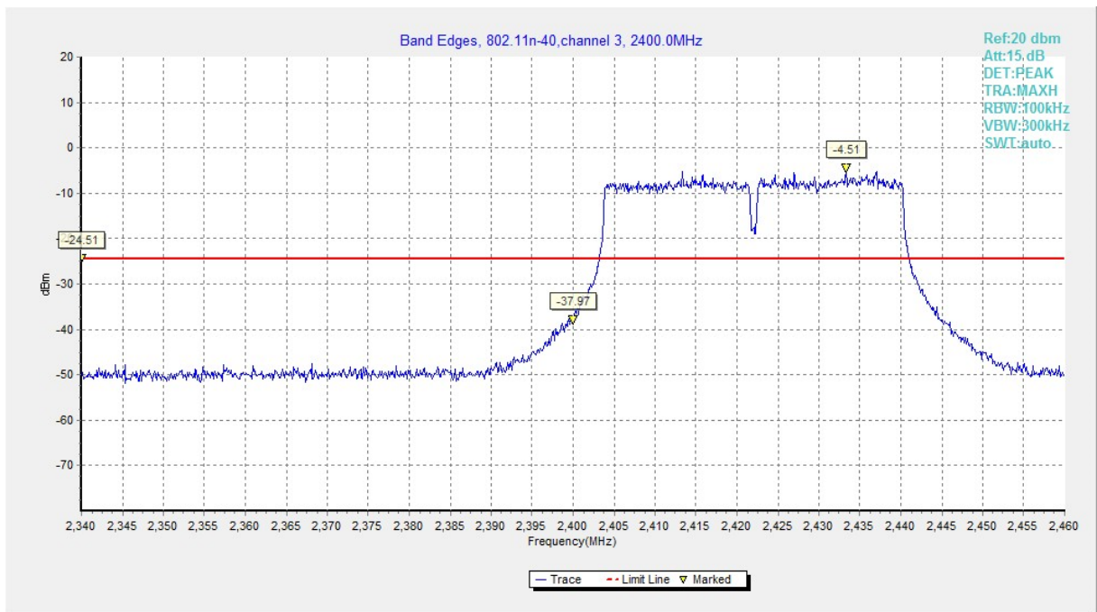
Fig.A.5.19 Band Edges (802.11n-HT40, Ch 3)
