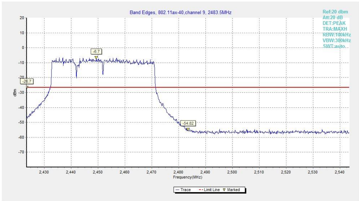
Fig.A.5.36 Band Edges (802.11ax-HE40, Ch 9)
