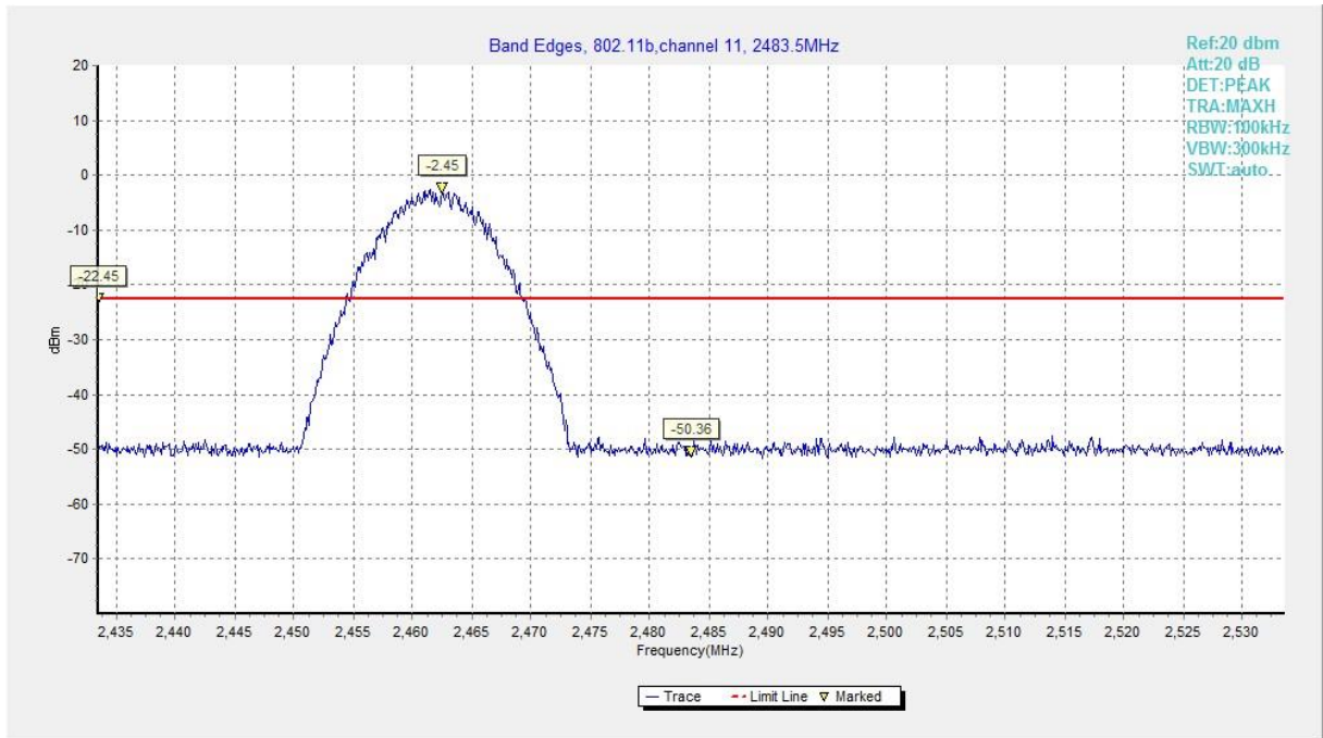
Fig.A.5.26 Band Edges (802.11b, Ch 11)
