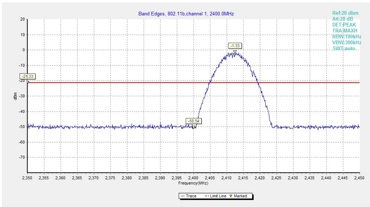
Fig.A.5.25 Band Edges (802.11b, Ch 1)
