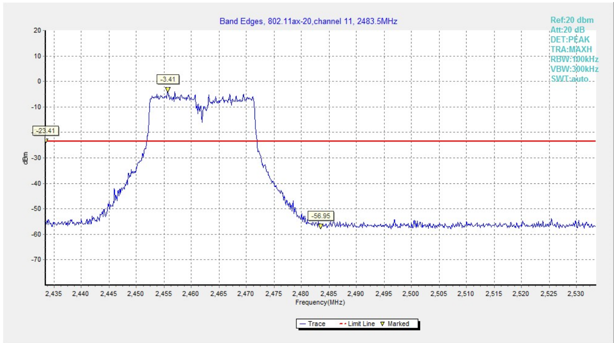
Fig.A.5.34 Band Edges (802.11ax-HE20, Ch 11)
