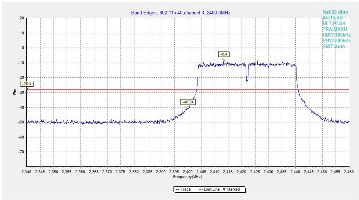
Fig.A.5.43 Band Edges (802.11n-HT40, Ch 3)
