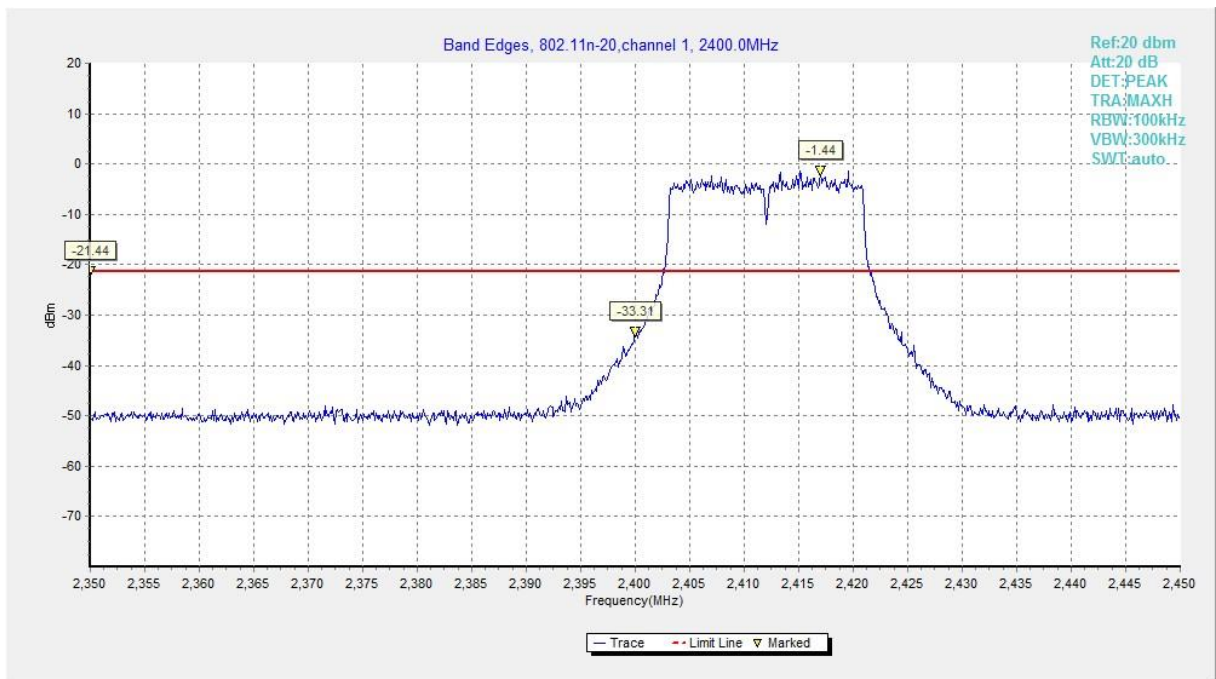
Fig.A.5.17 Band Edges (802.11n-HT20, Ch 1)
