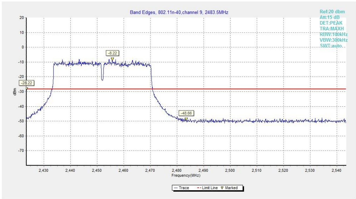
Fig.A.5.44 Band Edges (802.11n-HT40, Ch 9)
