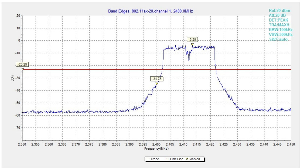
Fig.A.5.21 Band Edges (802.11ax-HE20, Ch 1)
