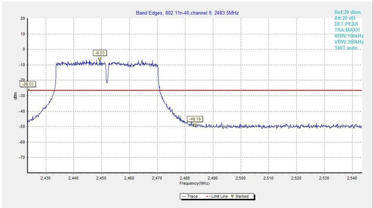
Fig.A.5.32 Band Edges (802.11n-HT40, Ch 9)
