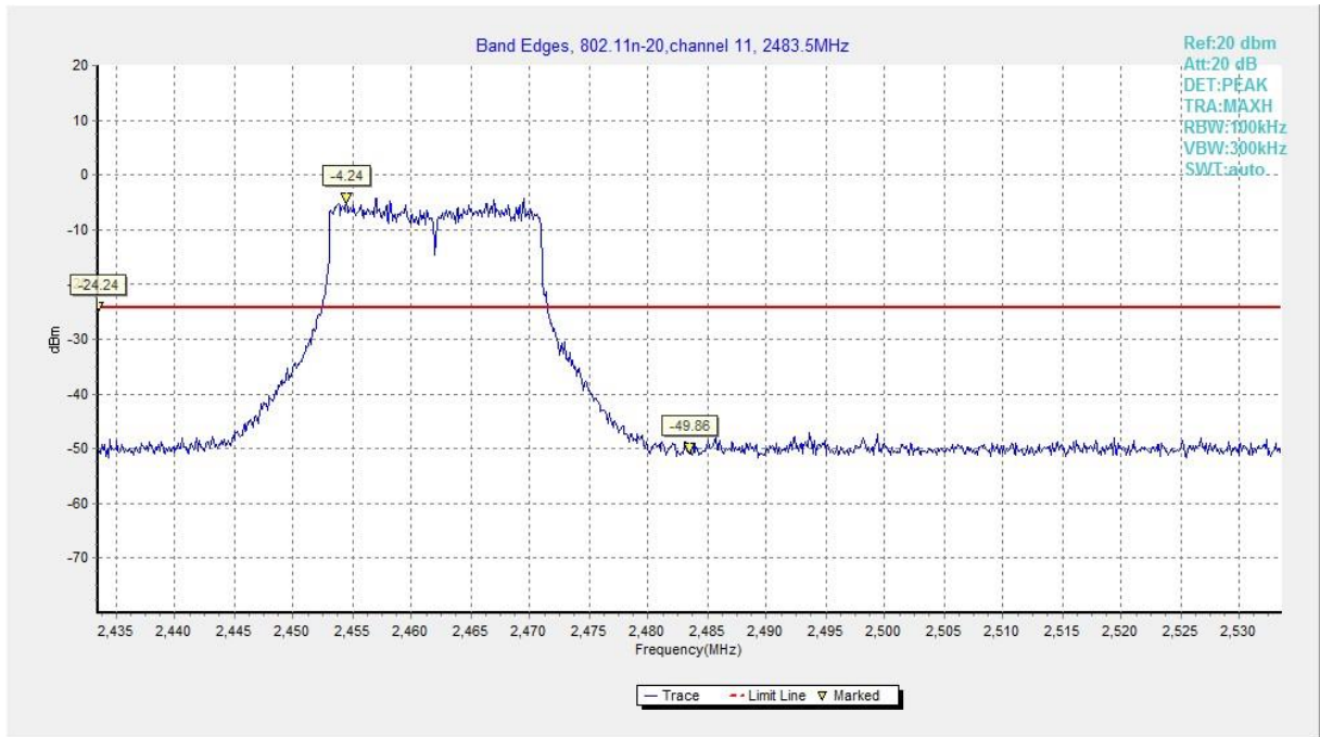
Fig.A.5.30 Band Edges (802.11n-HT20, Ch 11)
