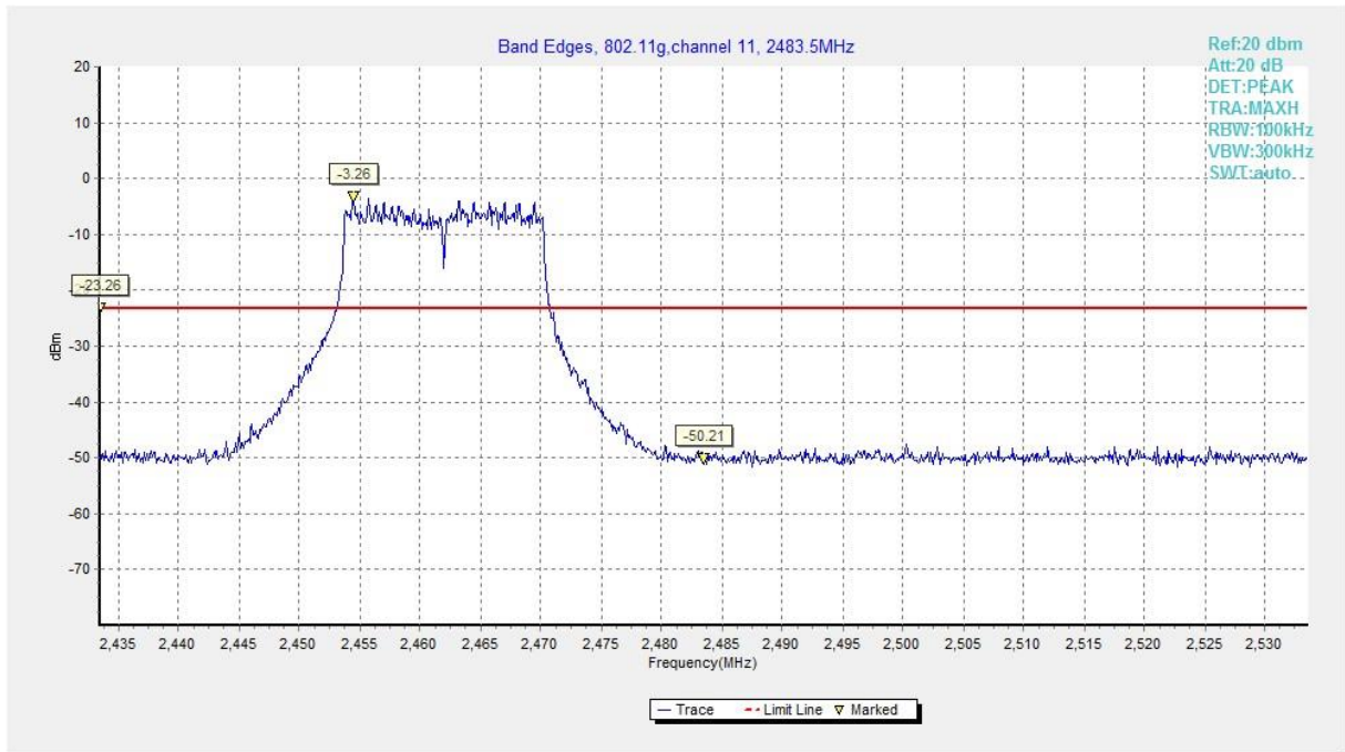
Fig.A.5.28 Band Edges (802.11g, Ch 11)
