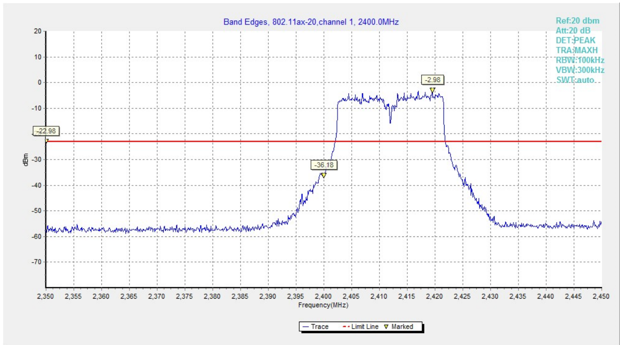
Fig.A.5.33 Band Edges (802.11ax-HE20, Ch 1)
