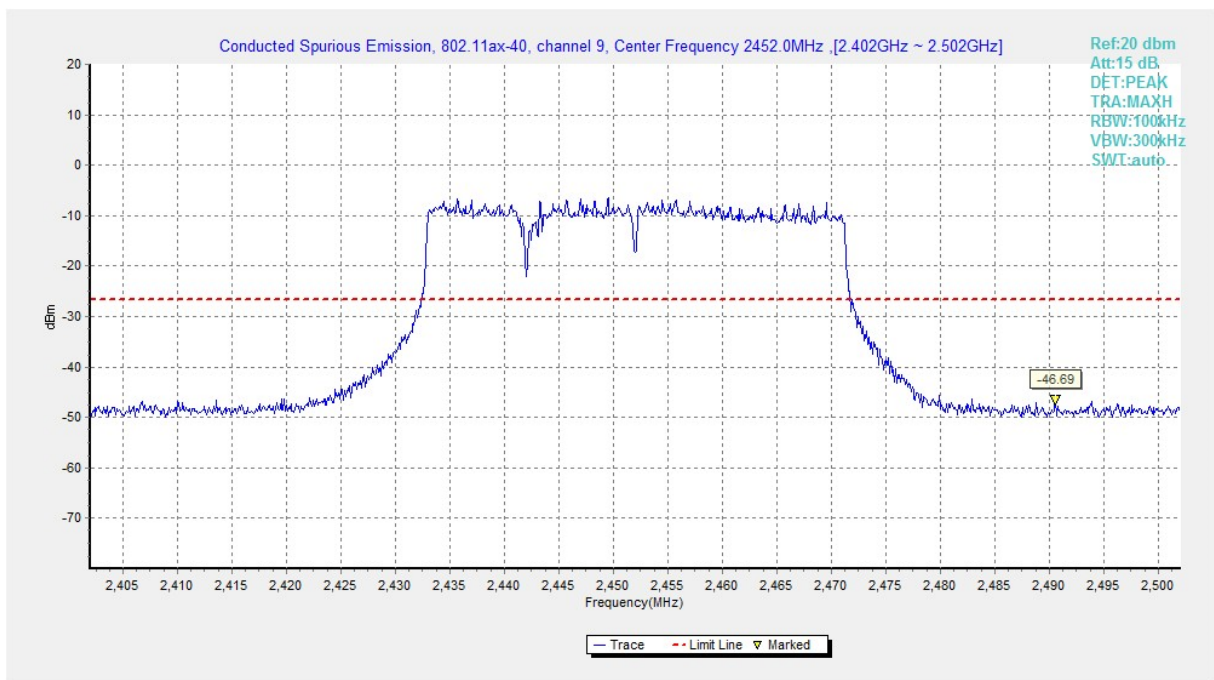
Fig.A.6.1.281 Transmitter Spurious Emission - Conducted 802.11ax-HE40, Ch9, Center Frequency)
