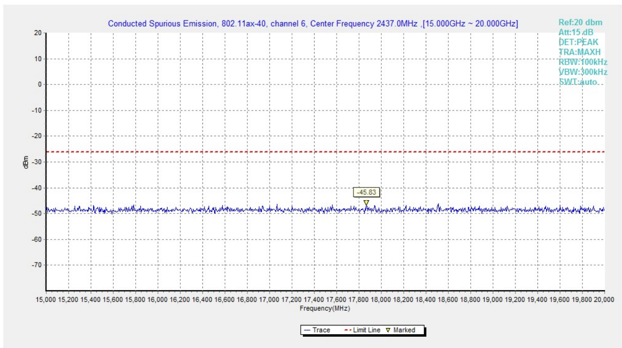
Fig.A.6.1.279 Transmitter Spurious Emission - Conducted (802.11ax-HE40, Ch6, 15 GHz-20 GHz)
