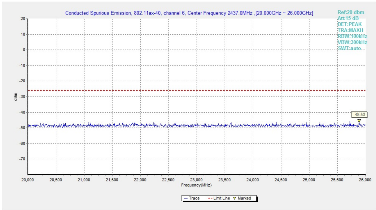
Fig.A.6.1.280 Transmitter Spurious Emission - Conducted (802.11ax-HE40, Ch6, 20 GHz-26 GHz)
