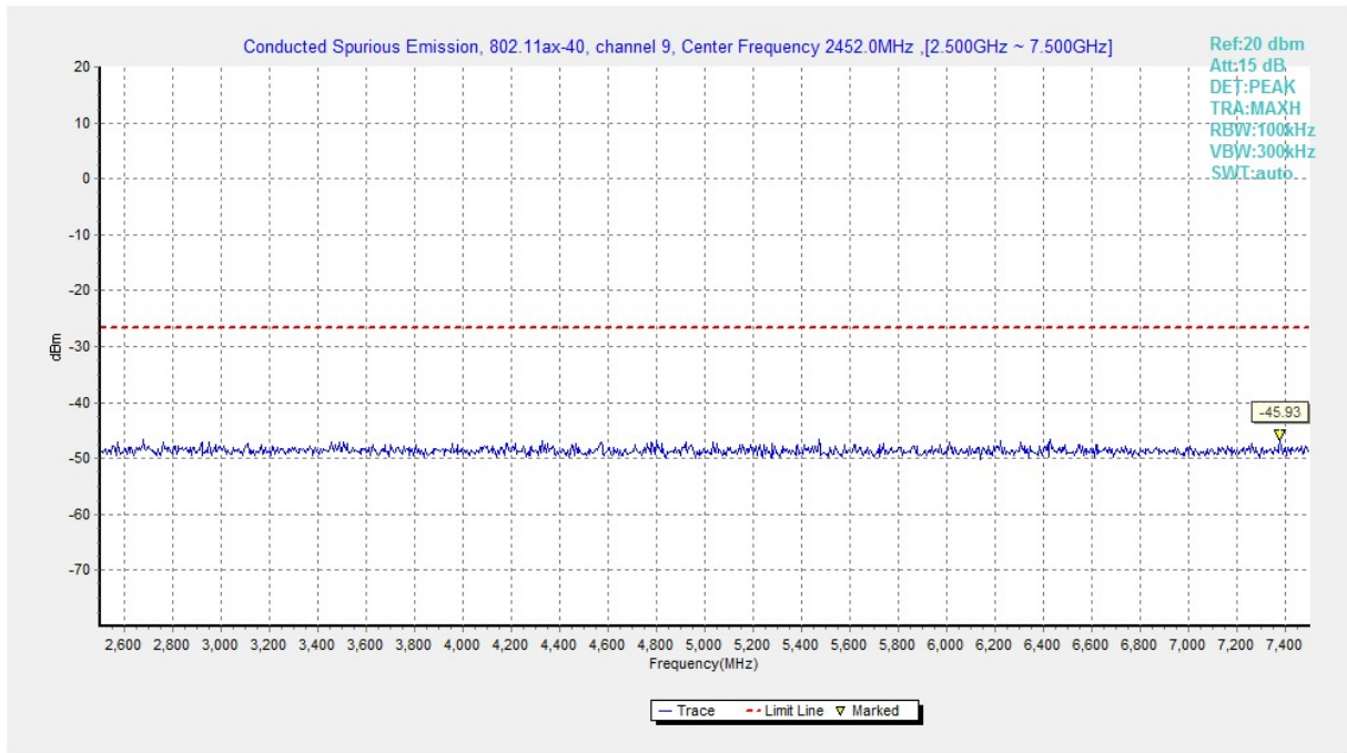
Fig.A.6.1.284 Transmitter Spurious Emission - Conducted (802.11ax-HE40, Ch9, 2.5 GHz-7.5 GHz)
