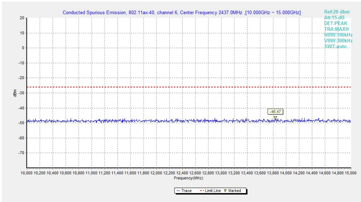
Fig.A.6.1.278 Transmitter Spurious Emission - Conducted (802.11ax-HE40, Ch6, 10 GHz-15 GHz)
