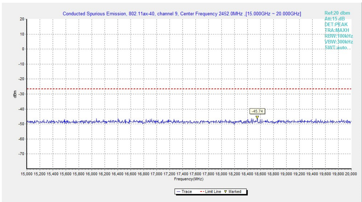
Fig.A.6.1.287 Transmitter Spurious Emission - Conducted (802.11ax-HE40, Ch9, 15 GHz-20 GHz)
