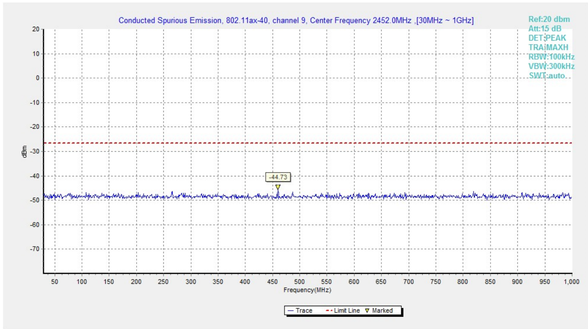
Fig.A.6.1.282 Transmitter Spurious Emission - Conducted (802.11ax-HE40, Ch9, 30 MHz-1 GHz)
