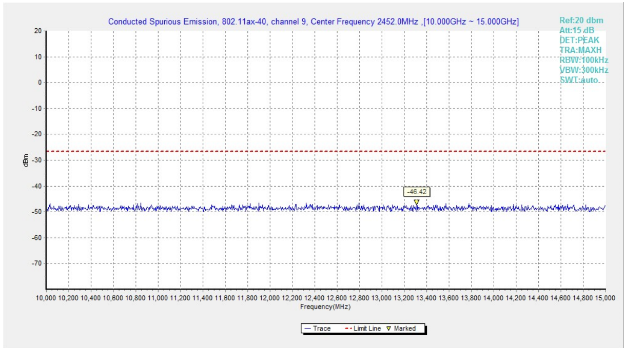
Fig.A.6.1.286 Transmitter Spurious Emission - Conducted (802.11ax-HE40, Ch9, 10 GHz-15 GHz)
