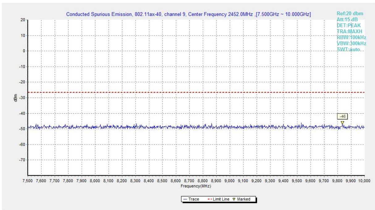
Fig.A.6.1.285 Transmitter Spurious Emission - Conducted (802.11ax-HE40, Ch9, 7.5 GHz-10 GHz)
