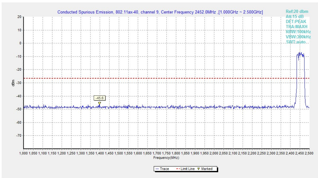
Fig.A.6.1.283 Transmitter Spurious Emission - Conducted (802.11ax-HE40, Ch9, 1 GHz-2.5 GHz)
