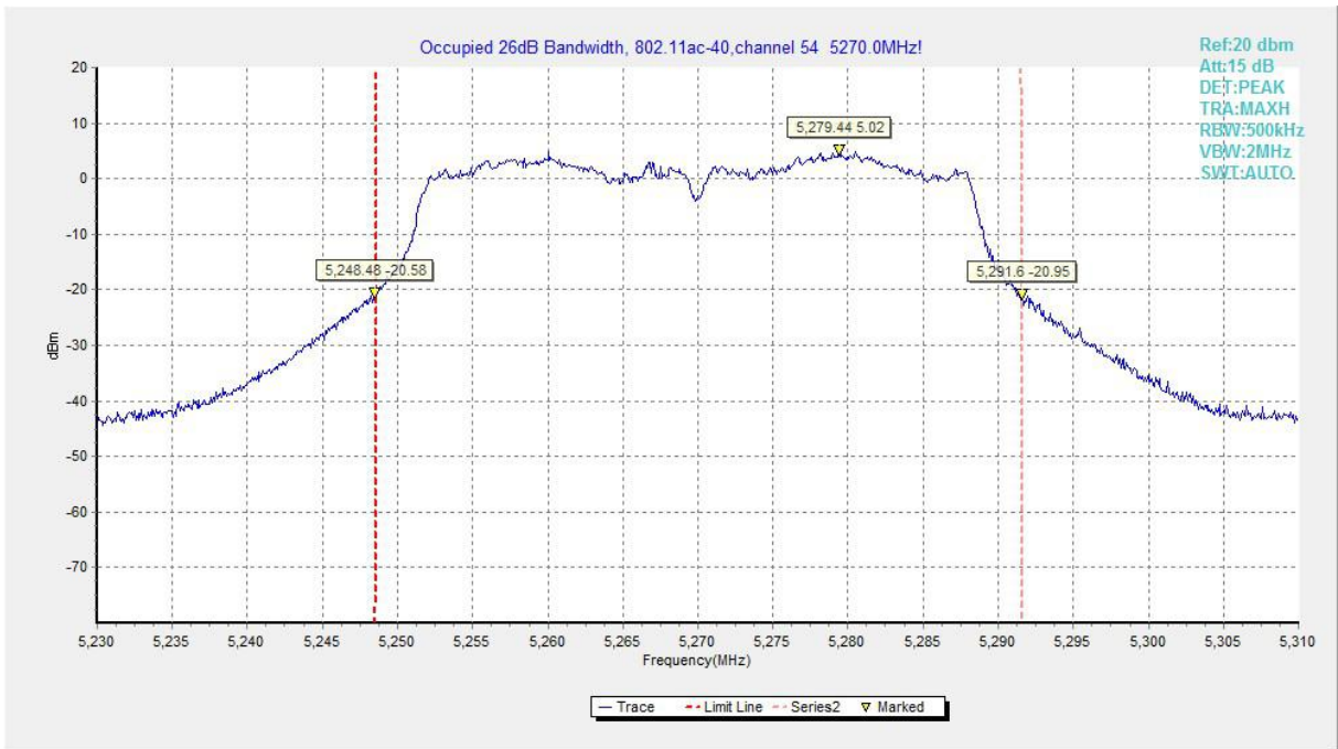
Fig.119 Occupied 26dB Bandwidth (802.11ac-HT40, 5270MHz)
