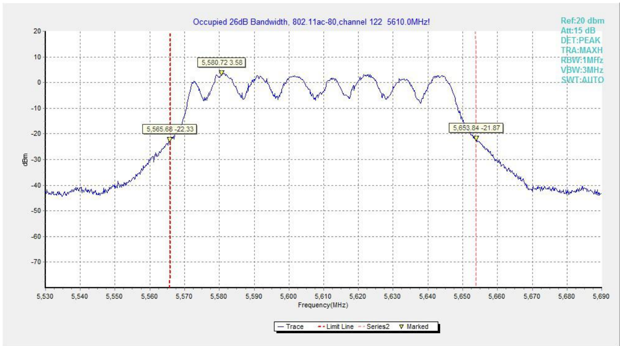
Fig.127 Occupied 26dB Bandwidth (802. 11ac-HT80, 5610MHz)
