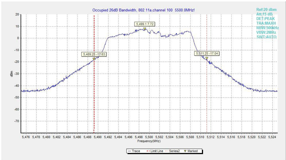
Fig.105 Occupied 26dB Bandwidth (802.11a, 5500MHz)
