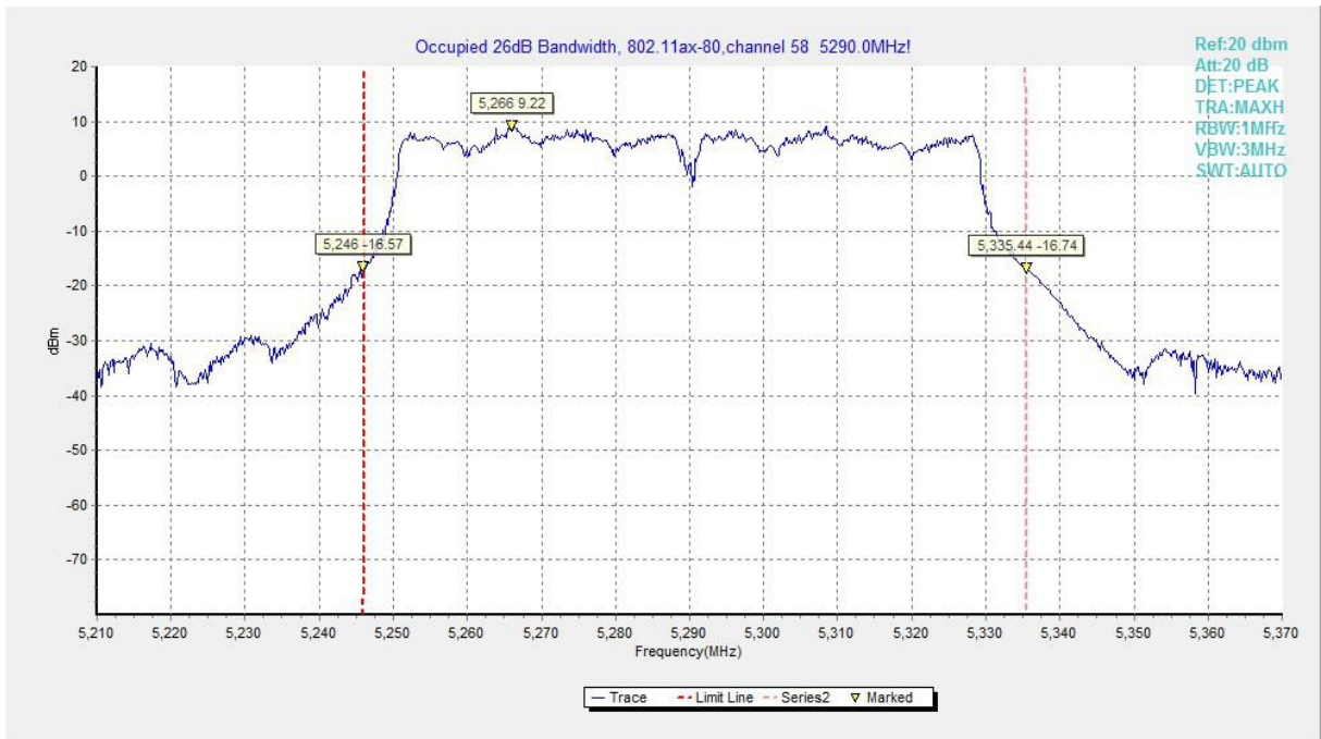
Fig.145 Occupied 26dB Bandwidth (802.11ax-HE80, 5290MHz)
