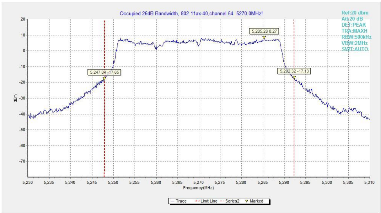
Fig.139 Occupied 26dB Bandwidth (802.11ax-HE40, 5270MHz)
