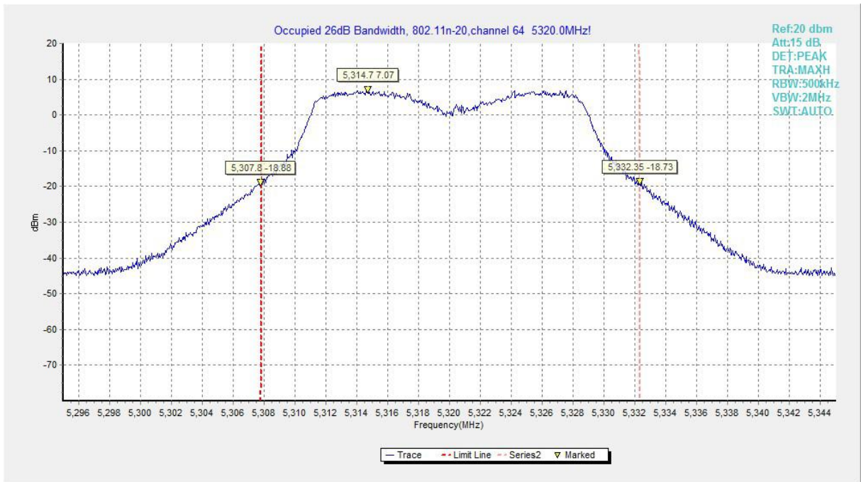
Fig.113 Occupied 26dB Bandwidth (802.11n-HT20, 5320MHz)
