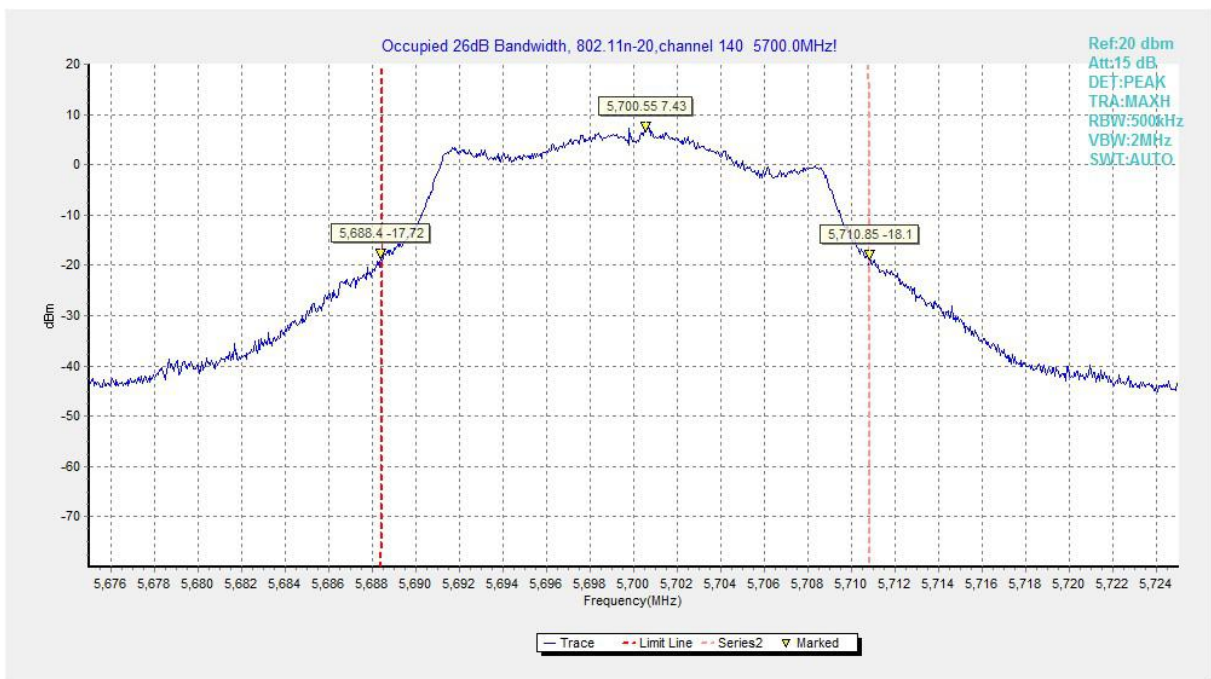
Fig.116 Occupied 26dB Bandwidth (802. 11n-HT20, 5700MHz)
