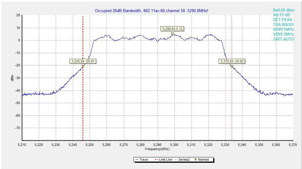
Fig.125 Occupied 26dB Bandwidth (802. 11ac-HT80, 5290MHz)
