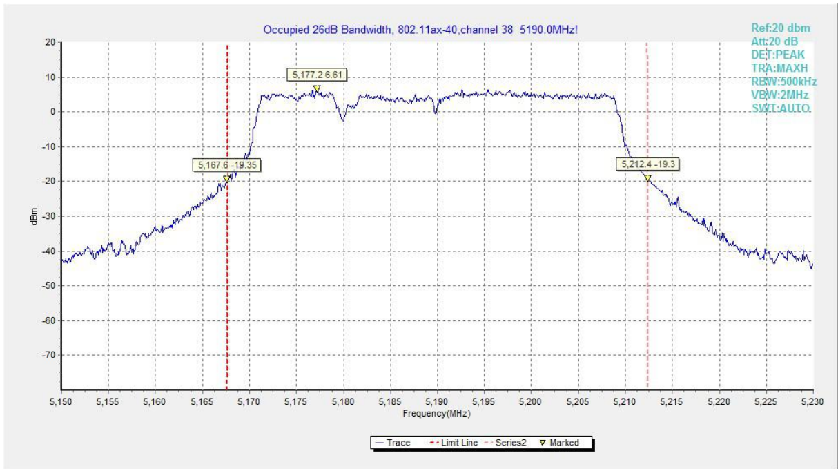
Fig.137 Occupied 26dB Bandwidth (802.11ax-HE40, 5190MHz)
