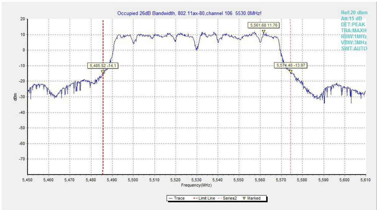
Fig.97 Occupied 26dB Bandwidth (802.11ax-HE80,5530MHz)
