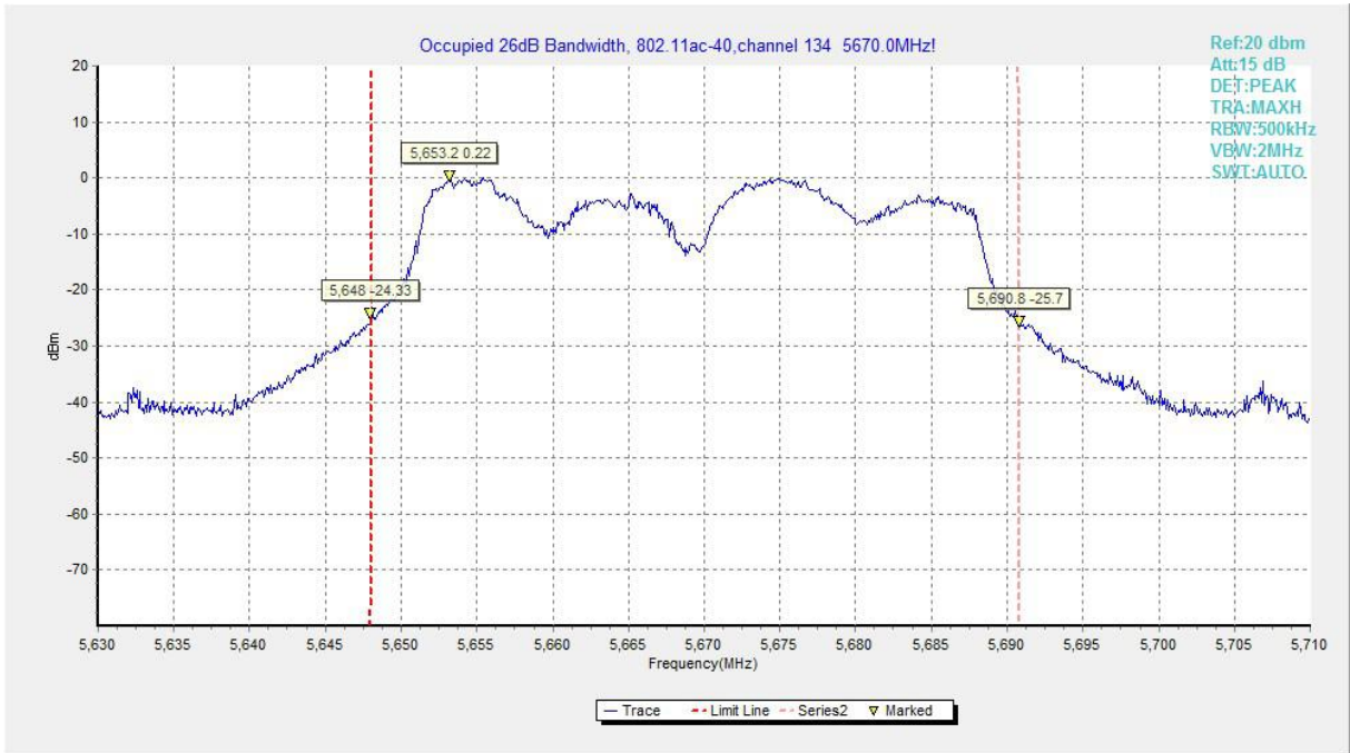
Fig.123 Occupied 26dB Bandwidth (802.11ac-HT40, 5670MHz)
