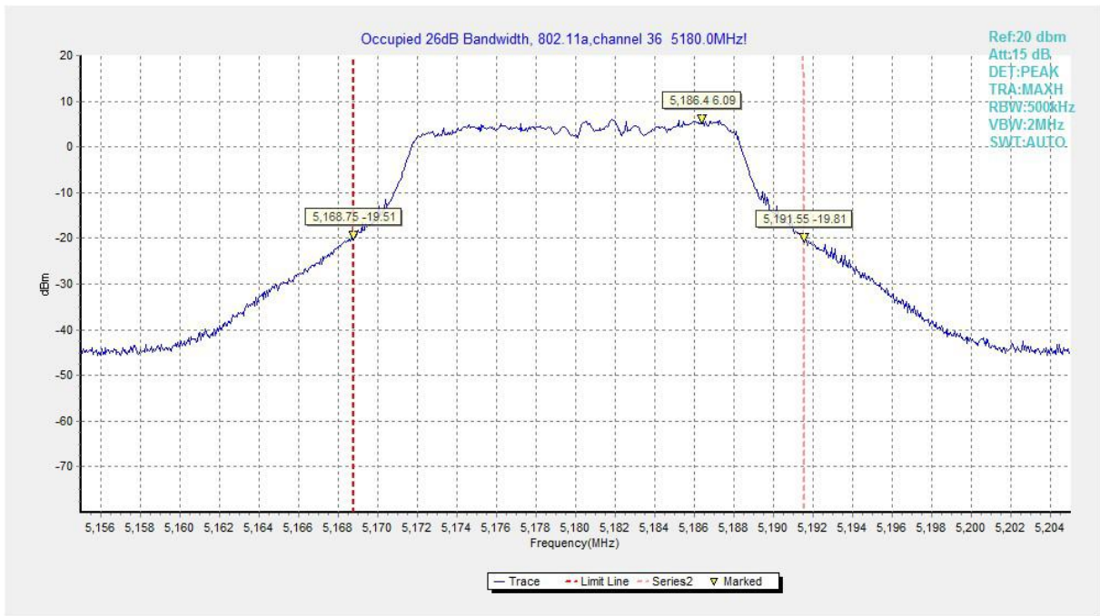
Fig.99 Occupied 26dB Bandwidth (802.11a, 5180MHz)
