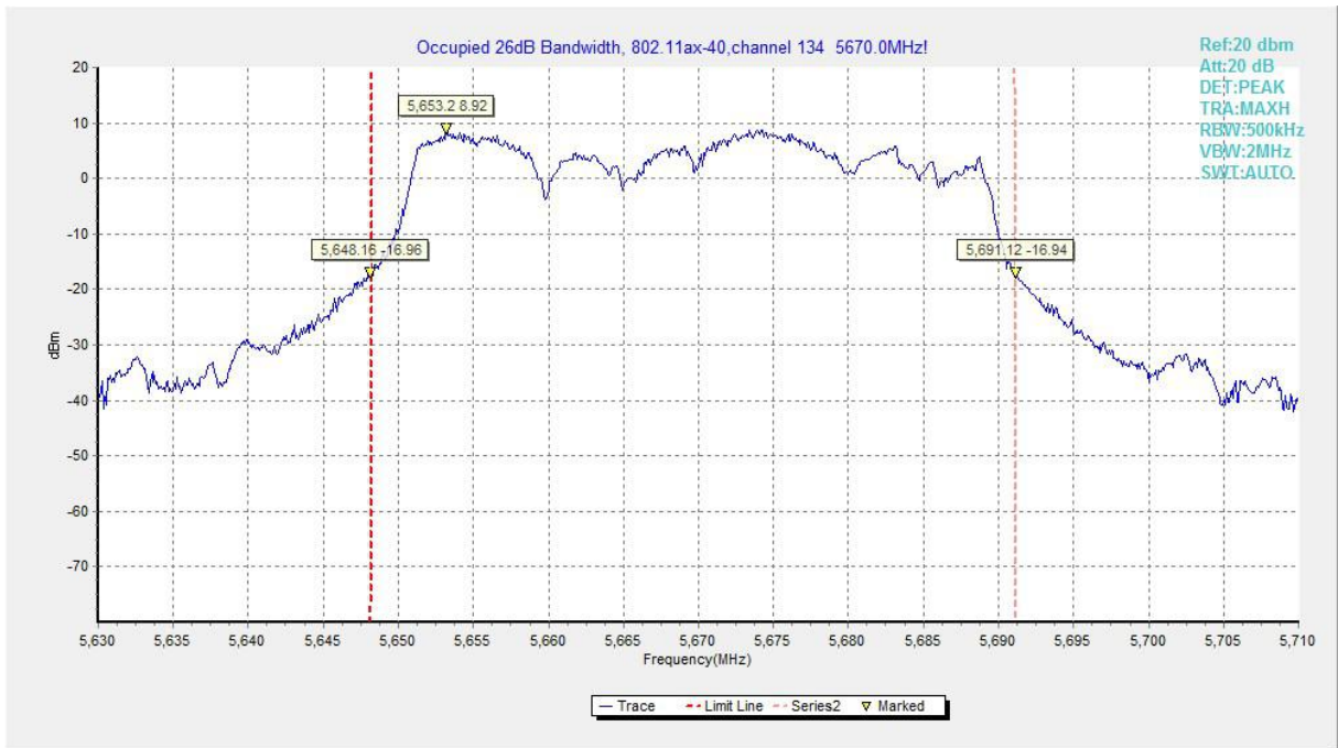
Fig.143 Occupied 26dB Bandwidth (802.11ax-HE40, 5670MHz)
