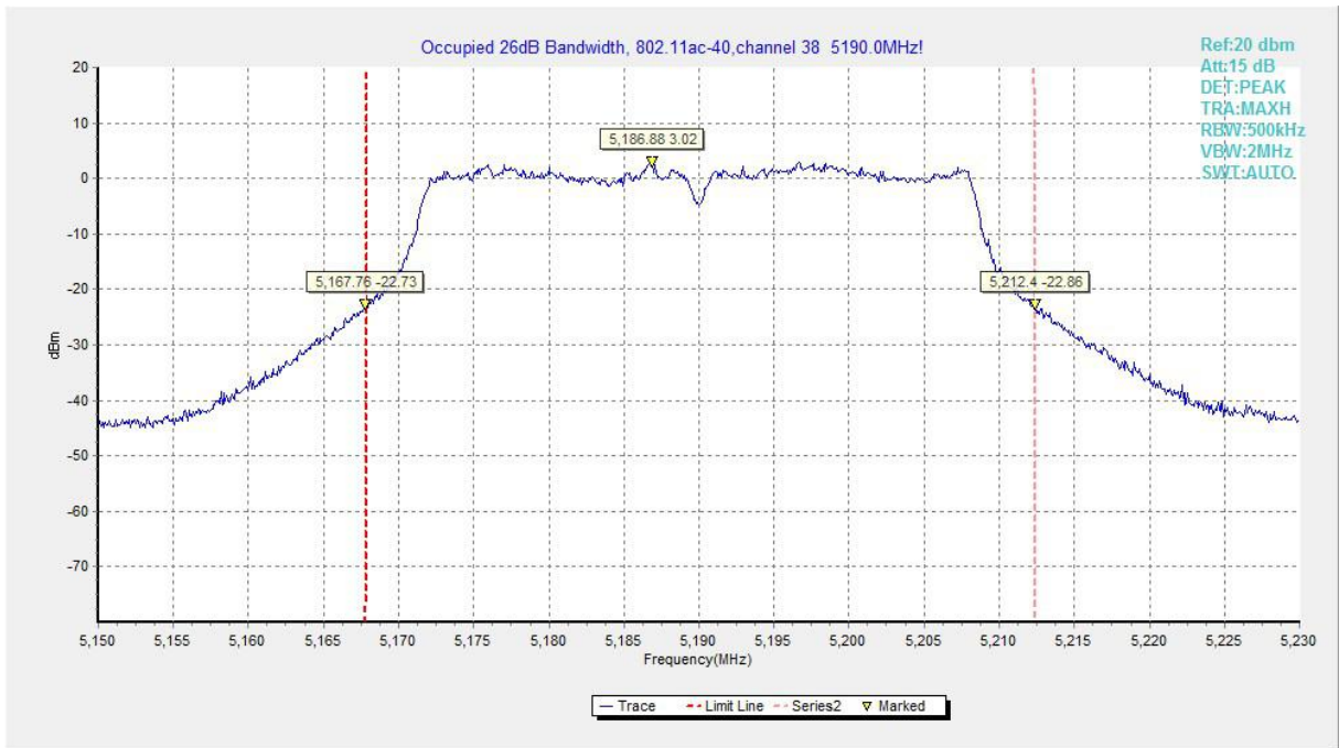
Fig.117 Occupied 26dB Bandwidth (802.11ac-HT40, 5190MHz)
