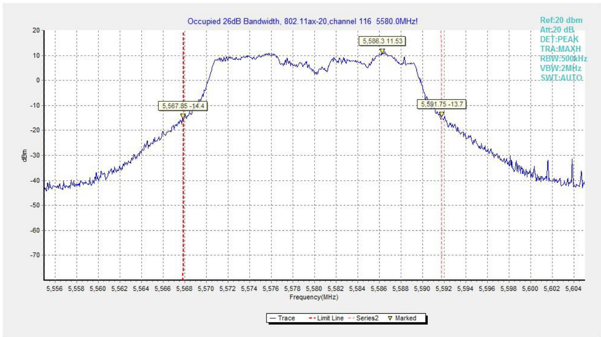
Fig.135 Occupied 26dB Bandwidth (802.11ax-HE20, 5580MHz)
