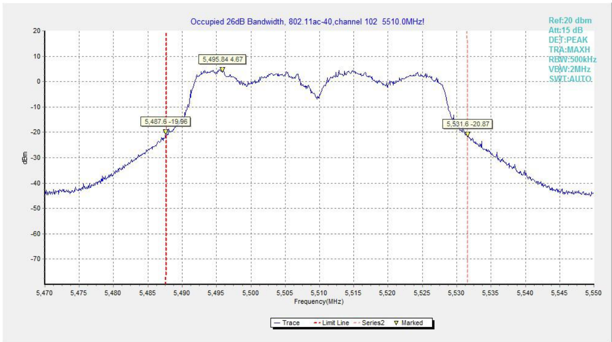
Fig.121 Occupied 26dB Bandwidth (802.11ac-HT40, 5510MHz)
