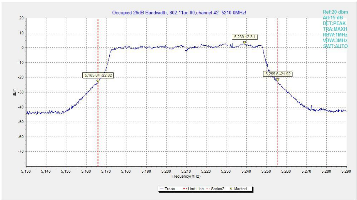
Fig.75 Occupied 26dB Bandwidth (802. 11ac-HT80, 5210MHz)
