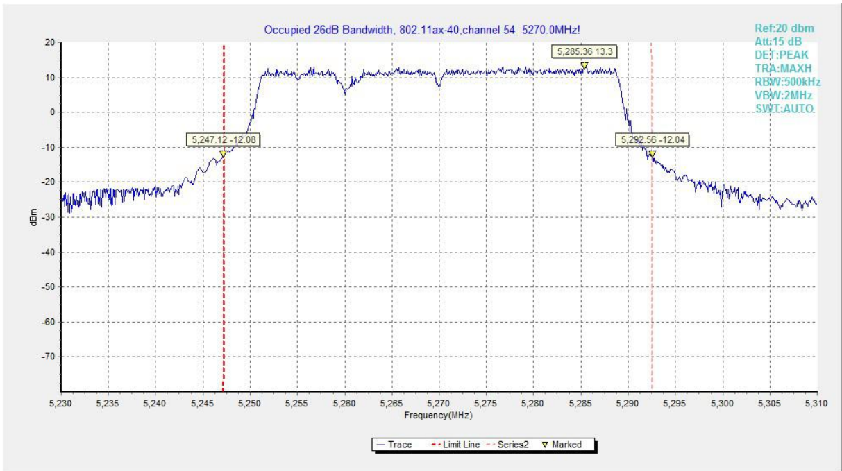
Fig.41 Occupied 26dB Bandwidth (802.11ax-HE40, 5270MHz)
