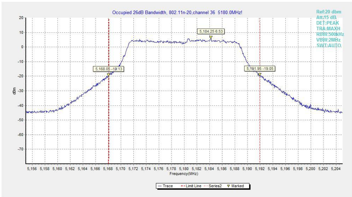
Fig.59 Occupied 26dB Bandwidth (802.11n-HT20, 5180MHz)
