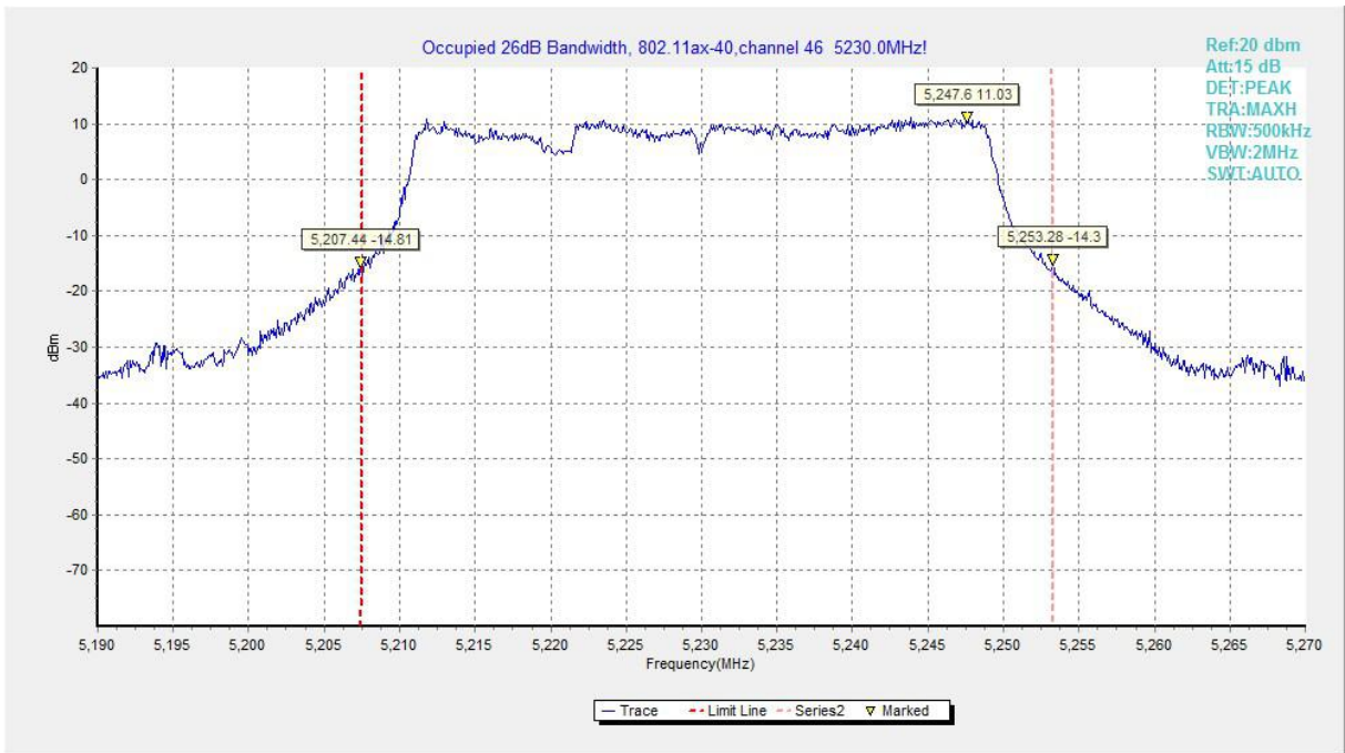
Fig.89 Occupied 26dB Bandwidth (802.11ax-HE40, 5230MHz)
