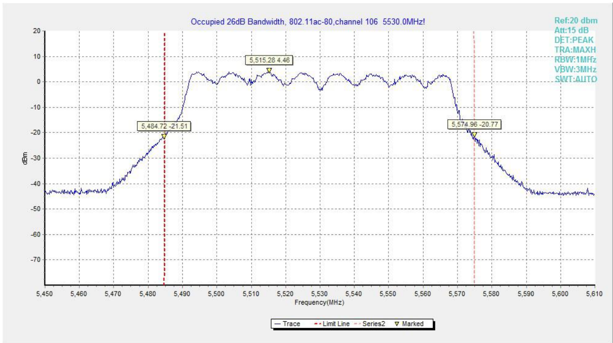
Fig.77 Occupied 26dB Bandwidth (802. 11ac-HT80, 5530MHz)
