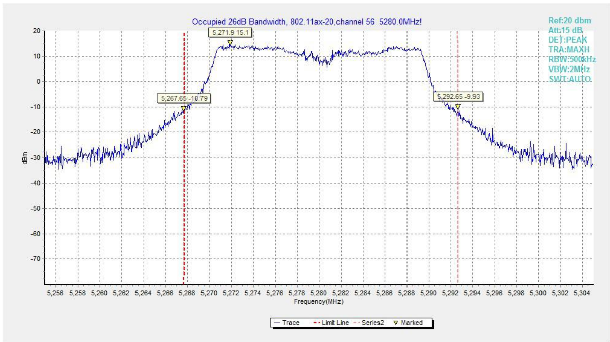
Fig.83 Occupied 26dB Bandwidth (802.11ax-HE20, 5280MHz)
