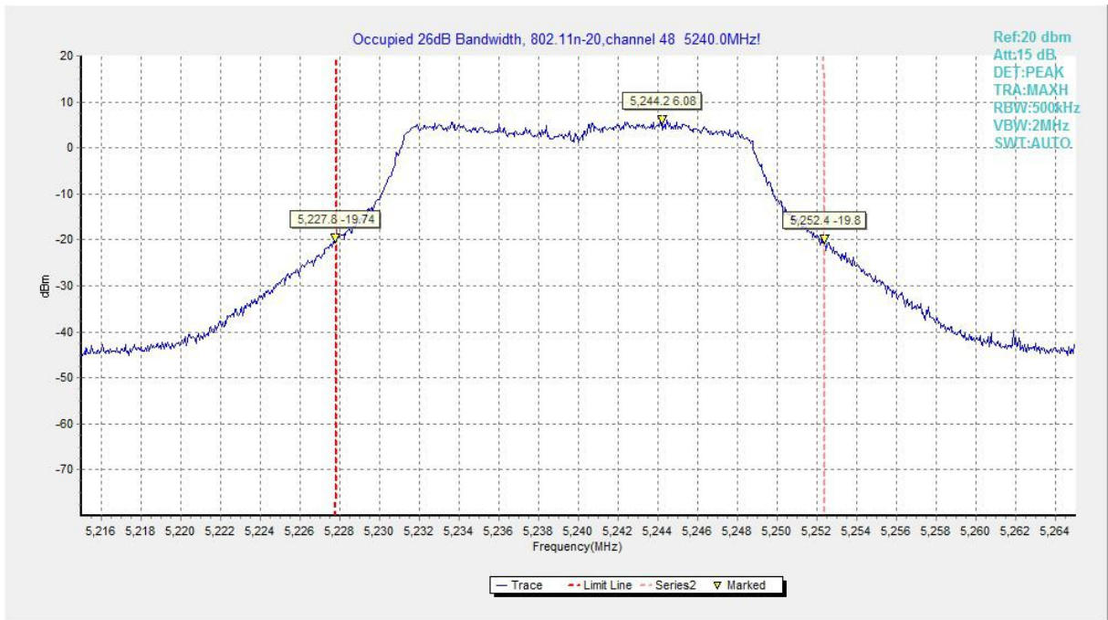
Fig.61 Occupied 26dB Bandwidth (802.11n-HT20, 5240MHz)
