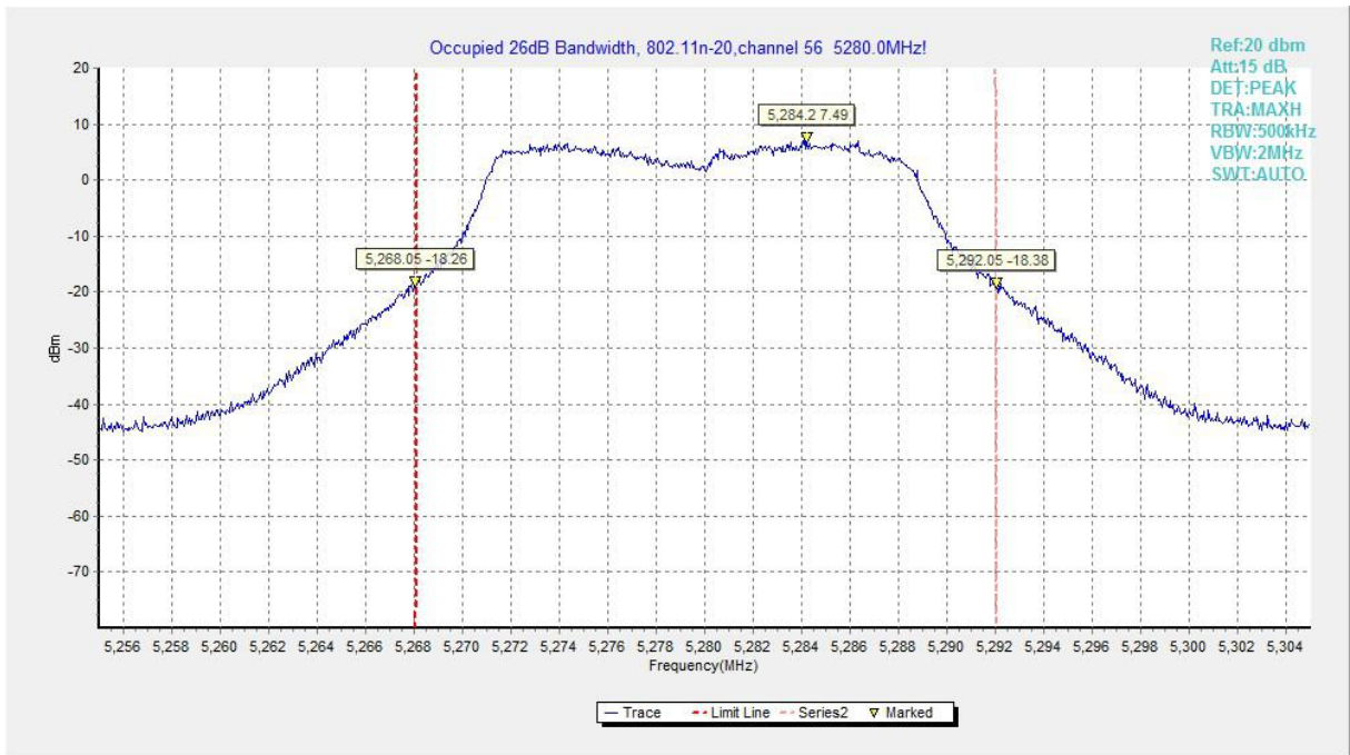
Fig.63 Occupied 26dB Bandwidth (802.11n-HT20, 5280MHz)
