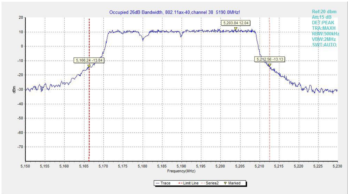
Fig.39 Occupied 26dB Bandwidth (802.11ax-HE40, 5190MHz)
