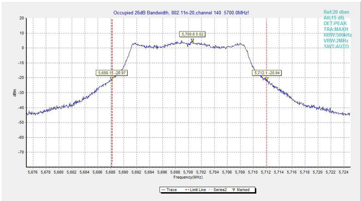
Fig.67 Occupied 26dB Bandwidth (802. 11n-HT20, 5700MHz)
