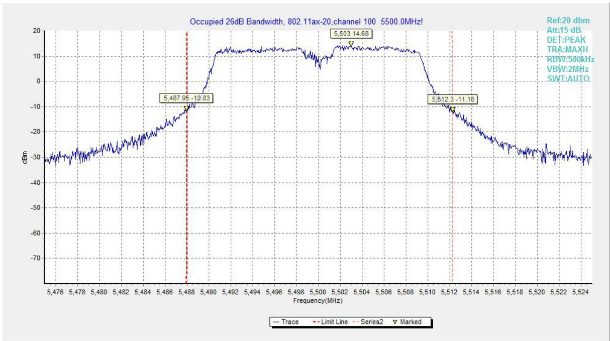
Fig.85 Occupied 26dB Bandwidth (802.11ax-HE20, 5500MHz)
