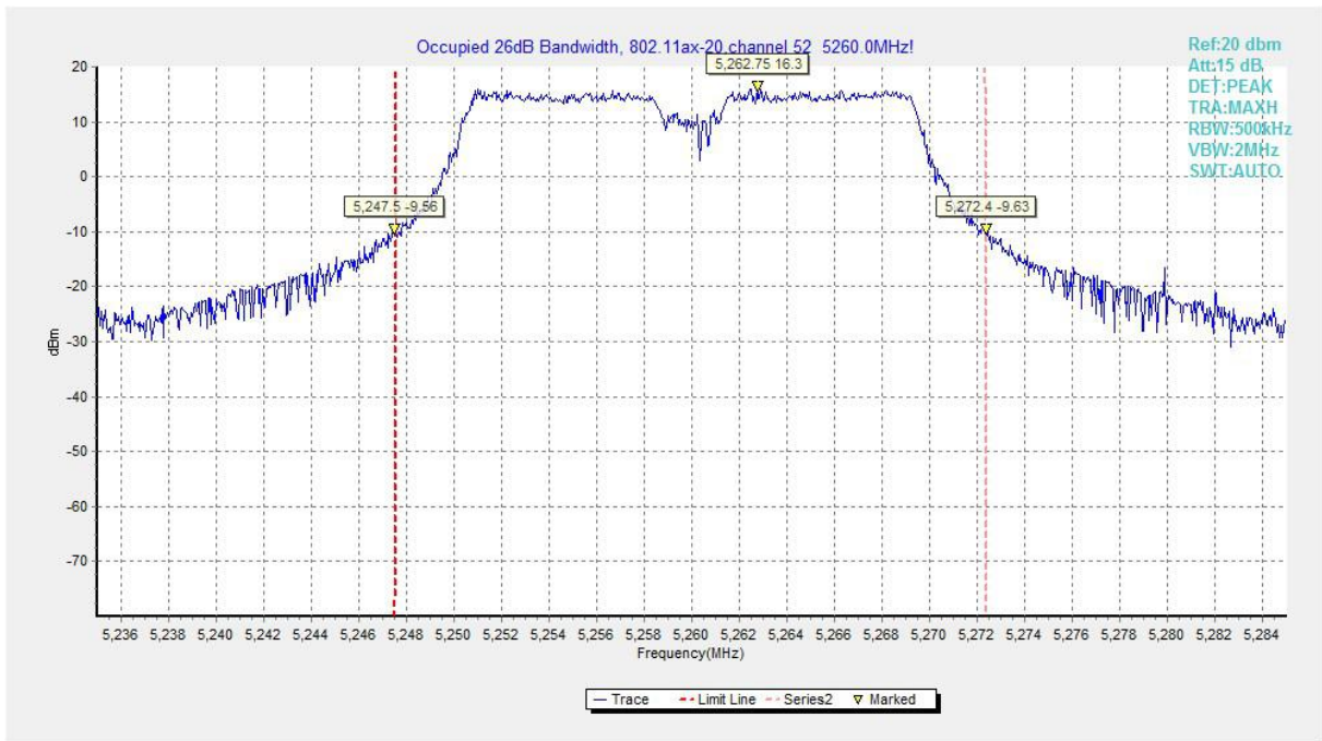
Fig.33 Occupied 26dB Bandwidth (802.11ax-HE20, 5260MHz)
