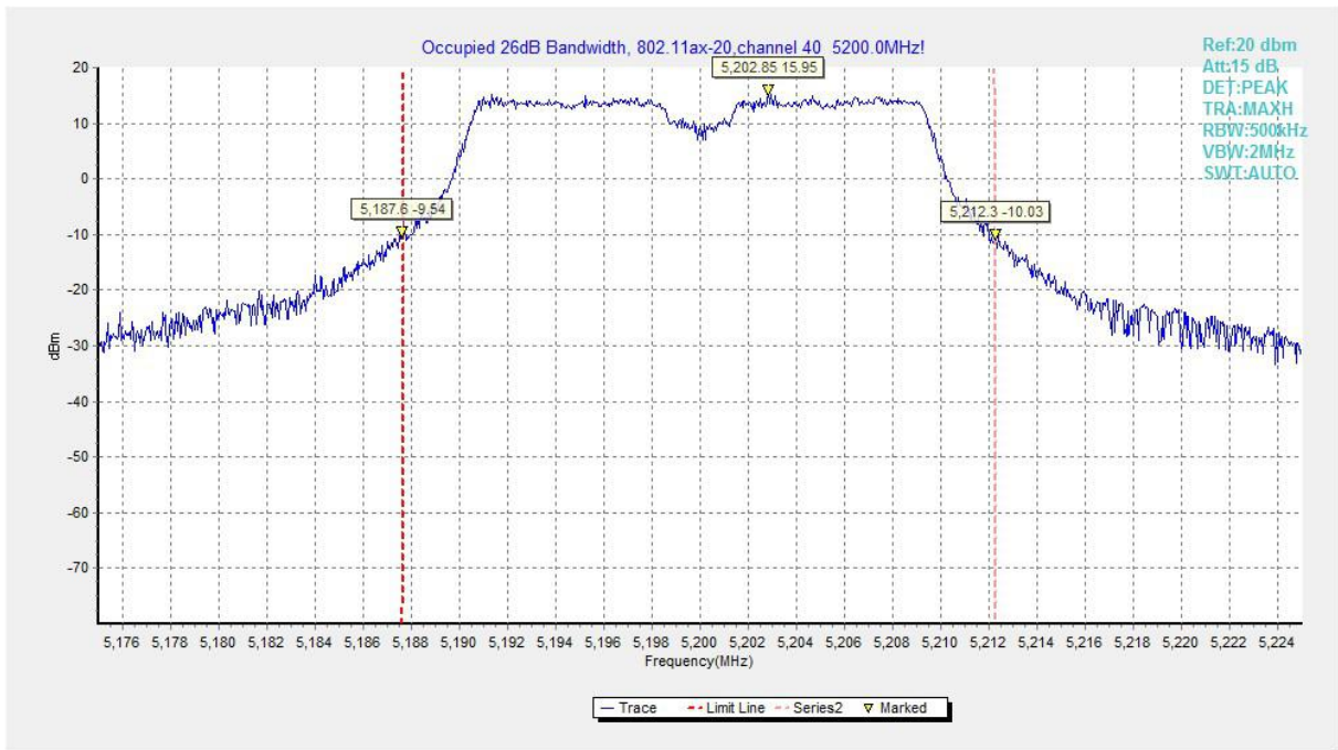
Fig.31 Occupied 26dB Bandwidth (802.11ax-HE20, 5200MHz)
