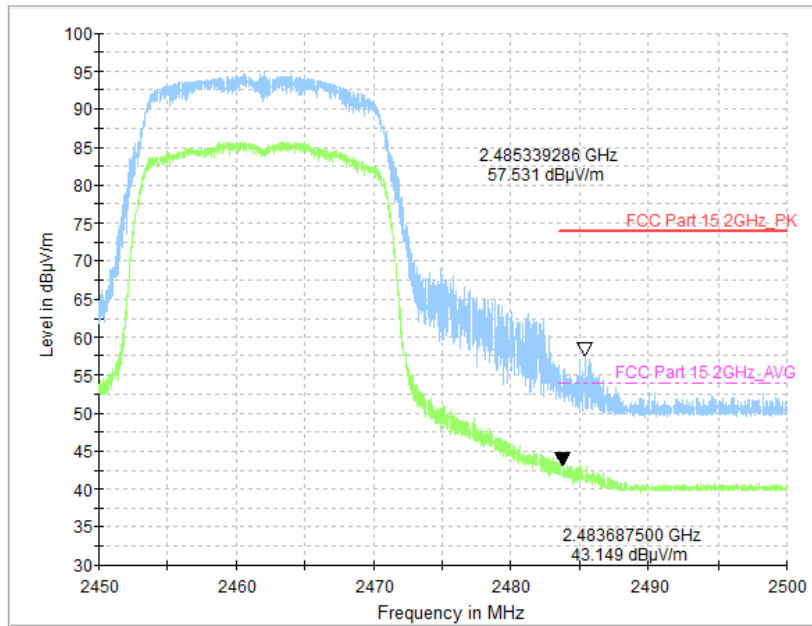
Fig.66 Radiated Restricted Band (802.11n-HT20, CH11, 2.45GHz~2.5GHz)
