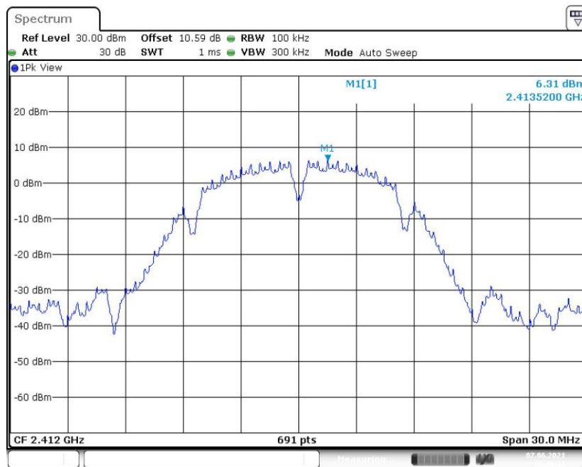
Fig.25 Conducted Spurious Emission (Center Frequency, 802.11b, CH1)
