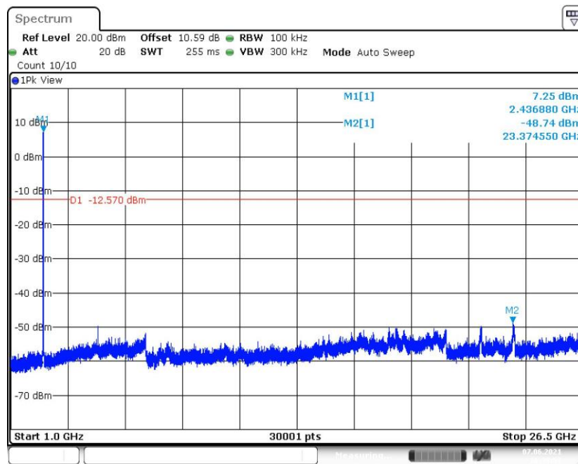
Fig.30 Conducted Spurious Emission (1GHz-26.5GHz, 802.11b, CH6)
