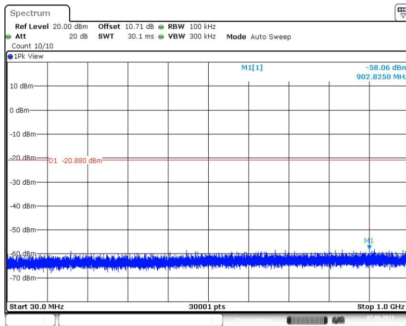
Fig.50 Conducted Spurious Emission (30MHz -1GHz, 802.11n-HT20, CH11)
