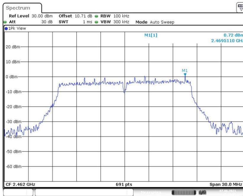
Fig.40 Conducted Spurious Emission (Center Frequency, 802.11g, CH11)
