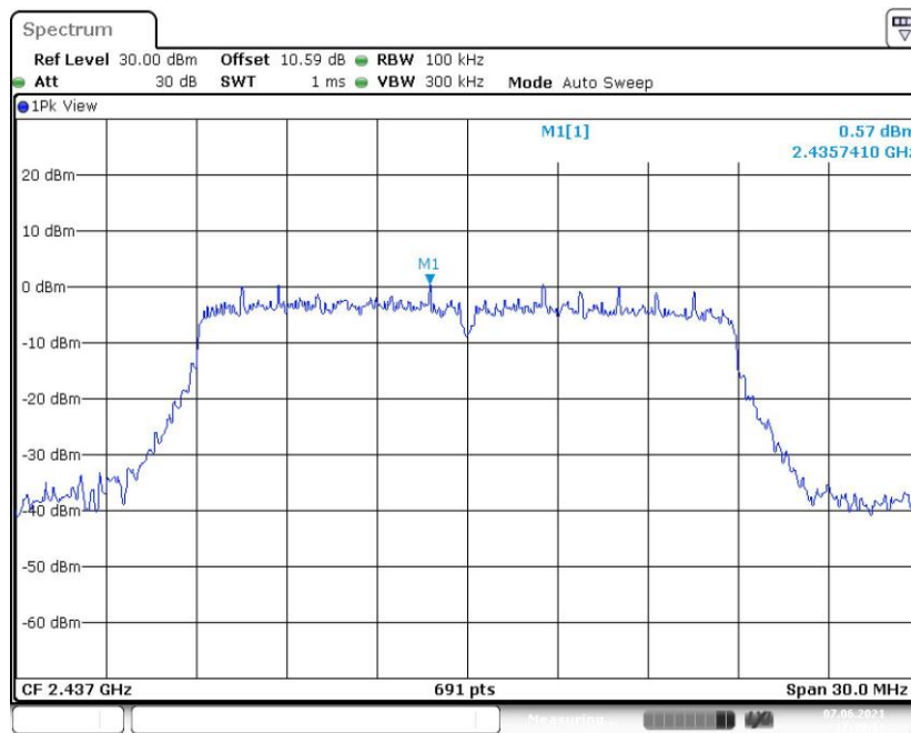
Fig.46 Conducted Spurious Emission (Center Frequency, 802.11n-HT20, CH6)
