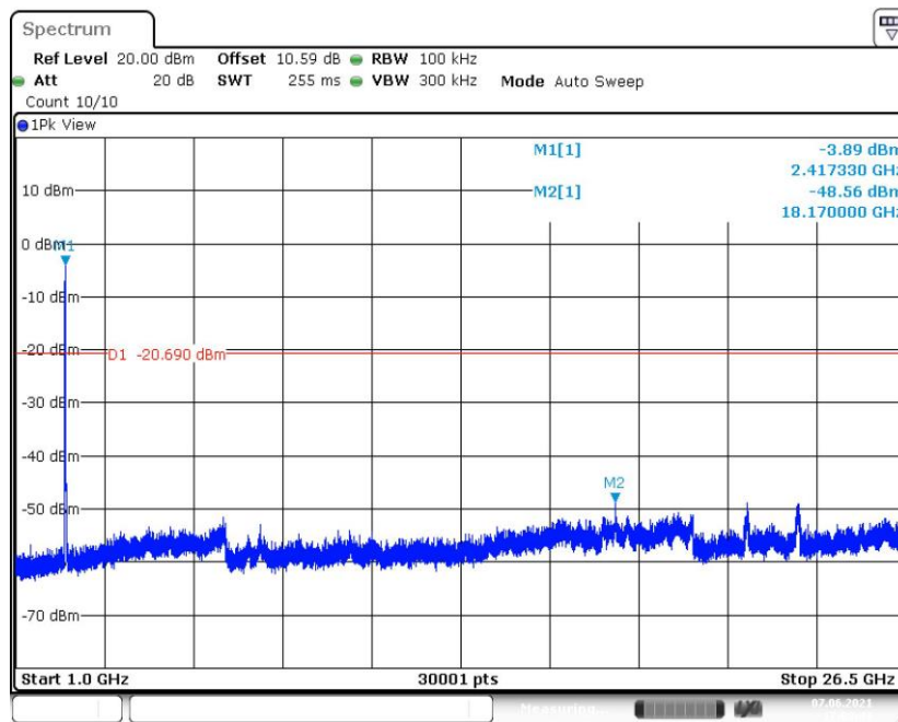
Fig.36 Conducted Spurious Emission (1GHz-26.5GHz, 802.11g, CH1)
