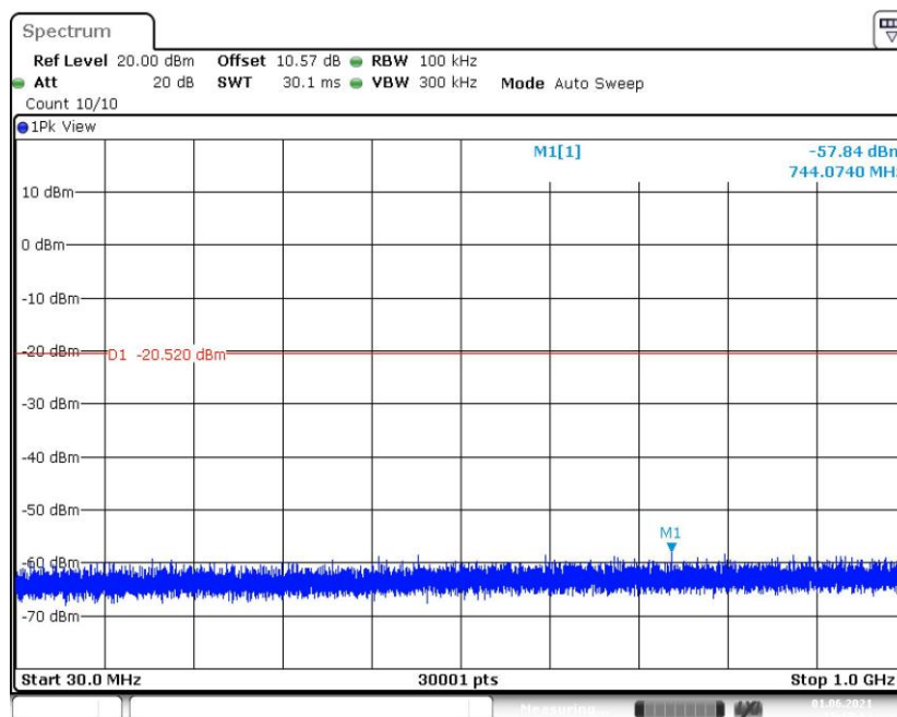
Fig.13 Conducted Spurious Emission (CH19, 30MHz -1GHz), LE 1M
