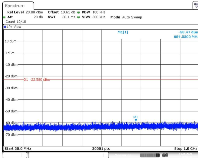
Fig.10 Conducted Spurious Emission (CH0, 30MHz -1GHz), LE 1M
