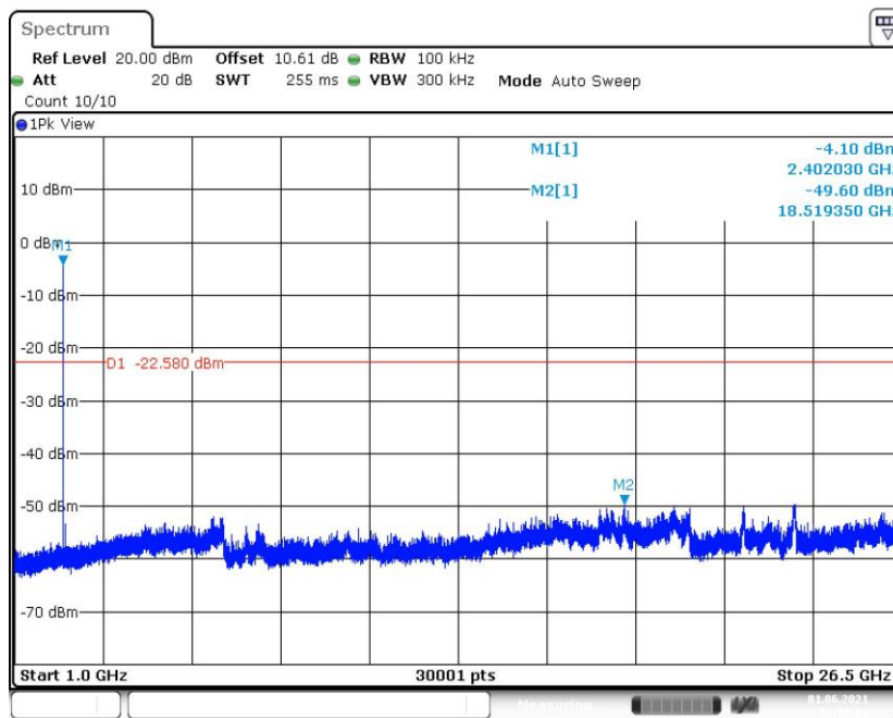
Fig.11 Conducted Spurious Emission (CH0, 1GHz-26.5GHz), LE 1M
