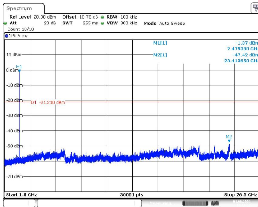
Fig.17 Conducted Spurious Emission (CH39, 1GHz-26.5GHz), LE 1M
