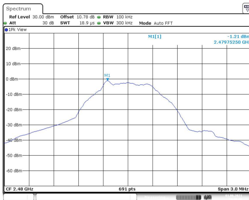
Fig.15 Conducted Spurious Emission (CH39, Center Frequency), LE 1M
