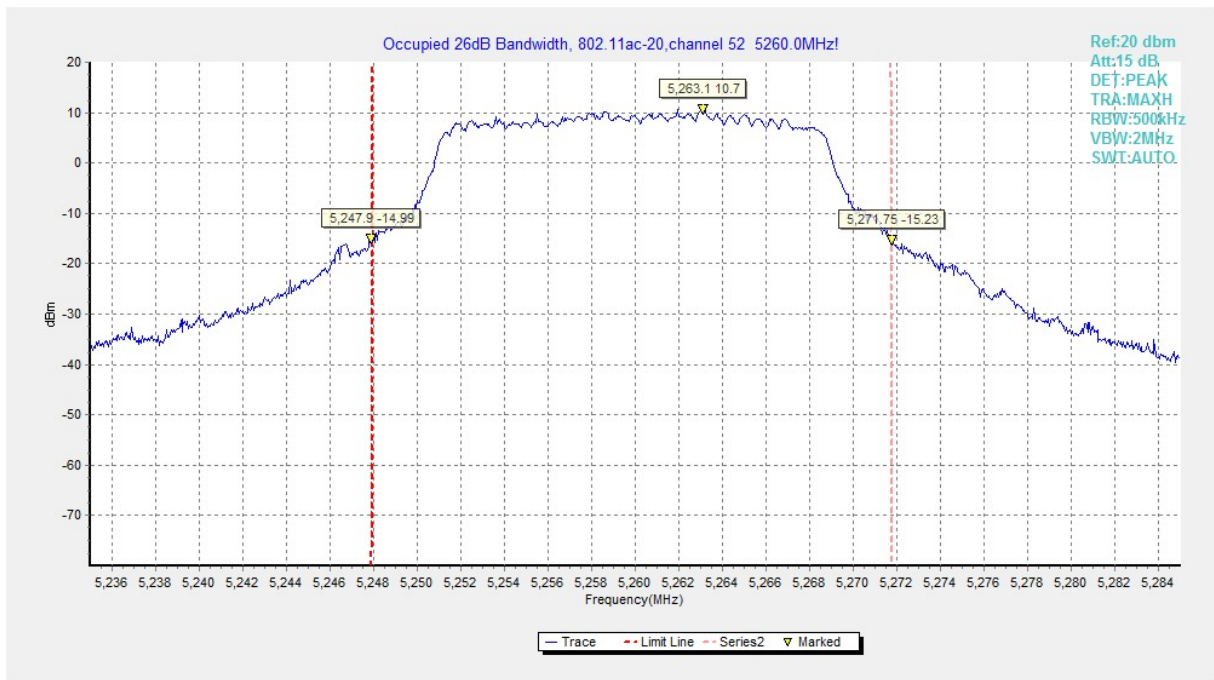
Fig.13 Occupied 26dB Bandwidth (802.11ac-HT20, 5260MHz)
