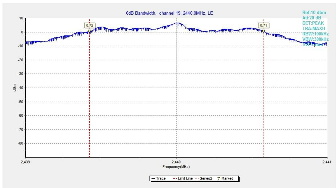
Fig.27. 6dB Bandwidth: GFSK, 2440 MHz
