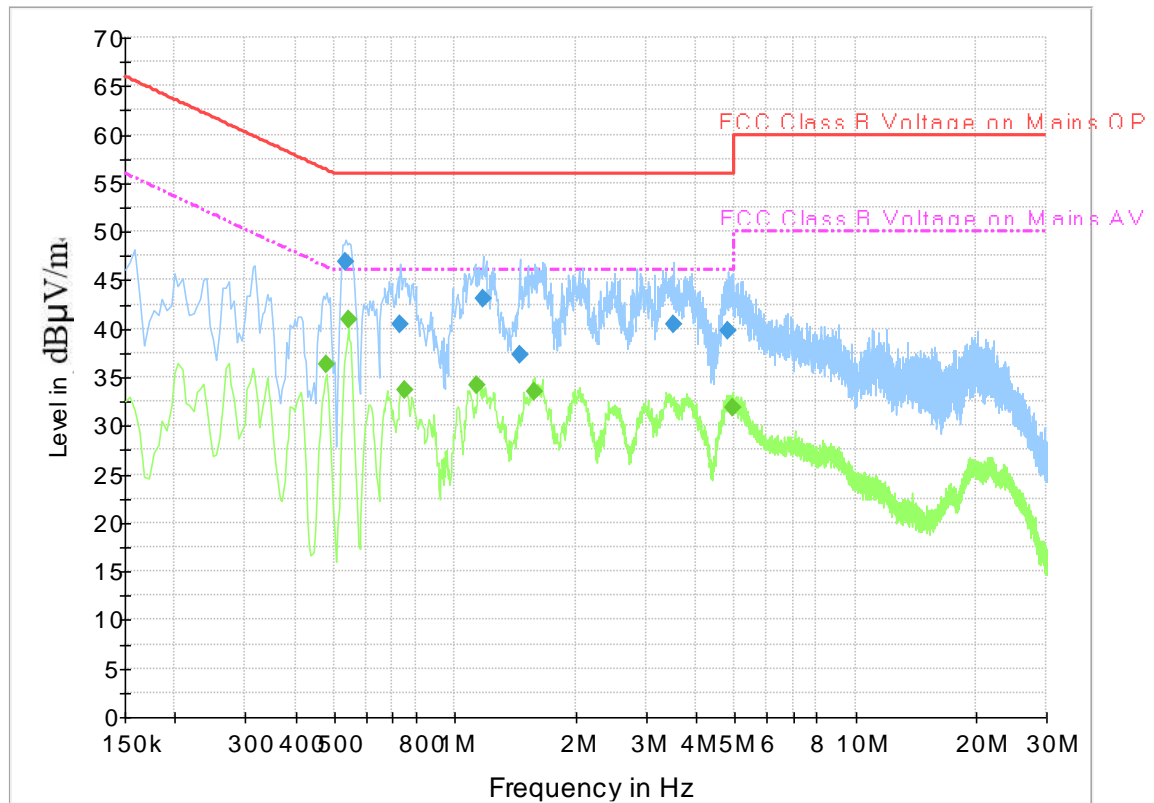
Fig.B.9.1 AC Powerline Conducted Emission- Bluetooth
