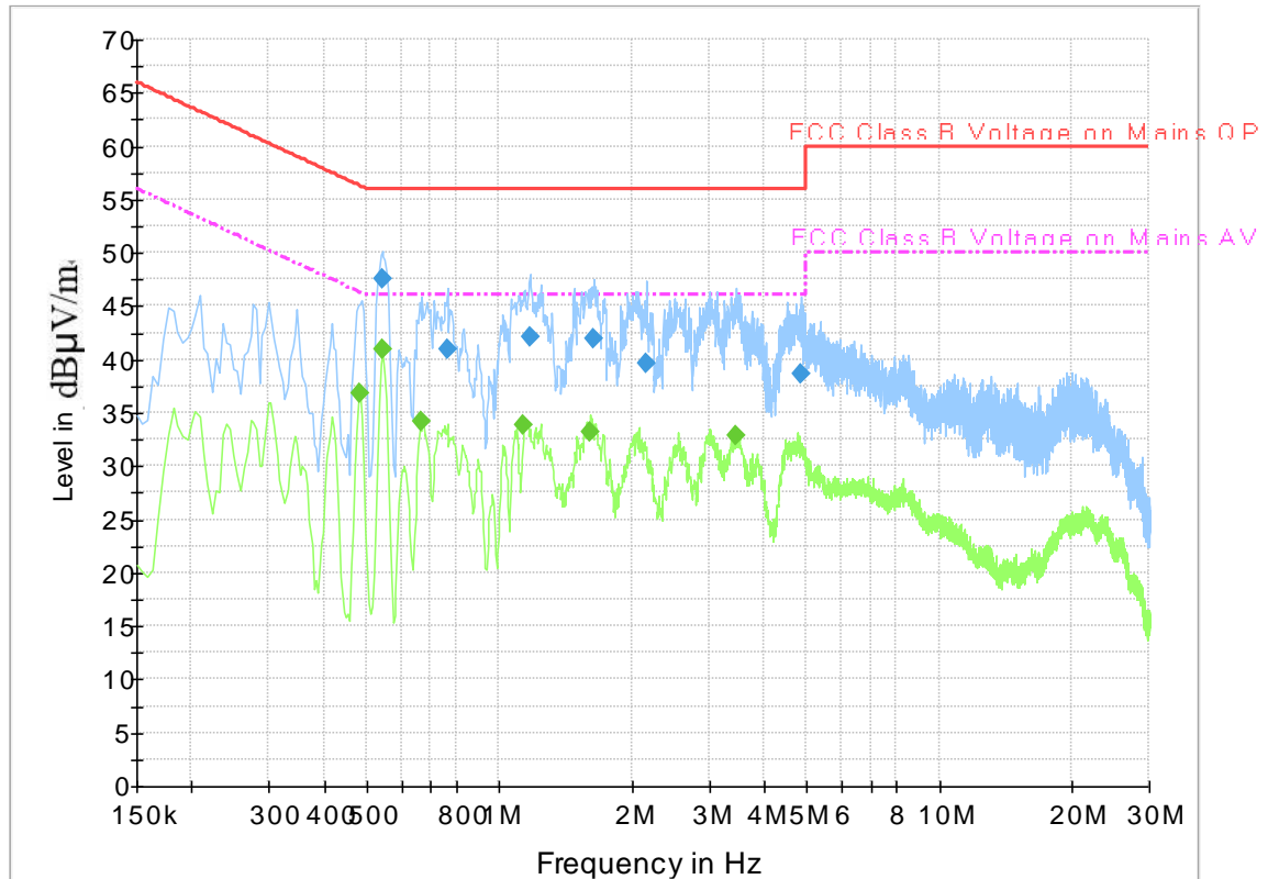
Fig.B.9.2 AC Powerline Conducted Emission-Idle
