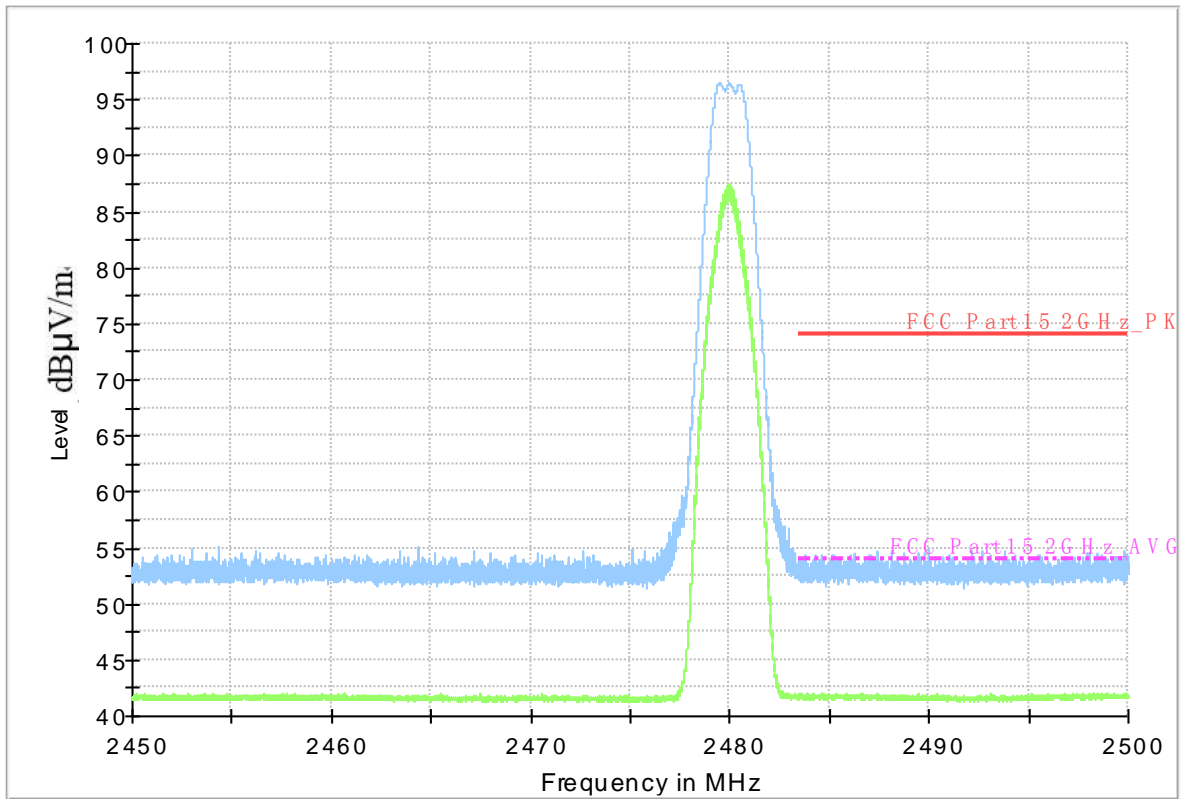
Fig.10. Frequency Band Edges: GFSK, 2480 MHz, 2.45 GHz - 2.50GHz
