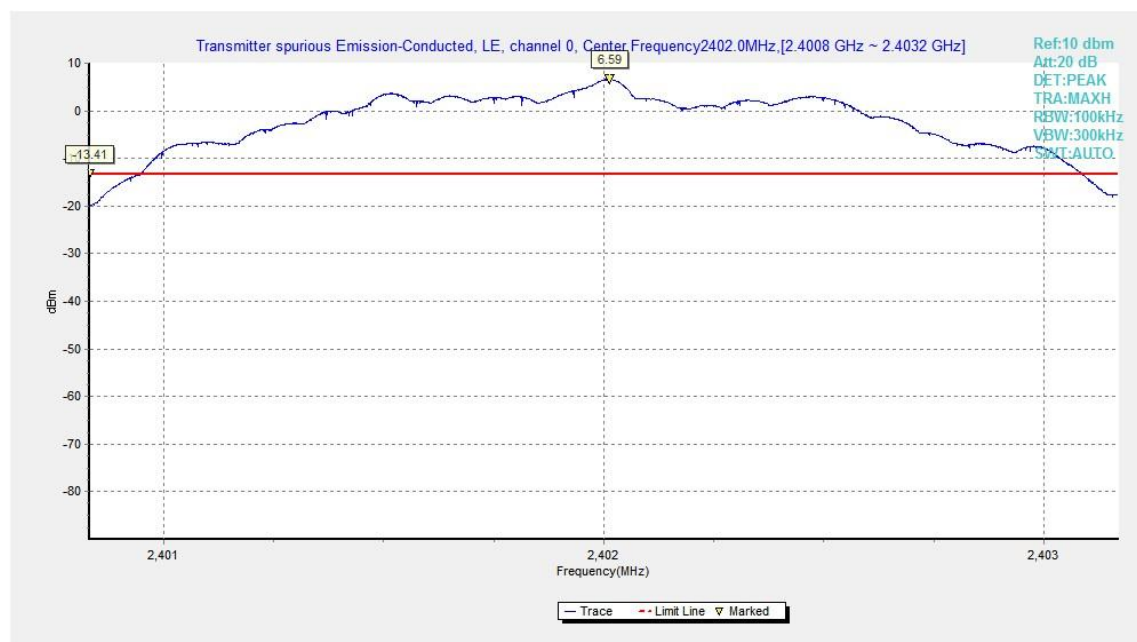
Fig.11. Transmitter Spurious Emission - Conducted: GFSK,2402MHz
