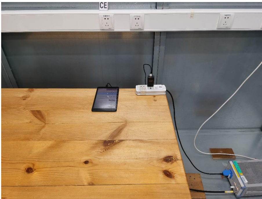
18. Conducted Emission (Part 15B, Camera/Video Player)
