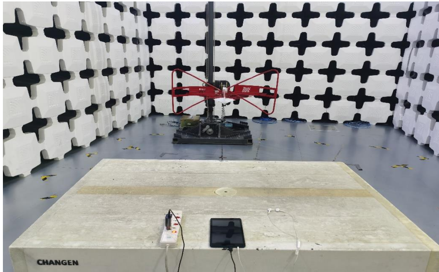
9. Radiated Emissions (Part 15B, FM receiver 30MHz-1GHz)
