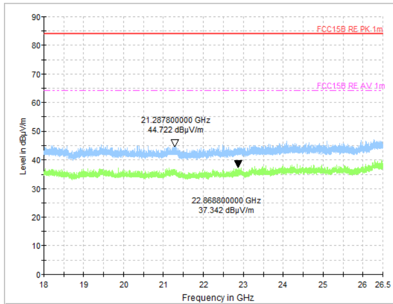
Fig.49 Radiated Spurious Emission (Ch19, 18 GHz - 26.5 GHz), 2M
