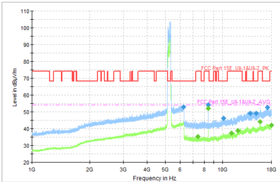
Fig. 32 Transmitter Spurious Emission (802.11a, CH48 5240MHz)
