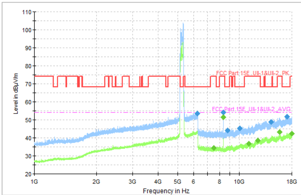
Fig. 40 Transmitter Spurious Emission (802.11n-HT40, CH46 5230MHz)
