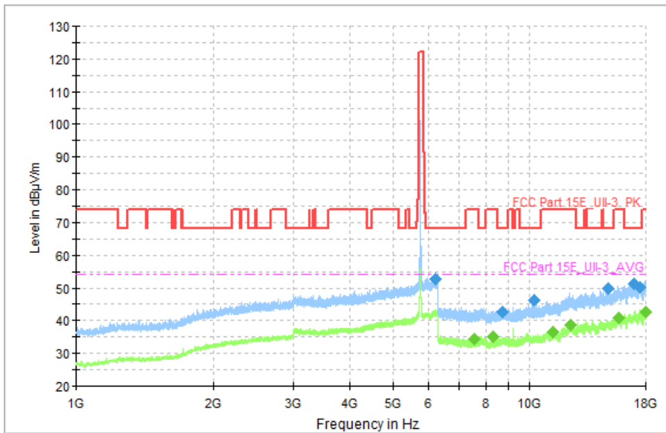
Fig. 36 Transmitter Spurious Emission (802. 11a, CH149 5745MHz)
