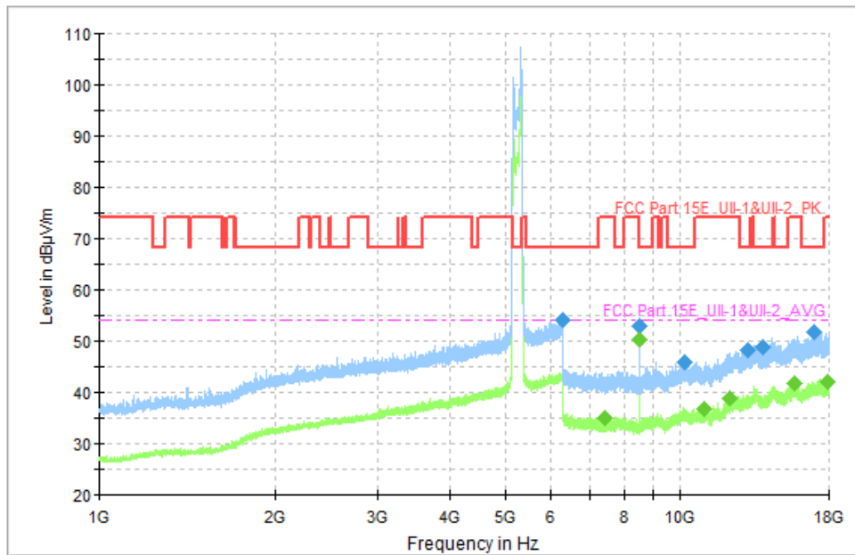
Fig. 42 Transmitter Spurious Emission (802.11n-HT40, CH62 5310MHz)
