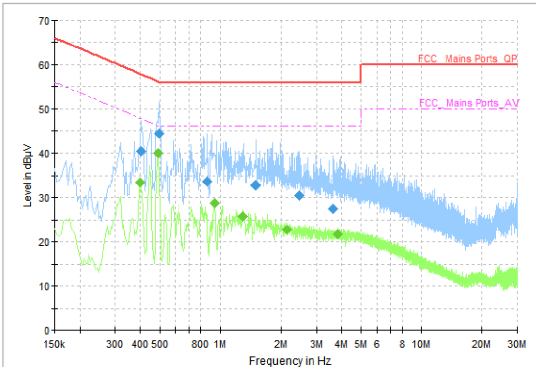
Fig. 53 AC Power line Conducted Emission (Idle)
