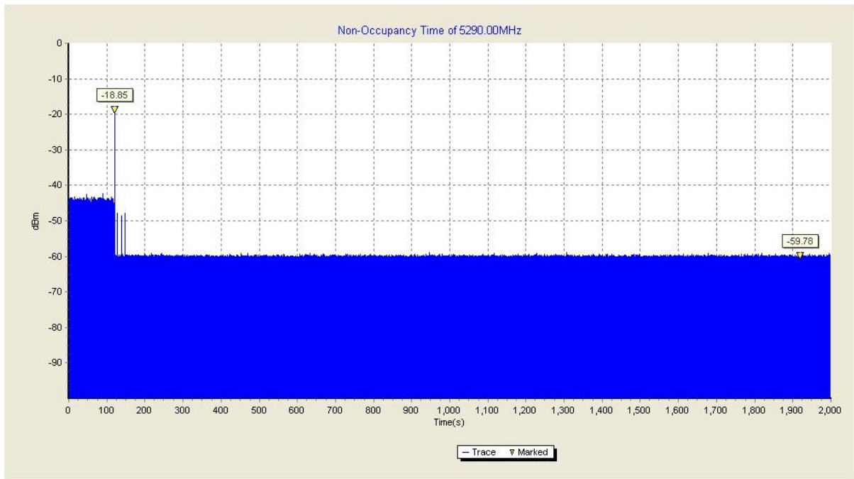
Fig.6 Non-Occupancy Period (HT80 Frequency Band: 5250MHz ~ 5350MHz)
