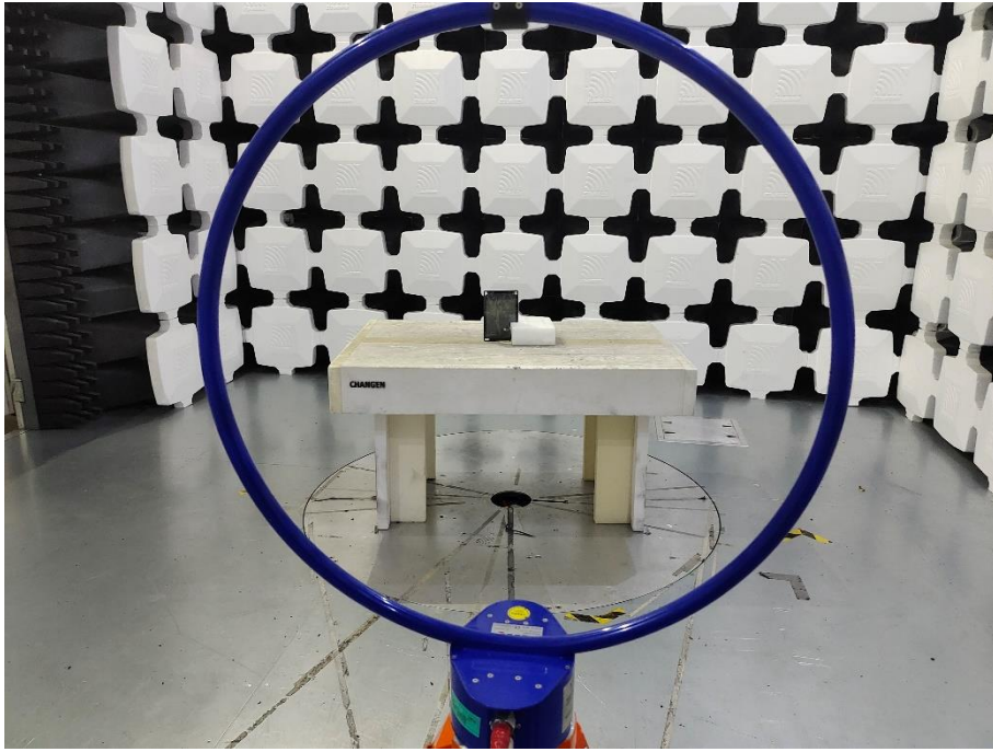
13. Radiated Emissions (Part 15C/15E, 9kHz-30MHz)
