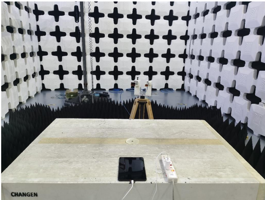
8. Radiated Emissions (Part 15B, Camera/Video Player,26.5GHz-30GHz)
