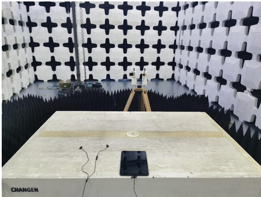
12. Radiated Emissions (Part 15B, FM receiver 26.5GHz-30GHz)
