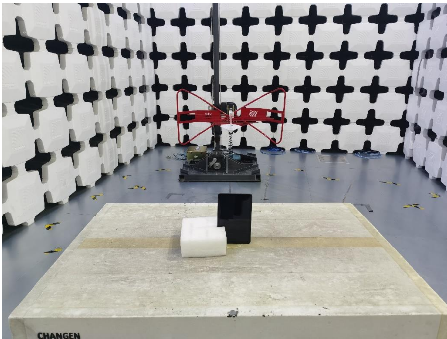
14. Radiated Emissions (Part 15C/15E, 30MHz-1GHz)
