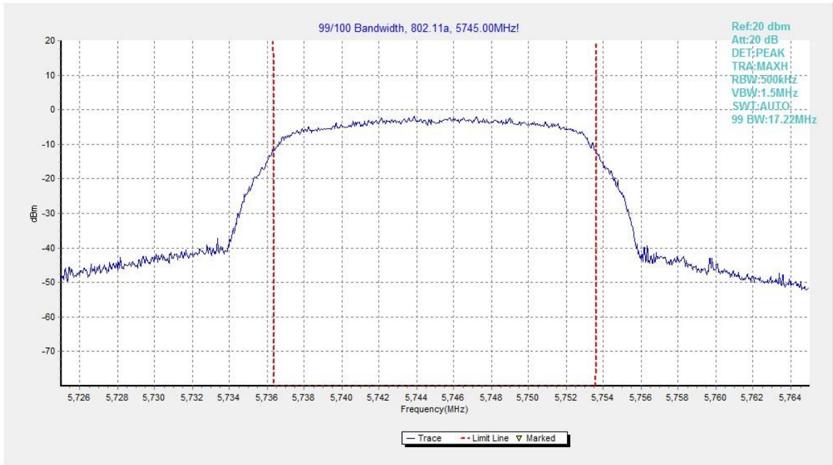
Fig. 25 99% Occupied Bandwidth (802.11a, 5745MHz)
