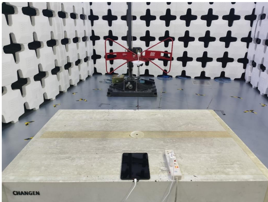
6. Radiated Emissions (Part 15B, Camera/Video Player/GSM receiver/ WCDMA receiver/LTE receiver,1GHz-18GHz)
