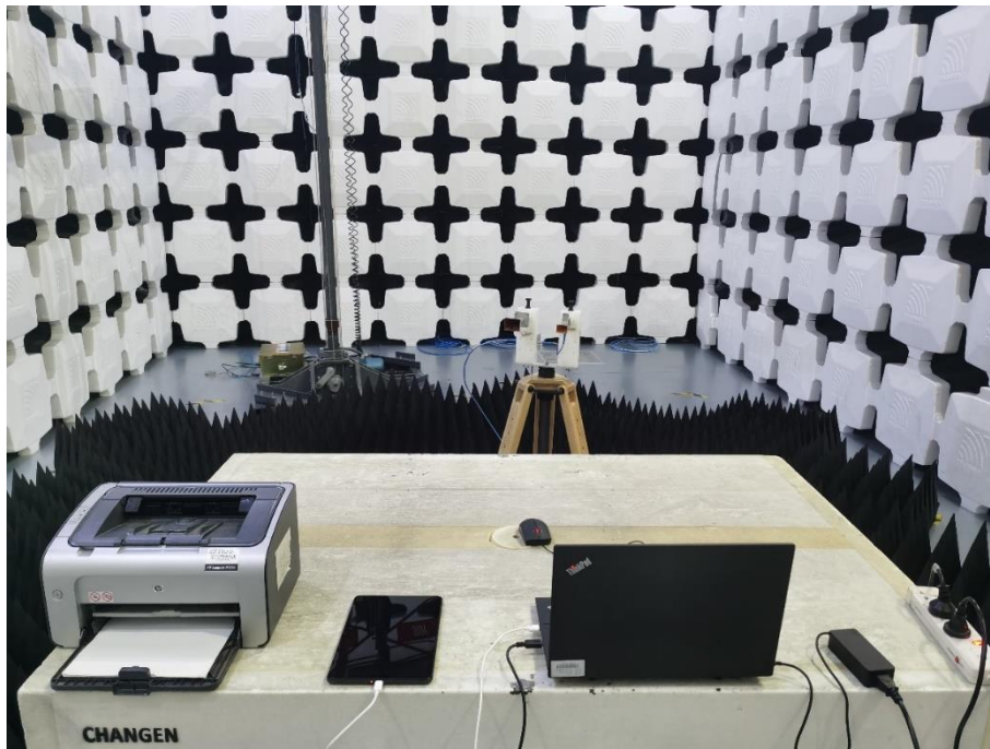
4. Radiated Emissions (Part 15B Data Transfer ,26.5GHz-30GHz)
