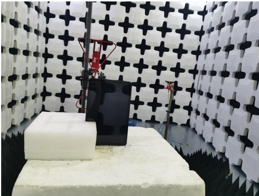
18. Radiated Emissions (Part 22/24/27/90,30MHz-18GHz)
