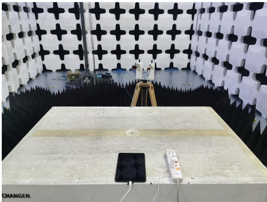
8. Radiated Emissions (Part 15B, Camera/Video Player/GSM receiver/ WCDMA receiver/LTE receiver,26.5GHz-30GHz)
