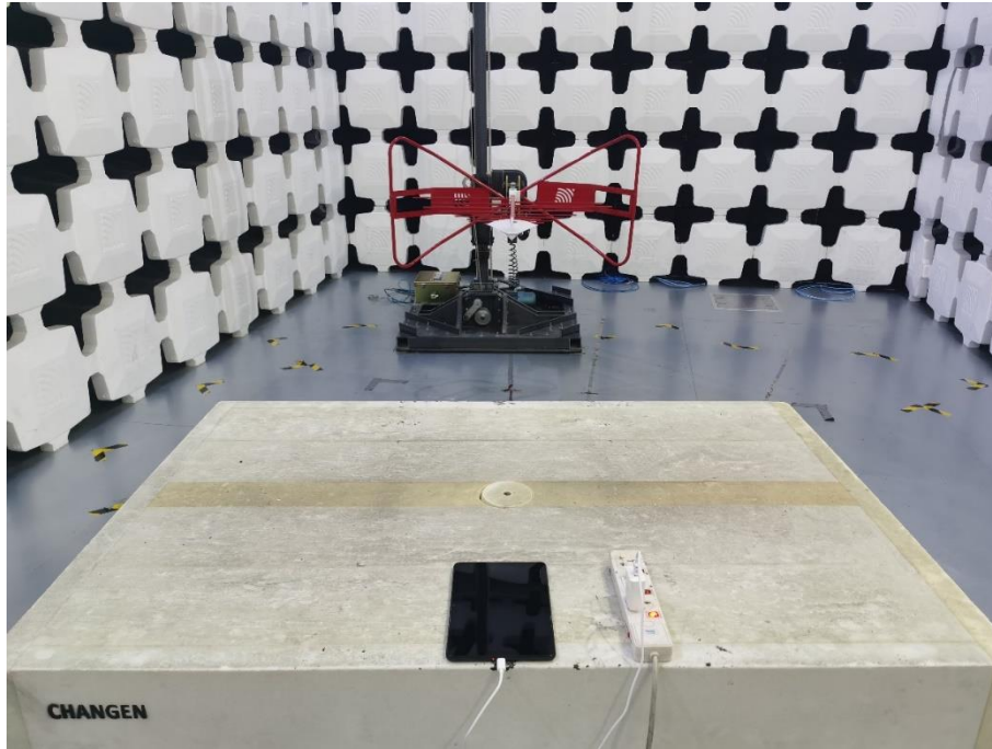
5. Radiated Emissions (Part 15B, Camera/Video Player /GSM receiver/WCDMA receiver/LTE receiver,30MHz-1GHz)
