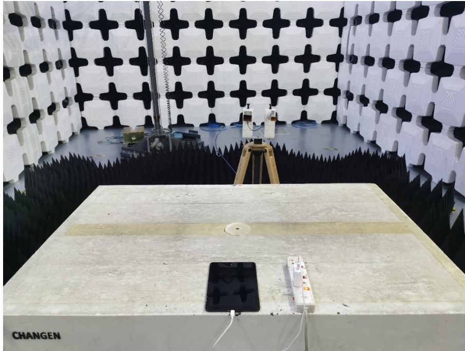
7. Radiated Emissions (Part 15B, Camera/Video Player/GSM receiver/ WCDMA receiver/LTE receiver,18GHz-26.5GHz)
