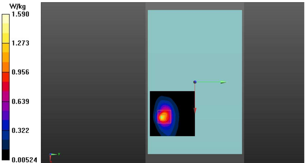
Fig.2 GSM 1900 Body
