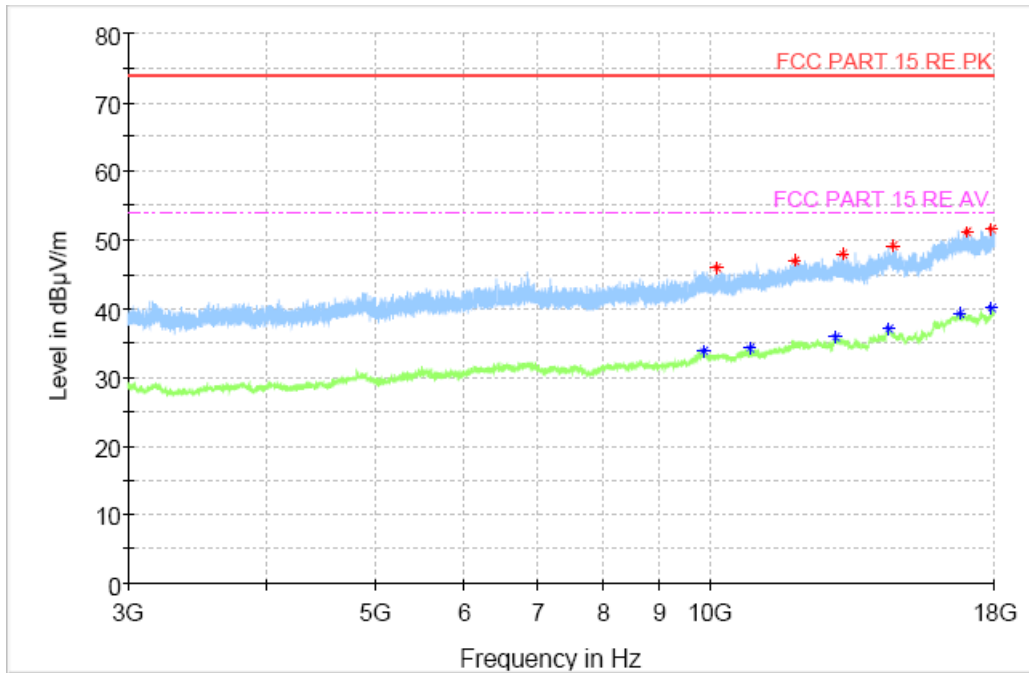
Fig.55 Radiated Spurious Emission (802.11n HT20, CH1, 3GHz-18GHz)
