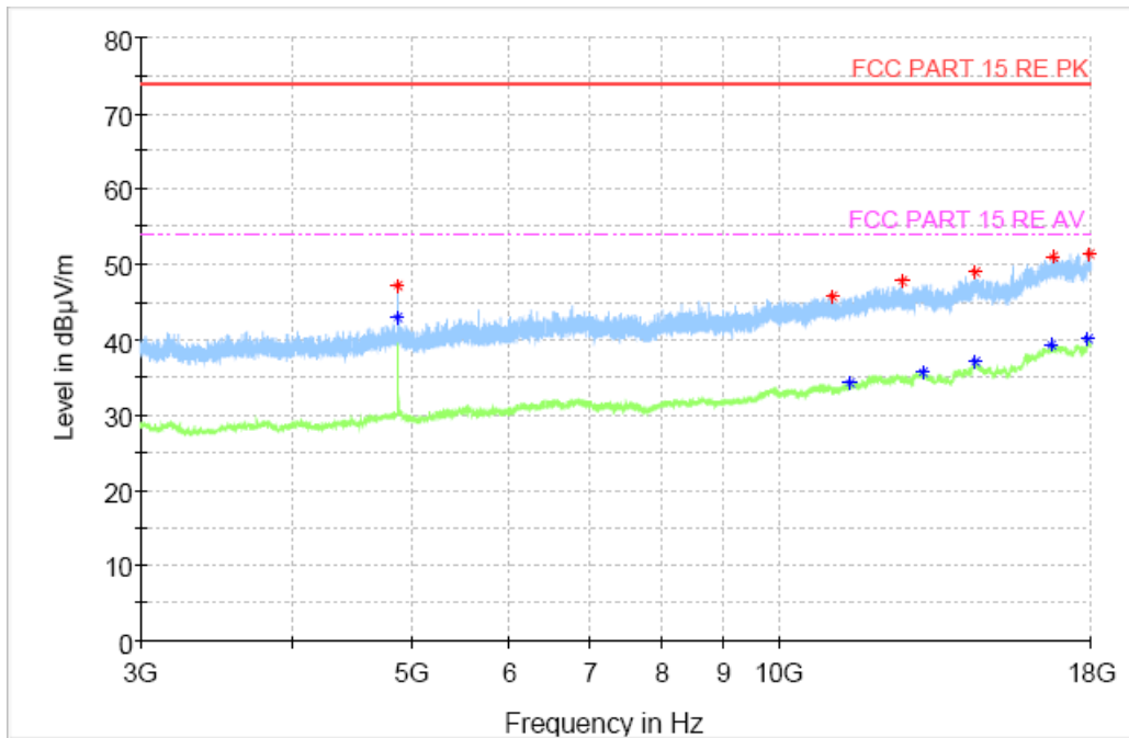
Fig.46 Radiated Spurious Emission (802.11b, CH6, 3GHz-18GHz)
