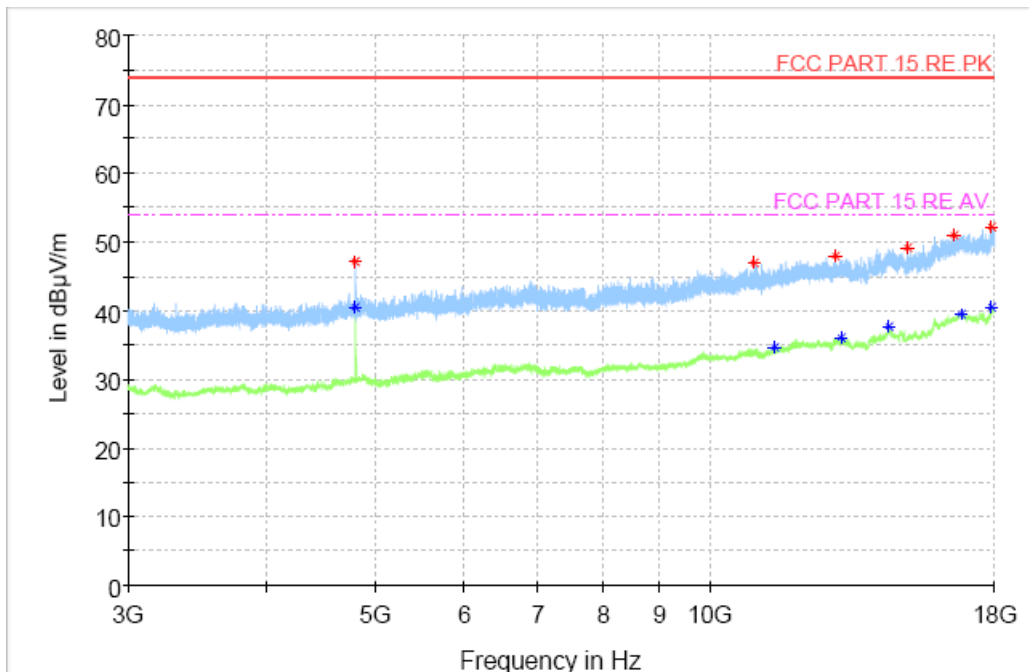
Fig. 47 Radiated Spurious Emission ( \pi/4 DQPSK, Ch0, 3GHz ~ 18GHz)
