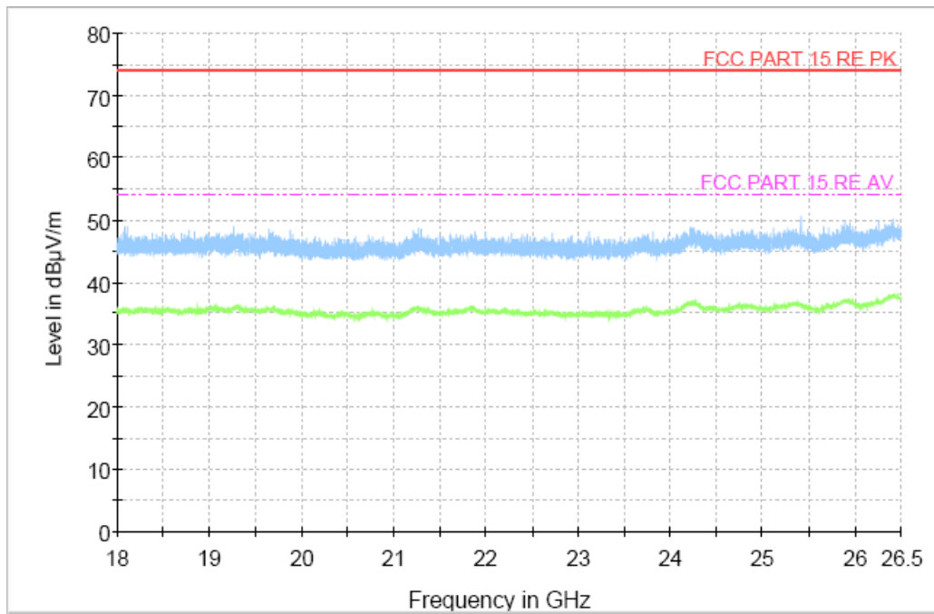
Fig. 60 Radiated Spurious Emission (All Channels, 18GHz ~ 26.5GHz)
