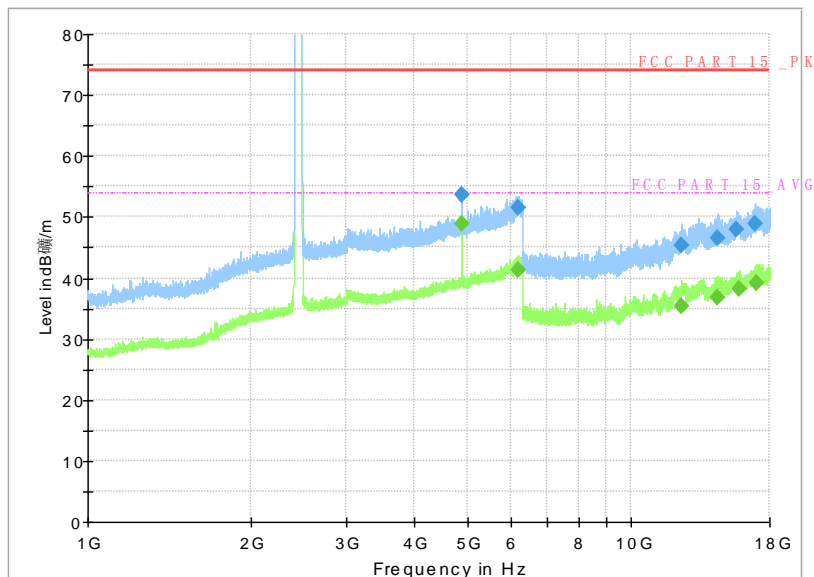
Fig.46 Radiated Spurious Emission (802.11b, CH6, 1GHz-18GHz)
