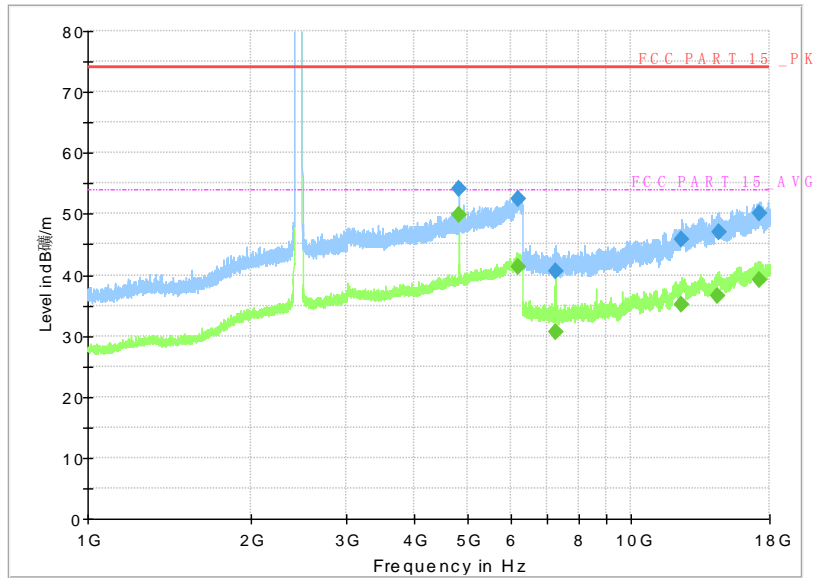
Fig.45 Radiated Spurious Emission (802.11b, CH1, 1GHz-18GHz)
