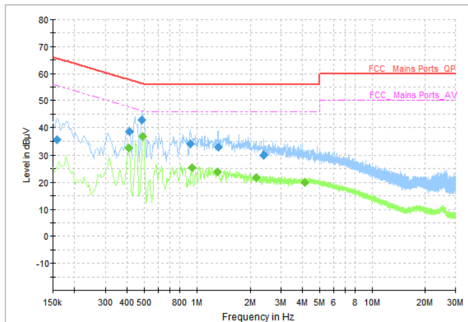
Fig.71 AC Power line Conducted Emission (Idle, AE4, 120V)
