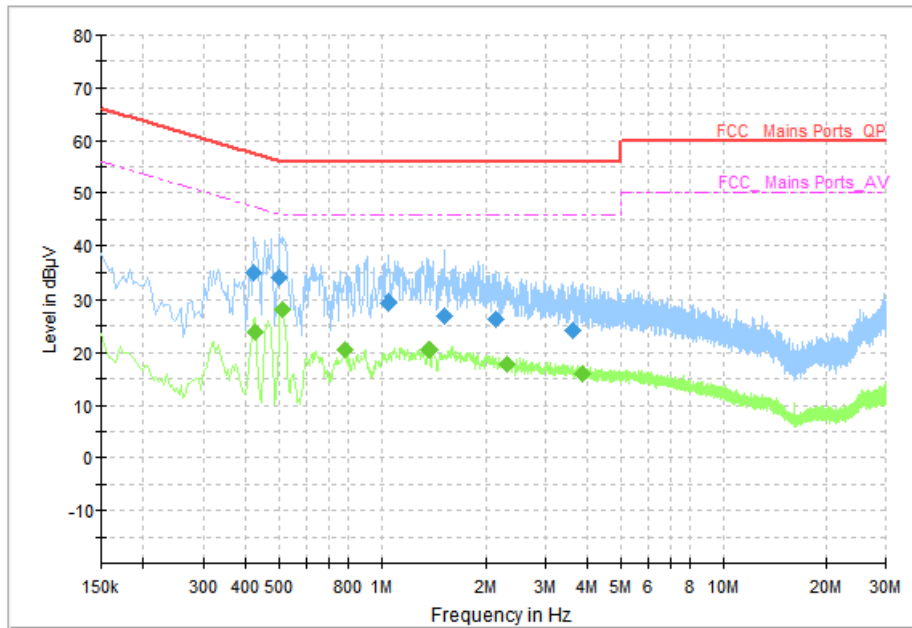
Fig.68 AC Power line Conducted Emission (Idle, AE3, 120V)
