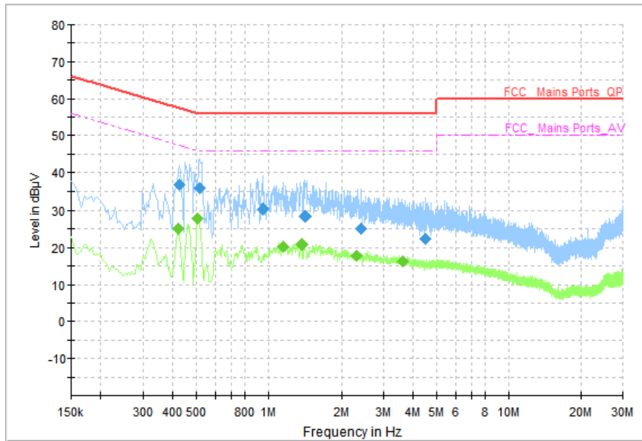
Fig.69 AC Power line Conducted Emission (Traffic, AE3, 120V)
