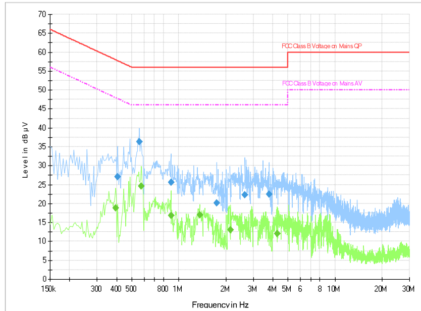
Fig.B.9.1 AC Powerline Conducted Emission- bluetooth
