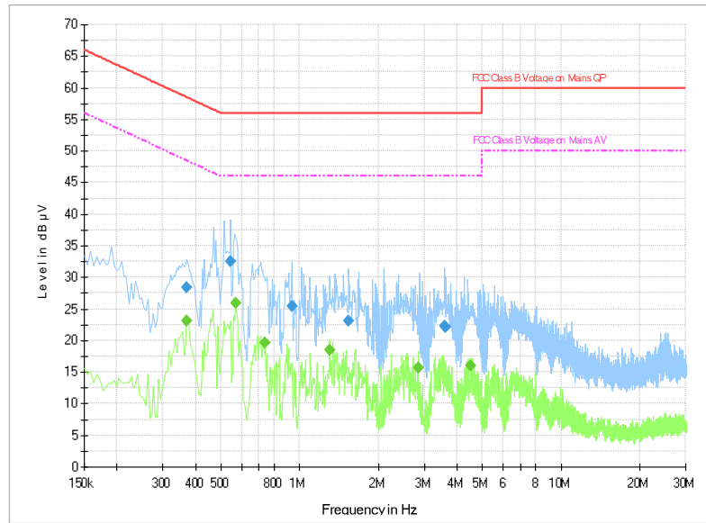
Fig.B.9.2 AC Powerline Conducted Emission-Idle
