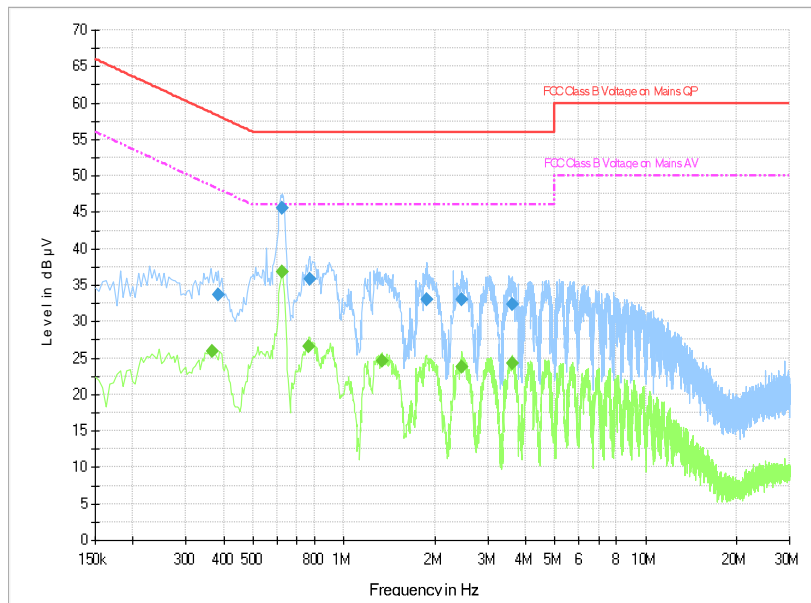
Fig.B.11.4 AC Powerline Conducted Emission-Idle
