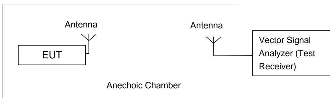
Fig.B.1.2.1: Test Setup Diagram for Radiated Measurements
