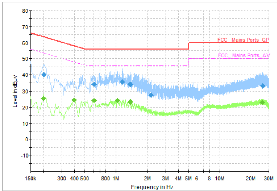
Fig.70 AC Power line Conducted Emission (Traffic, AE4, 120V)
