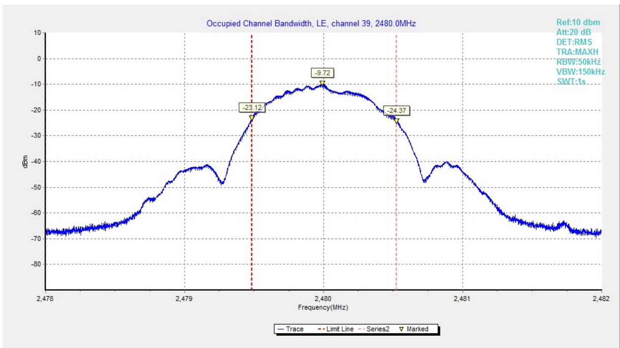
Fig.33 99% Occupied Bandwidth: GFSK, Channel 39, LE 1M
