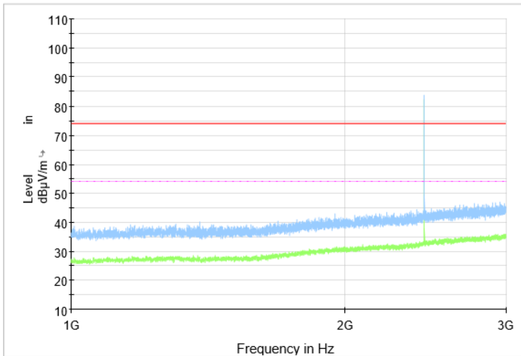
Fig.22 Radiated Spurious Emission (GFSK, Ch19, 1 GHz ~3 GHz), LE 1M
