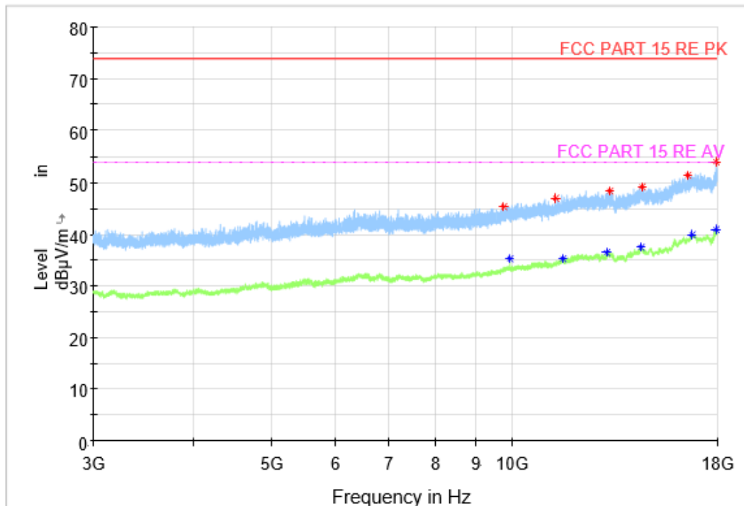
Fig.25 Radiated Spurious Emission (GFSK, Ch39, 3 GHz ~18 GHz), LE 1M
