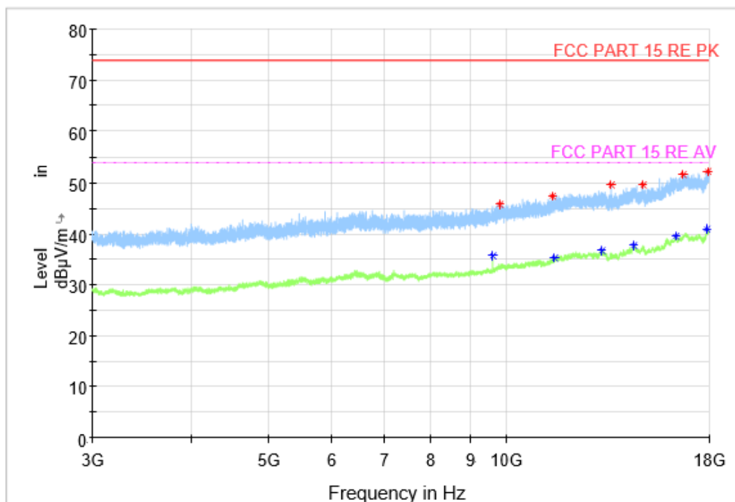
Fig.21 Radiated Spurious Emission (GFSK, Ch0, 3 GHz ~18 GHz), LE 1M
