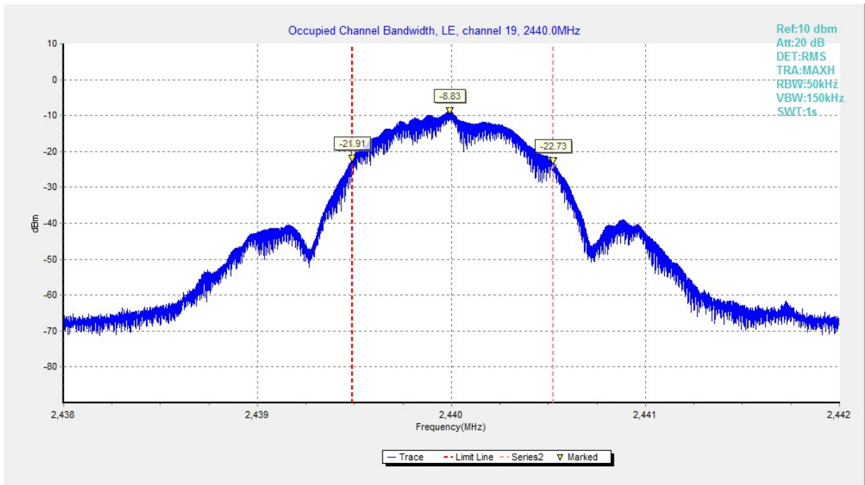
Fig.32 99% Occupied Bandwidth: GFSK, Channel 19, LE 1M
