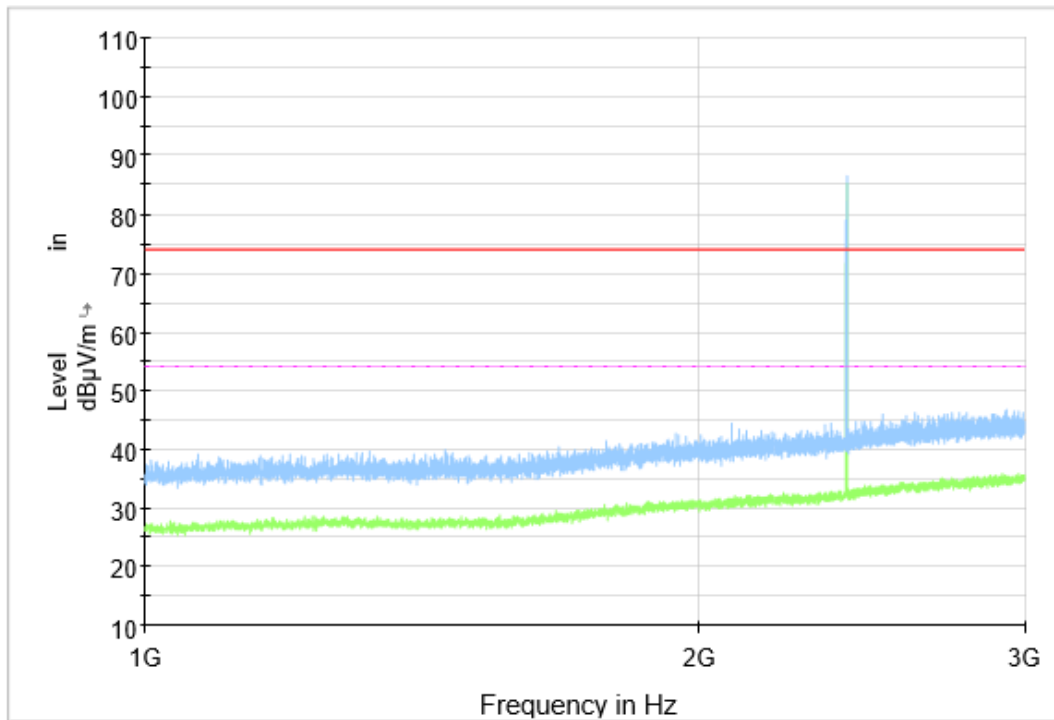
Fig.20 Radiated Spurious Emission (GFSK, Ch0, 1 GHz ~3 GHz), LE 1M
