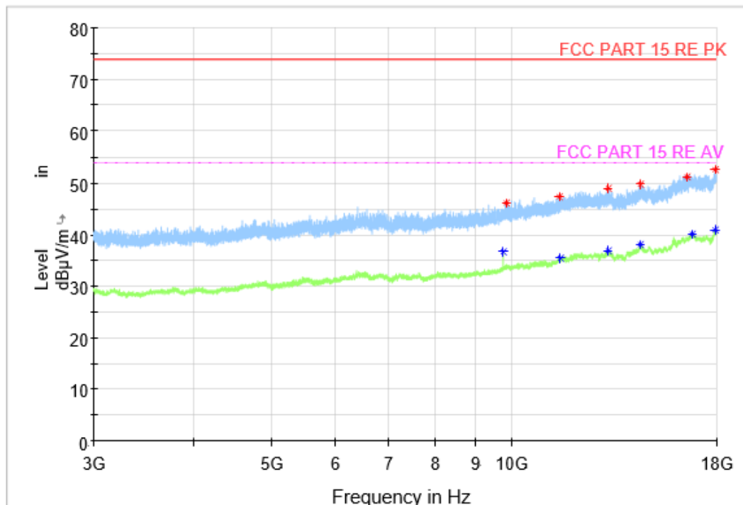
Fig.23 Radiated Spurious Emission (GFSK, Ch19, 3 GHz ~18 GHz), LE 1M
