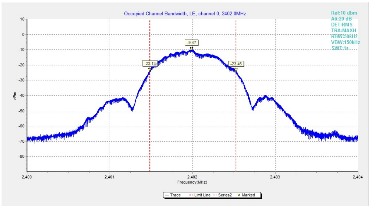
Fig.31 99% Occupied Bandwidth: GFSK, Channel 0, LE 1M
