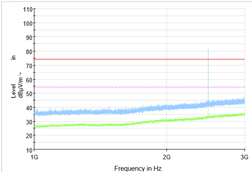
Fig.24 Radiated Spurious Emission (GFSK, Ch39, 1 GHz ~3 GHz), LE 1M
