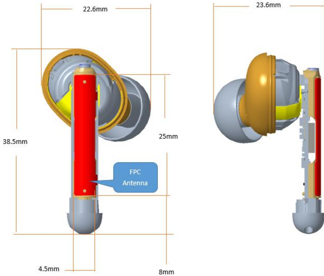
Antenna Location
