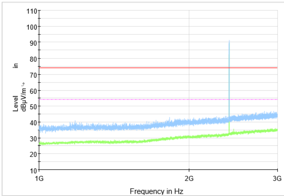
Fig.20 Radiated Spurious Emission (GFSK, Ch0, 1 GHz ~3 GHz), LE 1M
