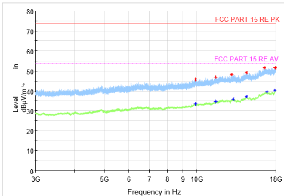
Fig.21 Radiated Spurious Emission (GFSK, Ch0, 3 GHz ~18 GHz), LE 1M
