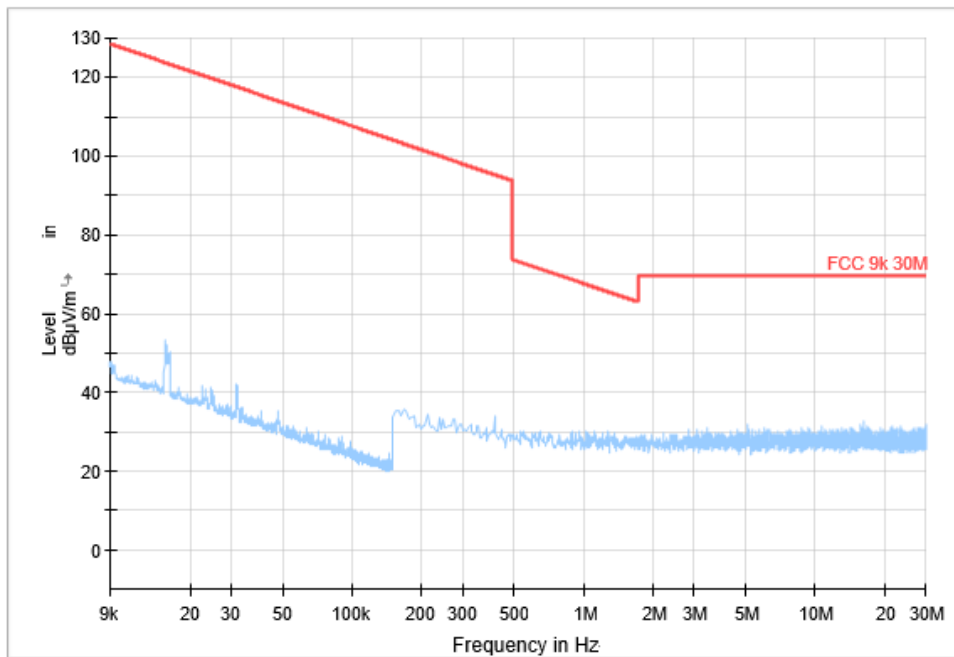
Fig.28 Radiated Spurious Emission (All Channels, 9 kHz-30 MHz), LE 1M
