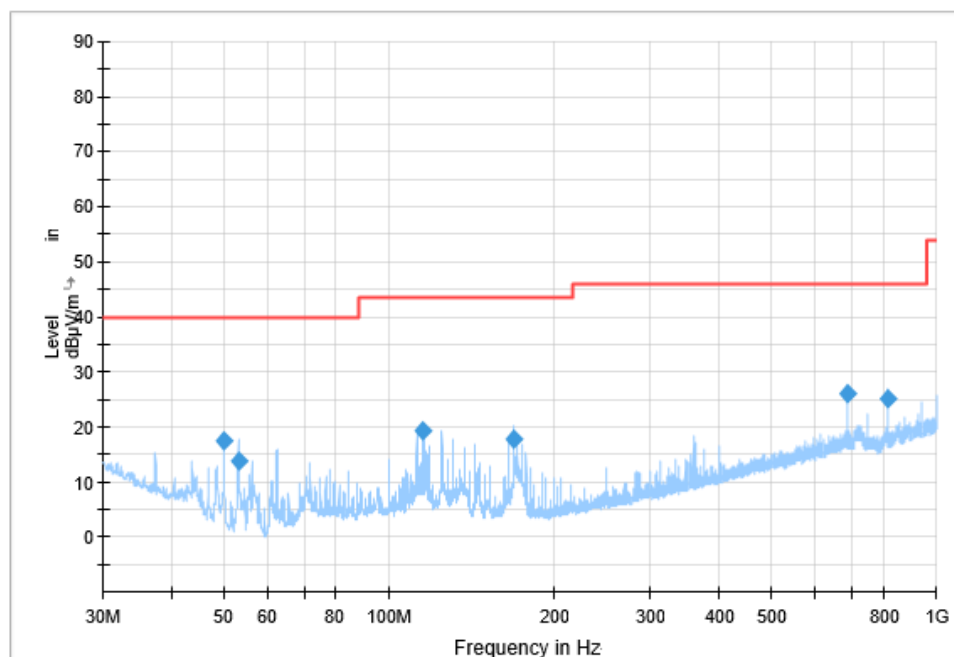
Fig.29 Radiated Spurious Emission (All Channels, 30 MHz-1 GHz), LE 1M
