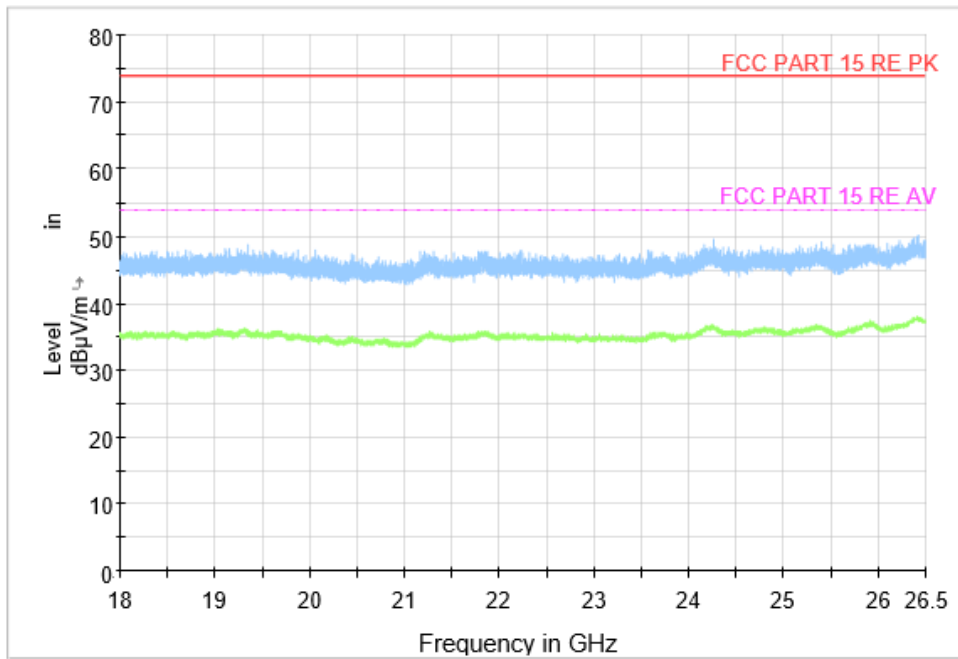
Fig.30 Radiated Spurious Emission (All Channels, 18 GHz-26.5 GHz), LE 1M
