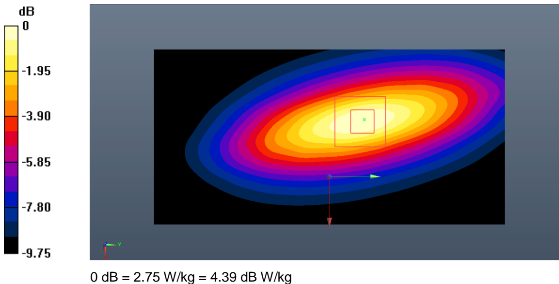
Fig.B.2. Validation 750MHz 250mW
