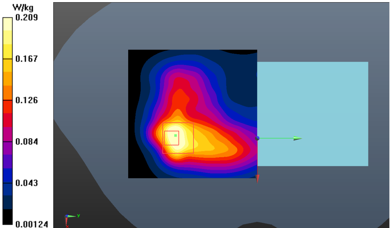
Fig.24 WLAN 2.4G Body
