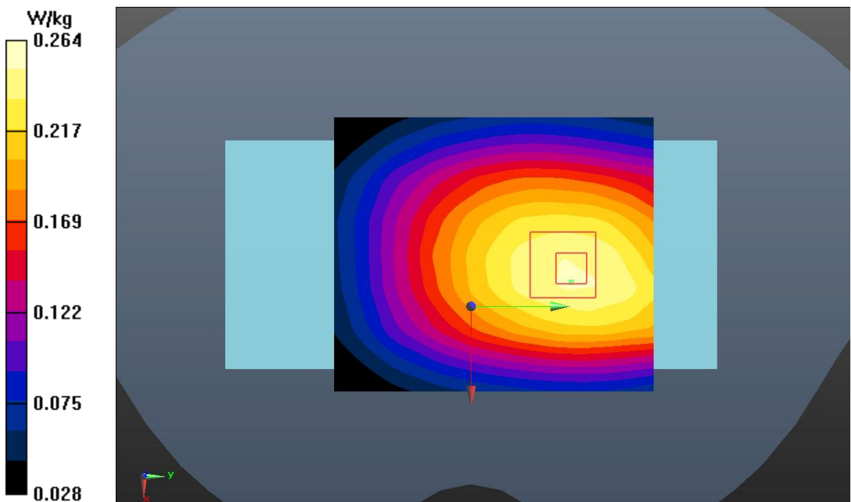
Fig.20 LTE Band 28 Body
