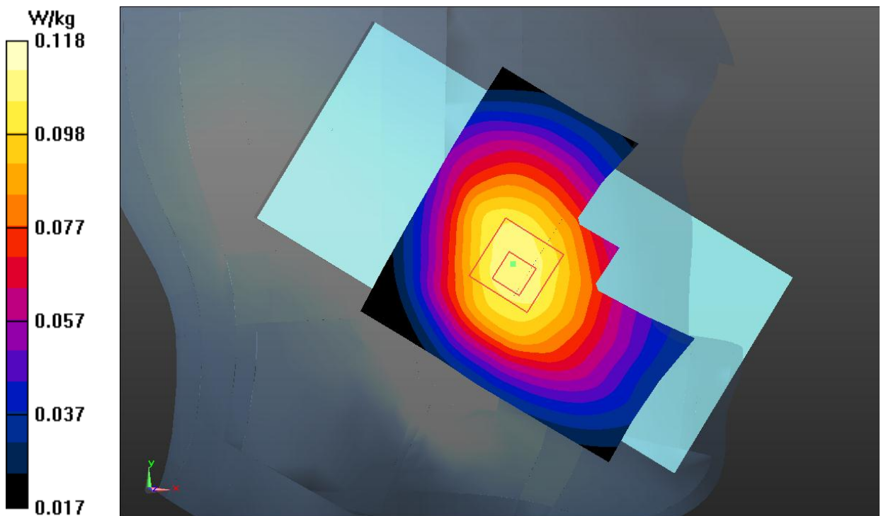
Fig.19 LTE Band 28 Head
