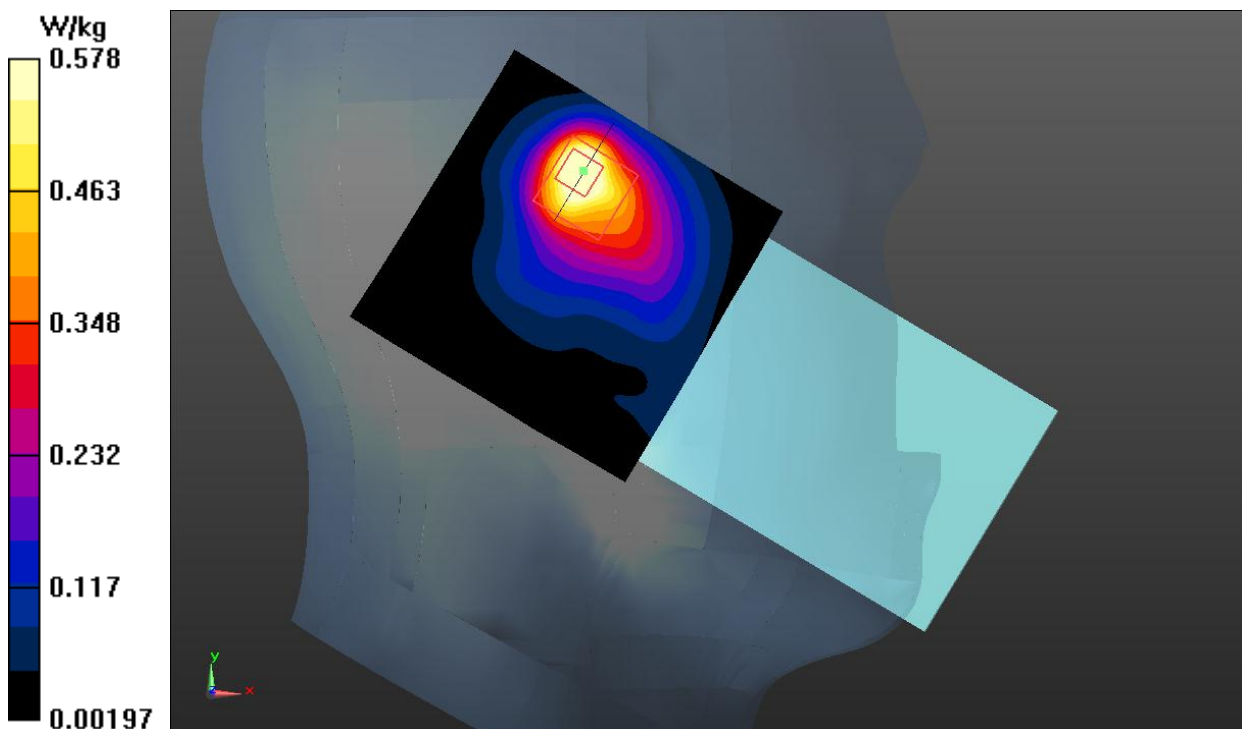
Fig.23 WLAN 2.4G Head
