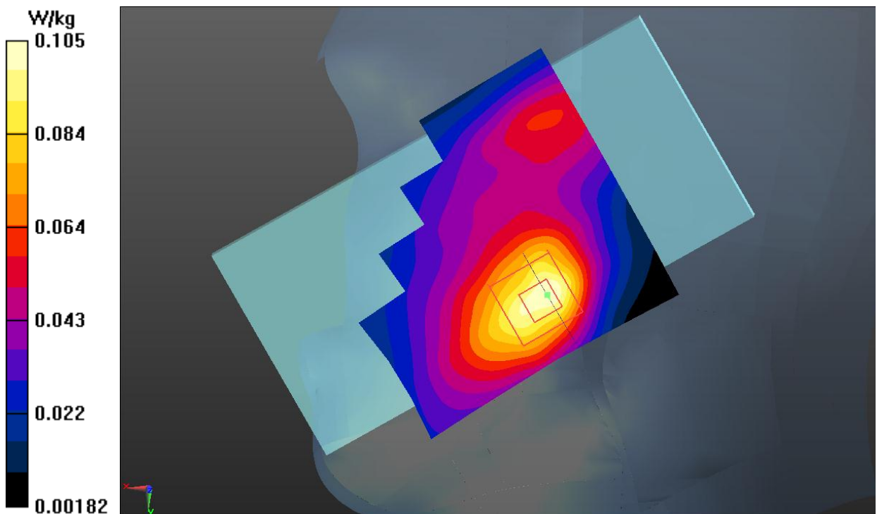
Fig.3 GSM 1900 Head
