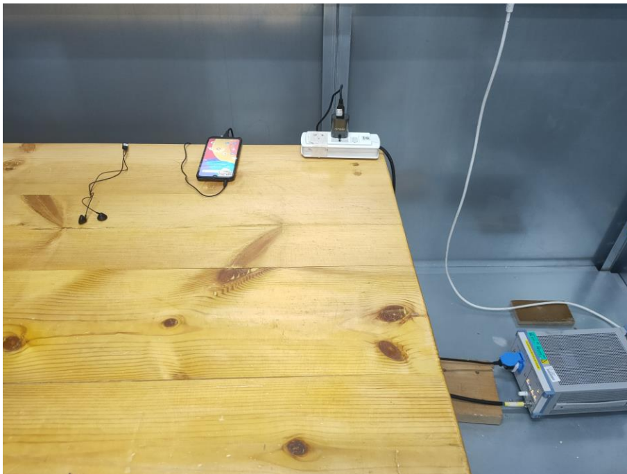
16. Conducted Emission (Part 15C, Bluetooth/Wi-Fi)
