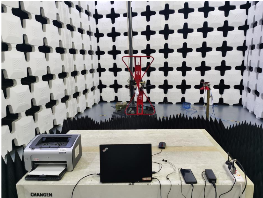
4. Radiated Emissions (Part 15B Bluetooth/Wi-Fi ,1GHz-18GHz)
