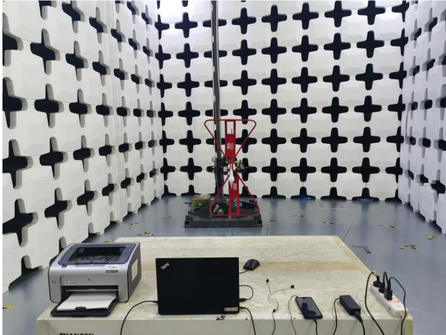
3. Radiated Emissions (Part 15B Bluetooth/Wi-Fi ,30MHz-1GHz)
