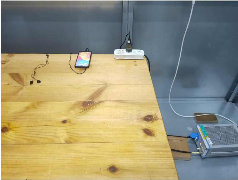
13. Conducted Emission (Part 15B, Camera/Video Player/GNSS/ FM receiver)
