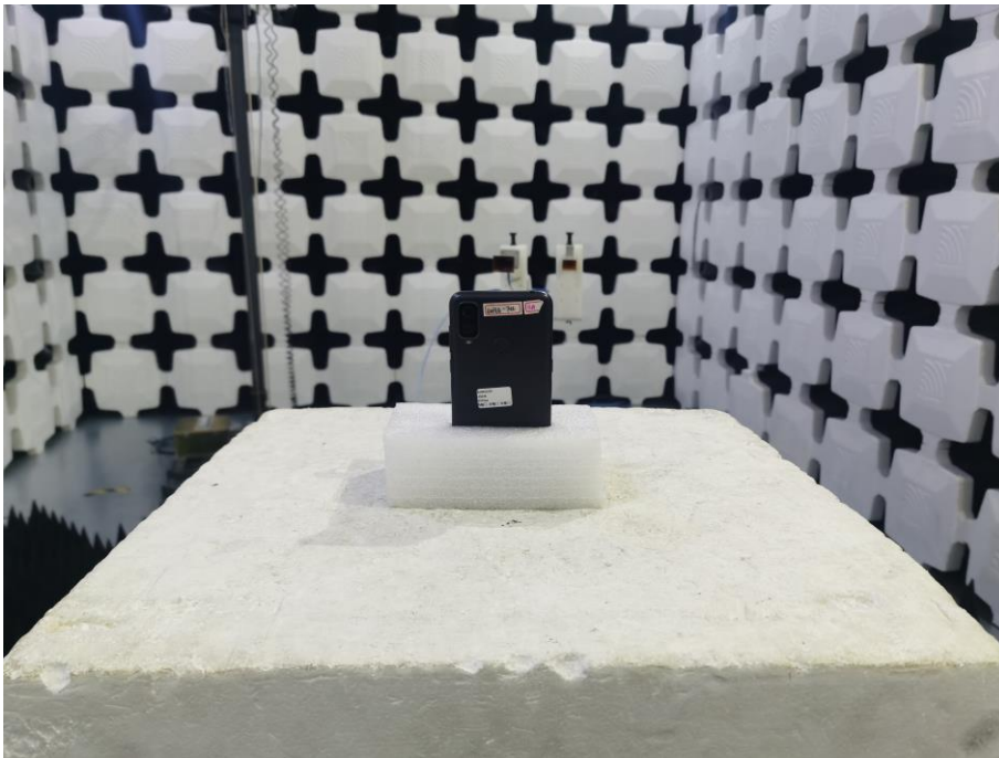
12. Radiated Emissions (Part 22/24/27, 18GHz -26.5GHz)
