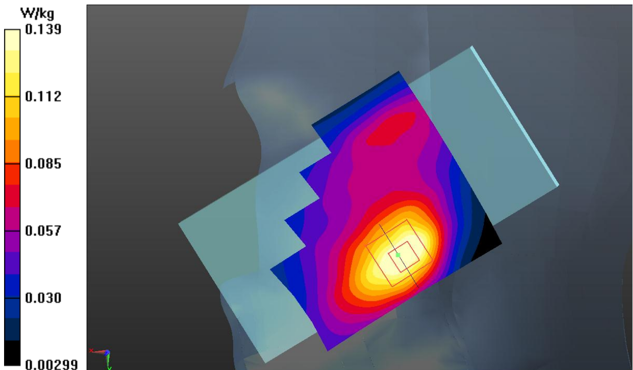
Fig.11 LTE Band 2 Head
