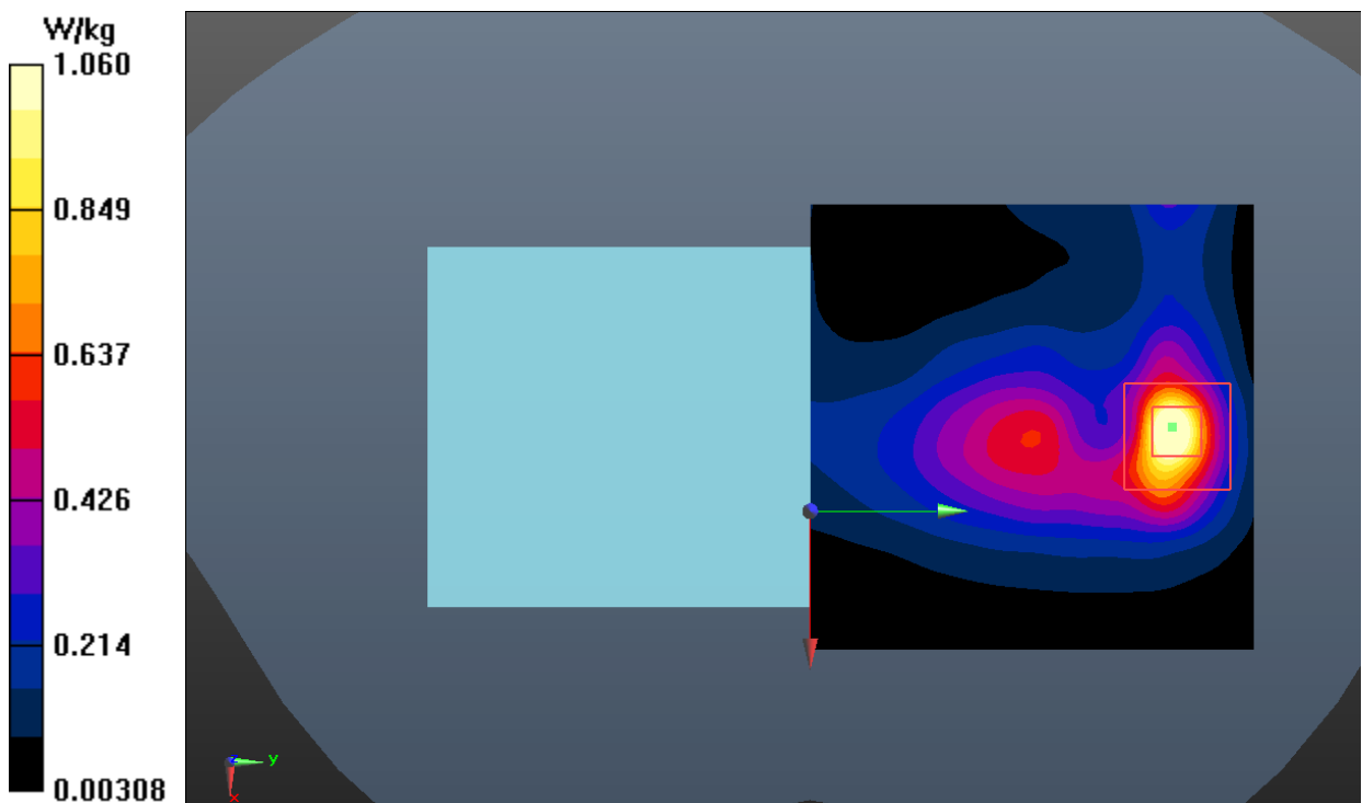
Fig.16 LTE Band 7 Body
