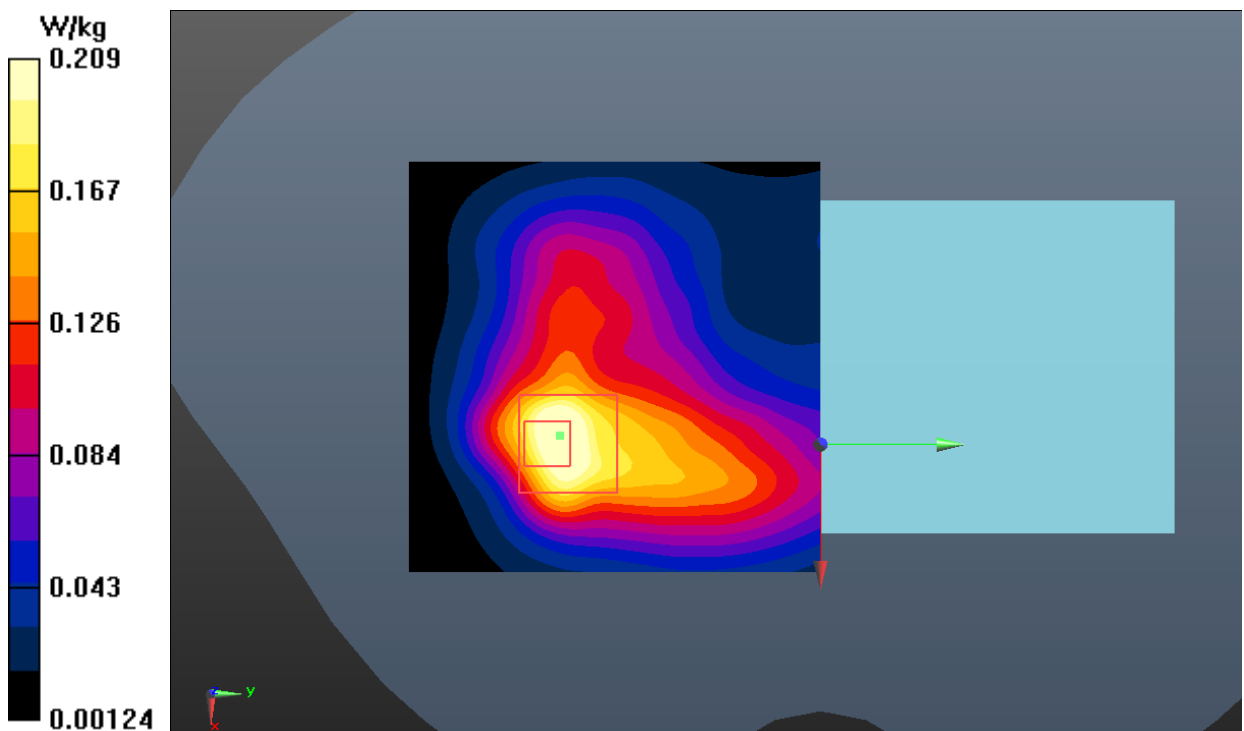
Fig.22 WLAN 2.4G Body
