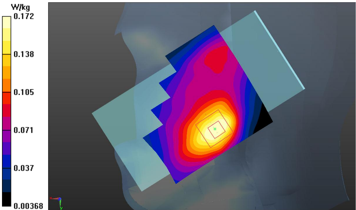
Fig.19 LTE Band 66 Head
