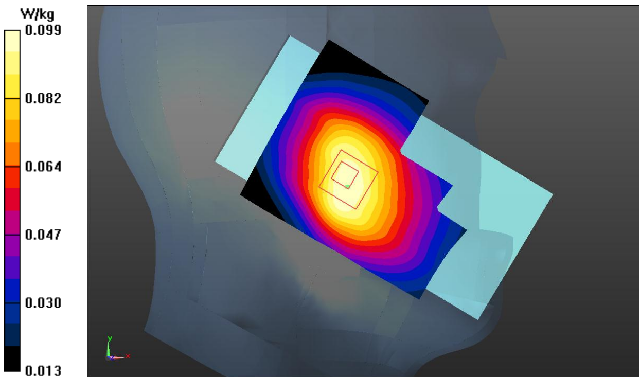
Fig.17 LTE Band 12 Head
