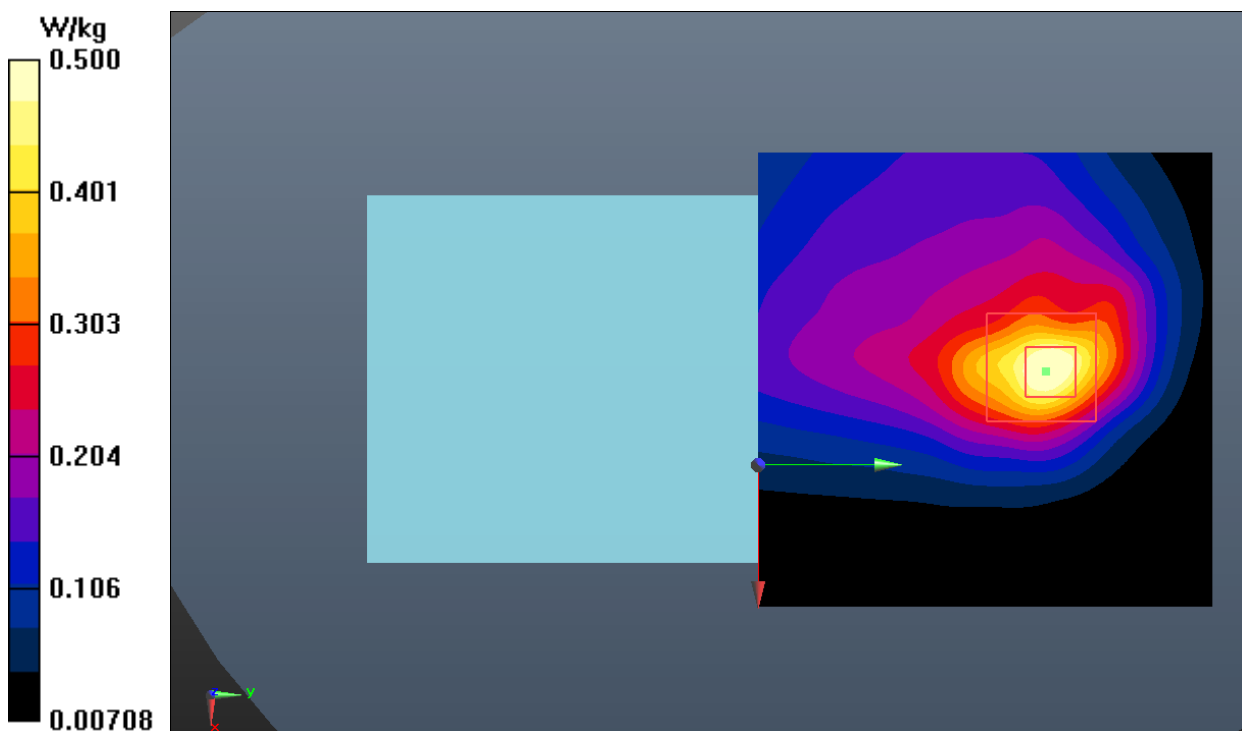
Fig.12 LTE Band 2 Body
