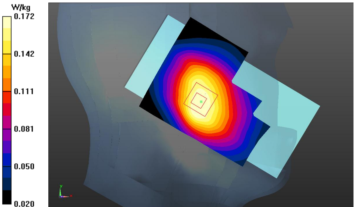
Fig.13 LTE Band 5 Head
