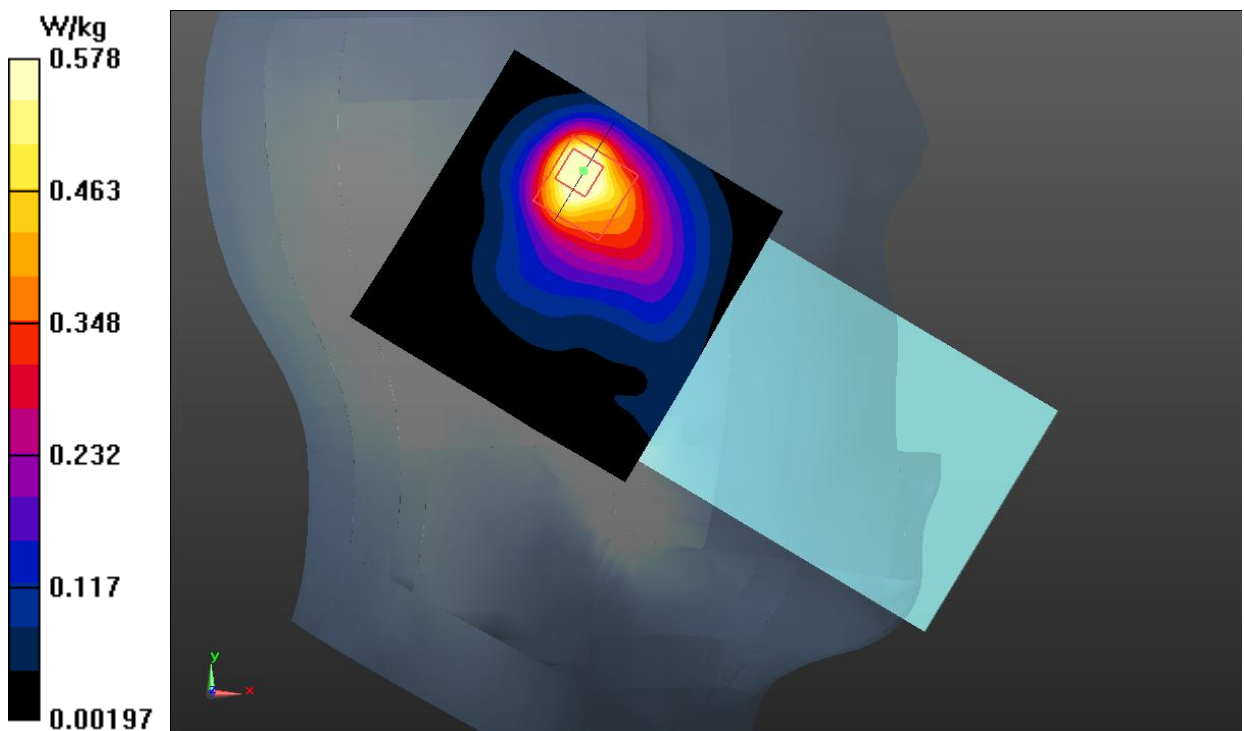
Fig.21 WLAN 2.4G Head
