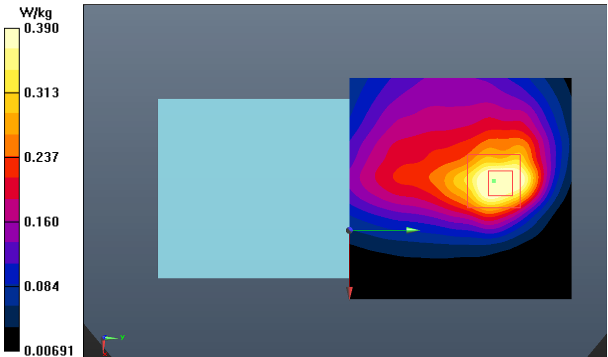
Fig.20 LTE Band 66 Body
