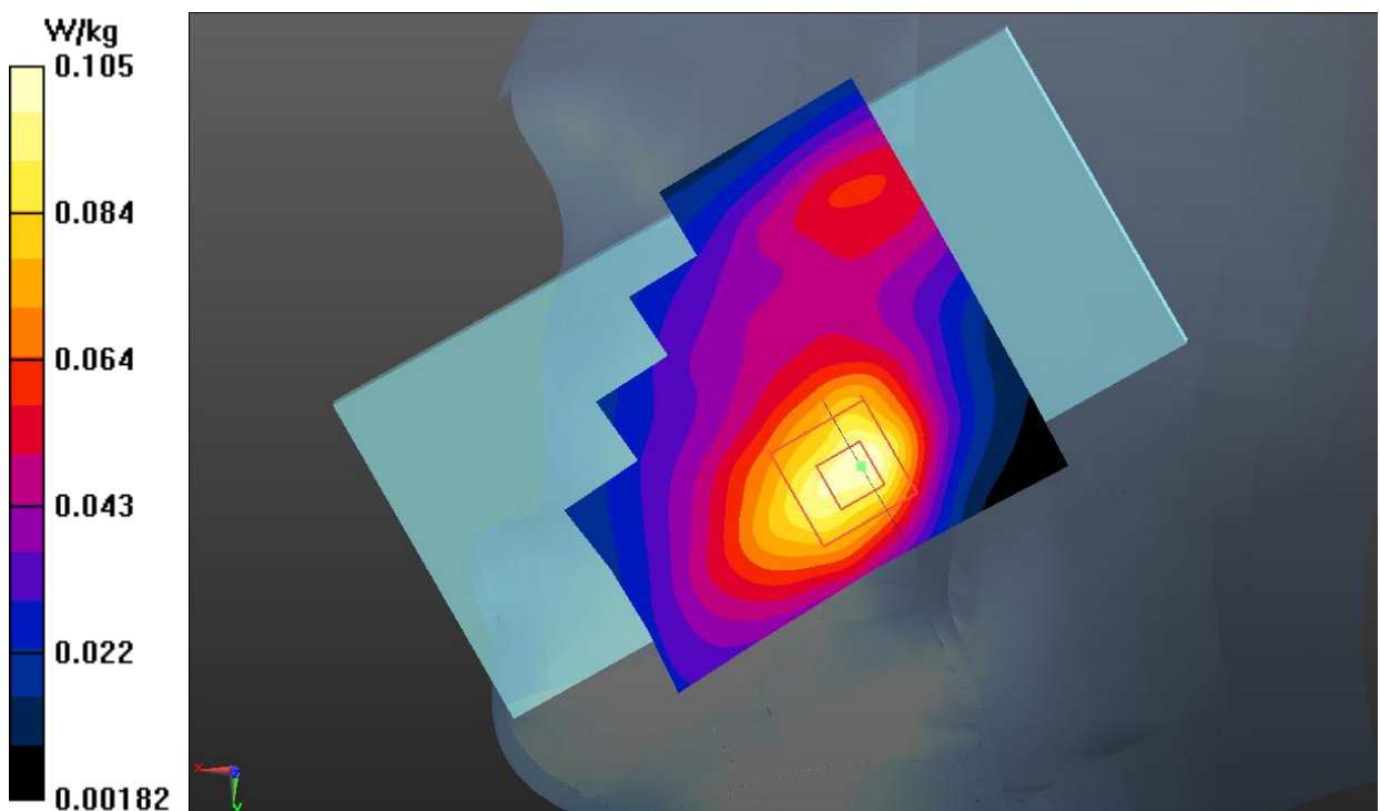
Fig.3 GSM 1900 Head
