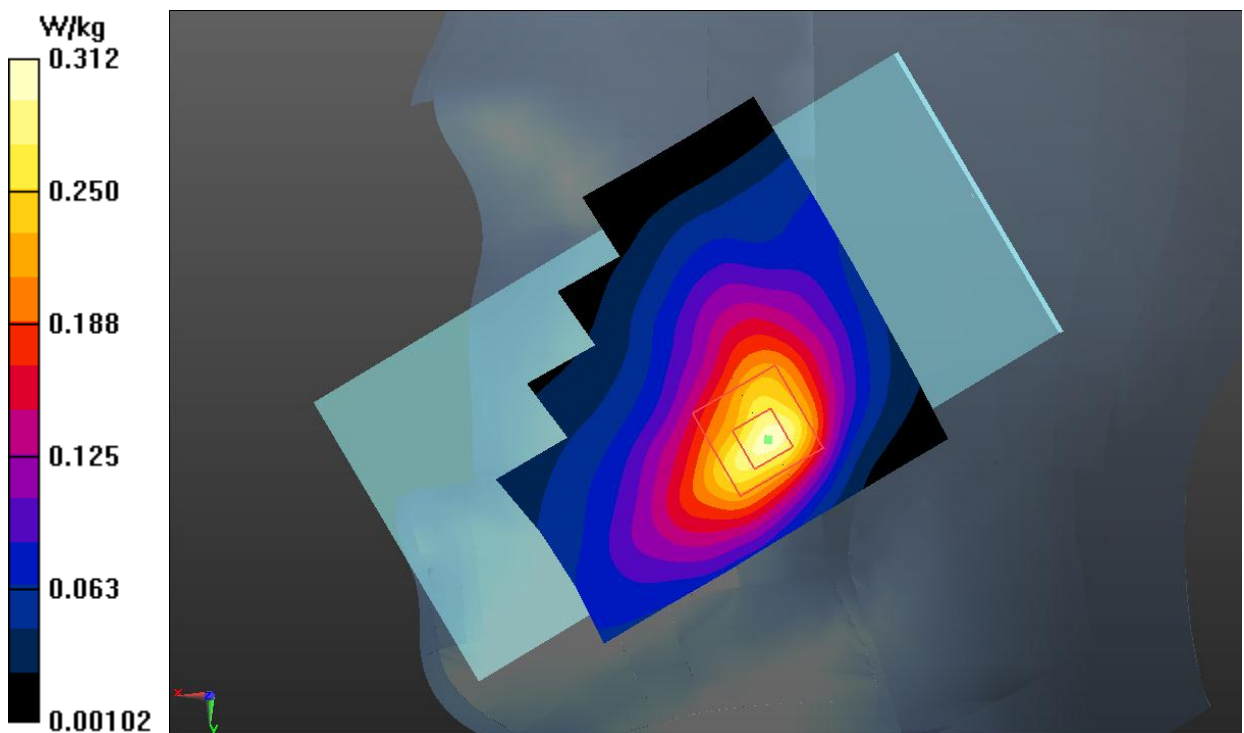
Fig.15 LTE Band 7 Head
