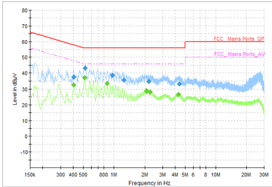
Fig. 85 AC Power line Conducted Emission (Idle, AE2, 120V)
