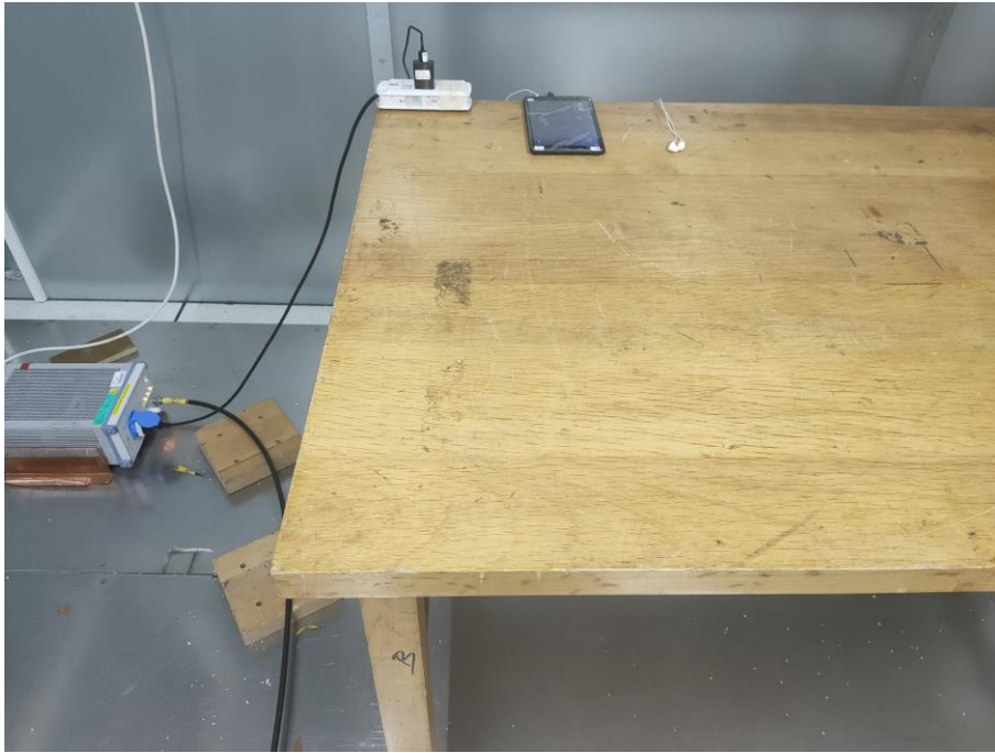
9. Conducted Emission (Part 15B, FM receiver)
