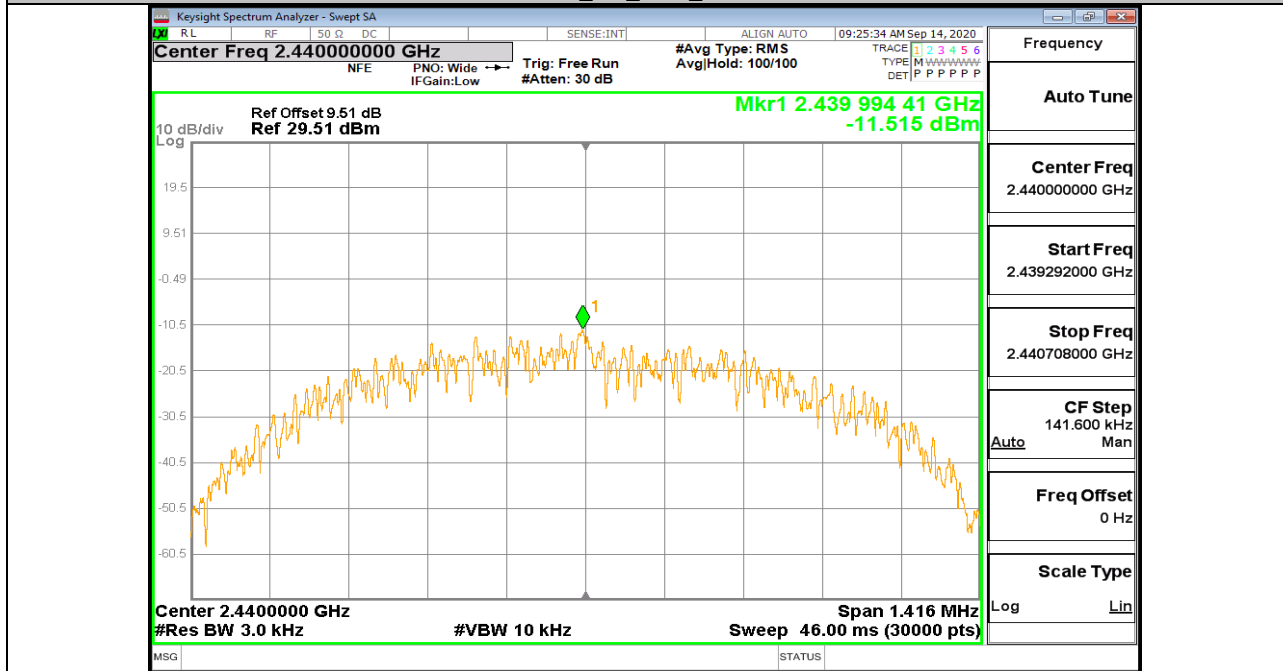
BLE_1M_Ant1_2440
