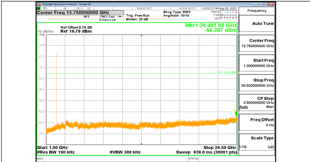
BLE_1M_Ant1_2402_1000~26500
