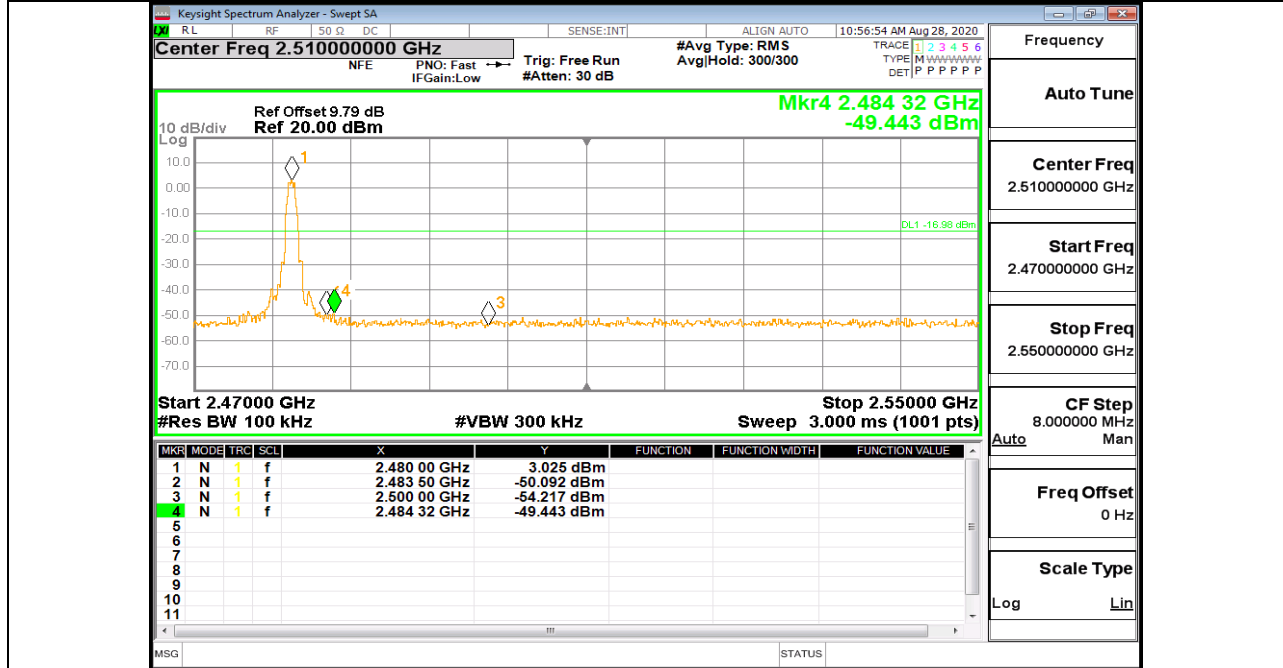
BLE_1M_Ant1_High_2480
