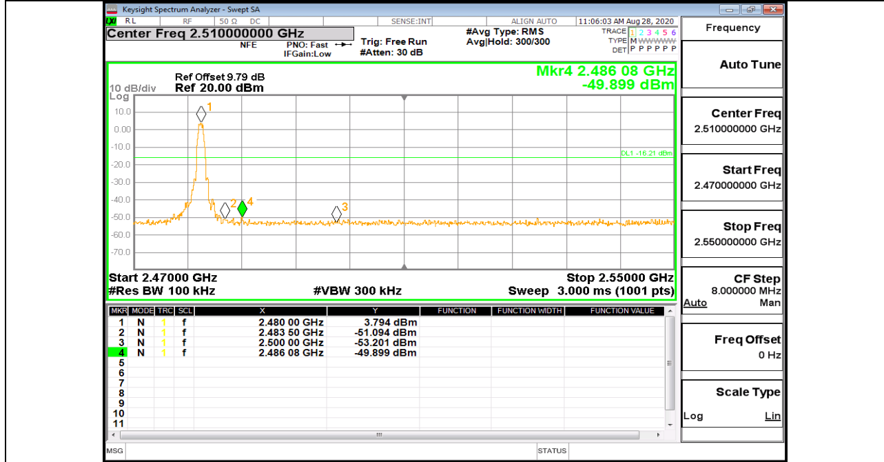
BLE_1M_Ant1_High_2480
