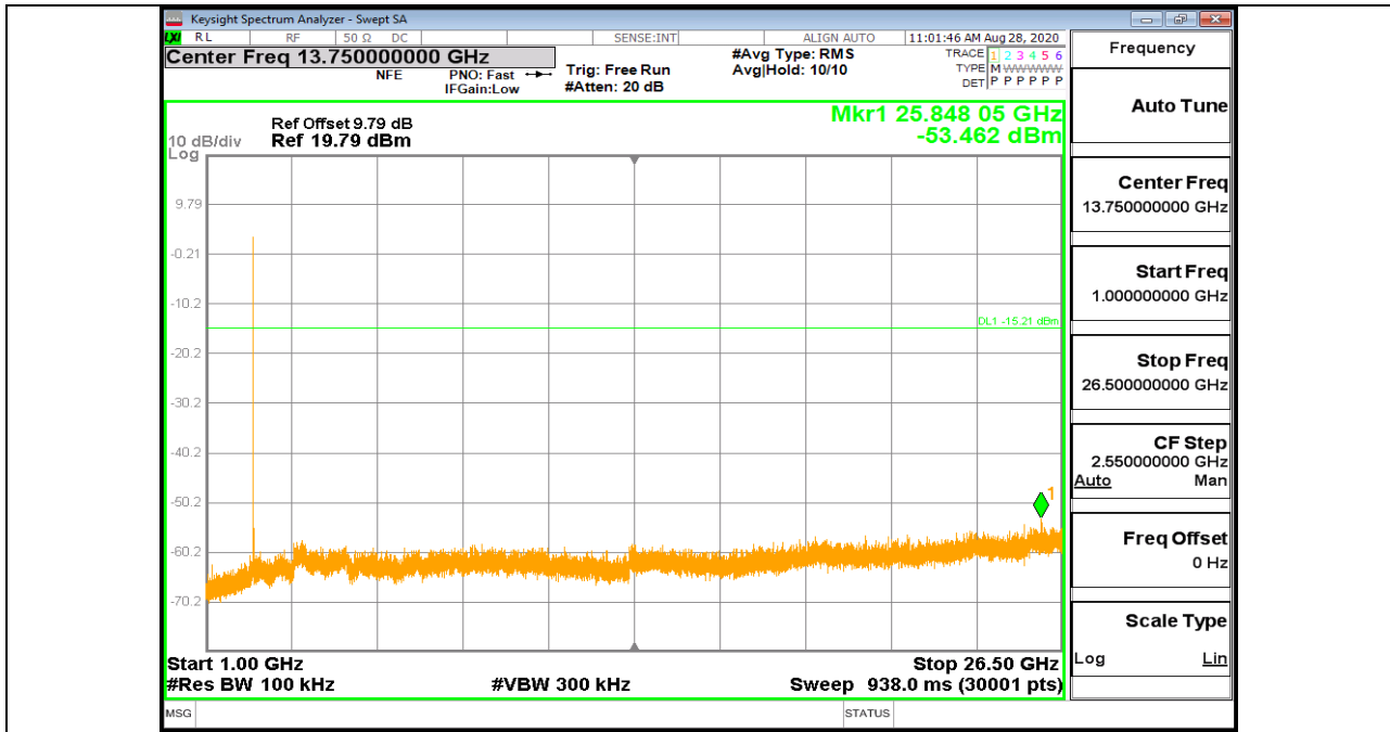
BLE_1M_Ant1_2402_1000~26500
