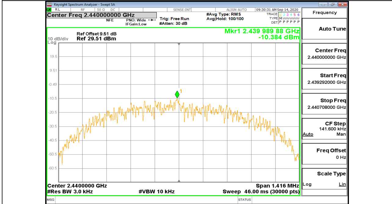
BLE_1M_Ant1_2440
