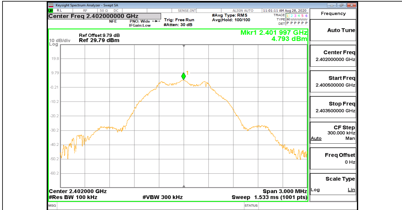
BLE_1M_Ant1_2402_0~Reference
