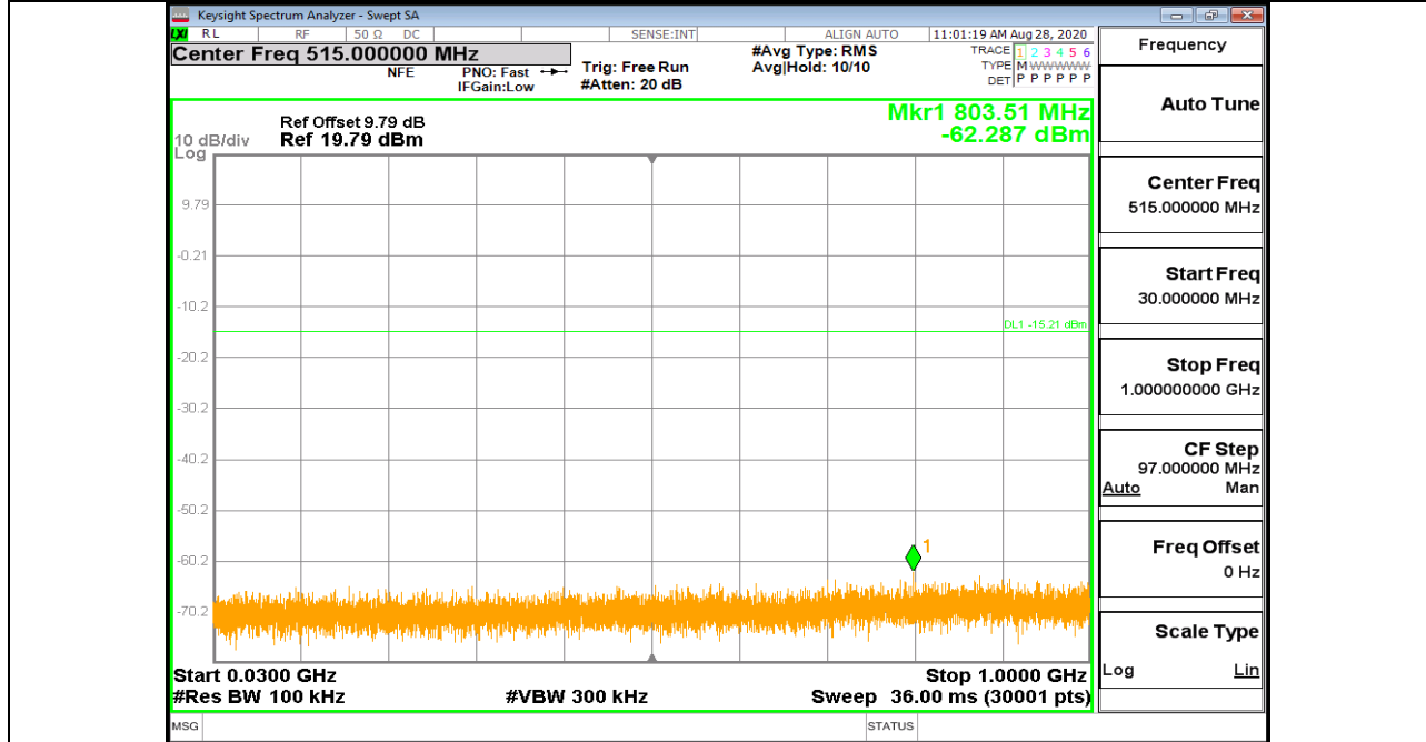
BLE_1M_Ant1_2402_30~1000
