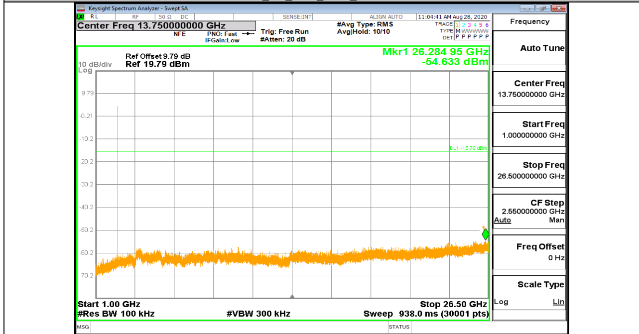
BLE_1M_Ant1_2440_1000~26500
