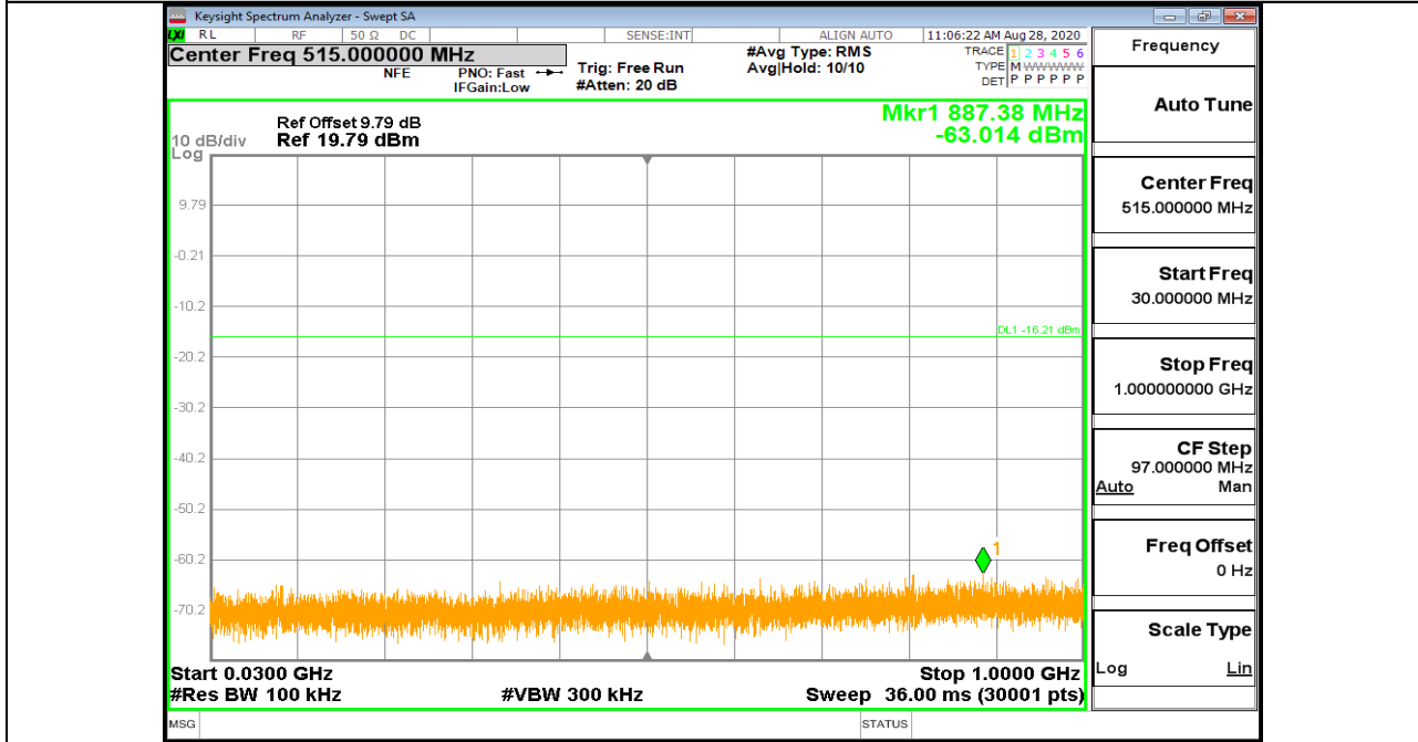
BLE_1M_Ant1_2480_30~1000
