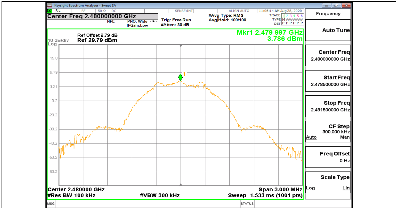
BLE_1M_Ant1_2480_0~Reference
