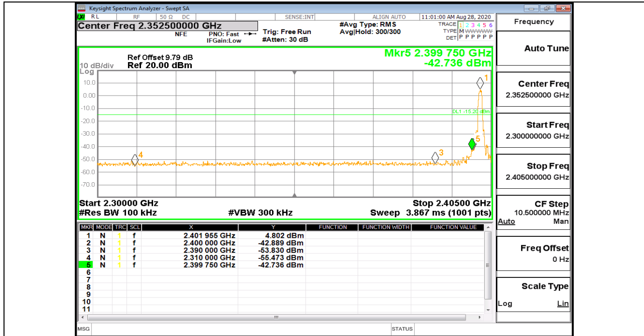
BLE_1M_Ant1_Low_2402
