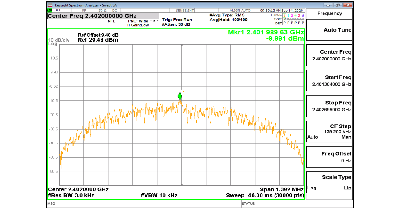
BLE_1M_Ant1_2402
