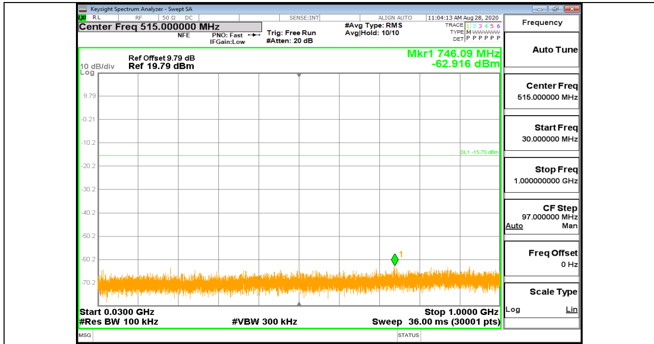
BLE_1M_Ant1_2440_30~1000
