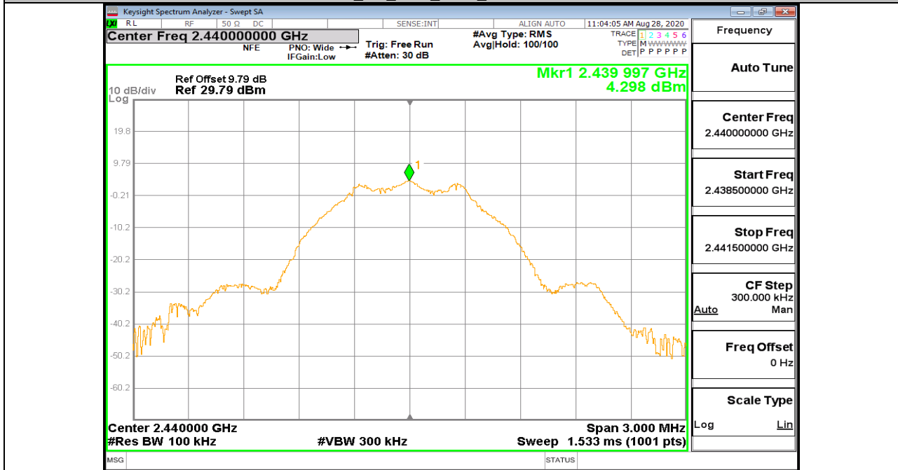
BLE_1M_Ant1_2440_0~Reference
