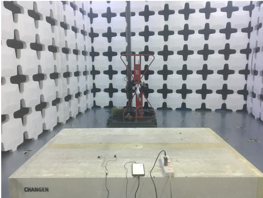
3. Radiated Emissions (Part 15B, Camera/Video Player/GSM receiver/WCDMA receiver/LTE receiver/FM receiver,30MHz-1GHz)
