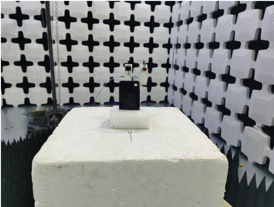
10. Radiated Emissions (Part 22/24/27/90, 18GHz -26.5GHz)
