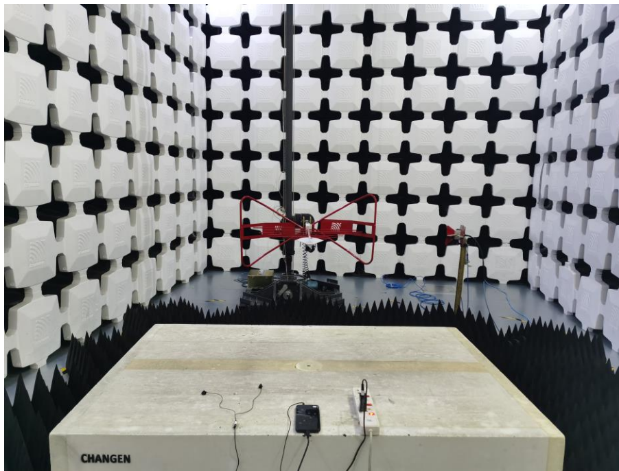
4. Radiated Emissions (Part 15B, Camera/Video Player/GSM receiver/WCDMA receiver/LTE receiver/FM receiver,1GHz-18GHz)
