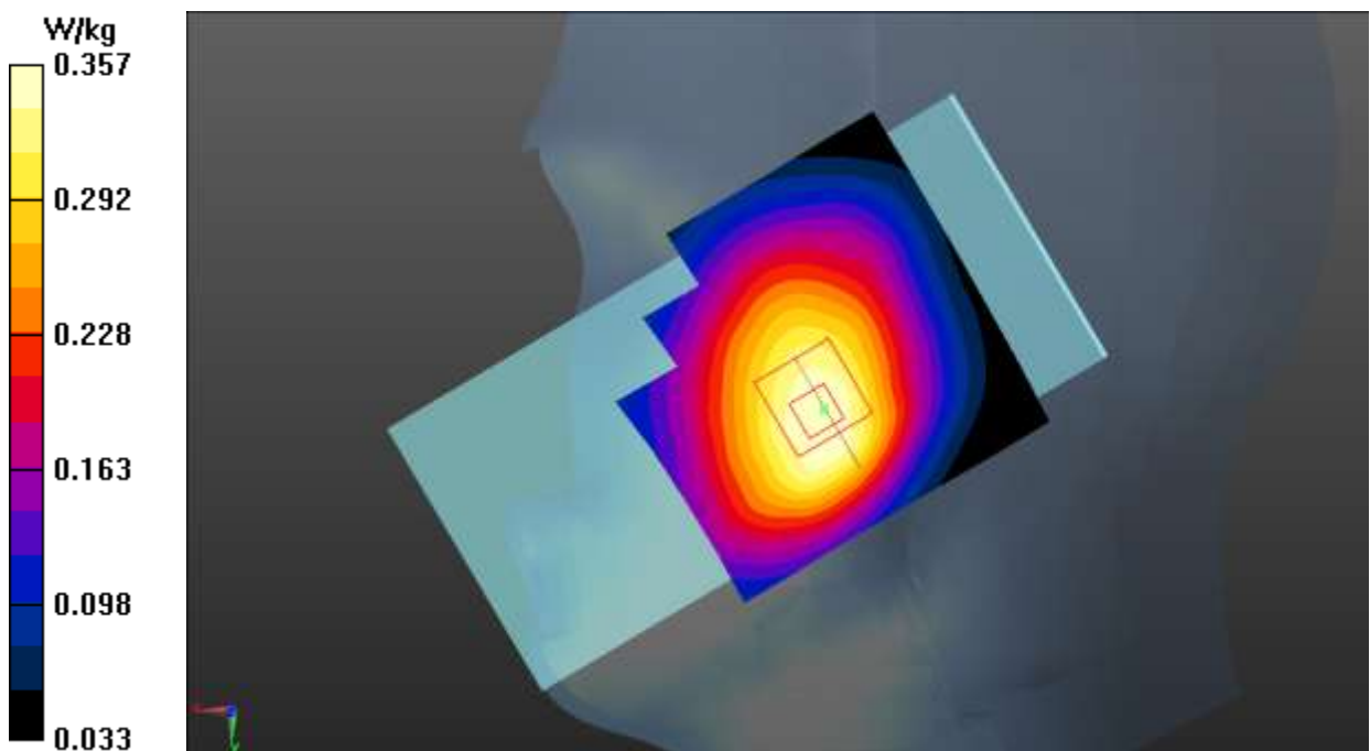
Fig.1 GSM 850 Head
